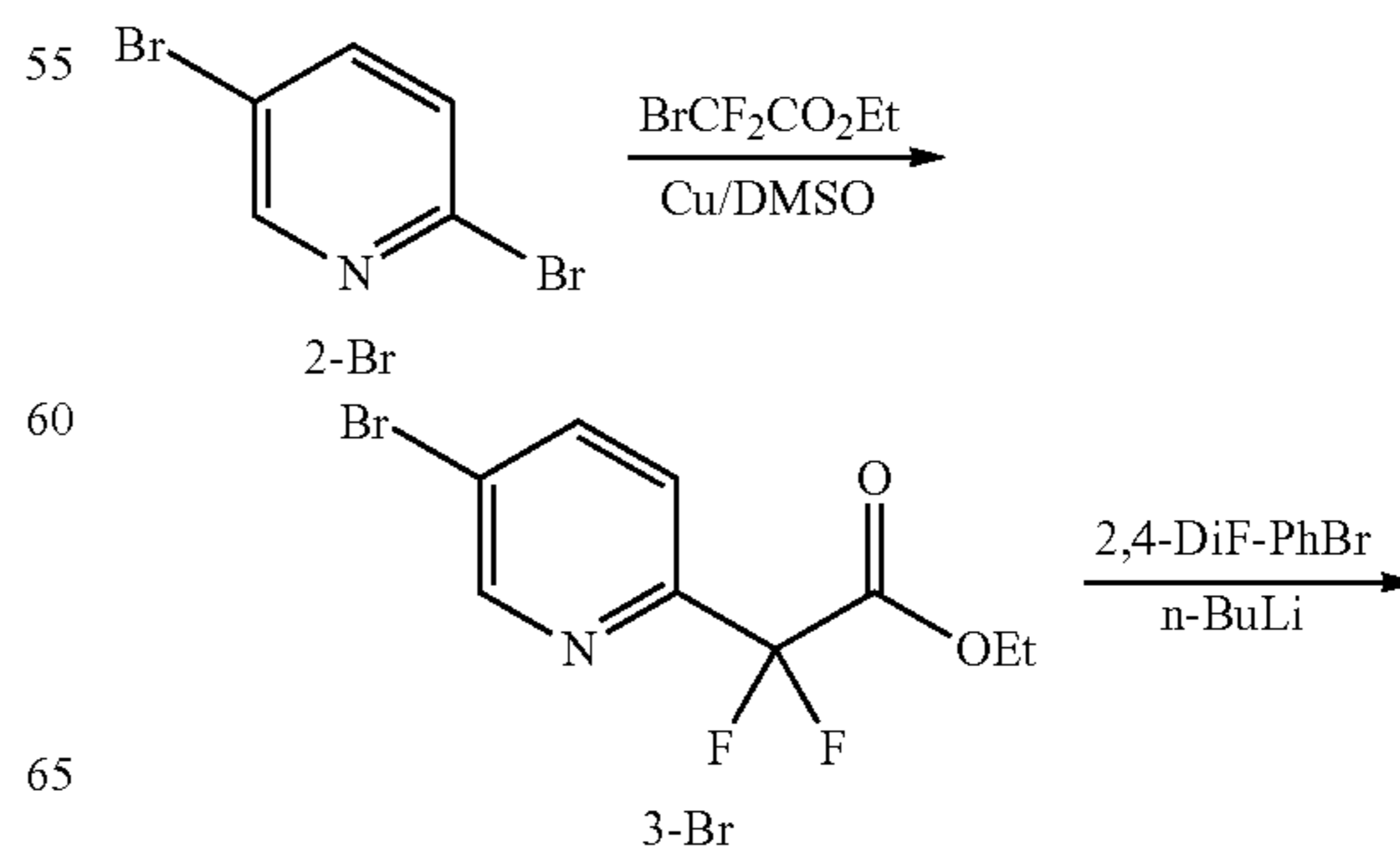
Scheme 5. Synthesis of ketone 15-Br
