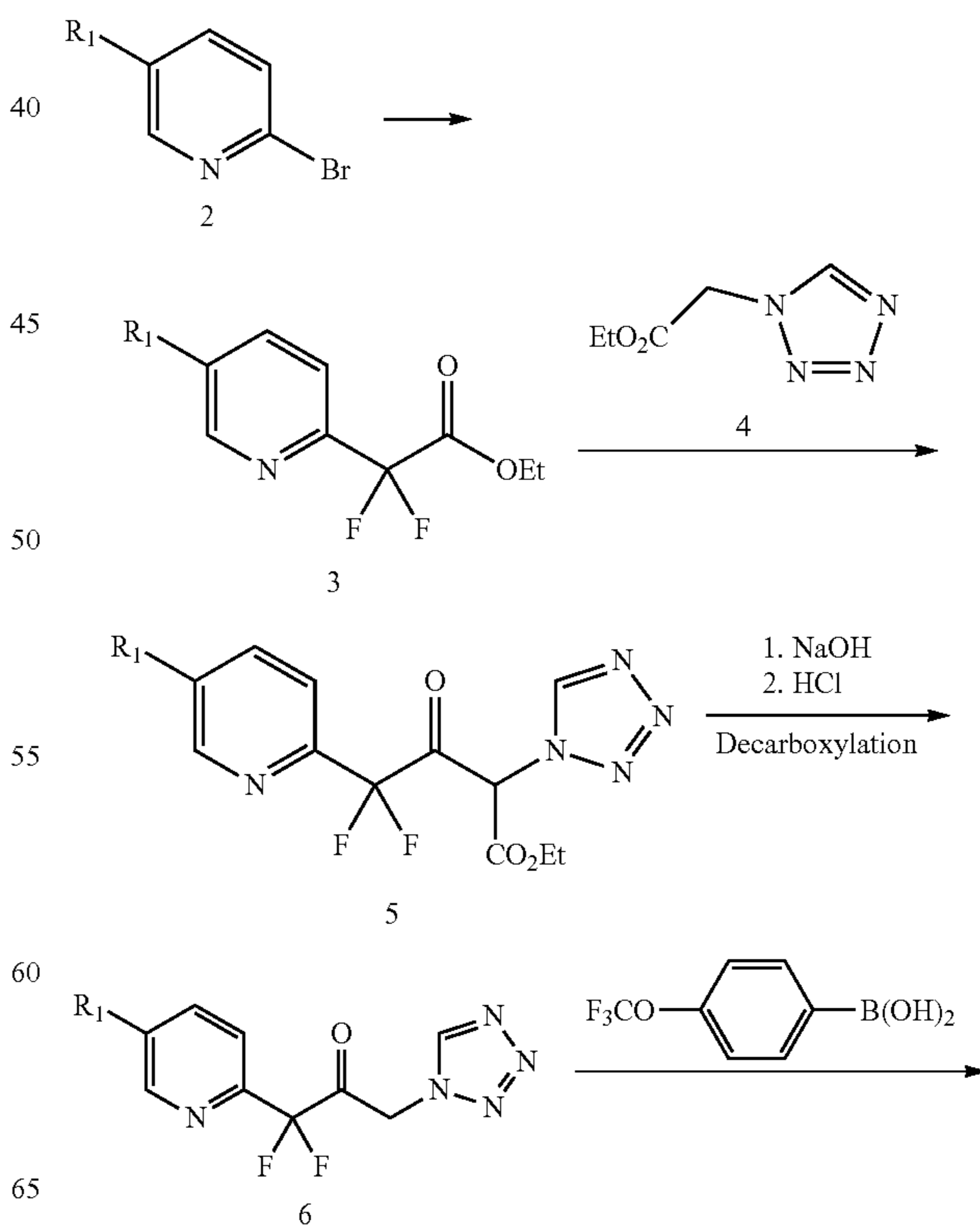
Scheme 2. Synthesis of ketone 8
