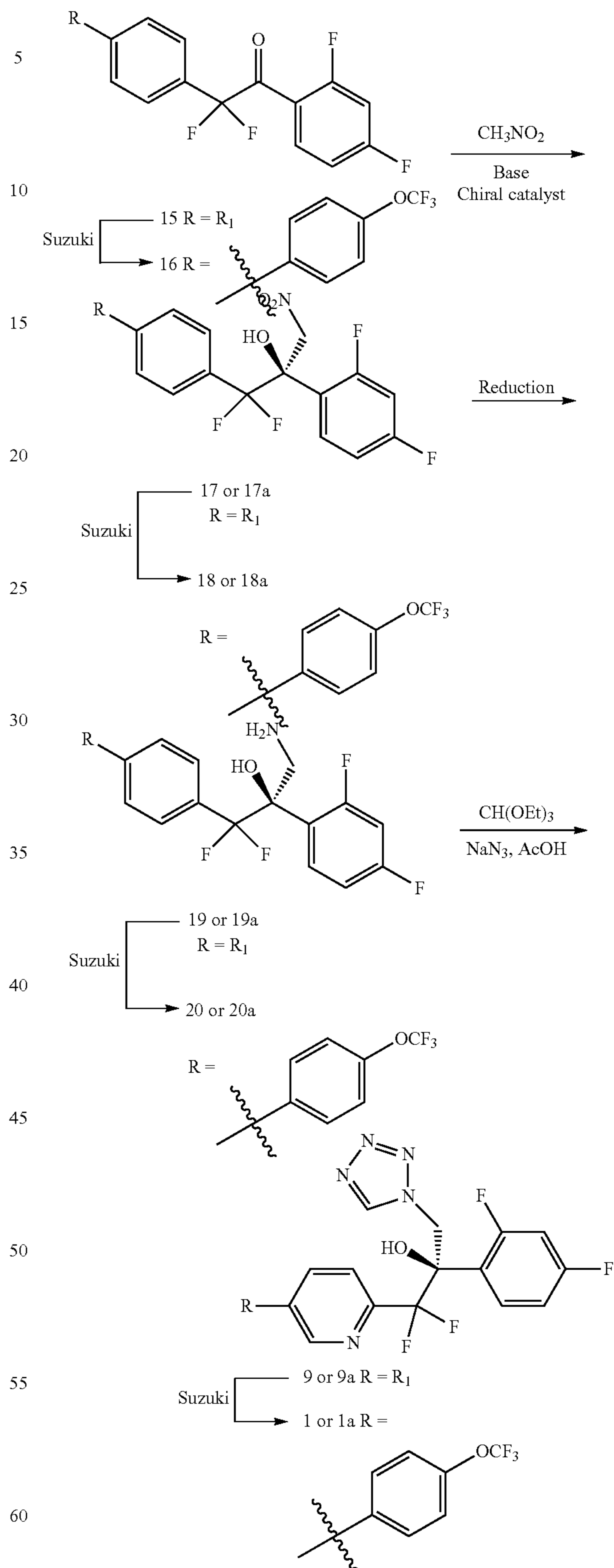
Scheme 7. Asymmetric Henry reaction
