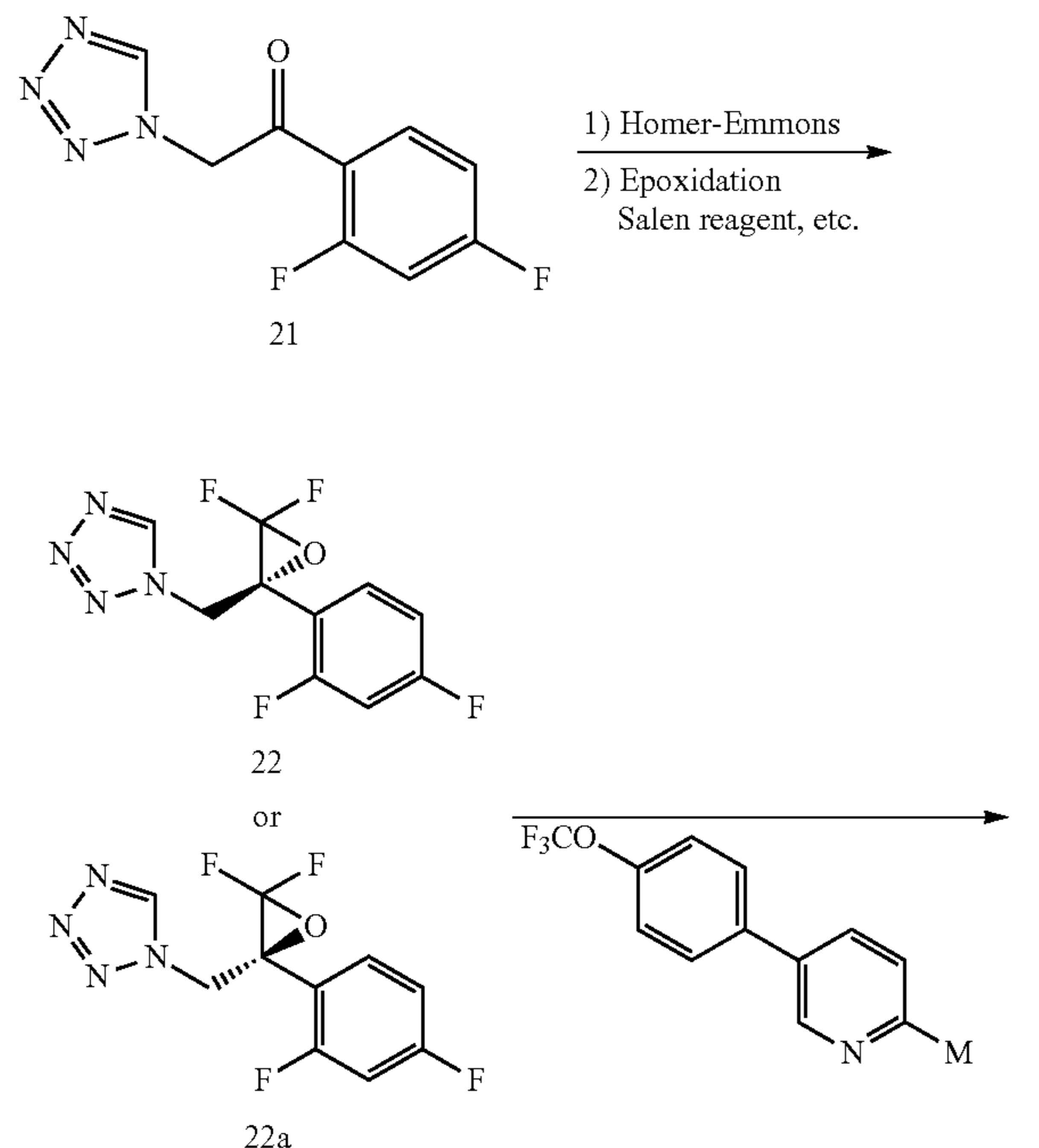
Scheme 8. Enantioselective epoxidation strategy
