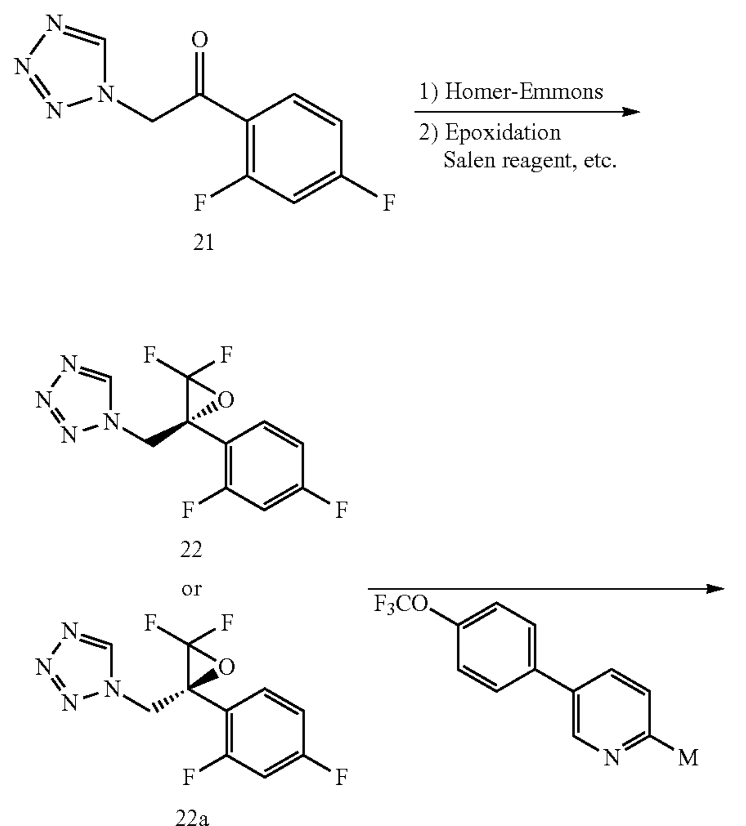
Scheme 8. Enantioselective epoxidation strategy
