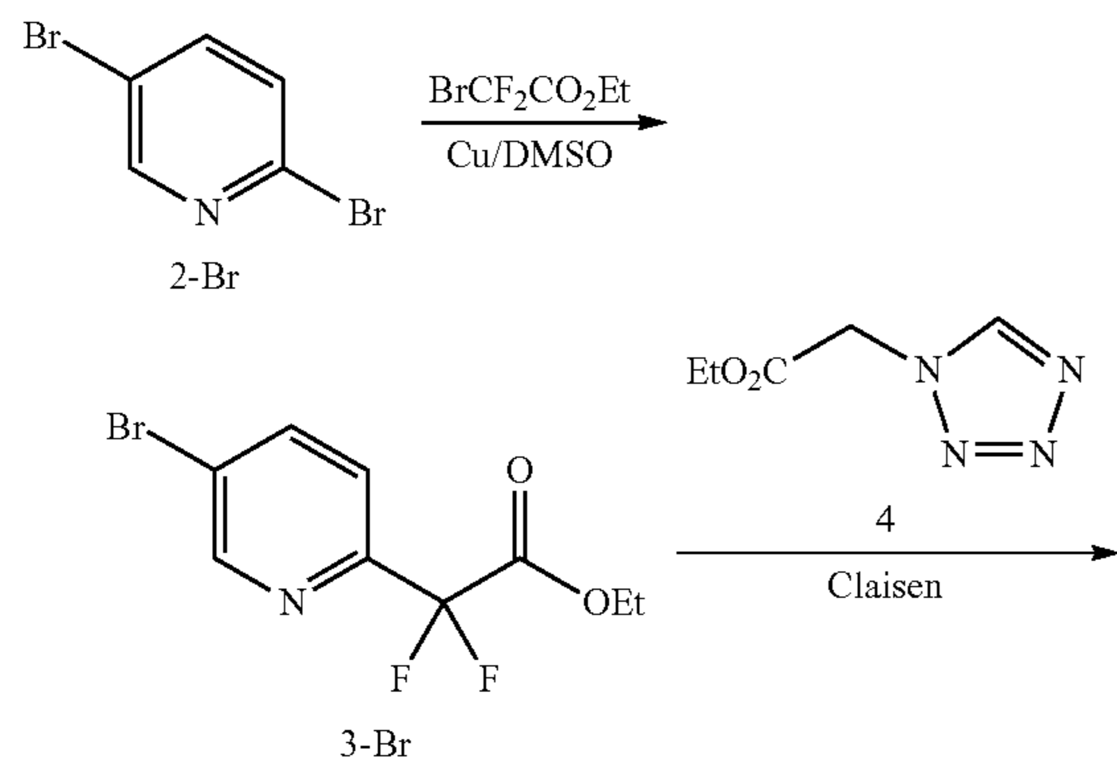
Scheme 1. Synthesis of ketone 8
