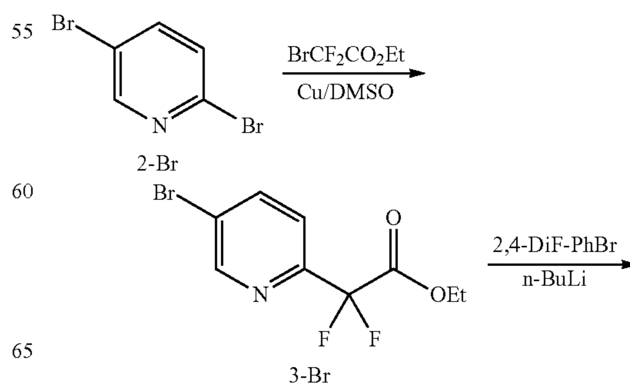
Scheme 5. Synthesis of ketone 15-Br
