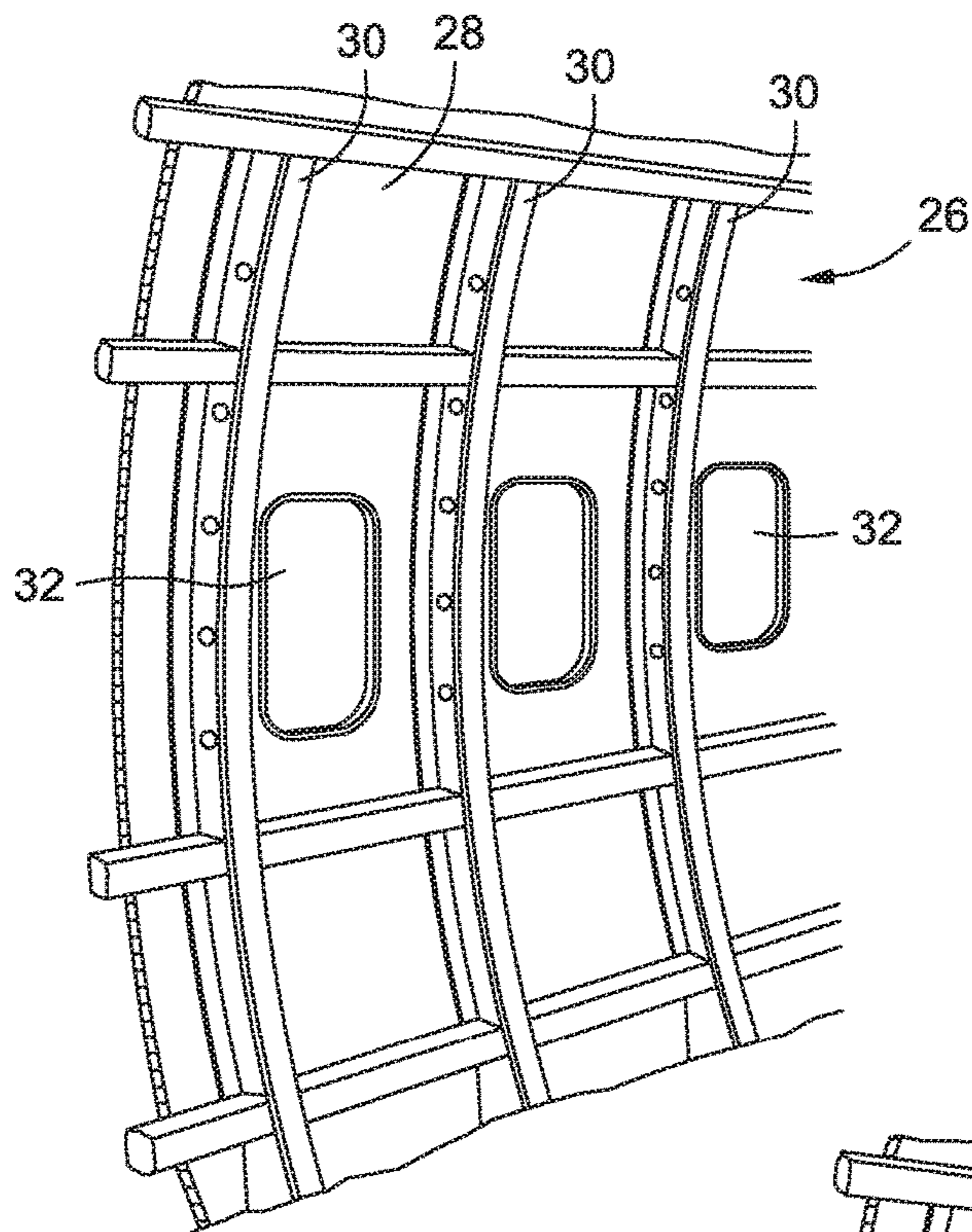
FIG. 2 (PRIOR ART)
