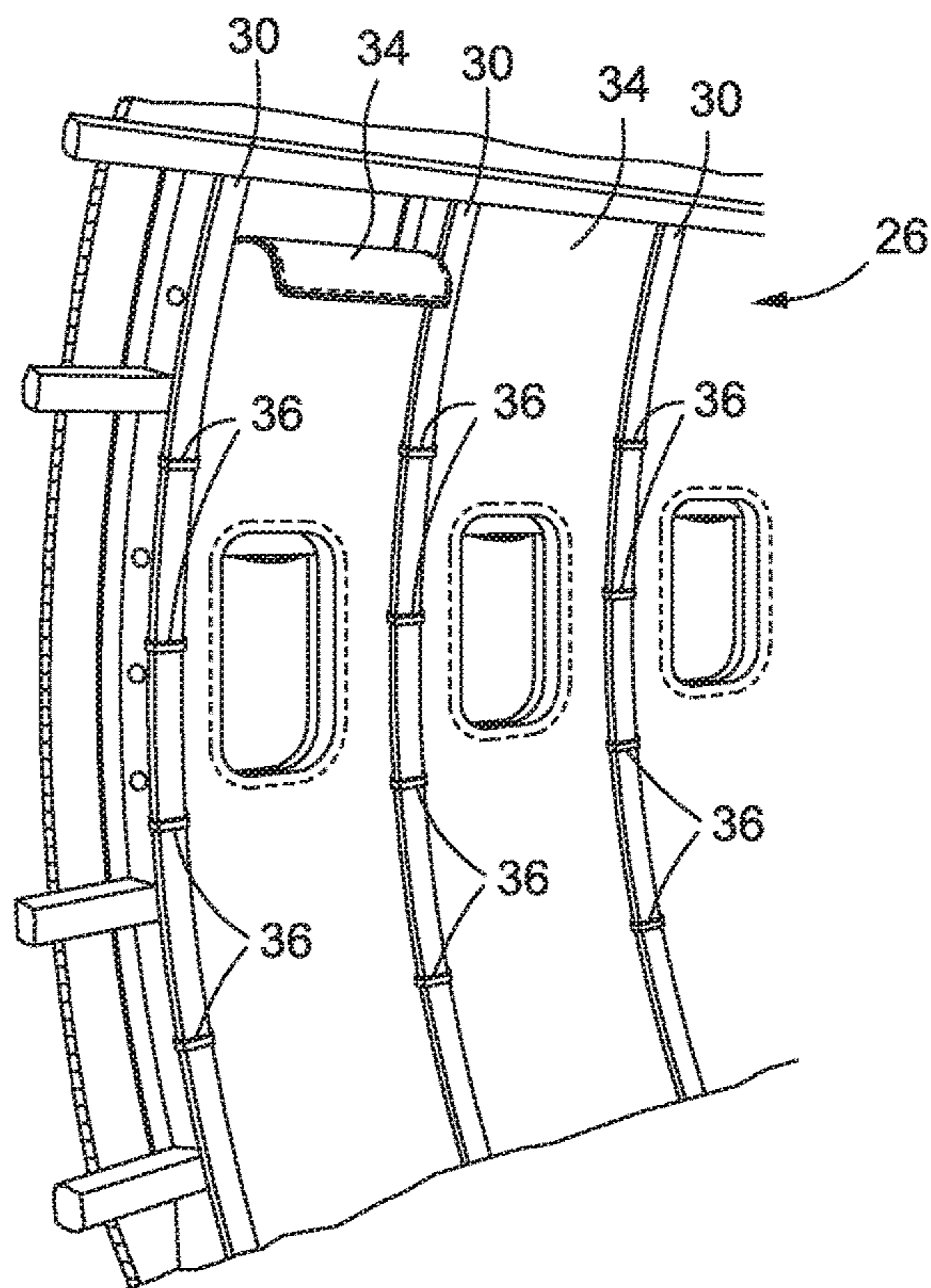
FIG. 3 (PRIOR ART)
