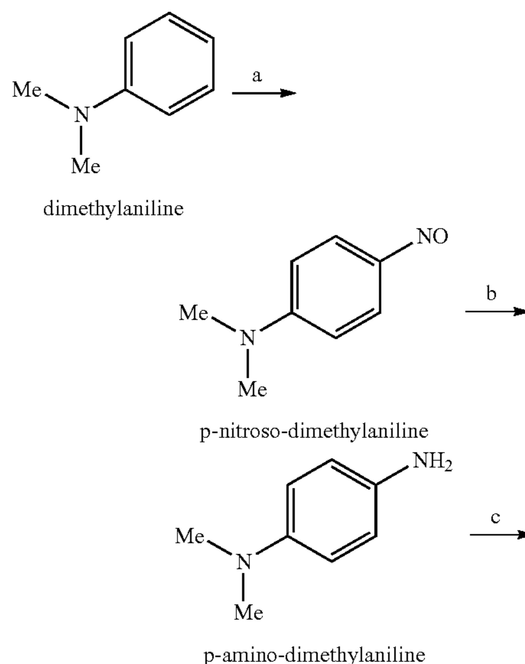
Scheme 1
