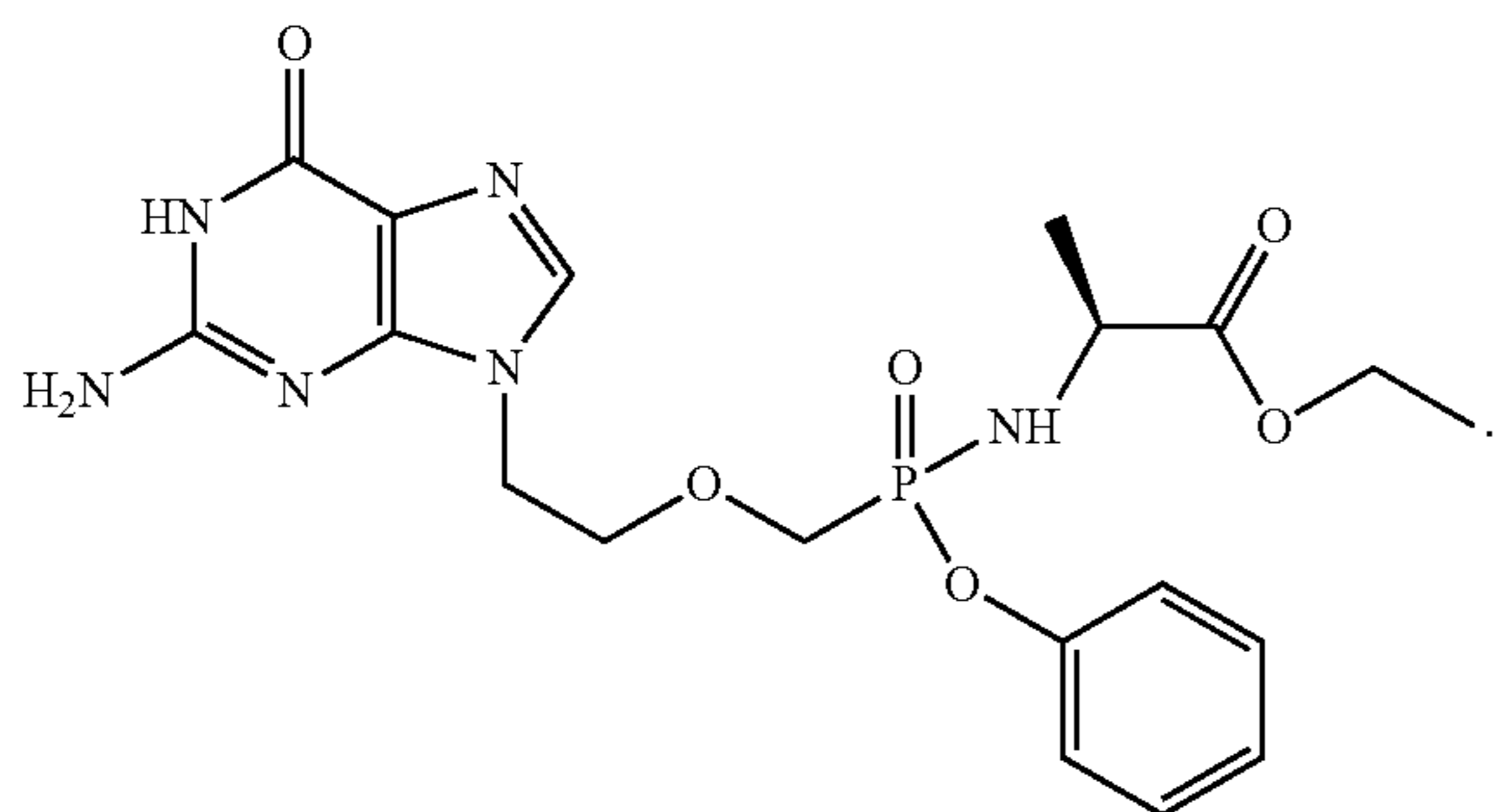
9-[2-(phenyloxy-(ethoxy-L-alaninyl))- phosphonomethoxy]ethyl]guanine
