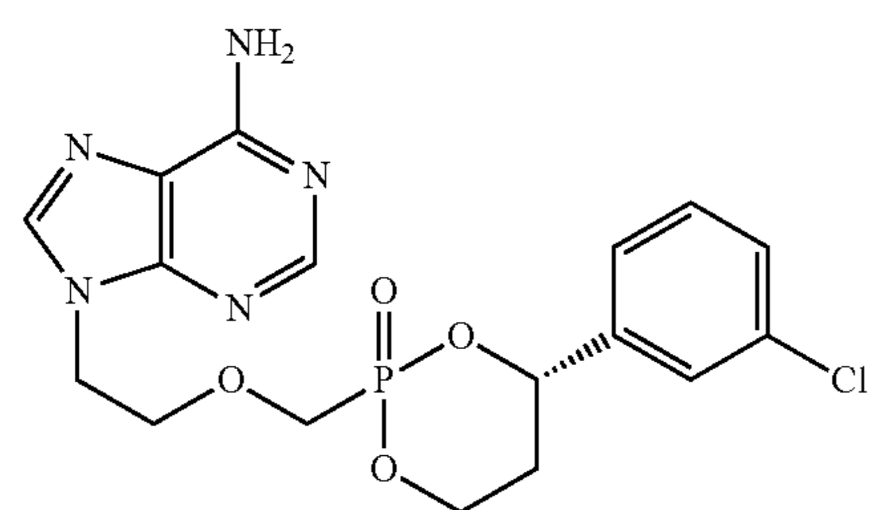
Pradefovir
