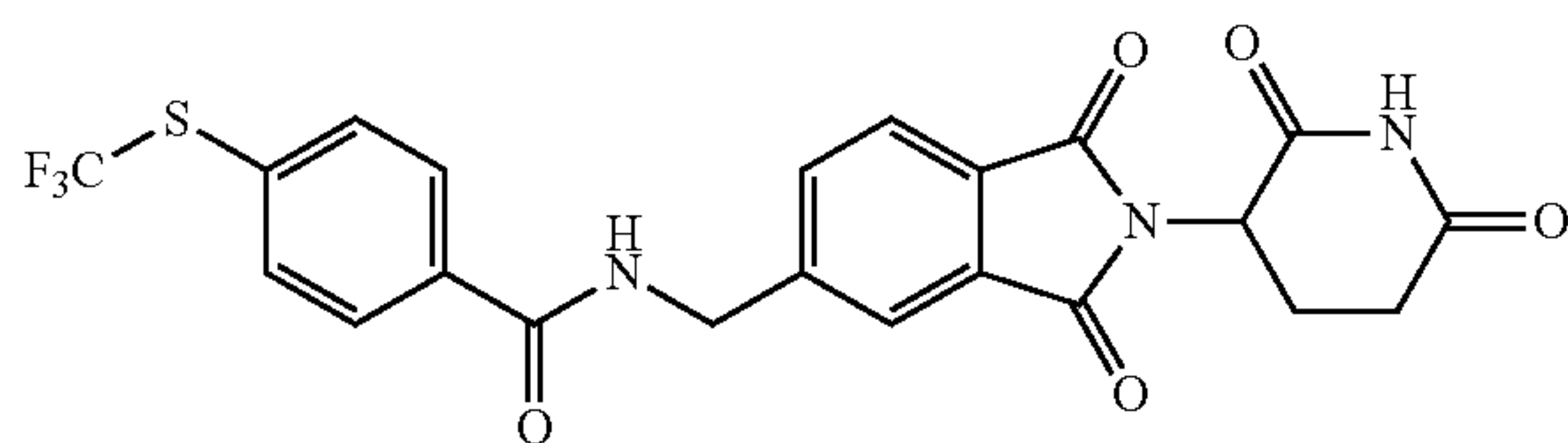
5.33 N-((2-(2,6-dioxopiperidin-3-yl)-1,3-dioxoisindolin-5-yl)methyl)-4-(trifluoromethylthio)benzamide
