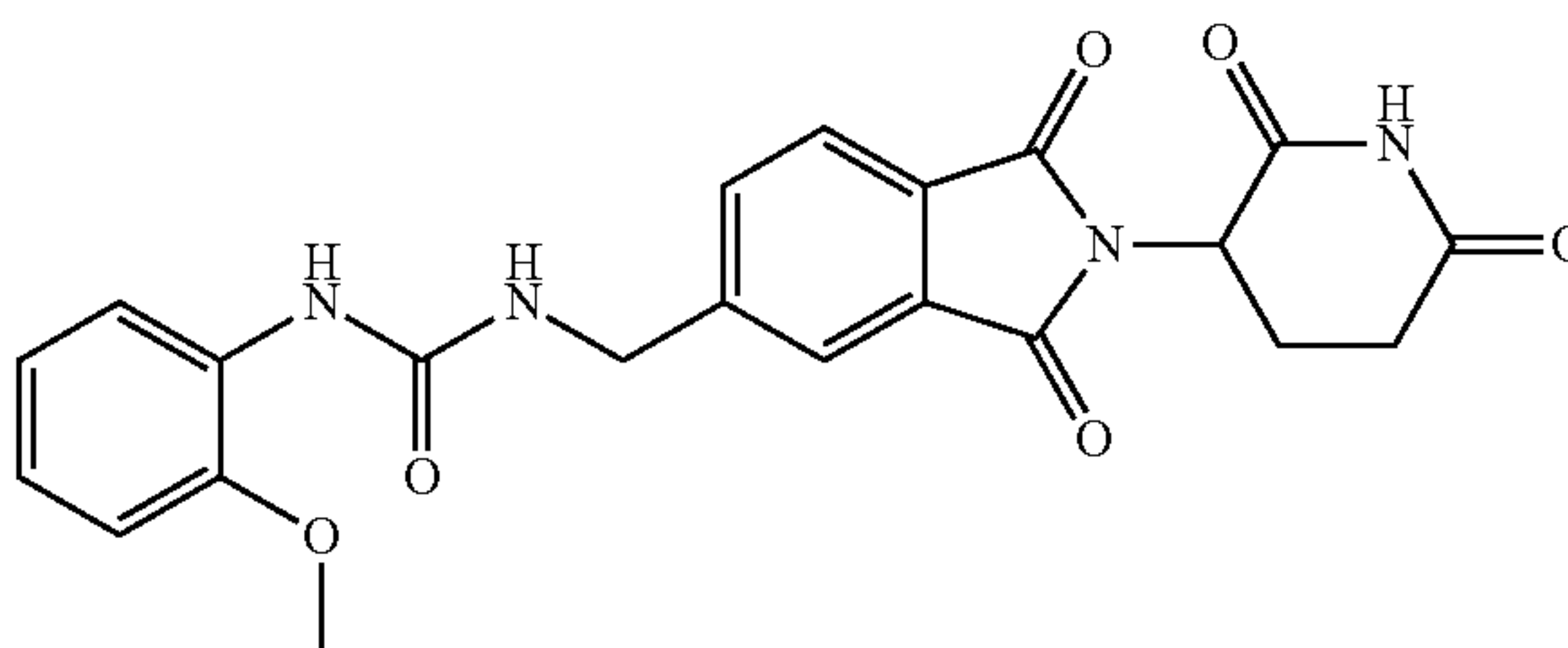
5.114 1-[2-(2,6-dioxo-piperidin-3-yl)-1,3-dioxo-2,3-dihydro-1H-isoindol-5-ylmethyl]-3-(2-methoxy-phenyl)-urea
