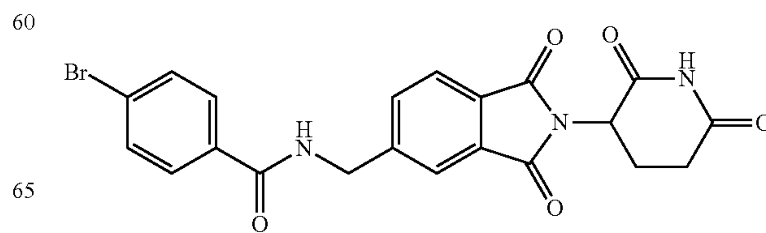
5.35 4-bromo-N-[2-(2,6-dioxo-piperidin-3-yl)-1,3-dioxo-2,3-dihydro-1H-isoindol-5-ylmethyl]-benzamide
