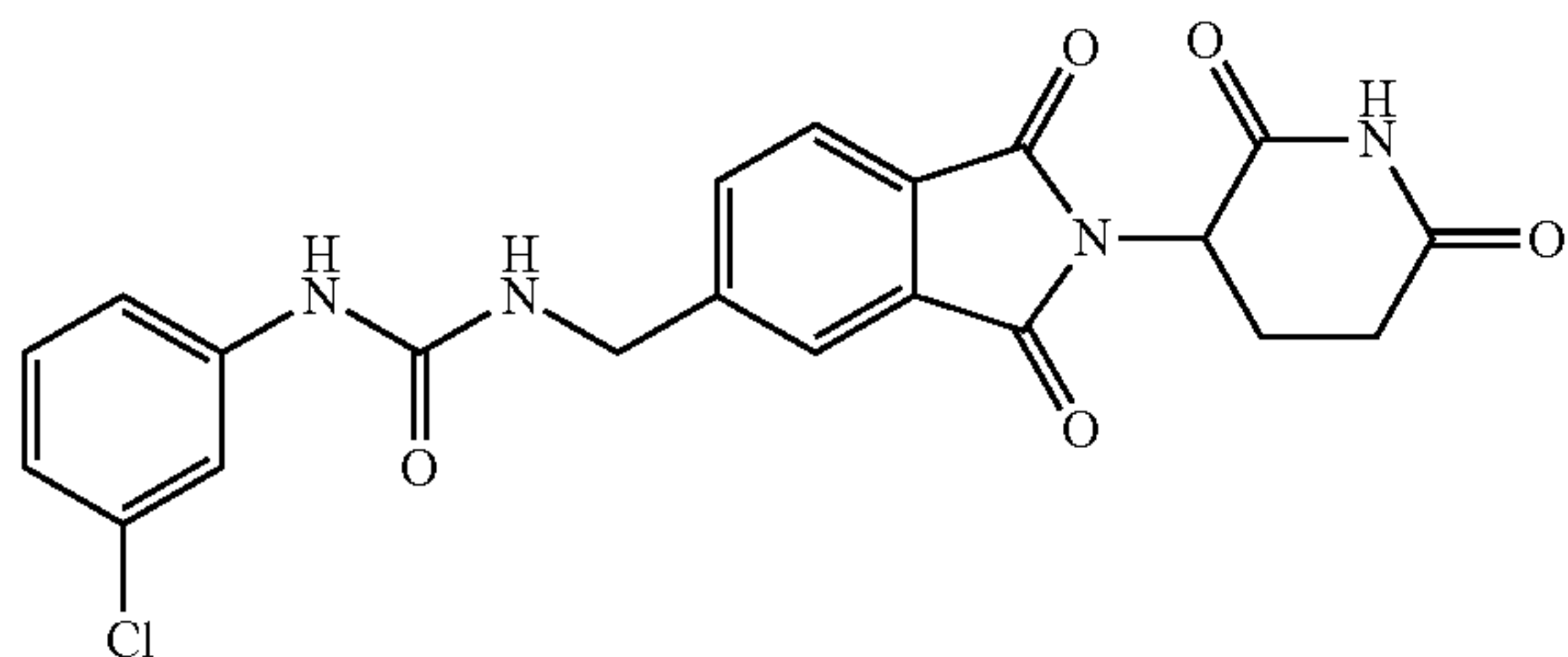
5.112 1-(3-chloro-phenyl)-3-[2-(2,6-dioxo-piperidin-3-yl)-1,3-dioxo-2,3-dihydro-1H-isoindol-5-ylmethyl]-urea
