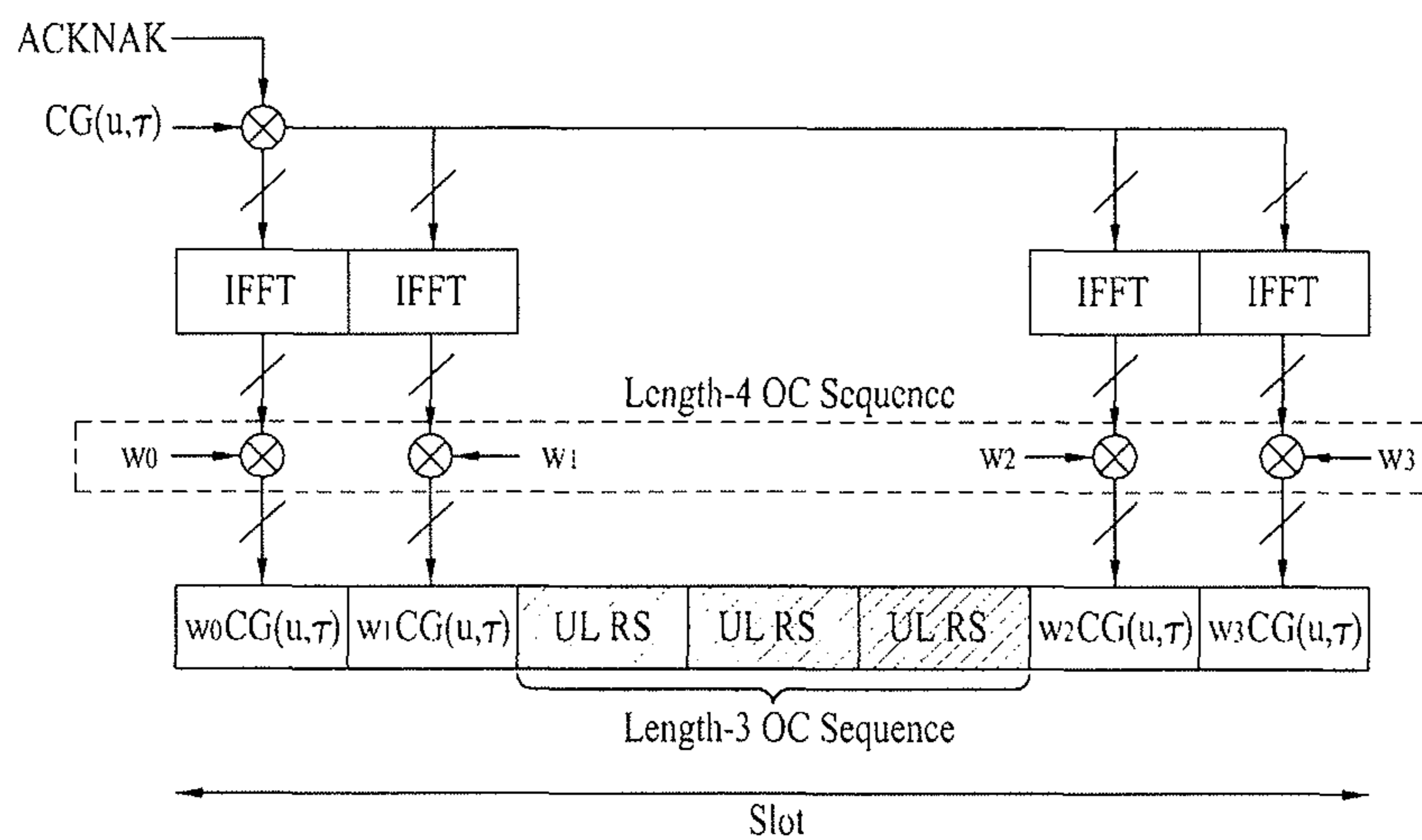
PUCCH format 1a and 1b structure (Case of normal CP)
