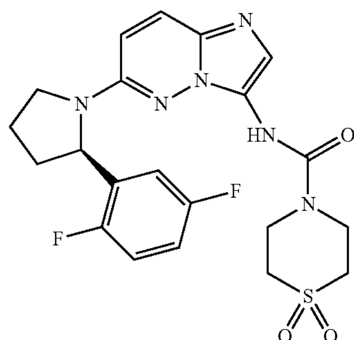
(R)-1-(6-(2-(2,5-difluorophenyl)pyrrolidin-1-yl)imidazo[1,2-b]pyridazin-3-yl)carbamoylpiperidin-4-sulfone
