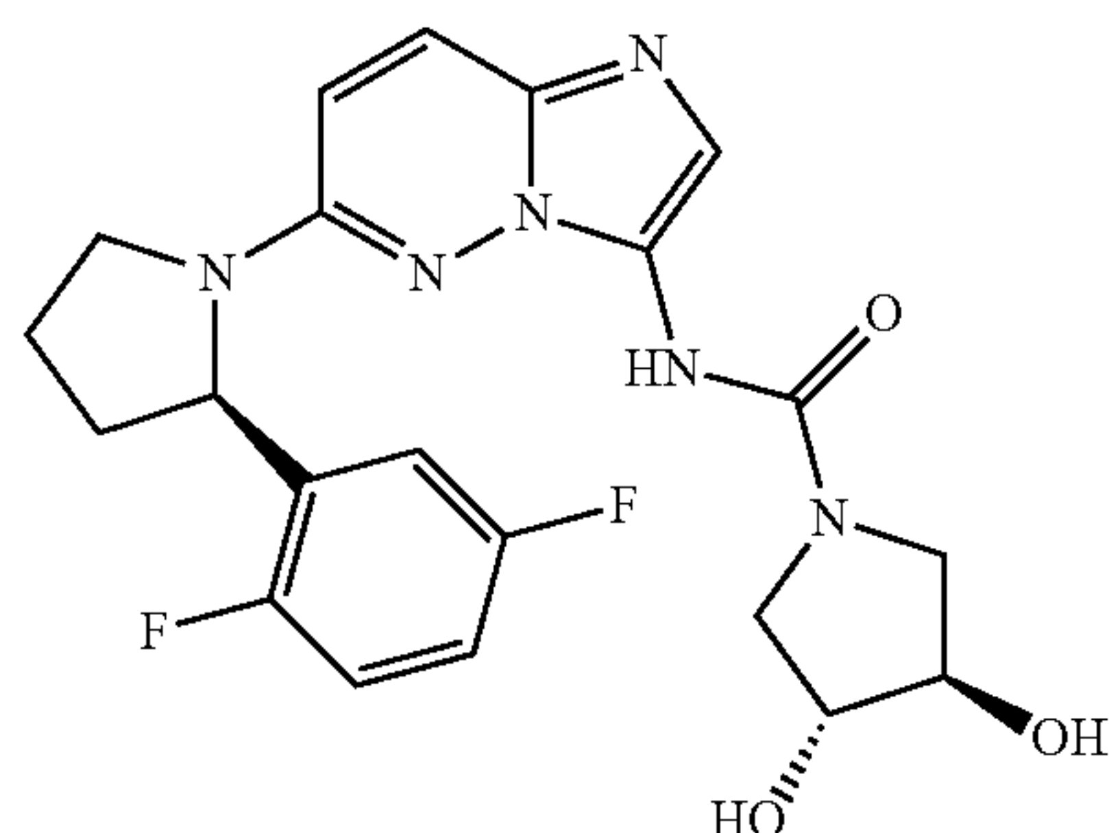
(3R,4R)—N-(6-((R)-2-(2,5-difluorophenyl)pyrrolidin-1-yl)imidazo[1,2-b]pyridazin-3-yl)-3,4-dihydroxypyrrolidine-1-carboxamide
