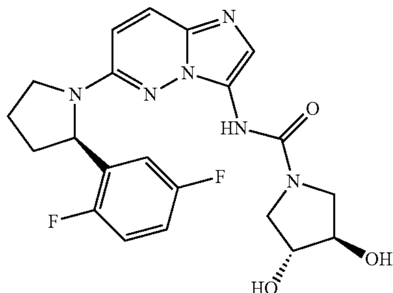
(3R,4R)—N-(6-((R)-2-(2,5-difluorophenyl)pyrrolidin-1-yl)imidazo[1,2-b]pyridazin-3-yl)-3,4-dihydroxypyrrolidine-1-carboxamide
