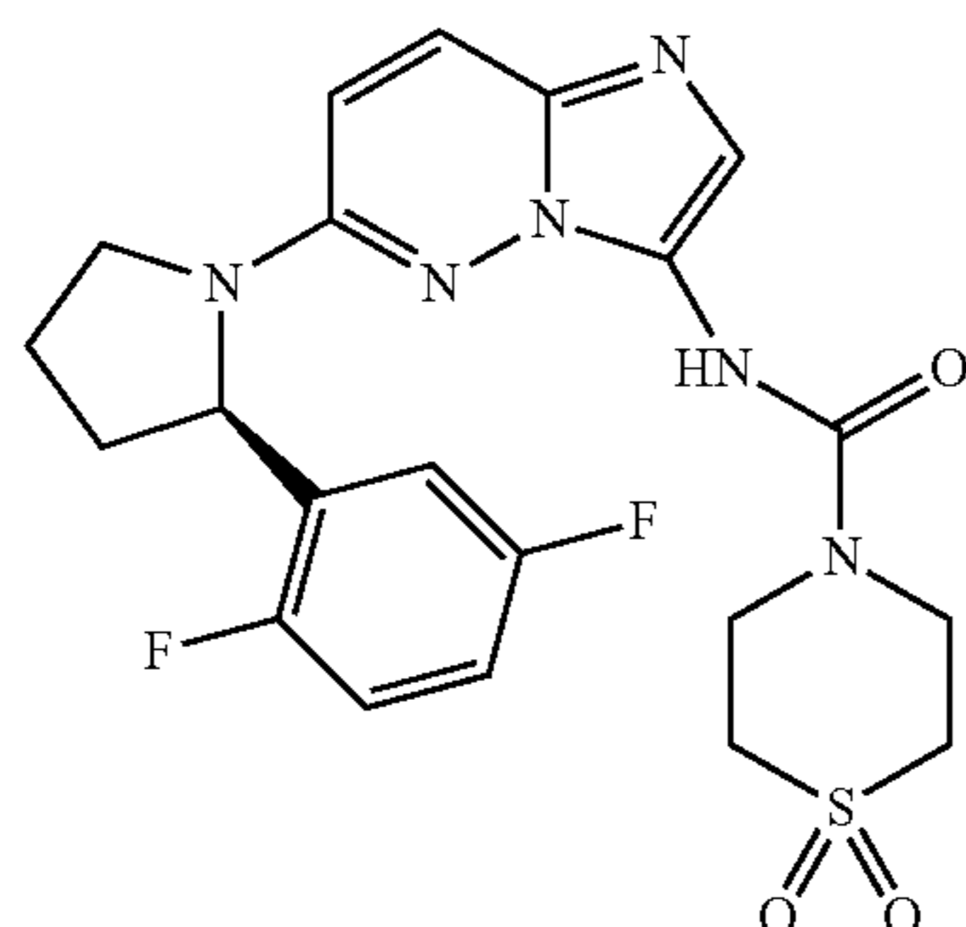
(R)-1-(6-(2-(2,5-difluorophenyl)pyrrolidin-1-yl)imidazo[1,2-b]pyridazin-3-yl)carbonylpiperidin-4-sulfone
