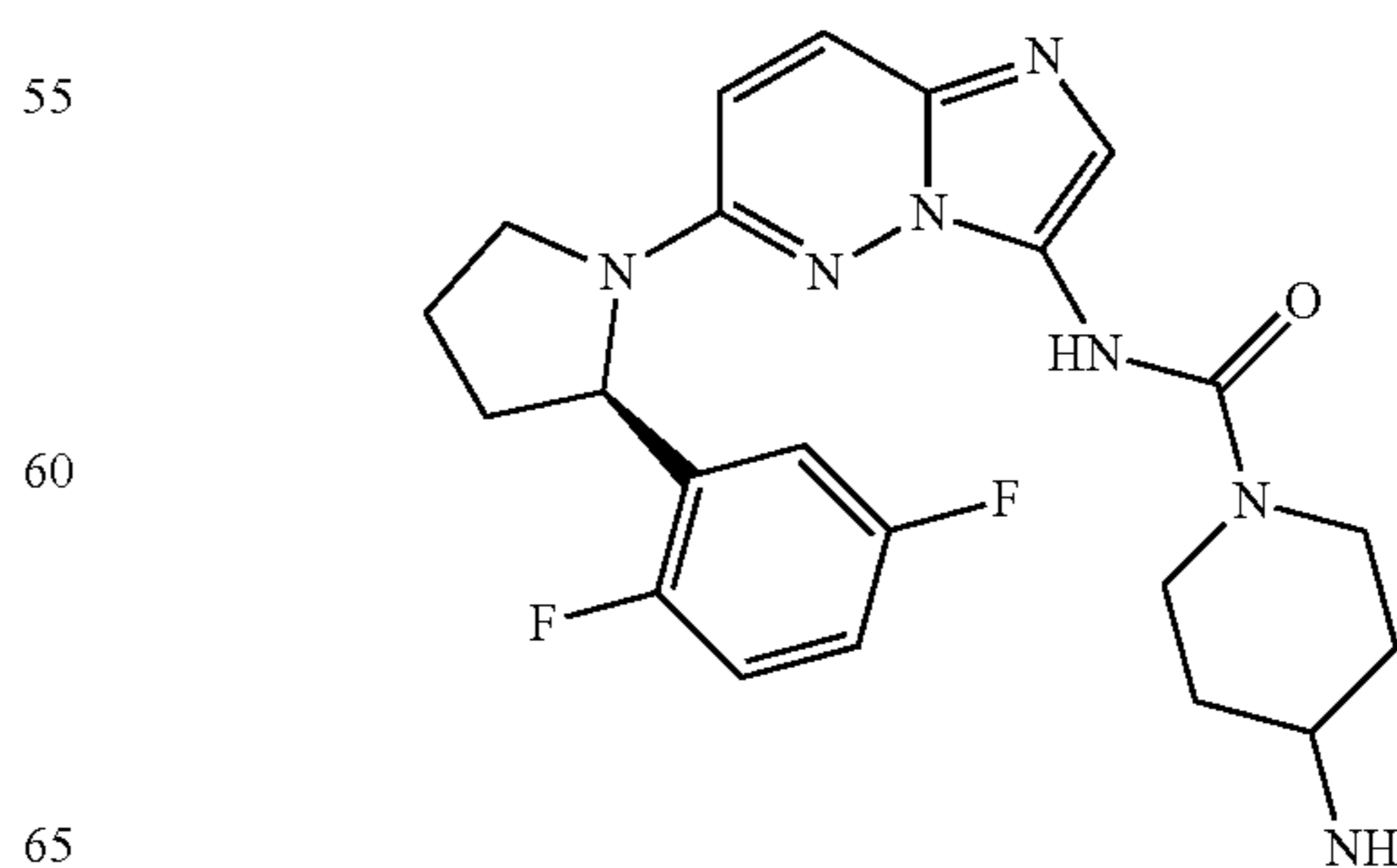
(R)-tert-butyl 4-(6-(2-(2,5-difluorophenyl)pyrrolidin-1-yl)imidazo[1,2-b]pyridazin-3-yl)carbamoyl piperazine-1-carboxylate
