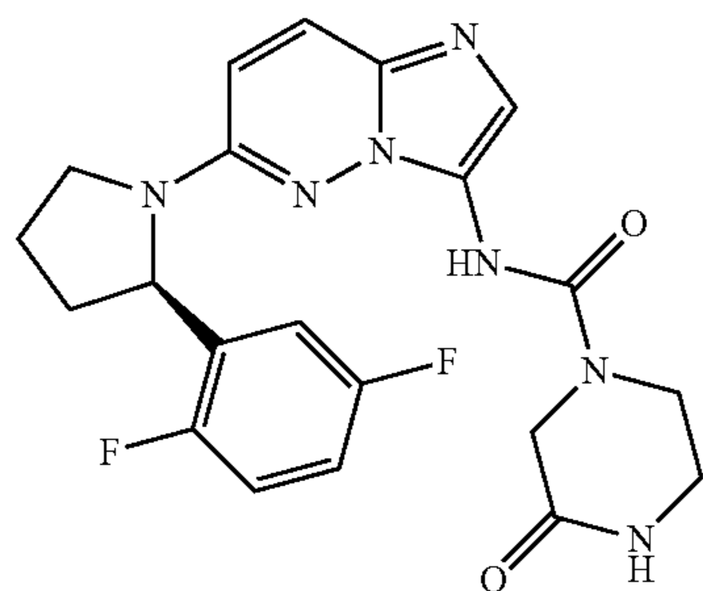
(R)—N-(6-(2-(2,5-difluorophenyl)pyrrolidin-1-yl)imidazo[1,2-b]pyridazin-3-yl)-3-oxopiperazine-1-carboxamide
