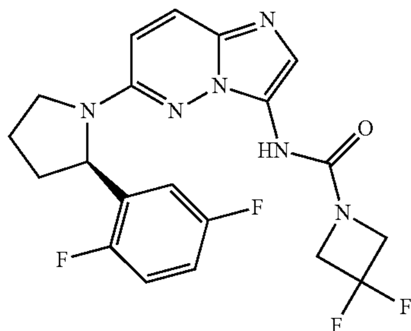
(R)-N-(6-(2-(2,5-difluorophenyl)pyrrolidin-1-yl)imidazo[1,2-b]pyridazin-3-yl)-3,3-difluoroazetidine-1-carboxamide
