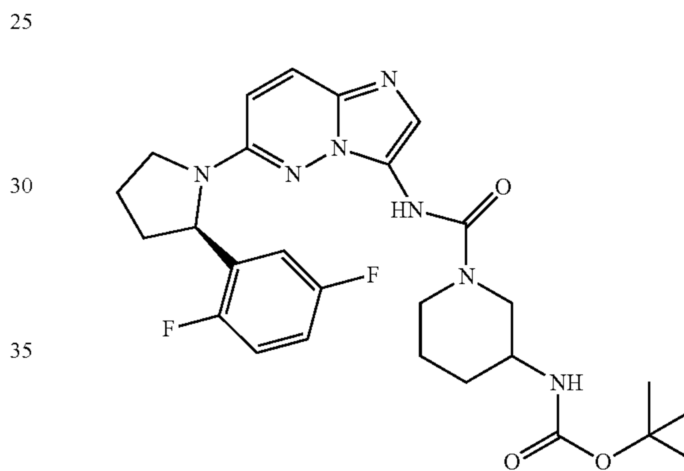
tert-Butyl 1-(6-((R)-2-(2,5-difluorophenyl)pyrrolidin-1-yl)imidazo[1,2-b]pyridazin-3-yl)carbamoyl piperidin-3-ylcarbamate
