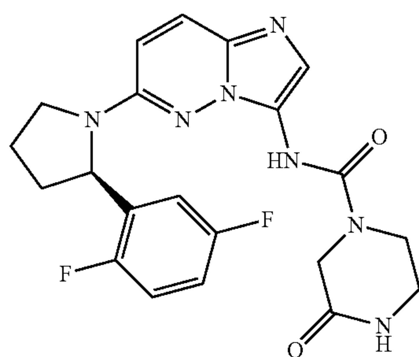
(R)—N-(6-(2-(2,5-difluorophenyl)pyrrolidin-1-yl)imidazo[1,2-b]pyridazin-3-yl)-3-oxopiperazine-1-carboxamide
