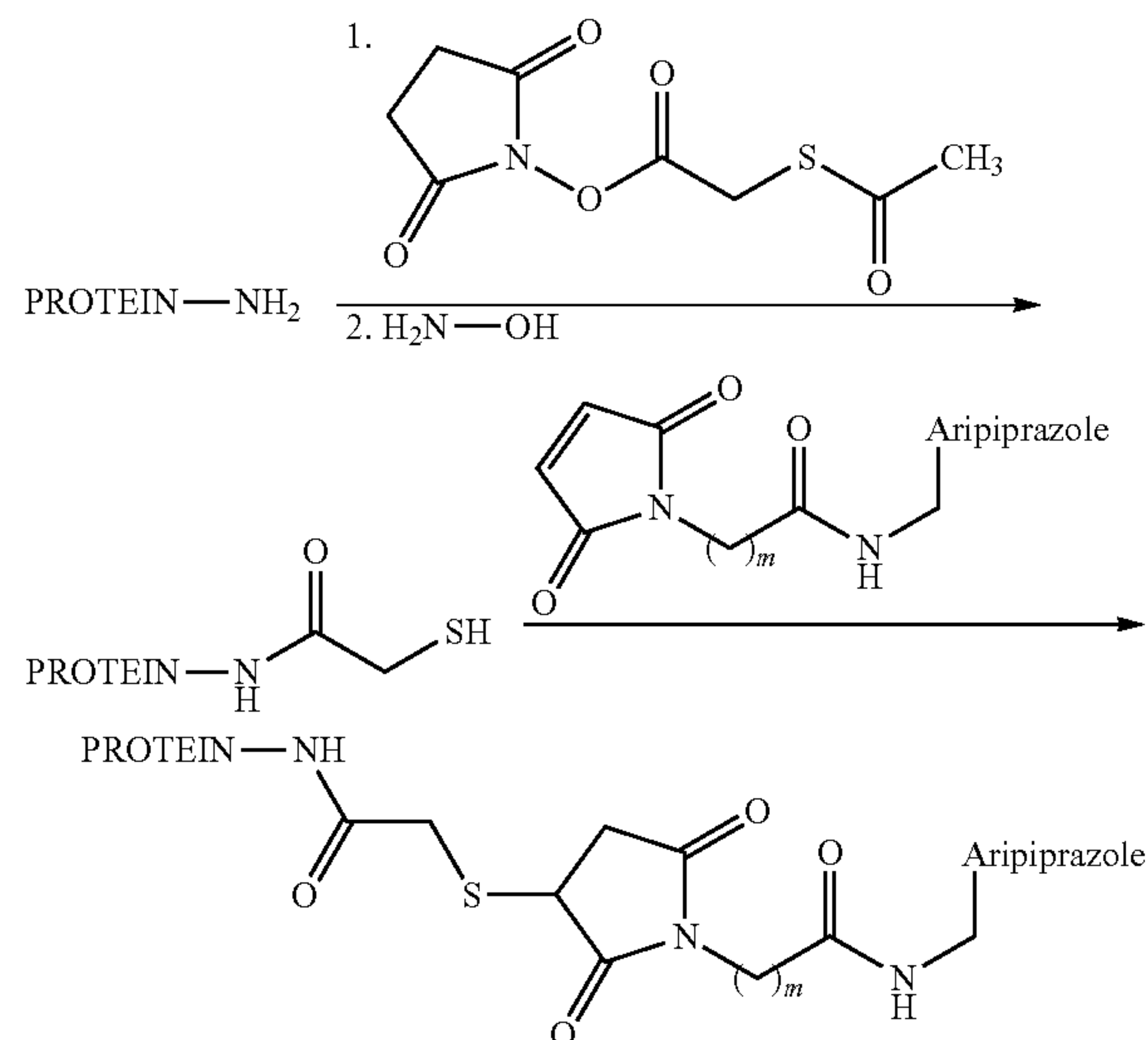
Scheme 8
