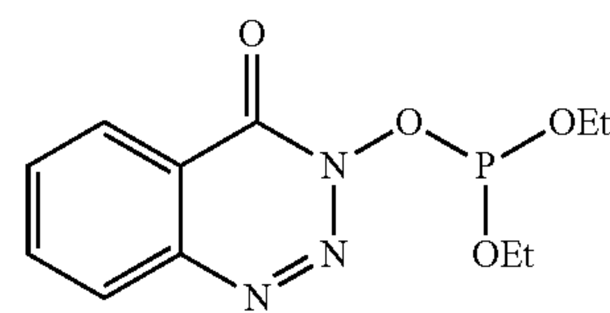
DEPT
