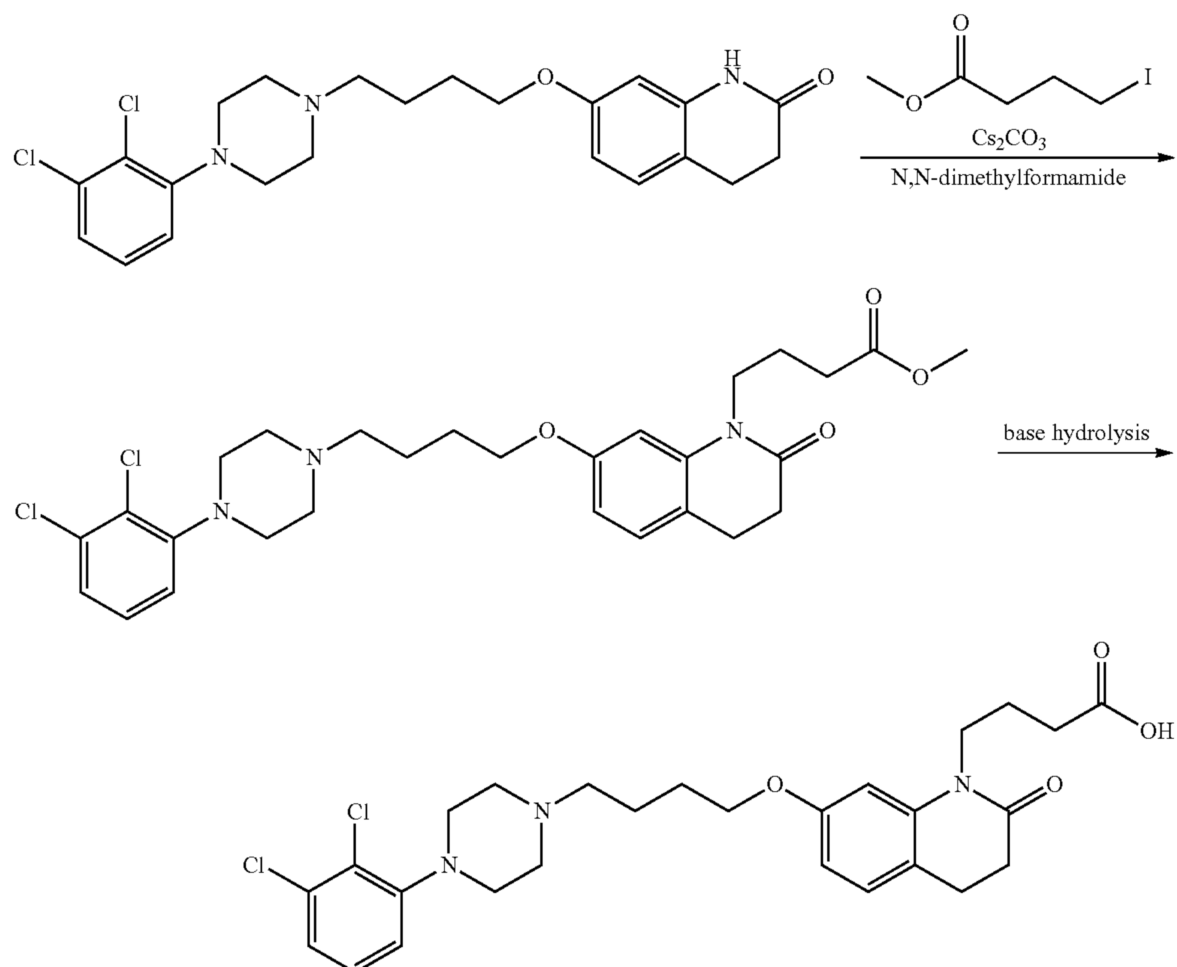
Scheme 7
