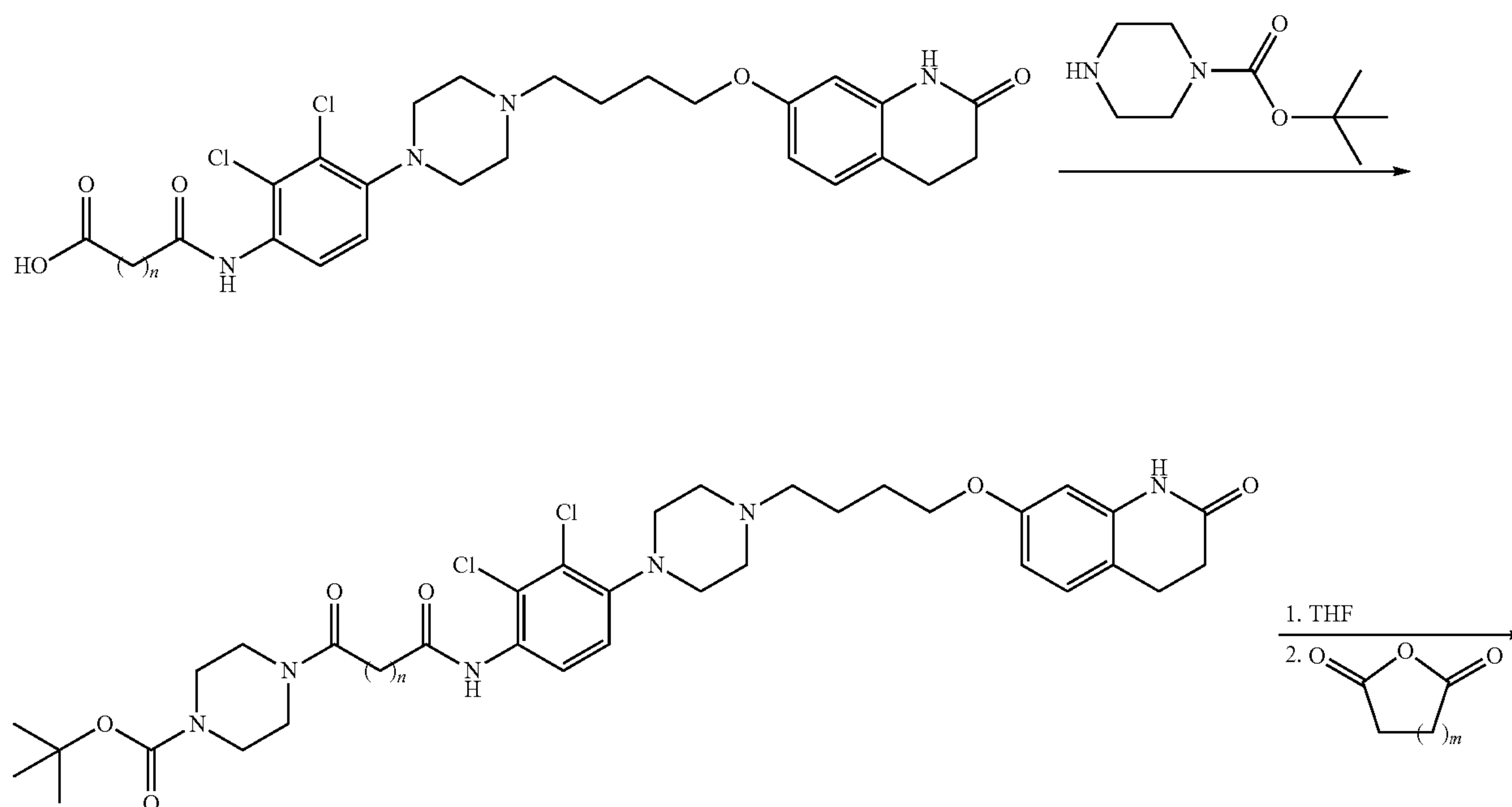
Scheme 5
