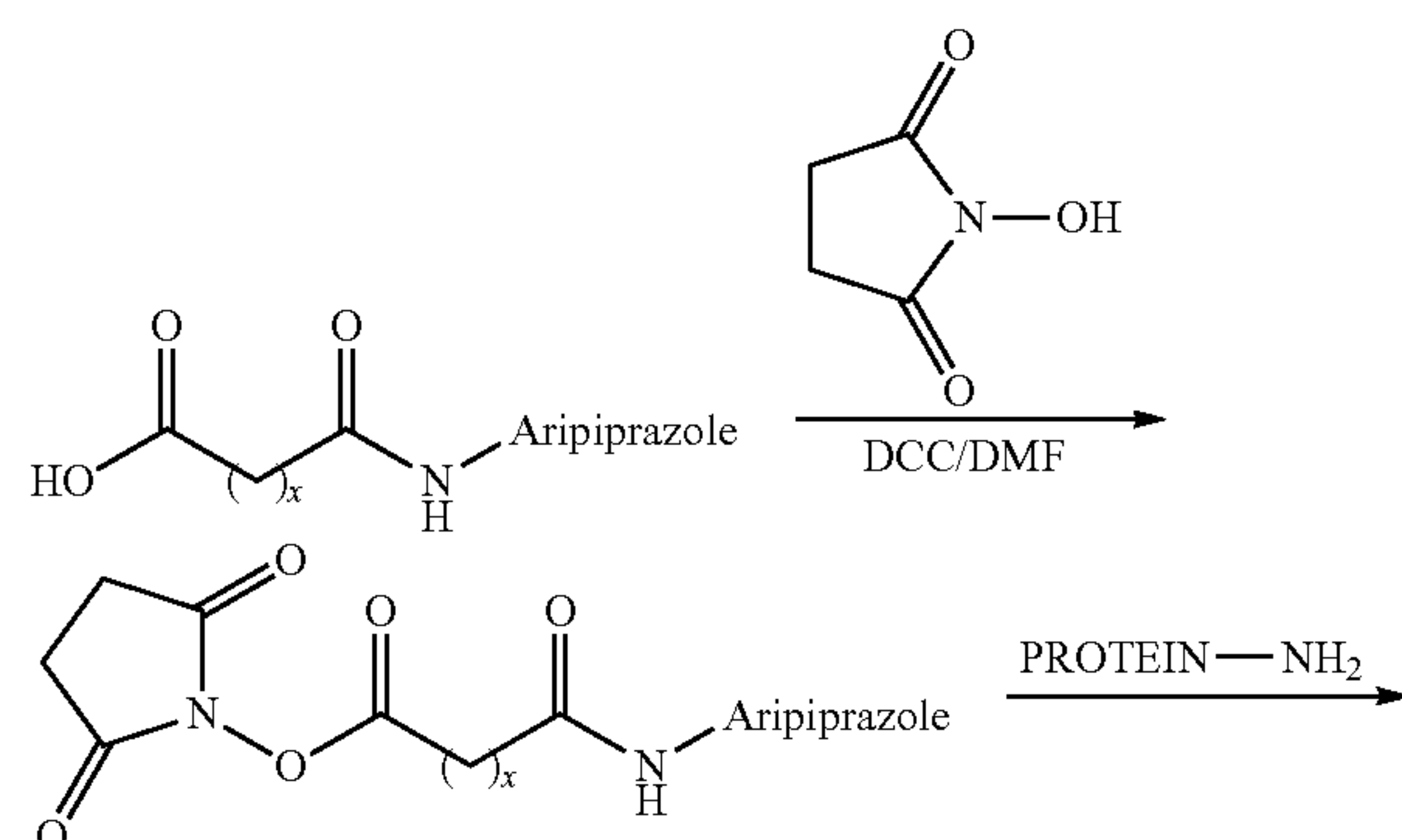
Scheme 9:
