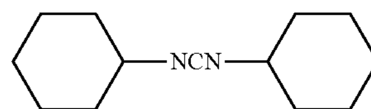
Dicyclohexylcarbodiimide (DCC)
