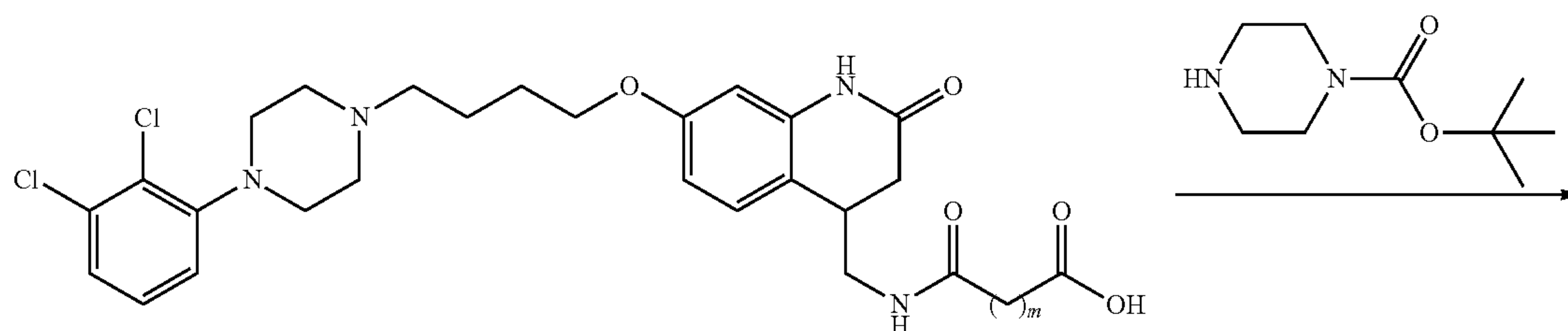
Scheme 4
