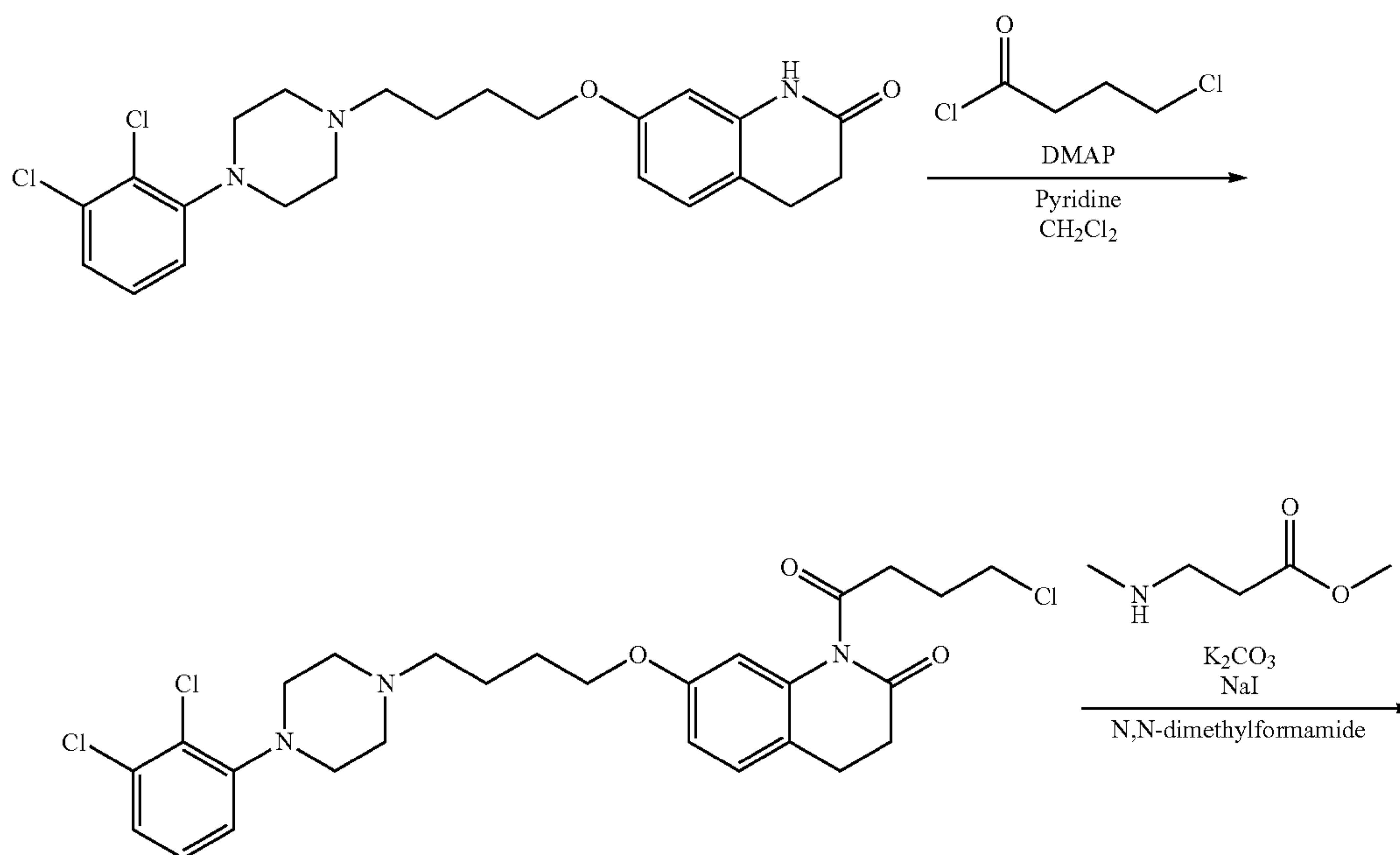
Scheme 6:
