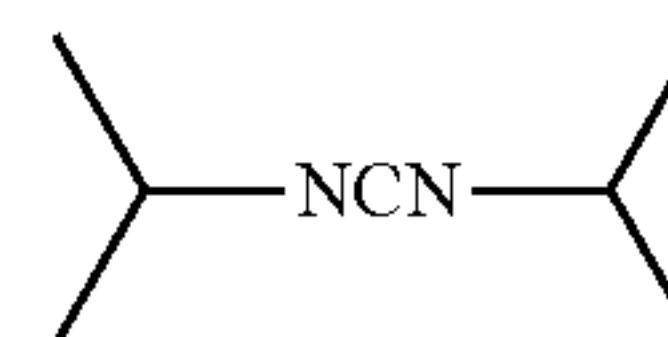
diisopropylcarbodiimide (DIC)
