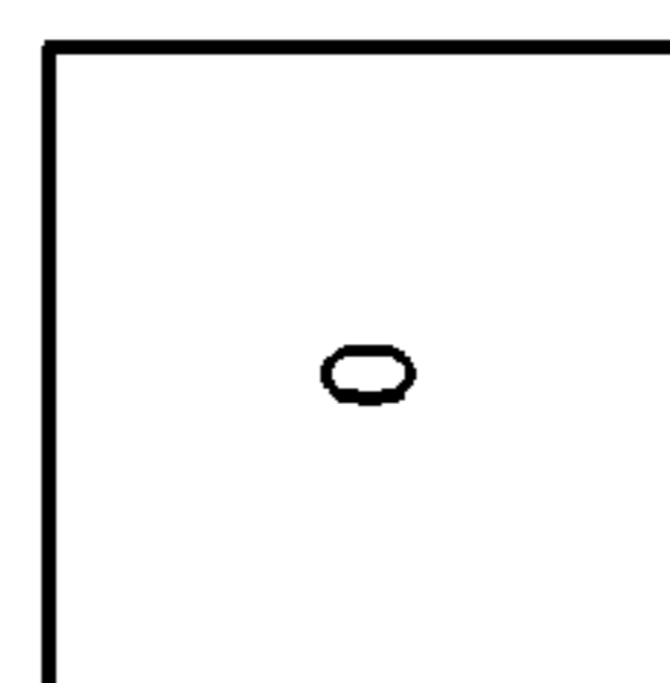
SUB-MACROBLOCK PARTITION
