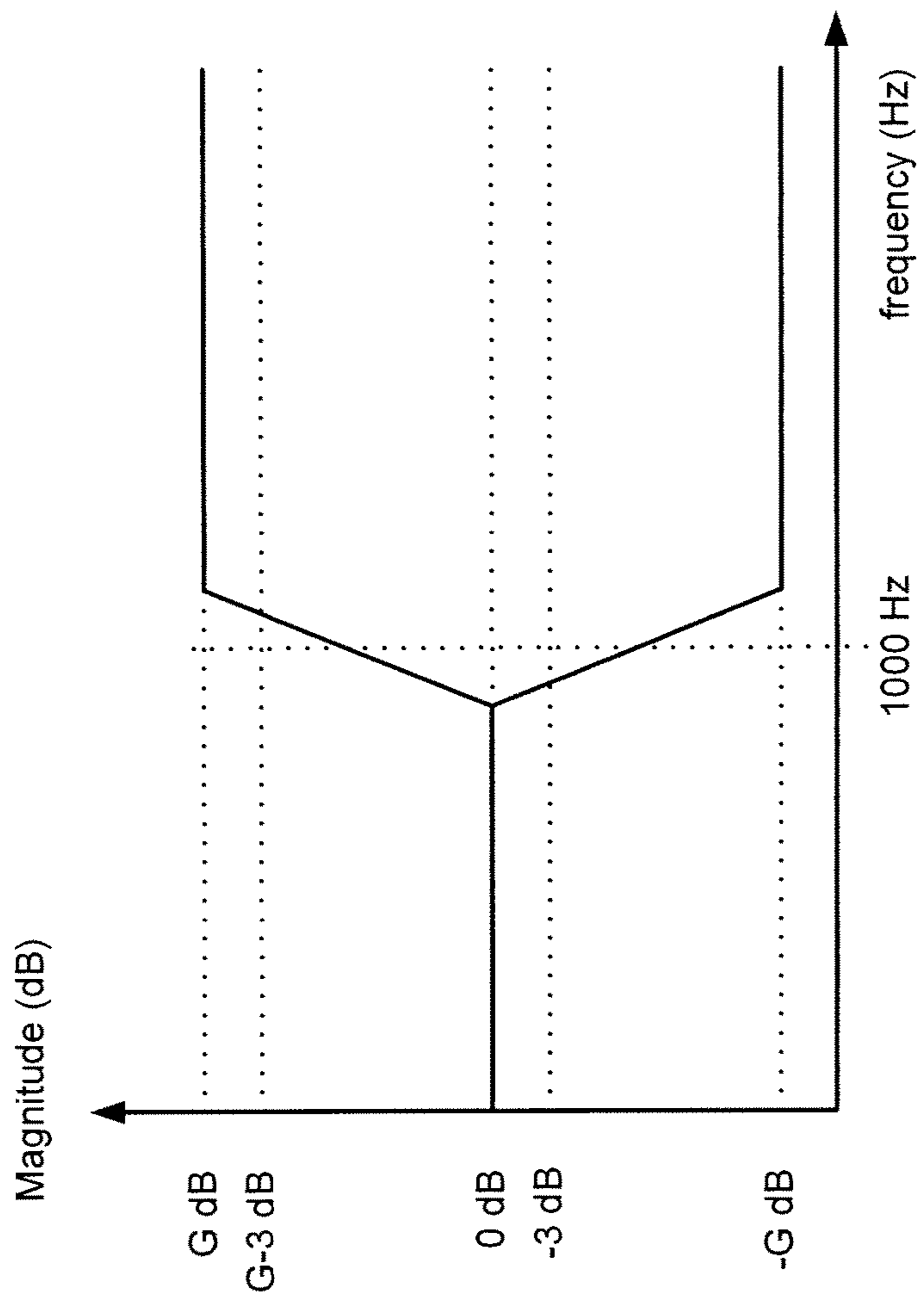
High shelving filters with cutoff frequency at 1000 Hz and gains \div GdB
