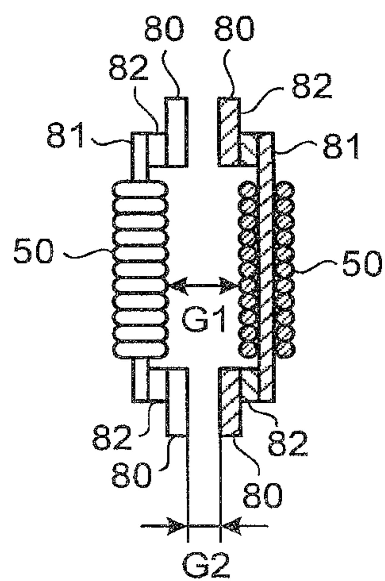
FIG.7C
