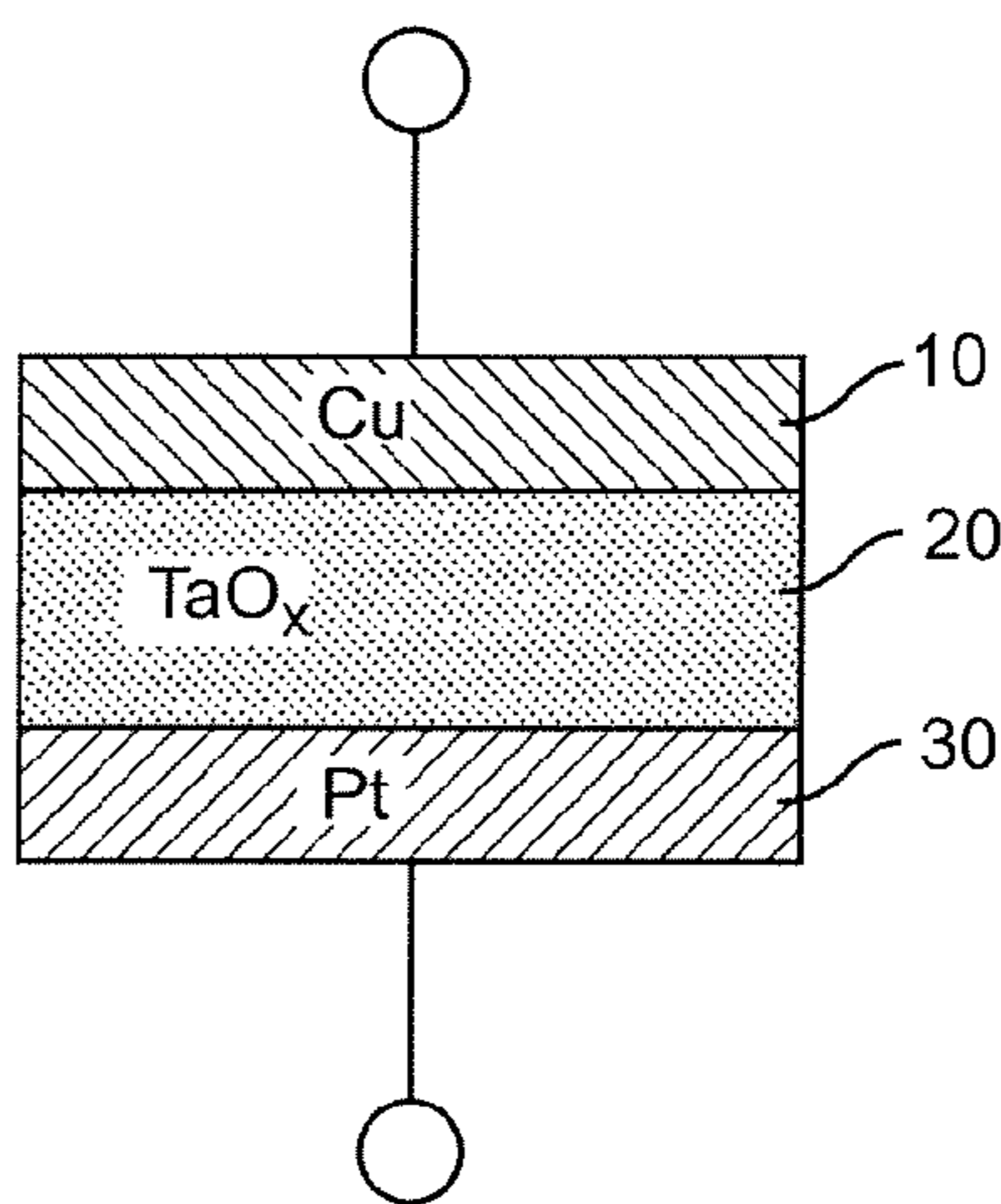
Figure 1 RELATED ART
