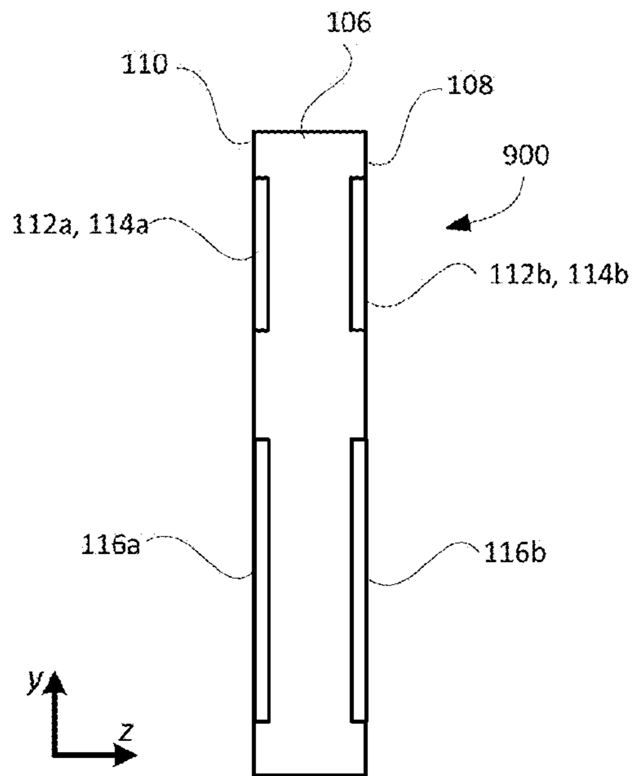
FIG. 9B (side view)
