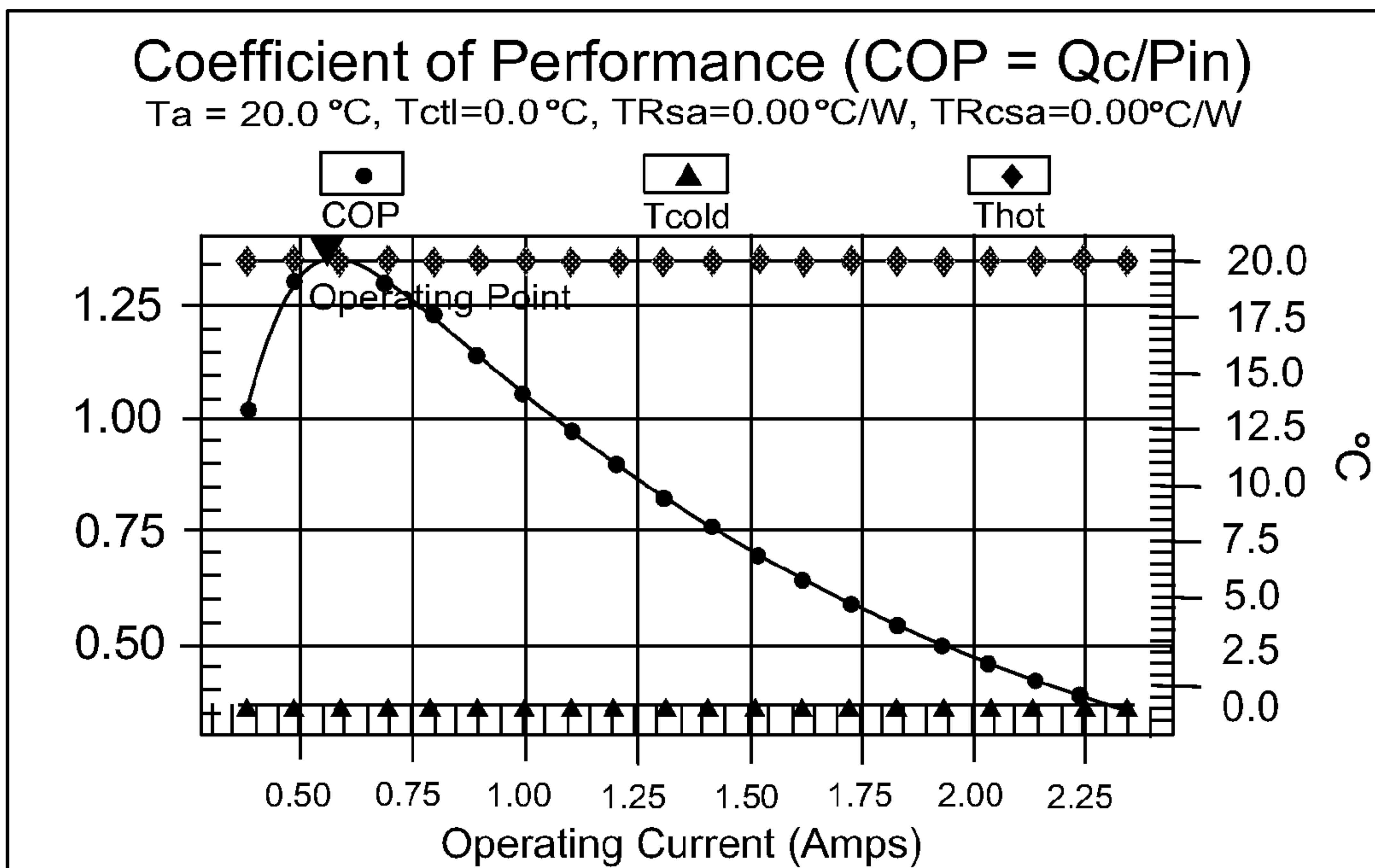
Optimum TE operating point at DT 20
