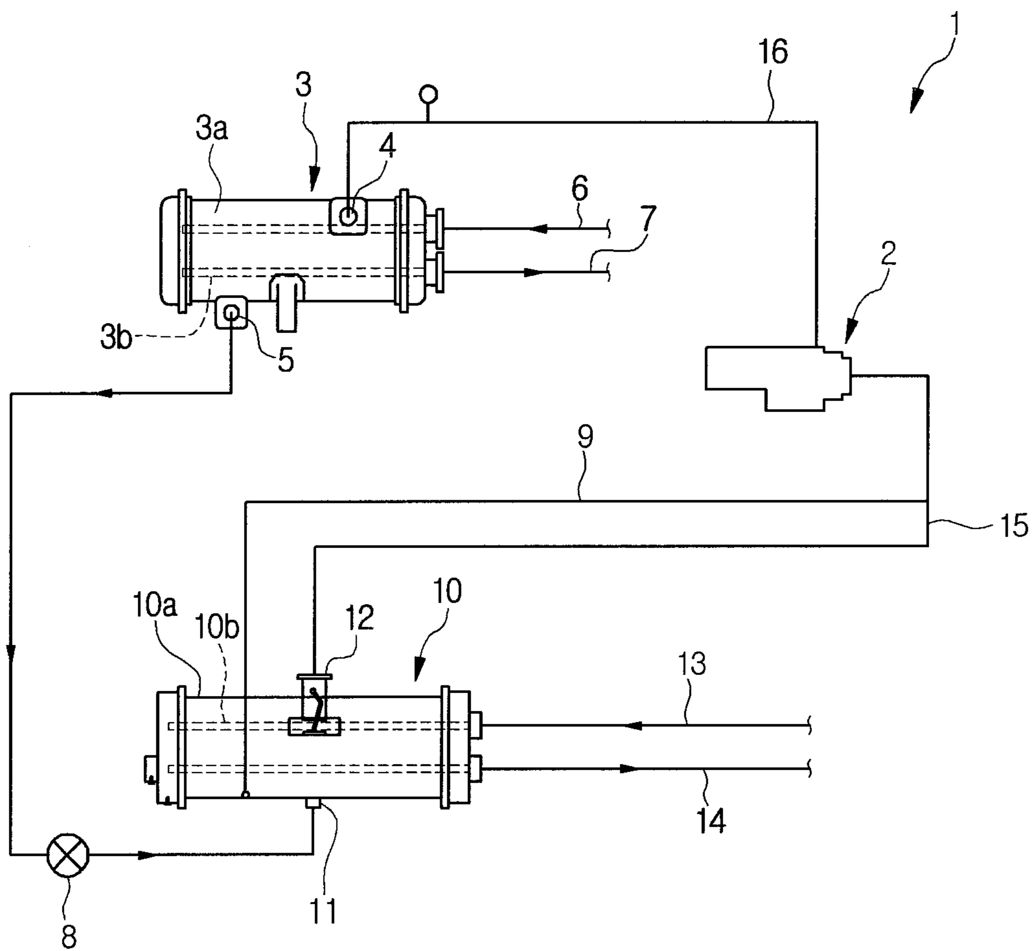
FIG. 1 -RELATED ART-
