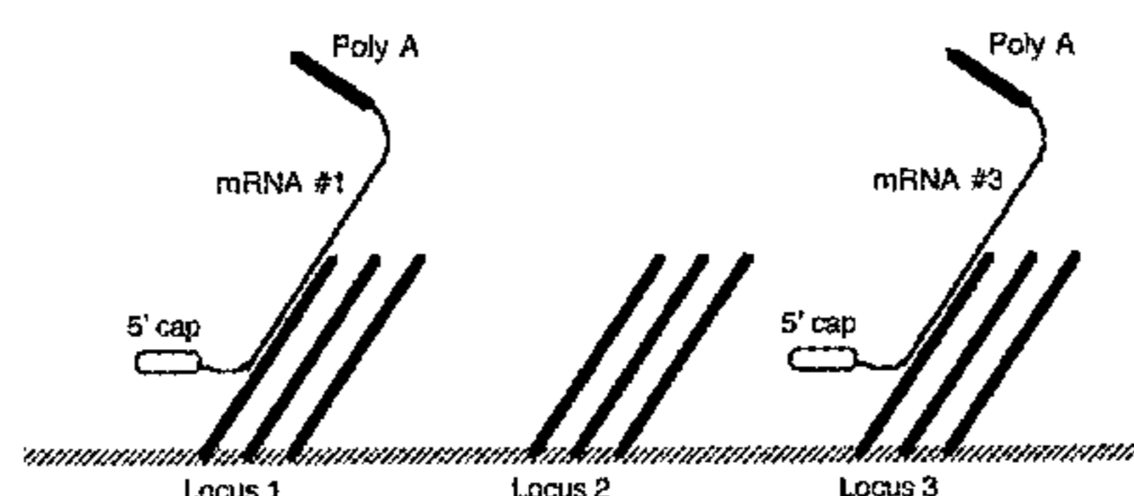
Library of mRNA analytes bound to an array
