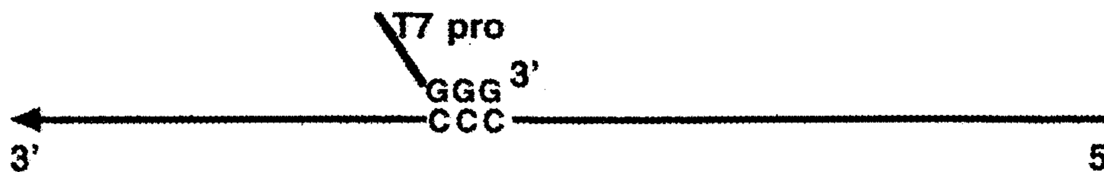
(E) Binding of Primer with T7 promoter to internal sequenced of cNDNA
