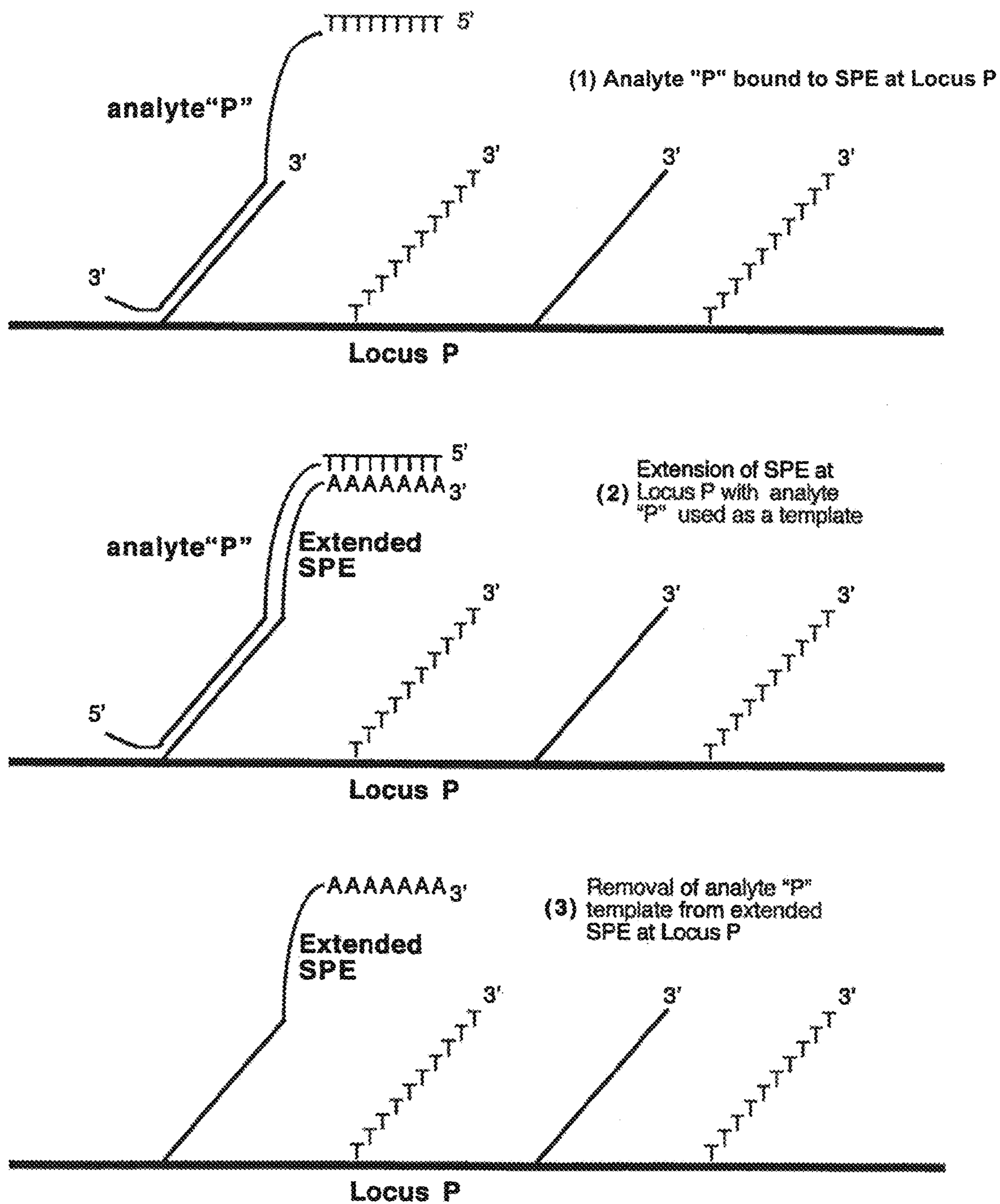
Figure 17 Extension of an SPE
