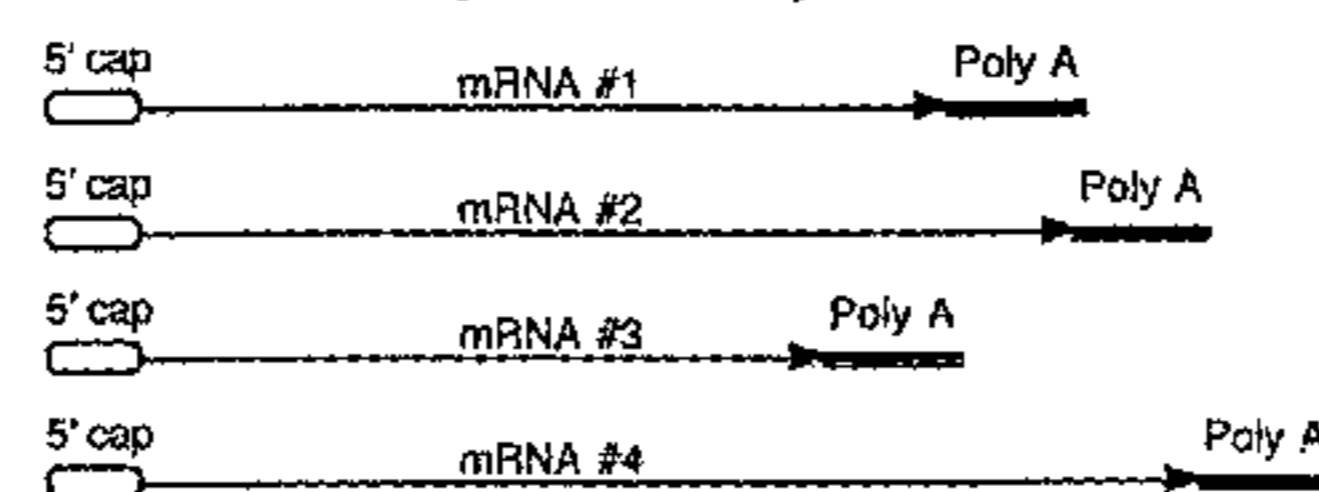
Library of mRNA analytes
