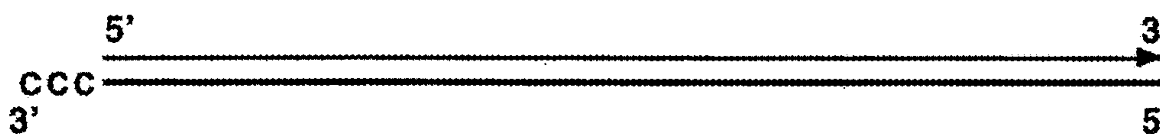
(C) Template Independent addition of dCTP
