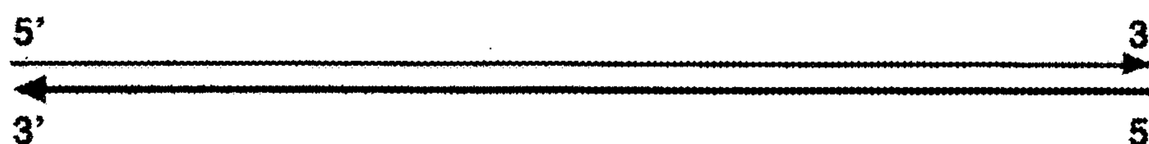
(B) Extension of Primer using analyte as template
