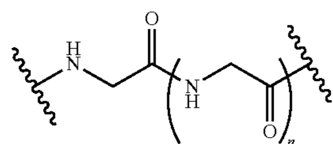
poly(glycine)
