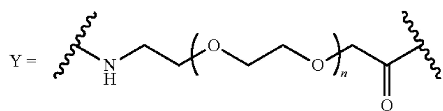
PEG
