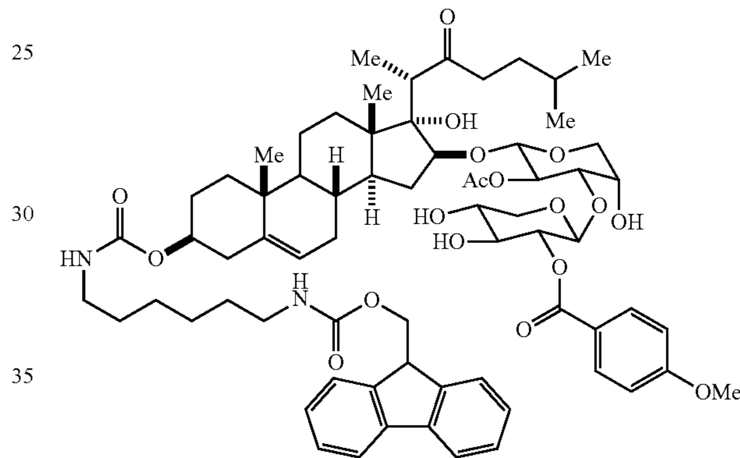
Chemical Formula: C 69 H 92 N 2 O 18 Exact Mass: 1236.63451
