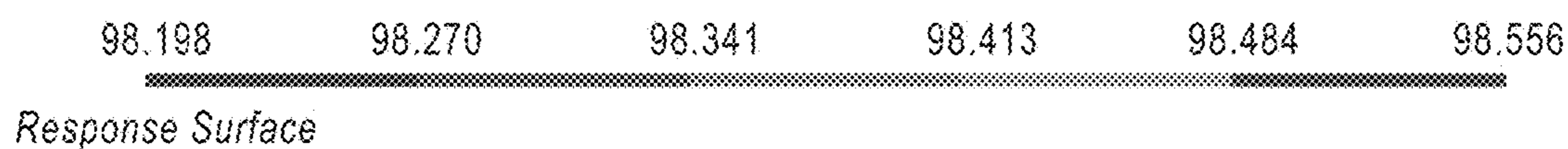
Effect of pH/His (PLS Model 1)
