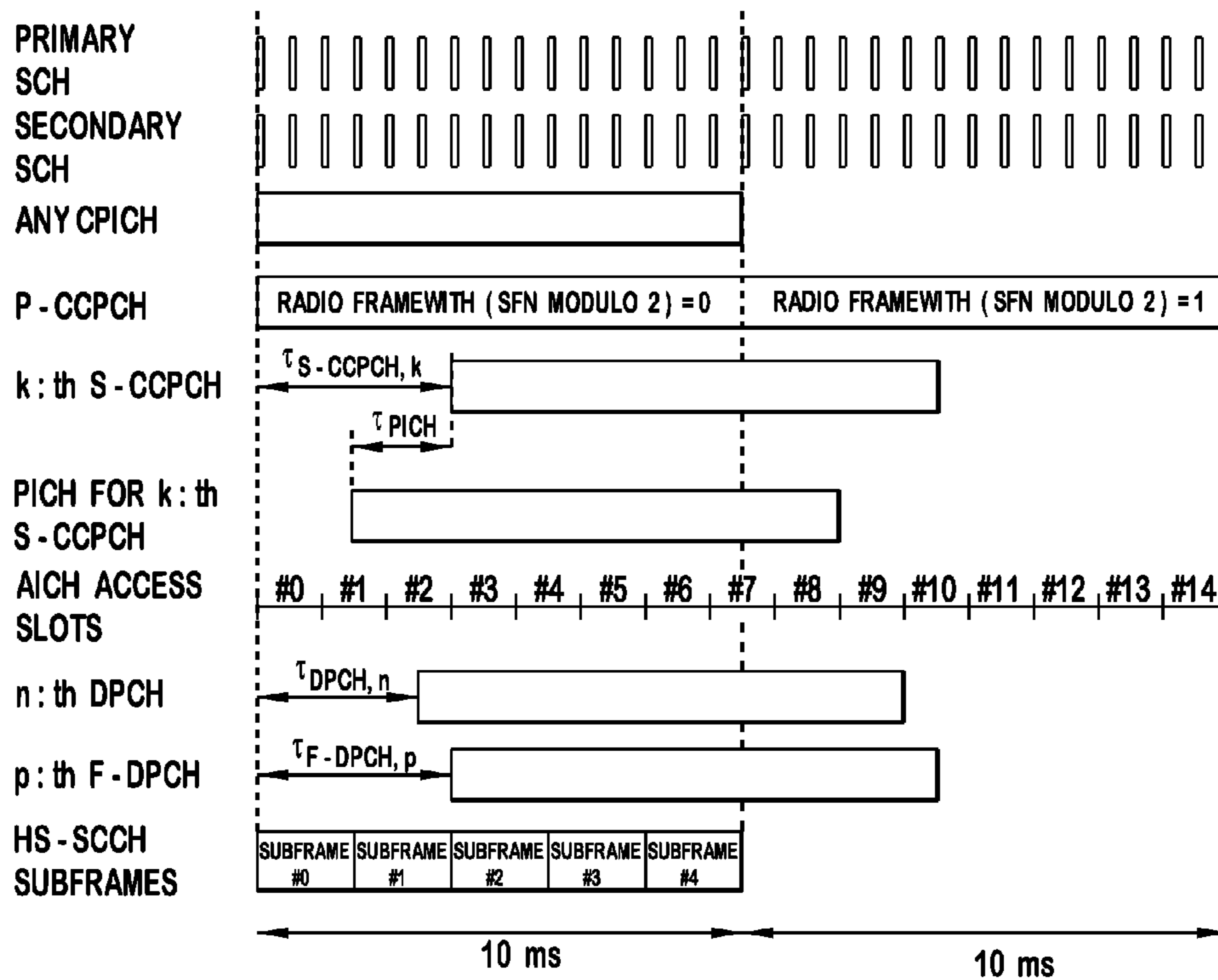
FIG. 3 (PRIOR ART)
