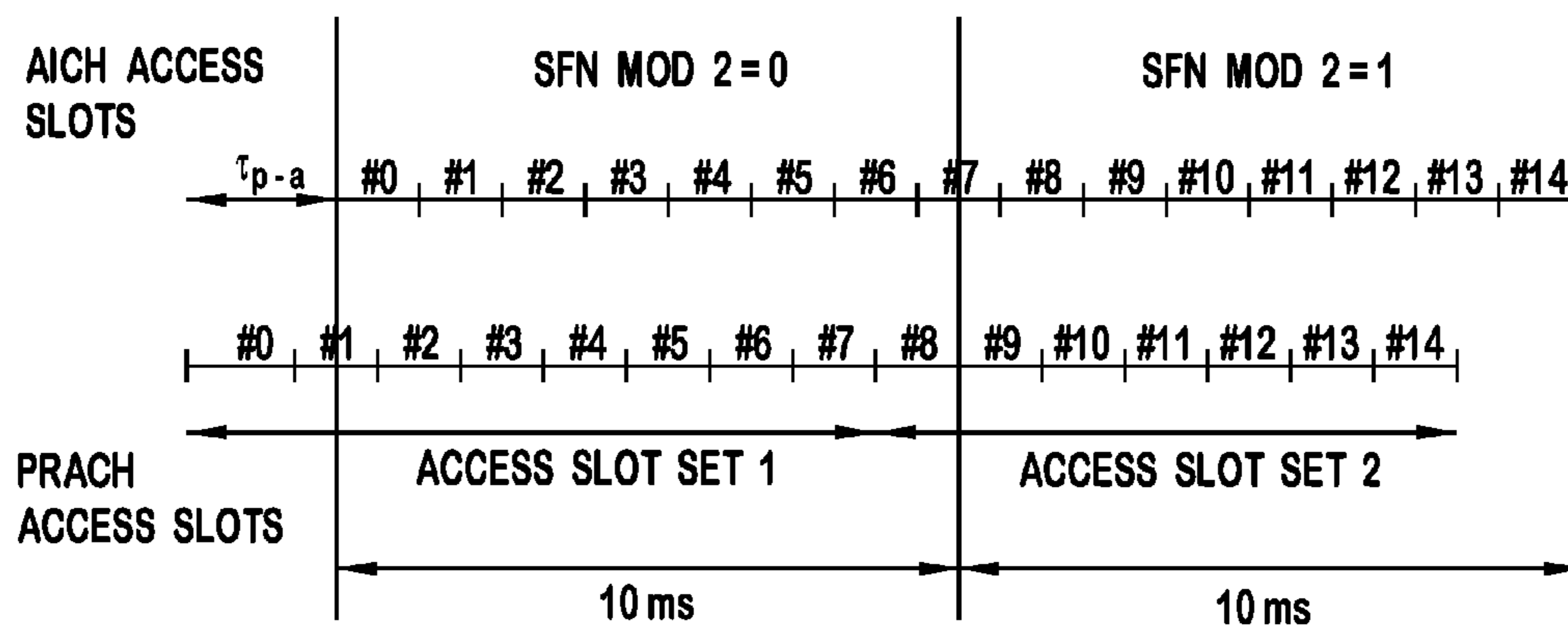
FIG. 2 (PRIOR ART)
