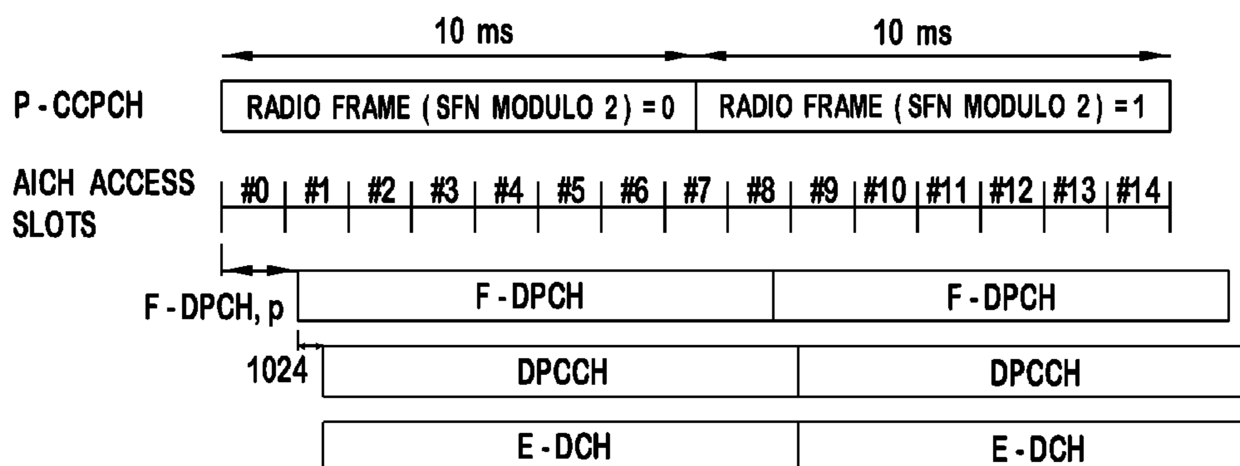
FIG. 4 (PRIOR ART)
