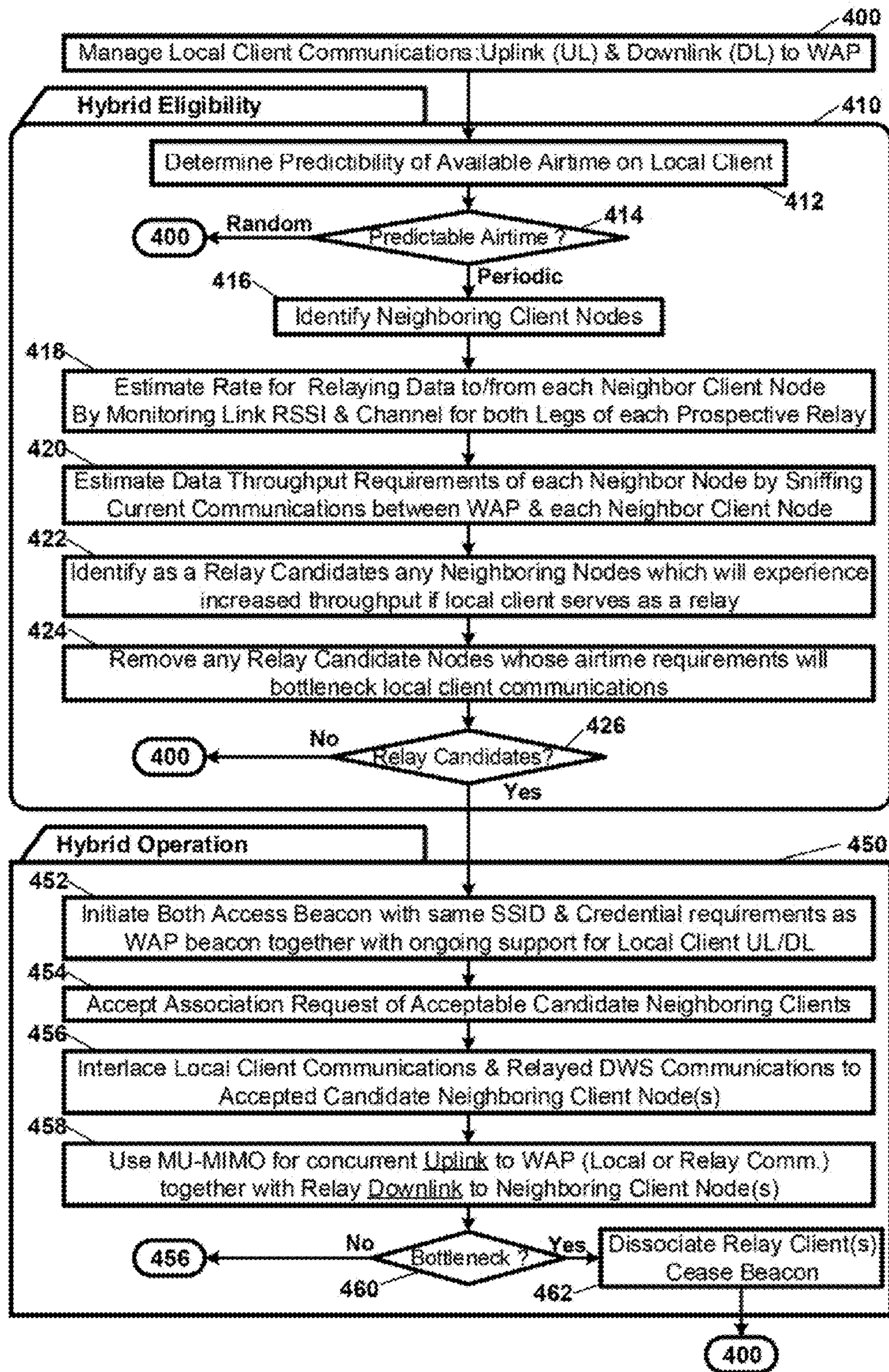
FIG. 4 Hybrid Client in WiFi Home Network
