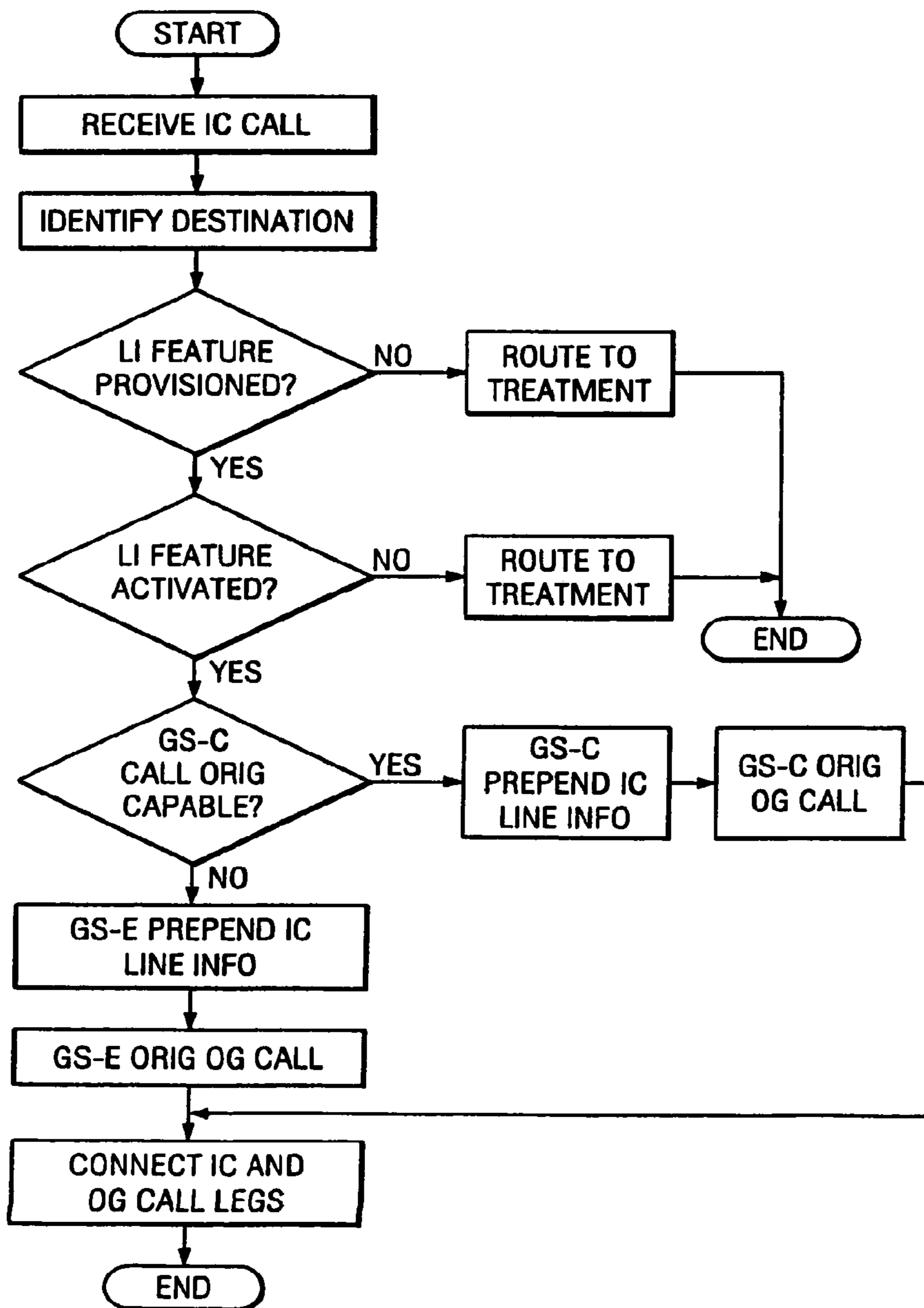
INCOMING CALL HANDLING FLOW CHART
