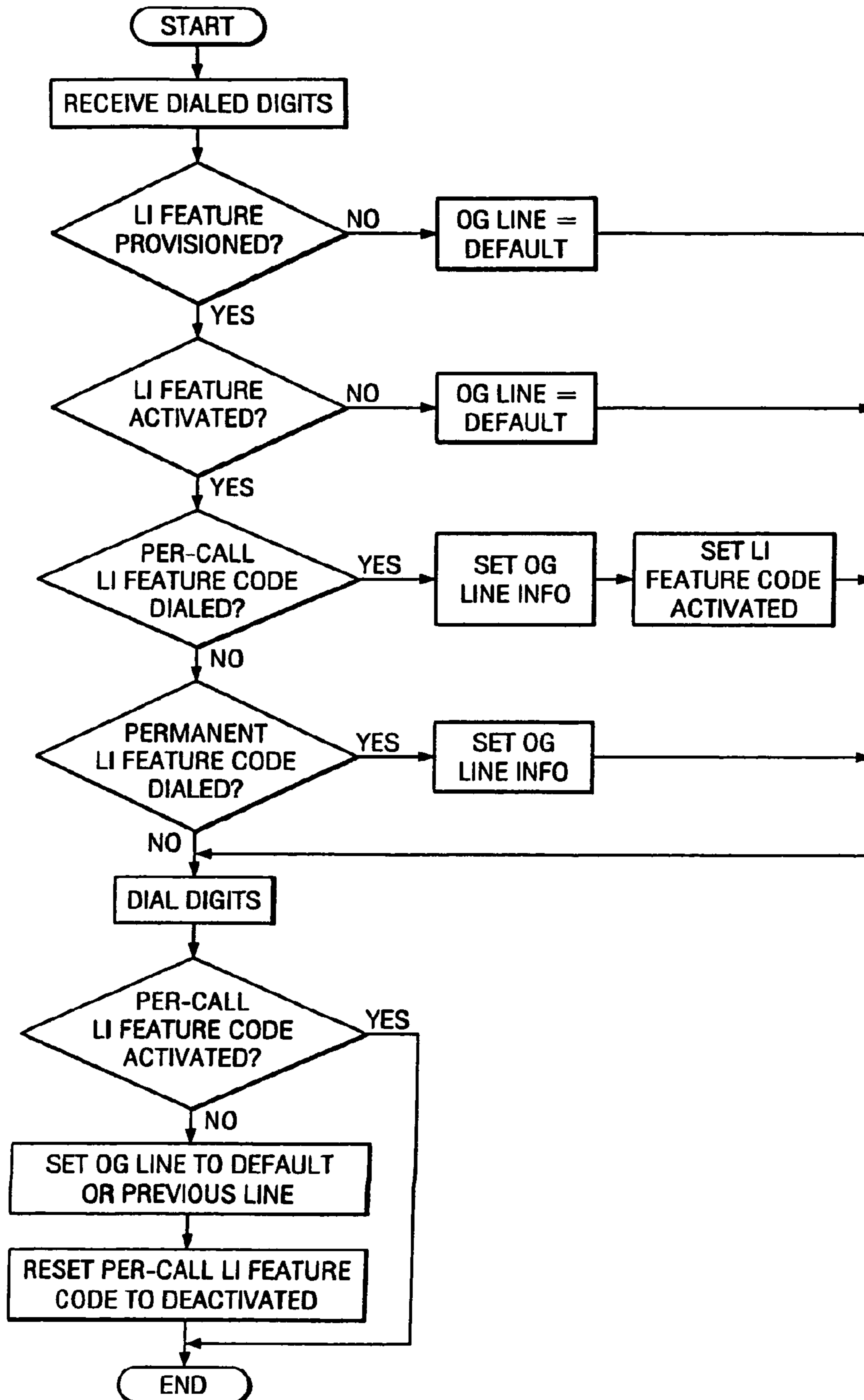
OUTGOING CALL HANDLING FLOW CHART
