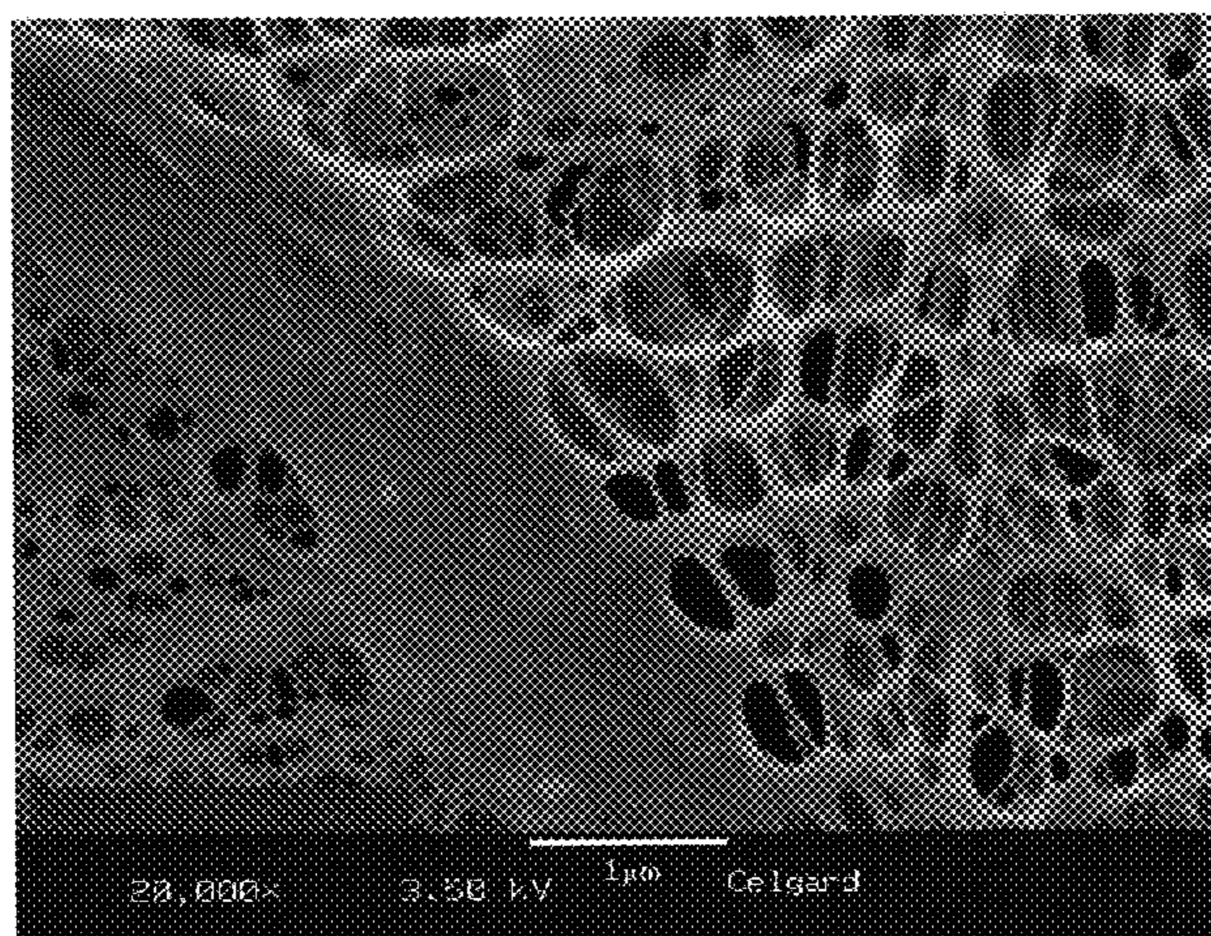
Surface SEM Micrograph of Example 5 at 20,000x Magnification.
