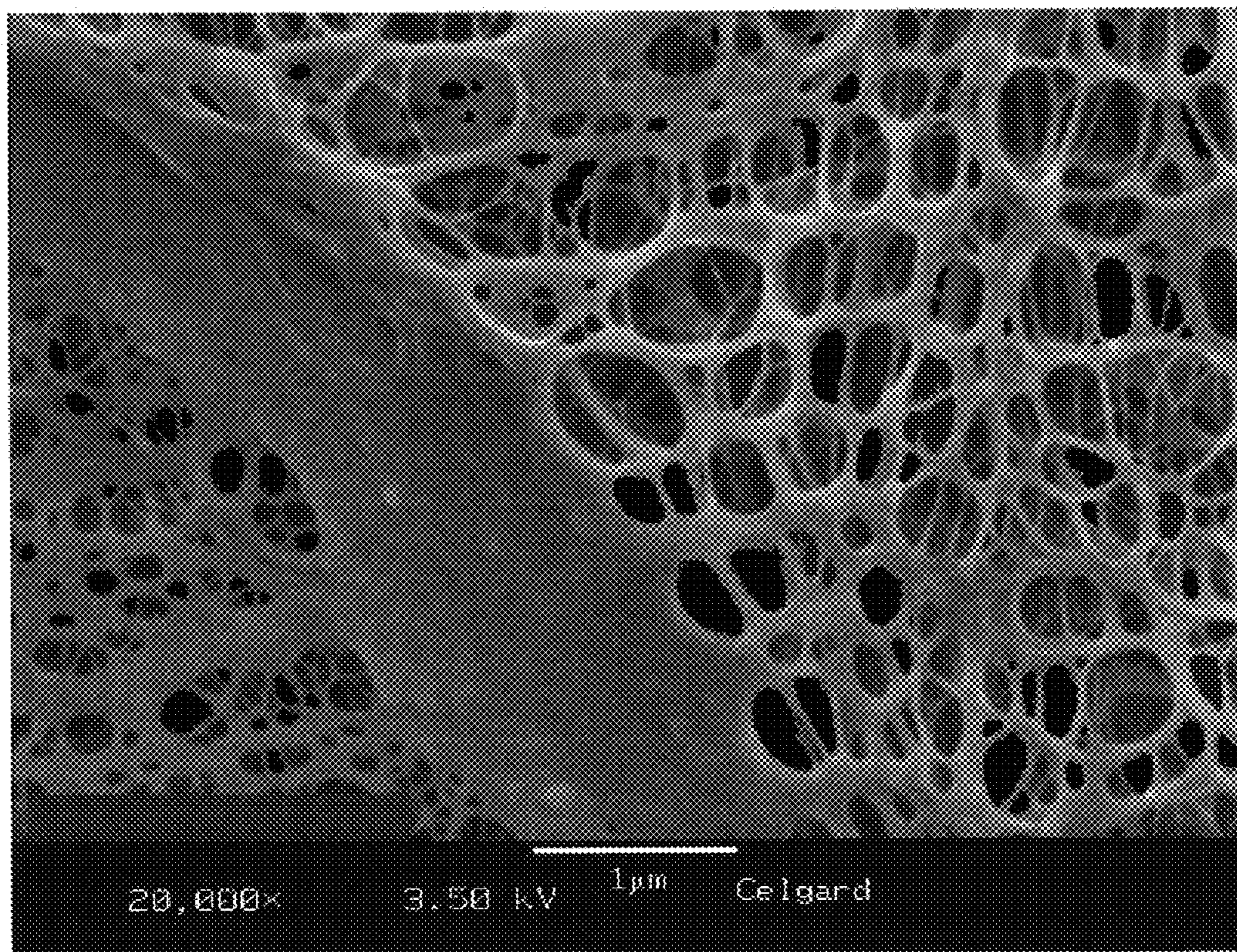
Figure 5. Surface SEM Micrograph of Example 5 at 20,000x Magnification.
