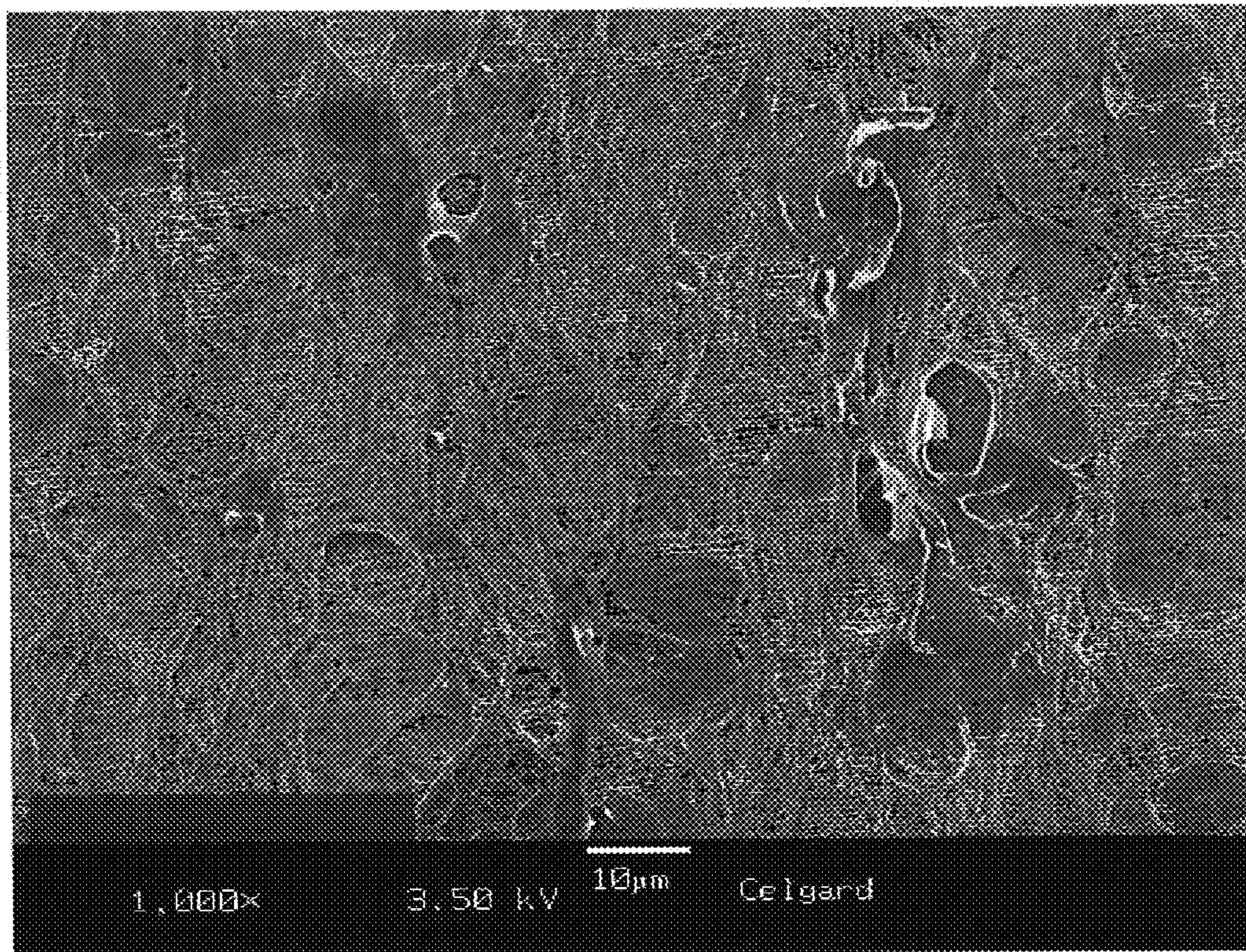
Figure 2. Surface SEM Micrograph of Example 5 at 1,000x Magnification.
