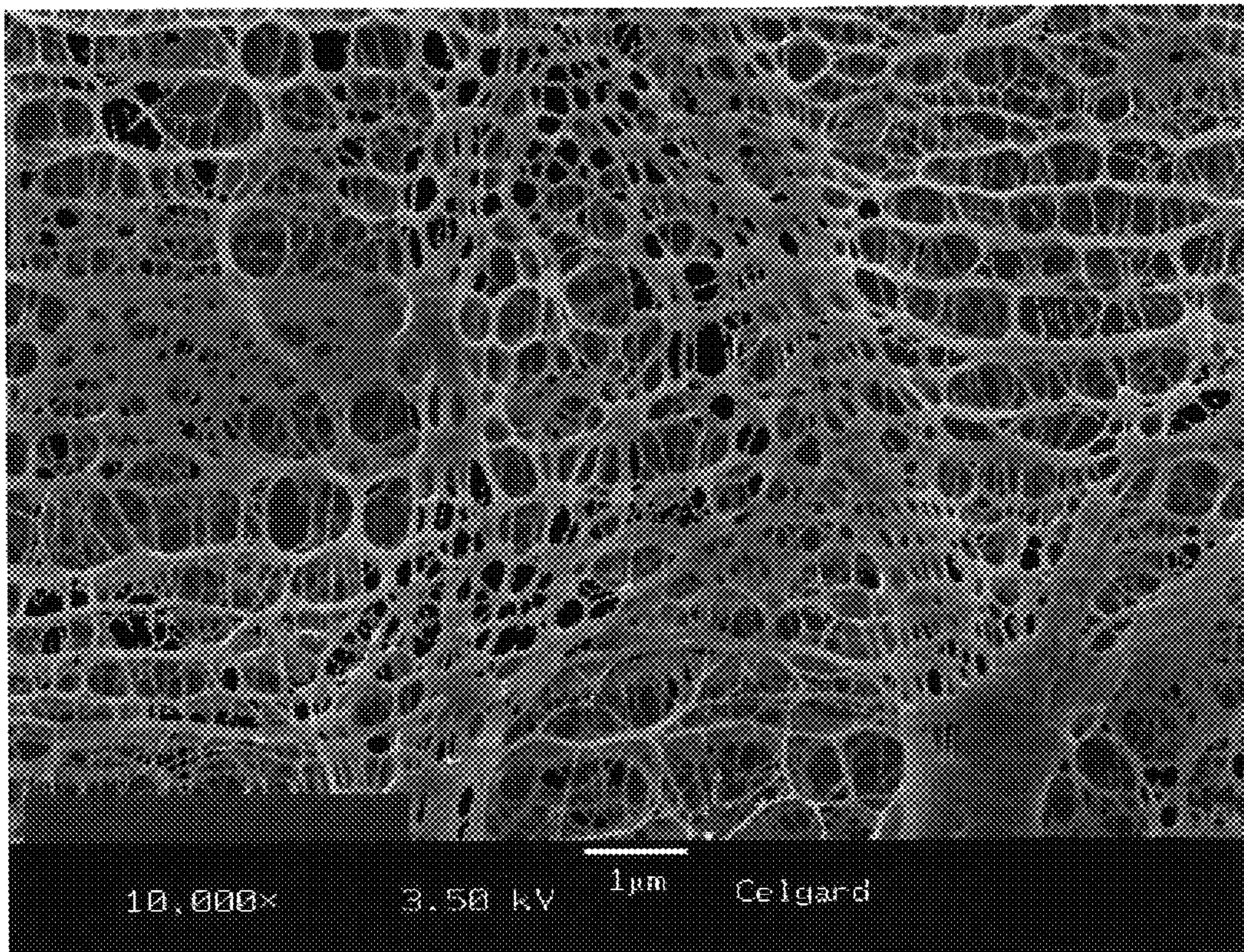
Figure 4. Surface SEM Micrograph of Example 5 at 10,000x Magnification.
