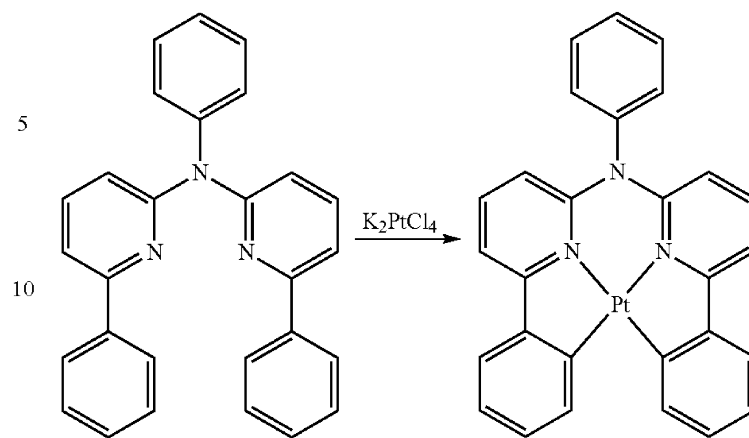
Synthesis of Compound X
