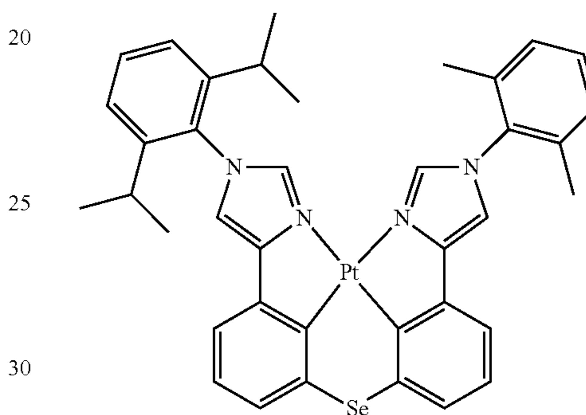
Compound 8'
