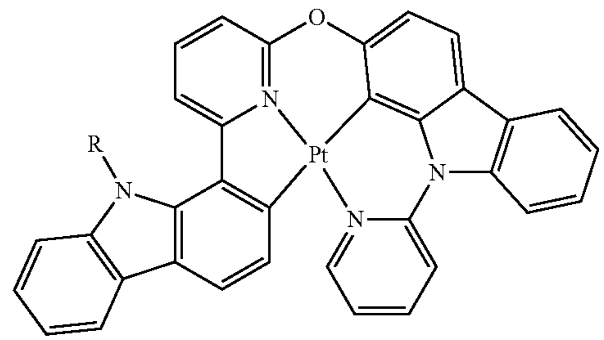
Compound 75
