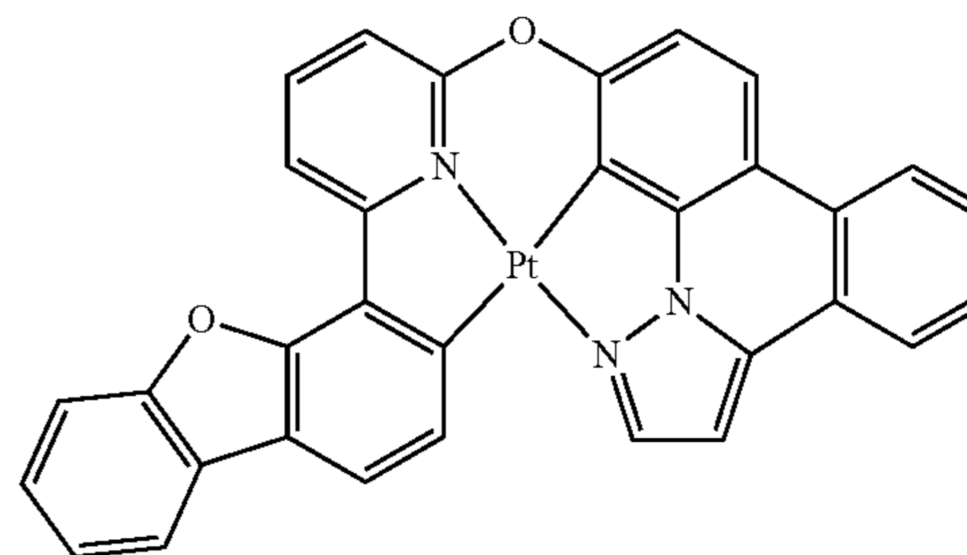
Compound 55
