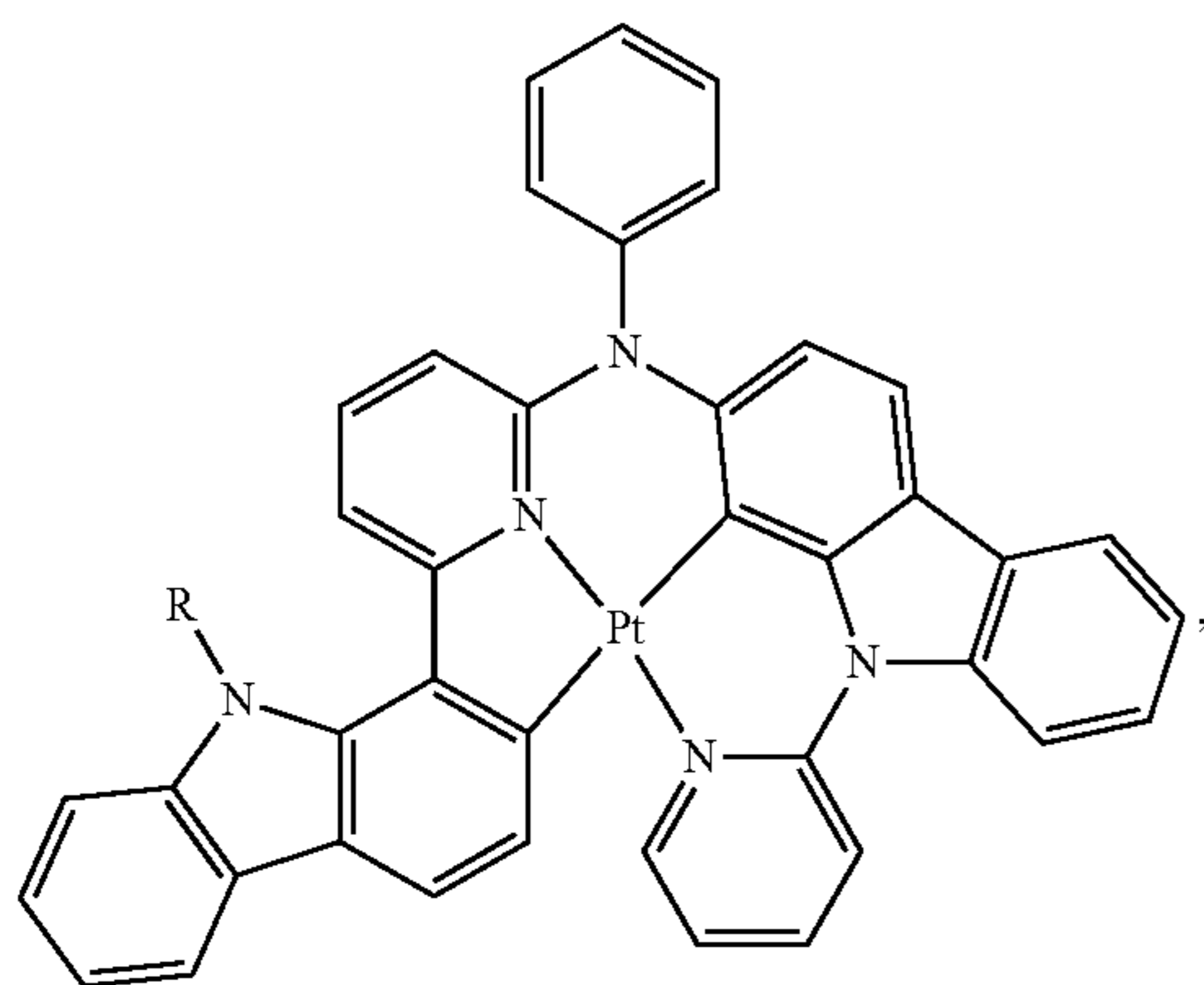
Compound 78
