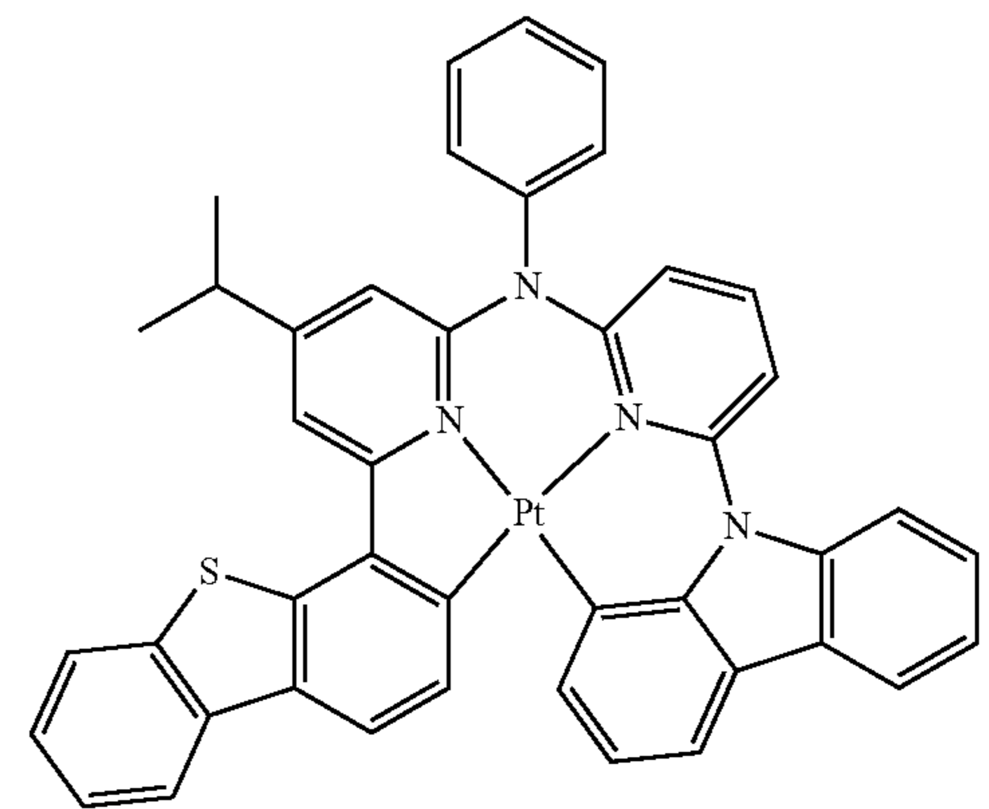
Compound 167
