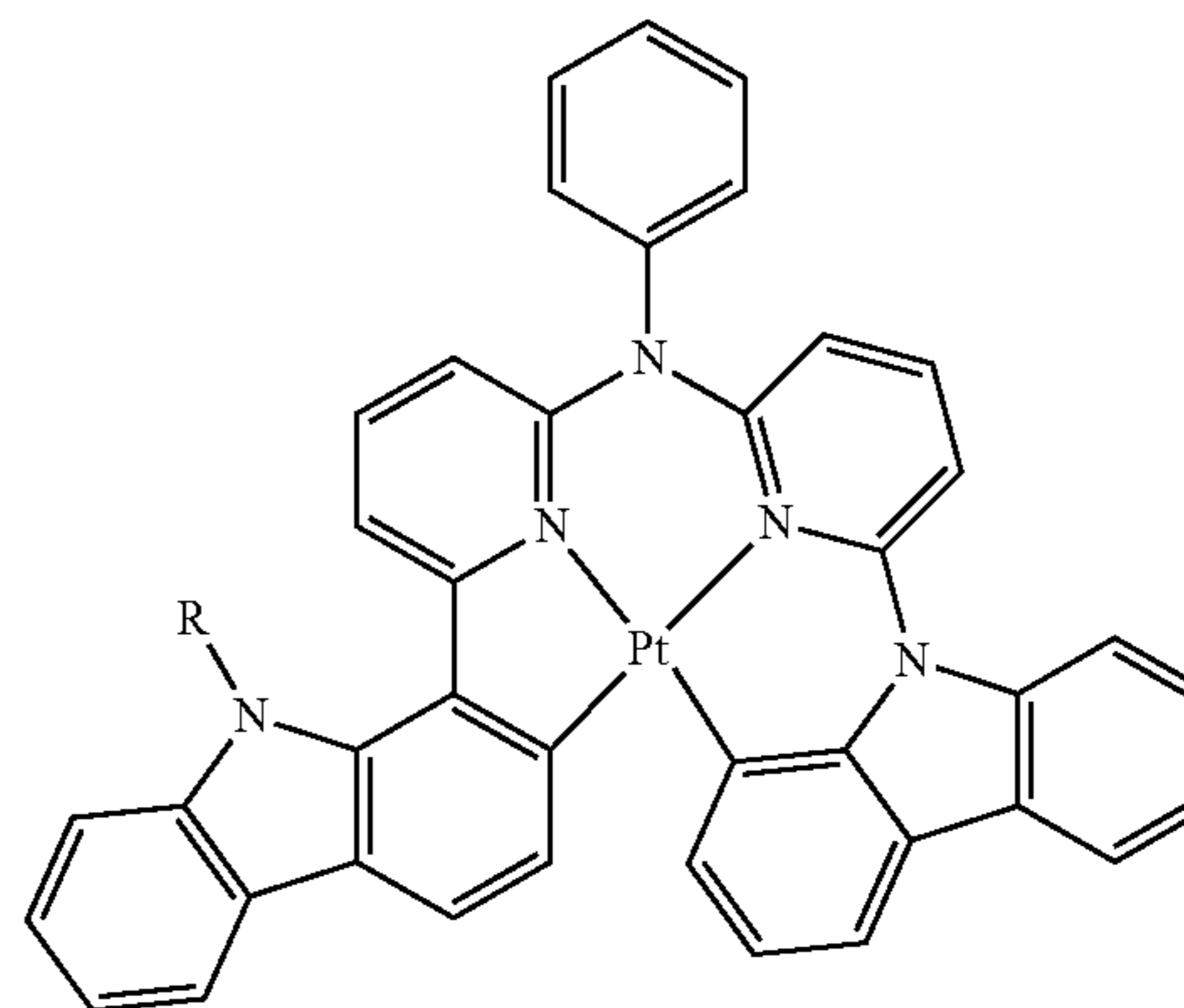
Compound 72
