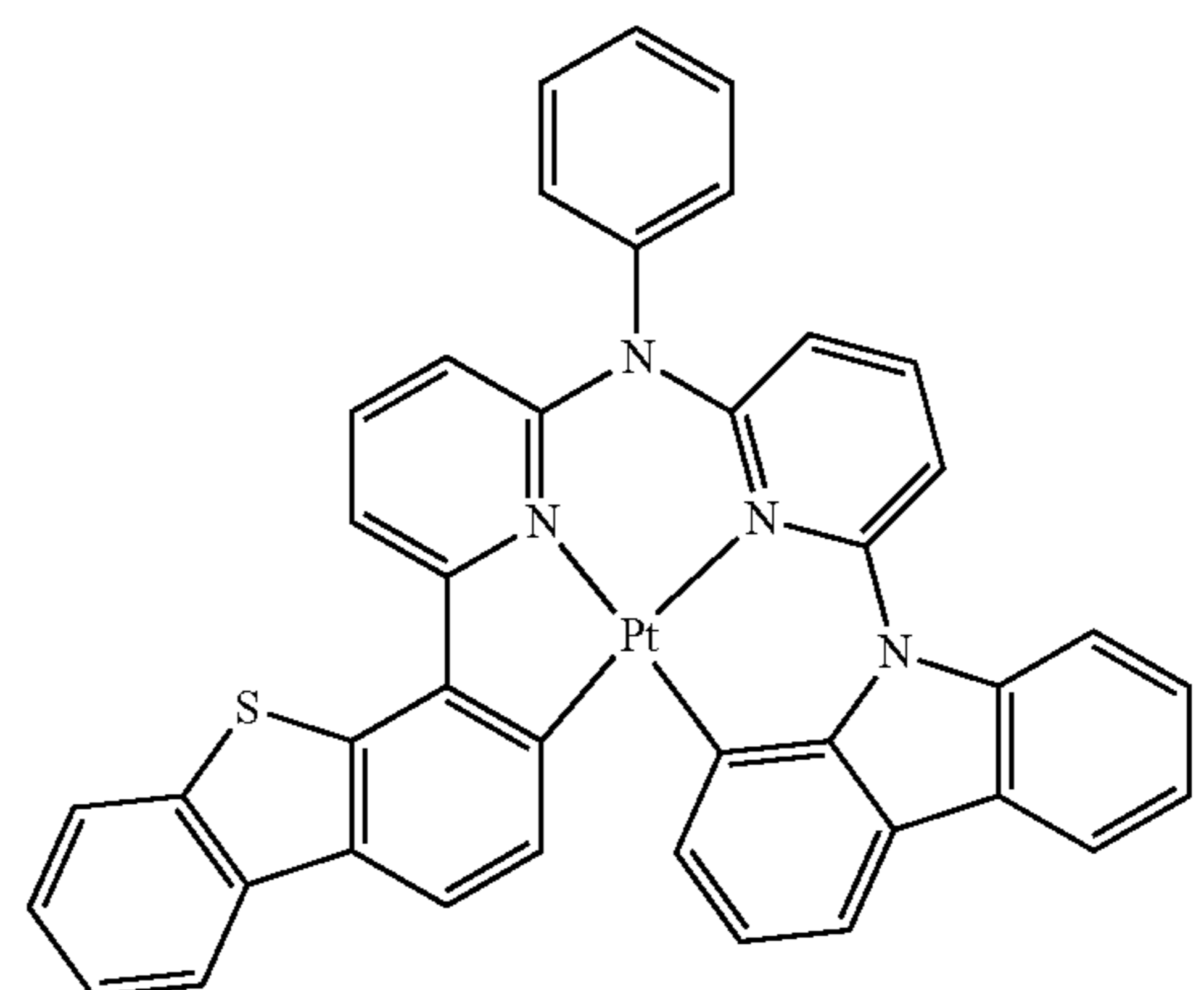
Compound 71
