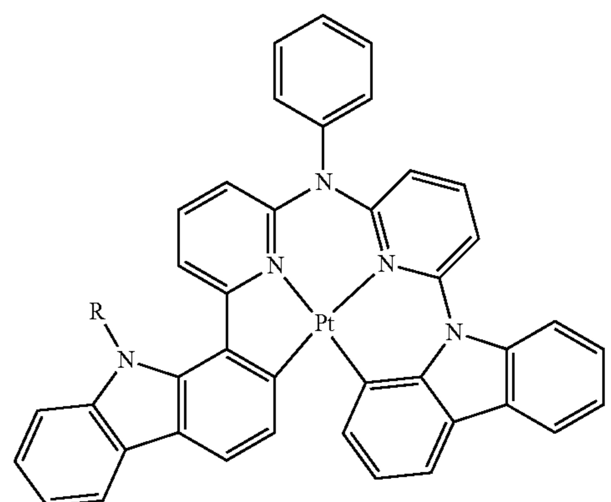
Compound 72
