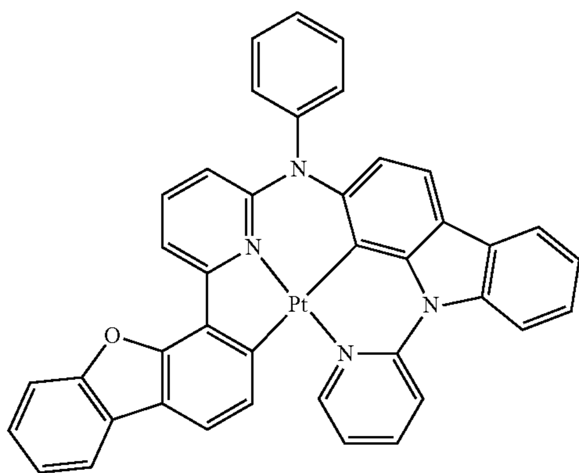
Compound 76
