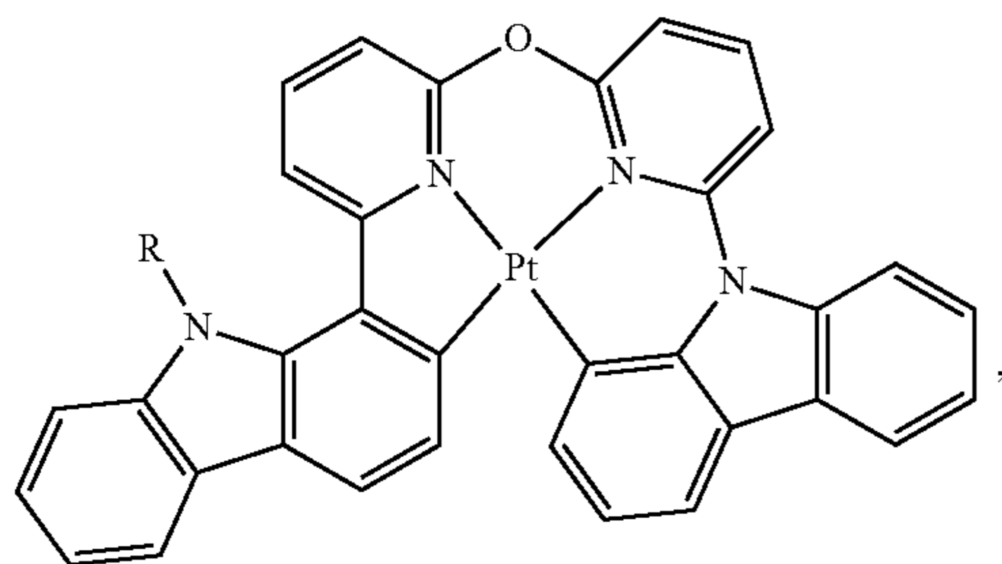
Compound 70
