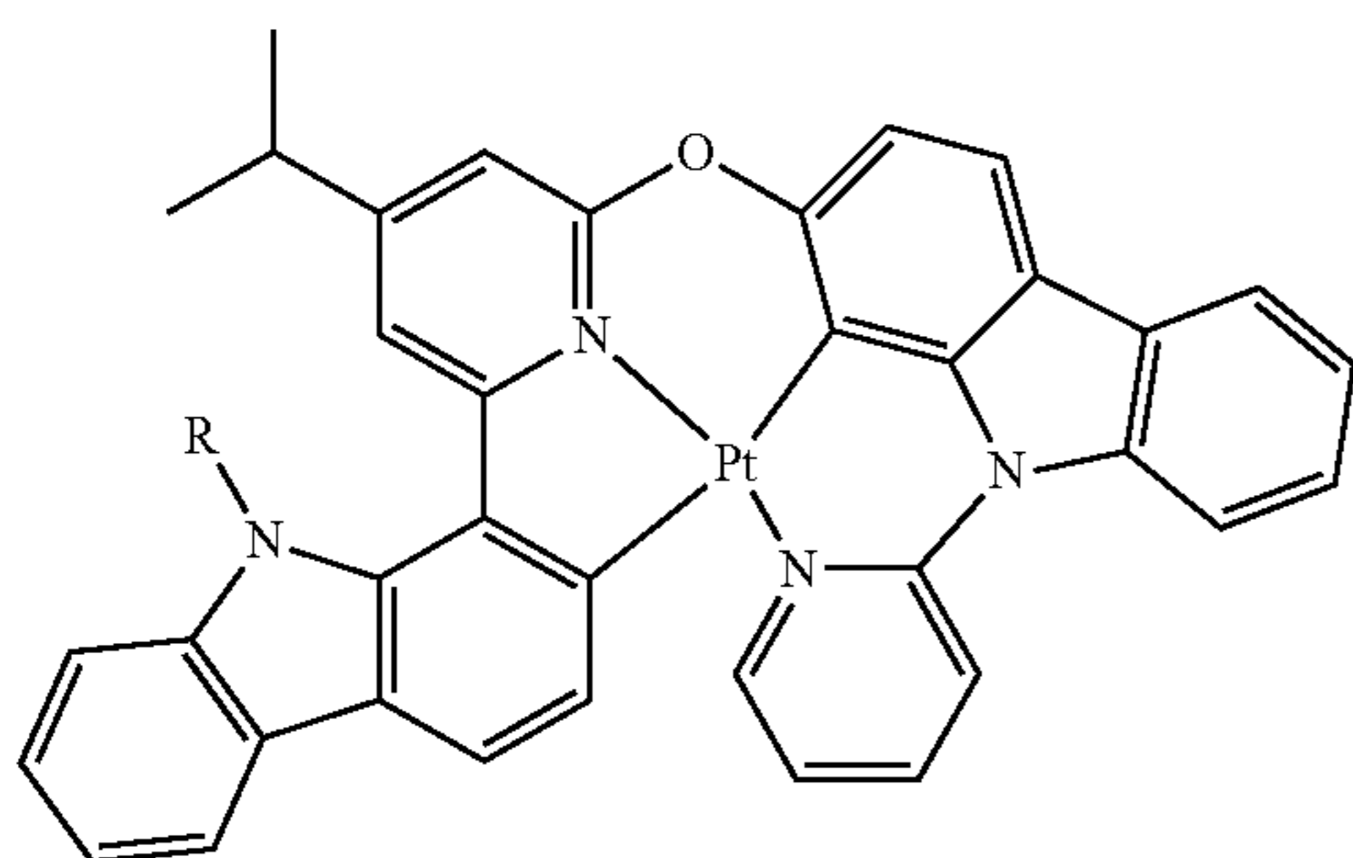
Compound 172
