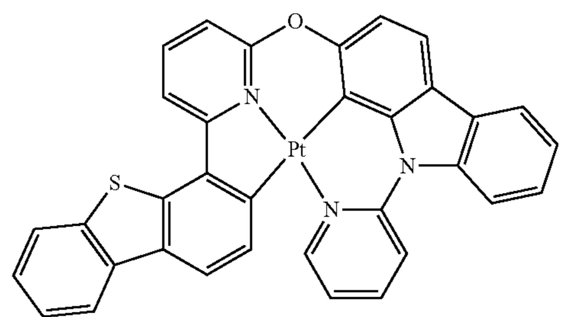
Compound 74
