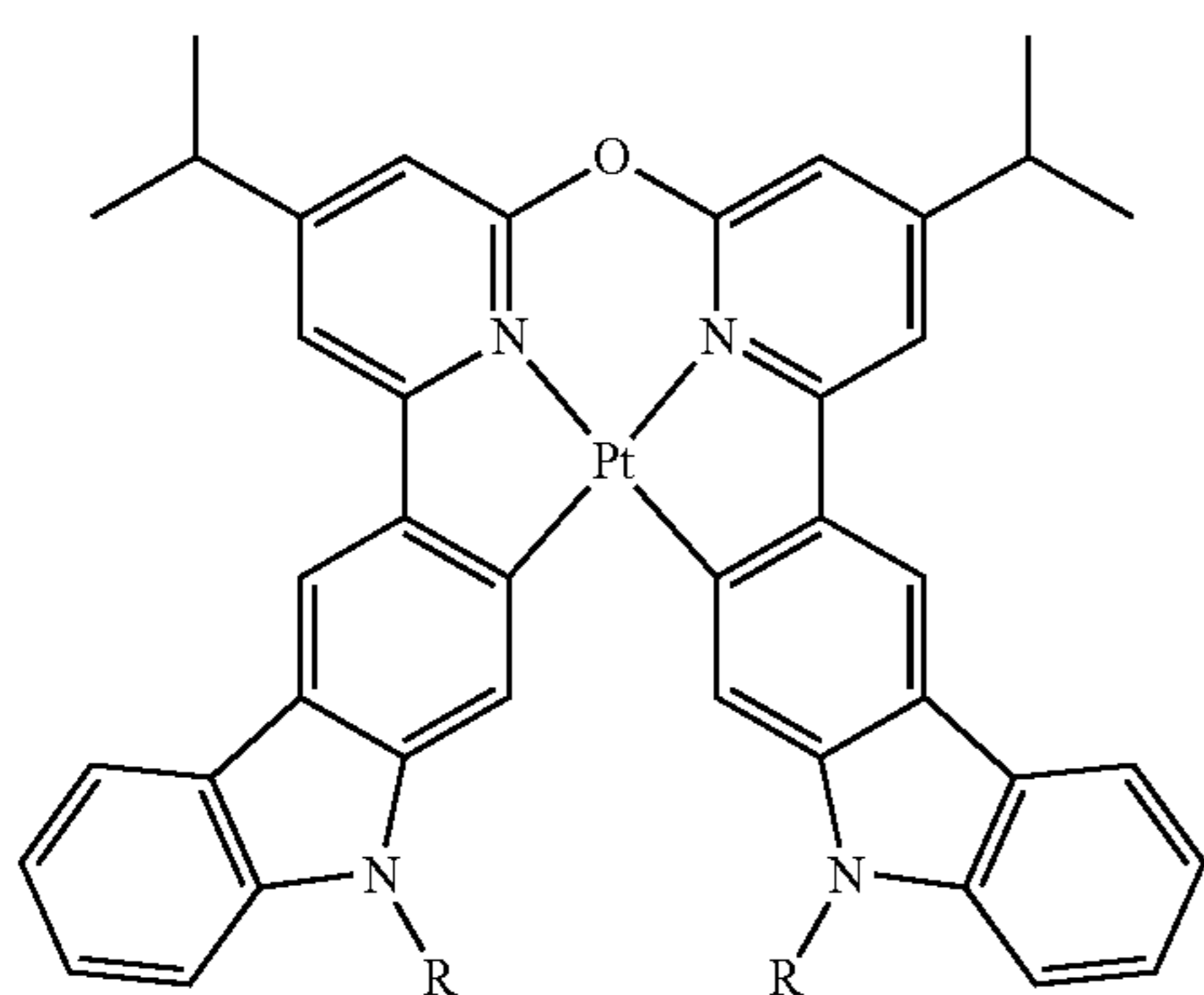
Compound 147
