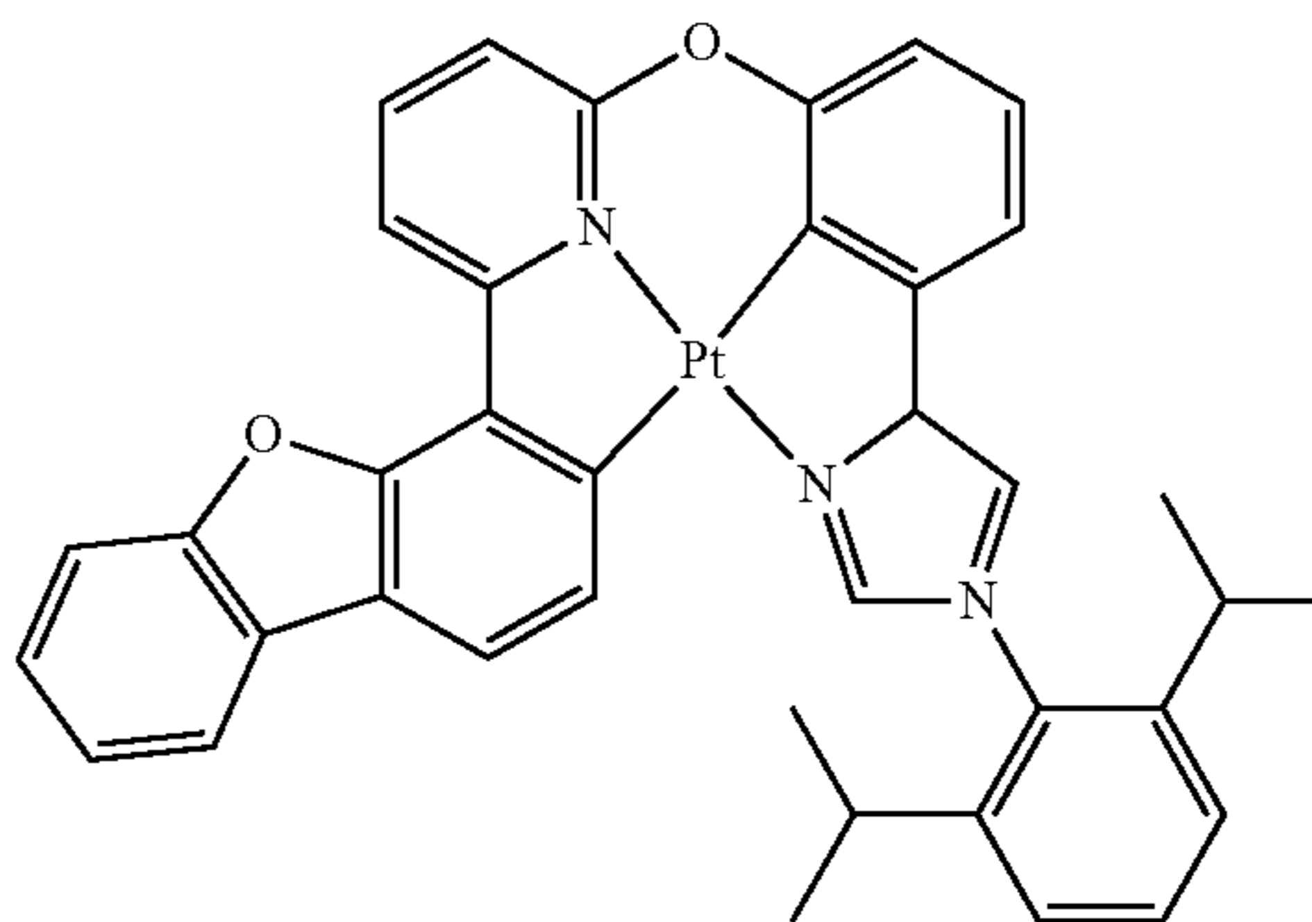
Compound 31
