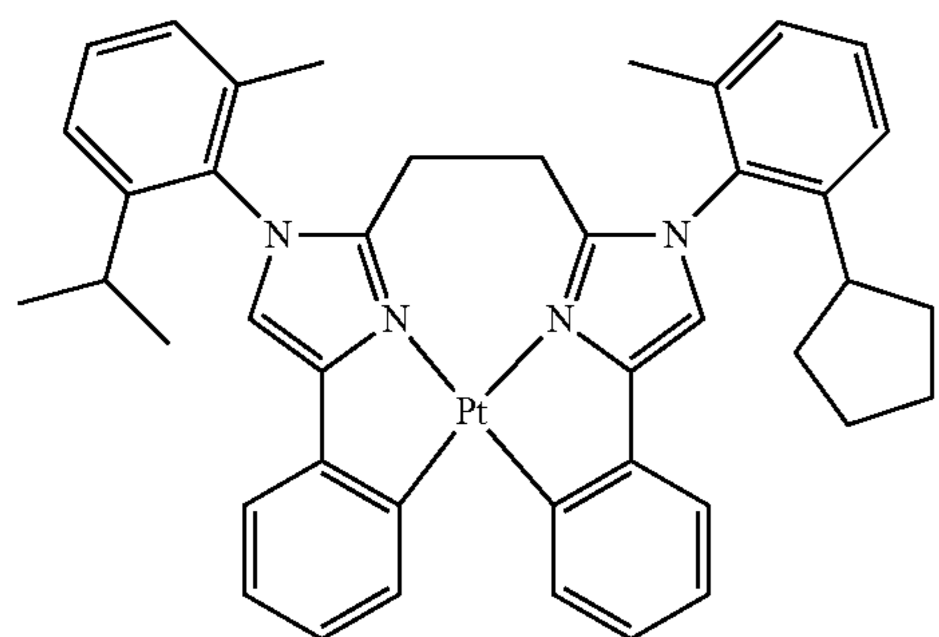
Compound 27'
