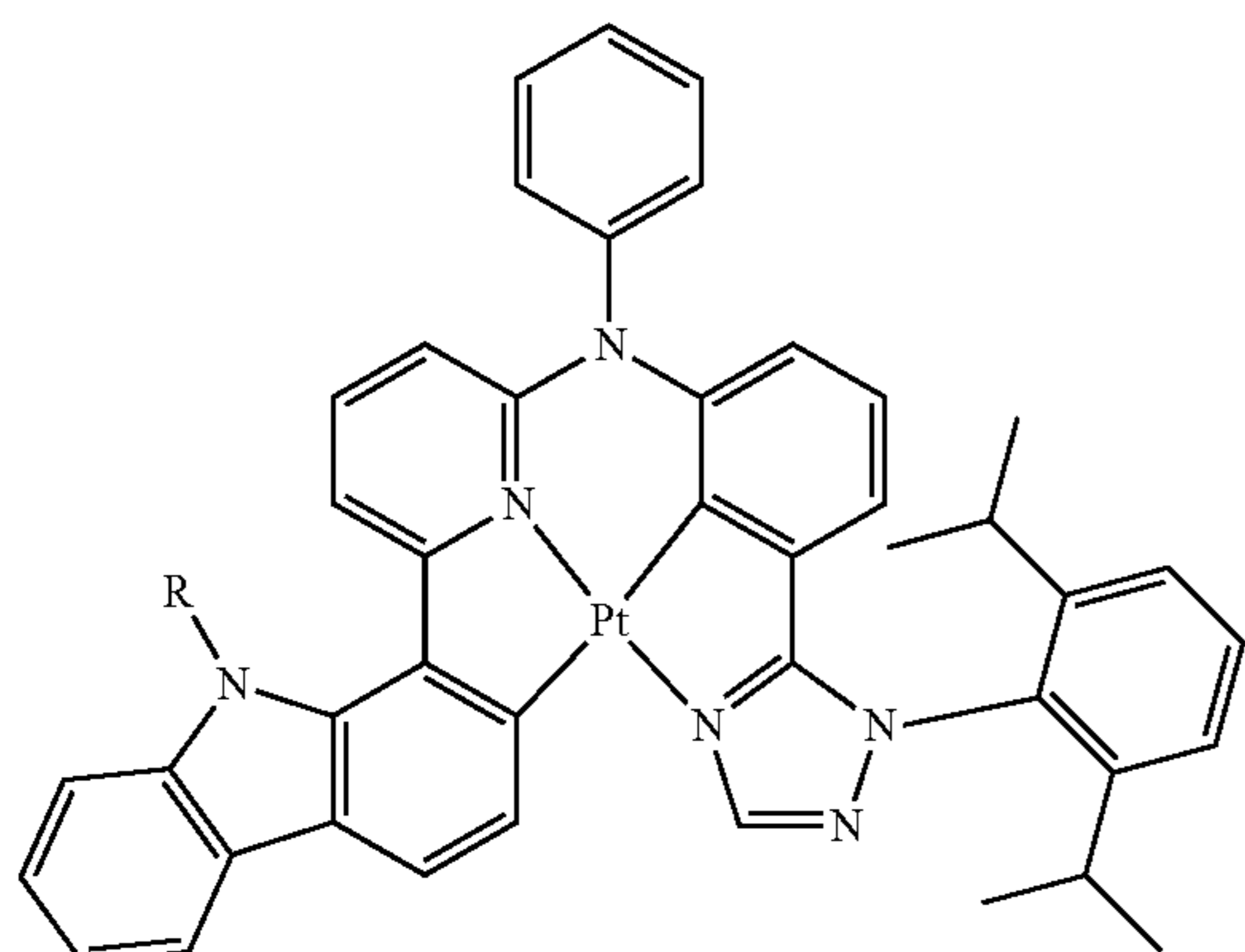
Compound 48
