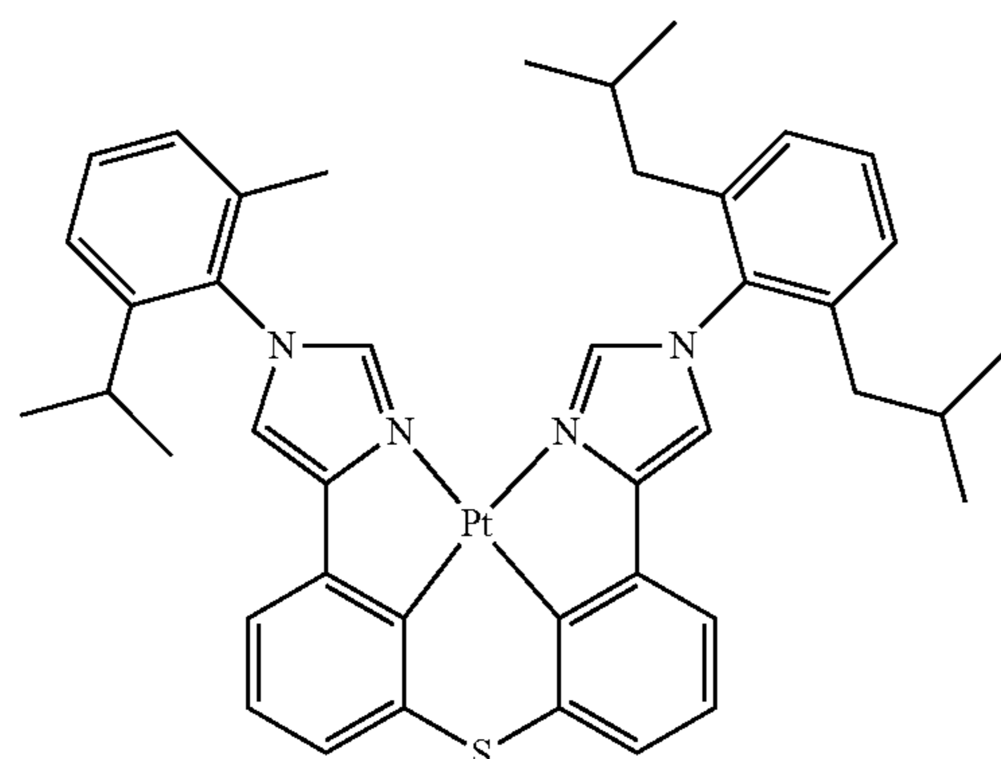
Compound 24'
