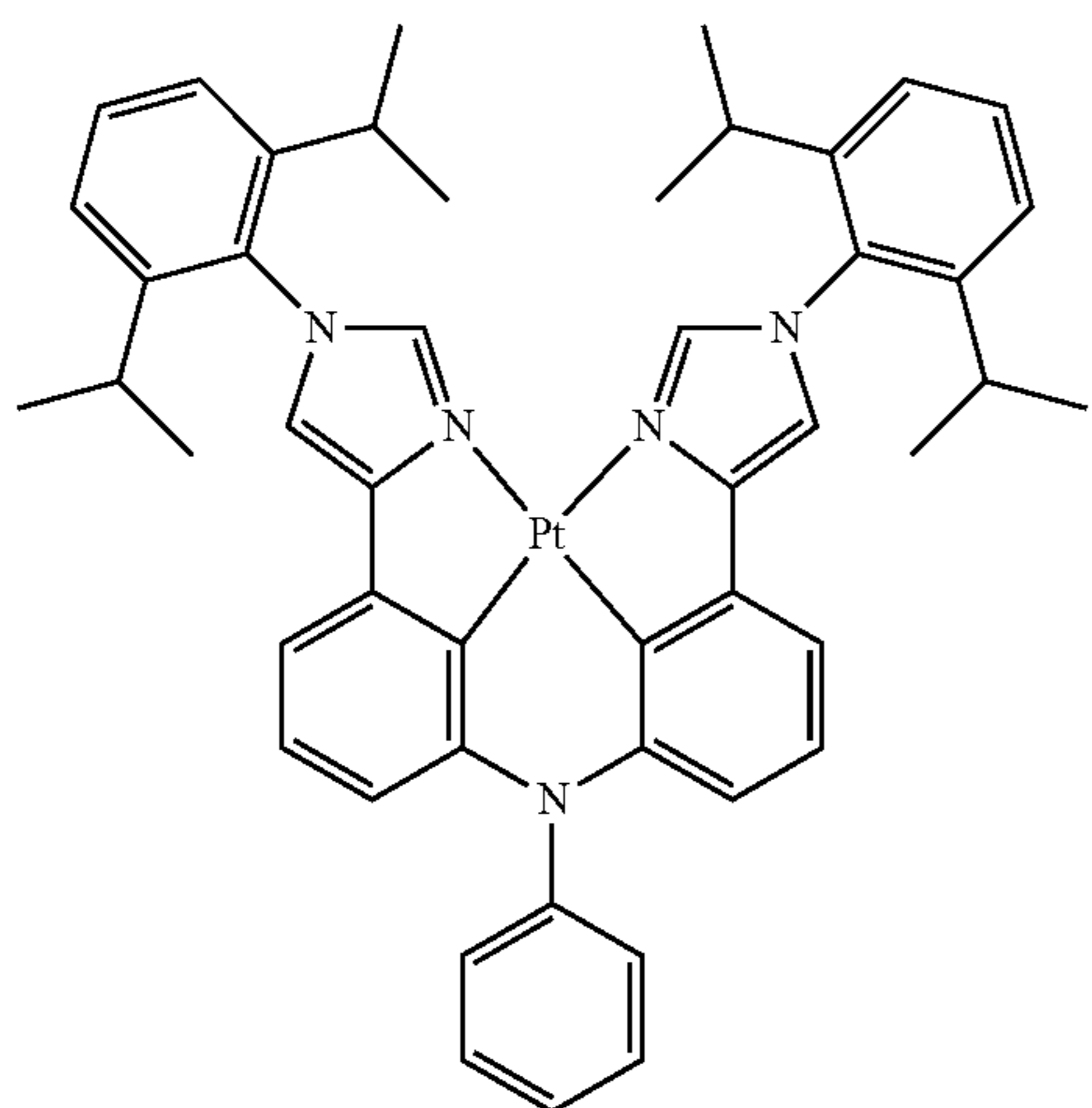
Compound 3'
