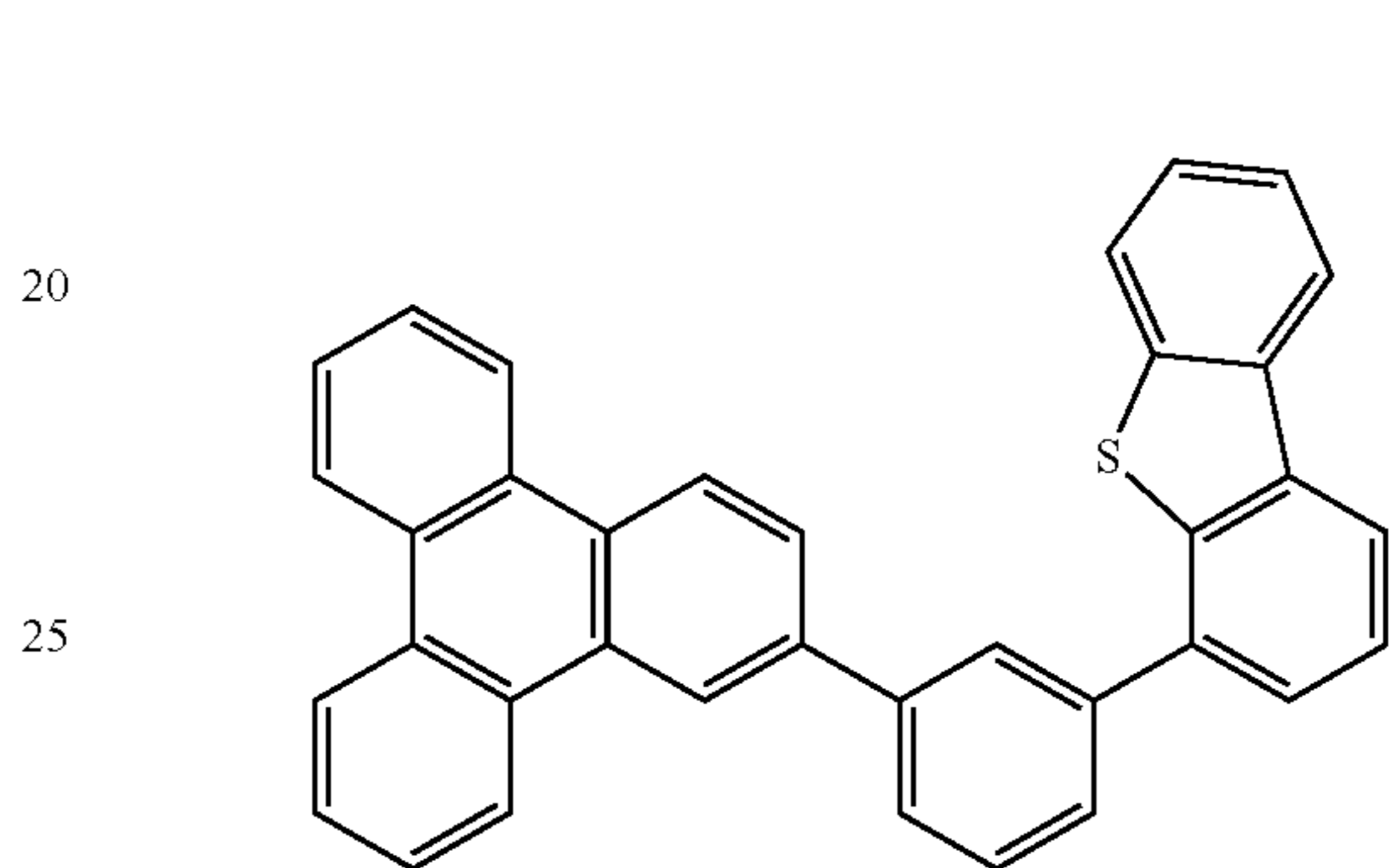
Formula I,
