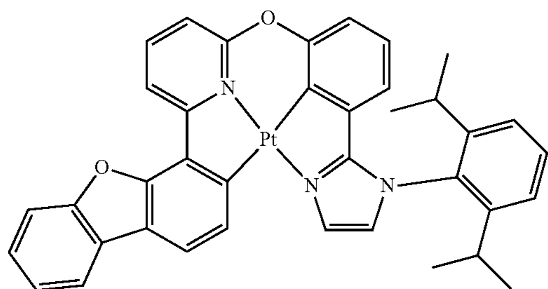
Compound 19
