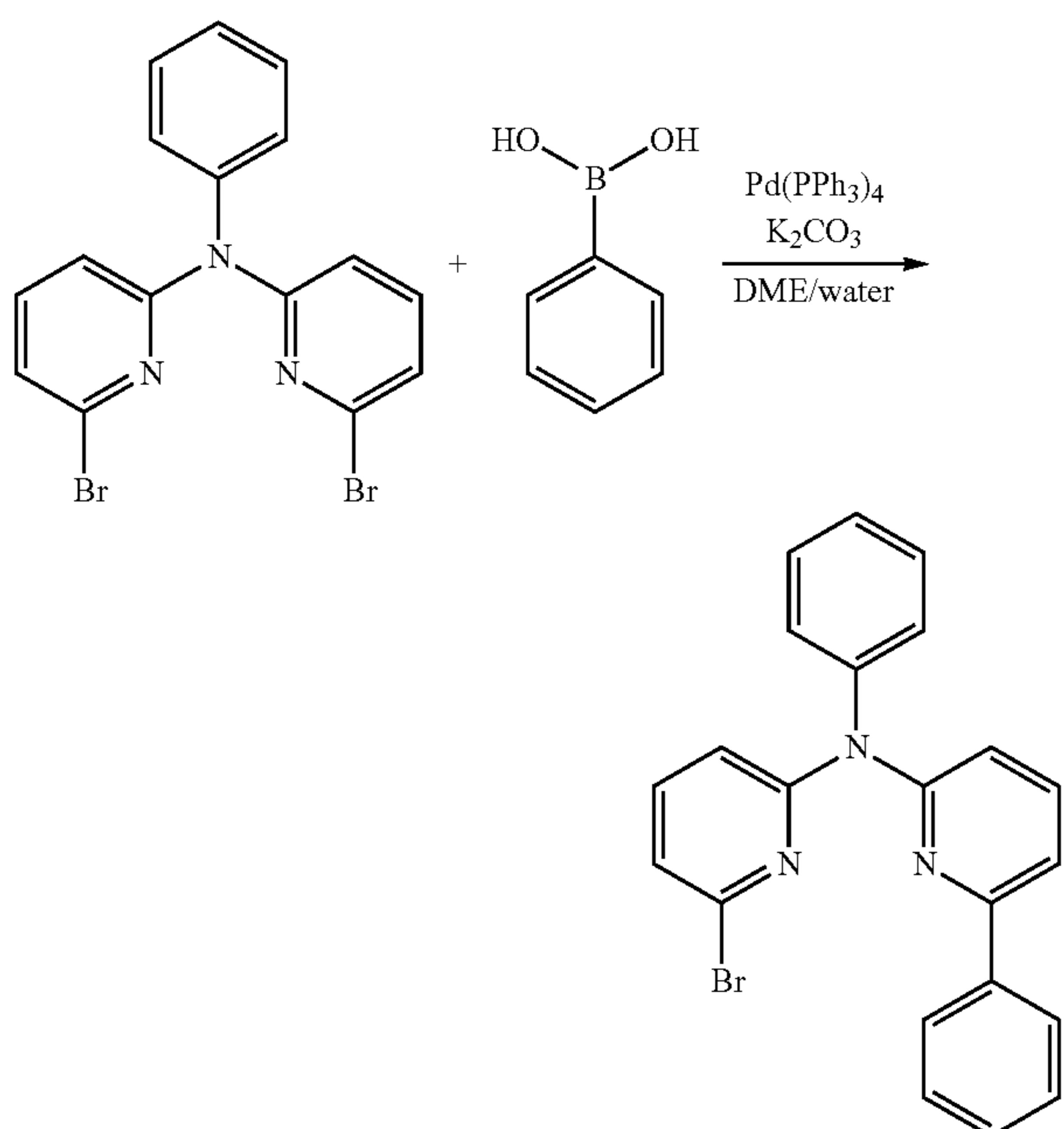
Synthesis of 6-bromo-N-phenyl-N-(6-phenylpyridin-2-yl)pyridine-2-amine
