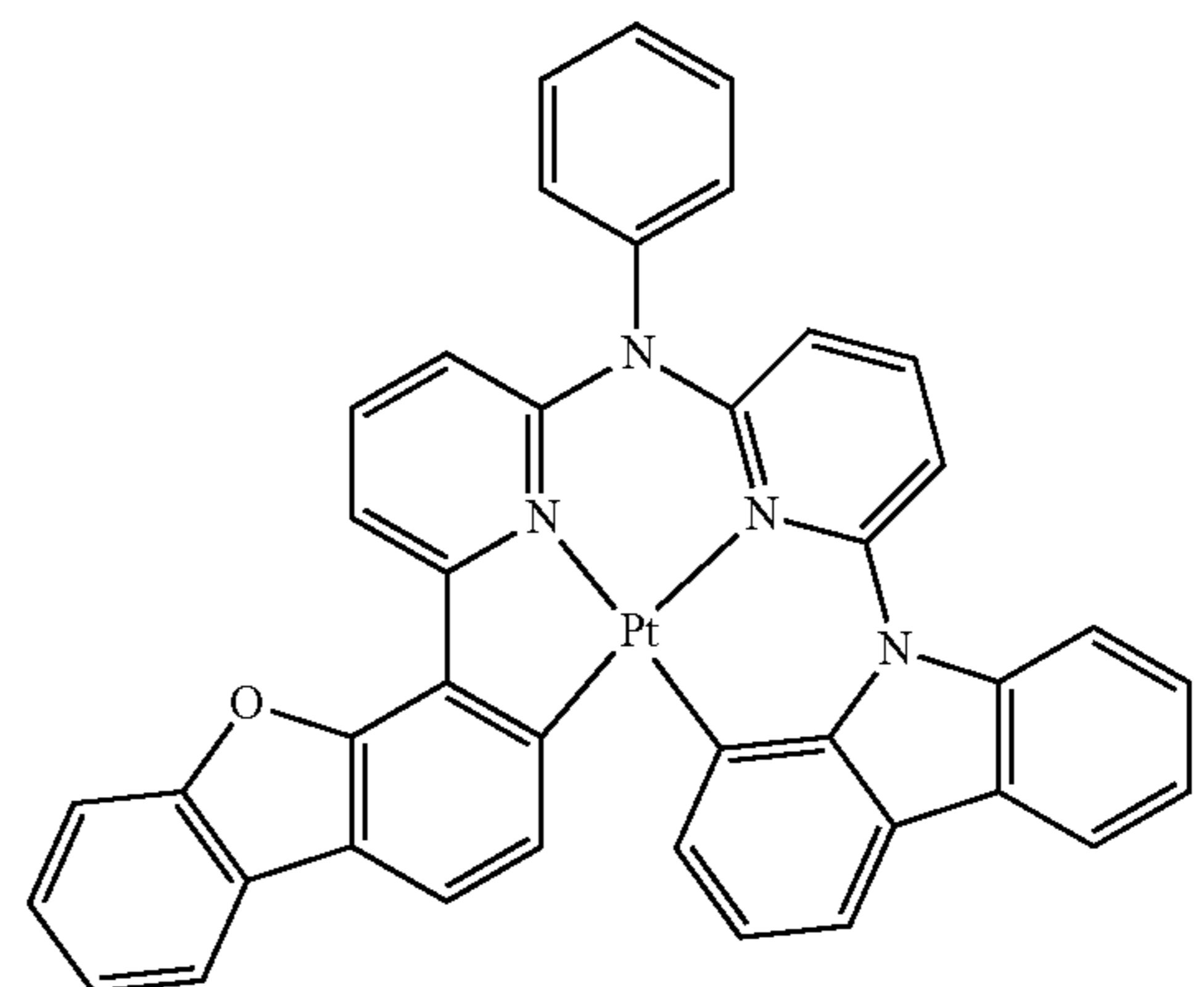
Compound 71
