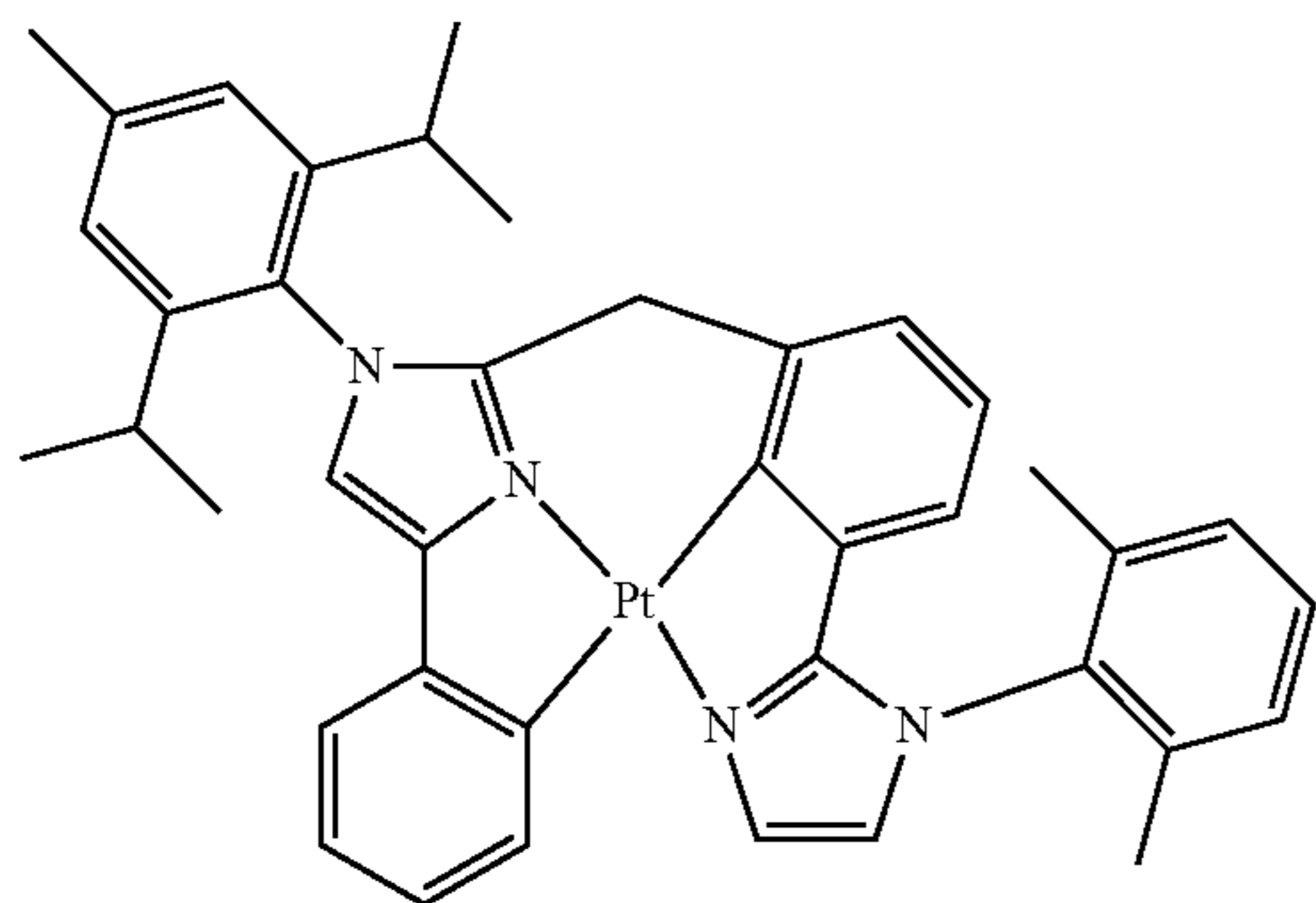
Compound 61'
