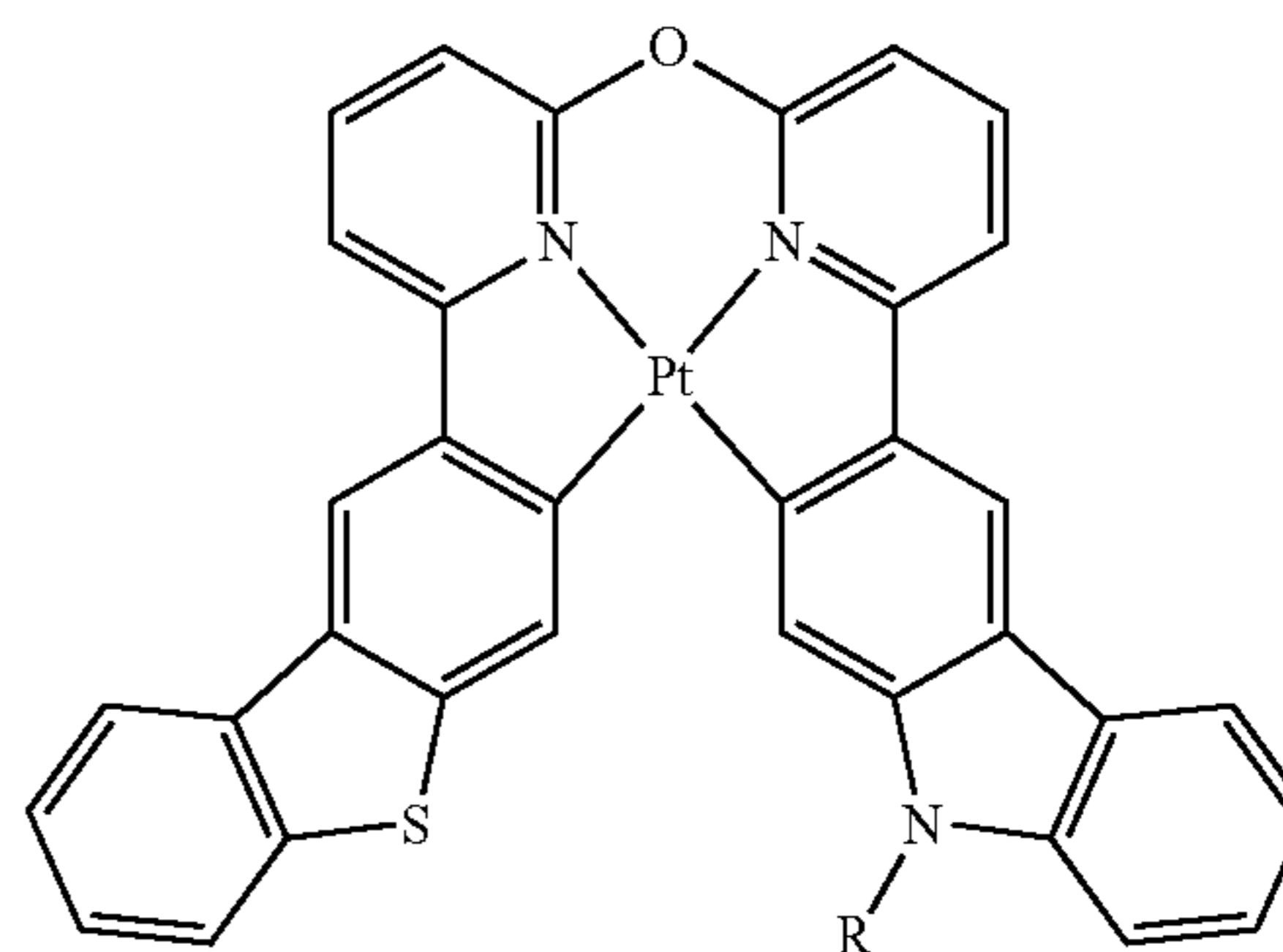
Compound 151
