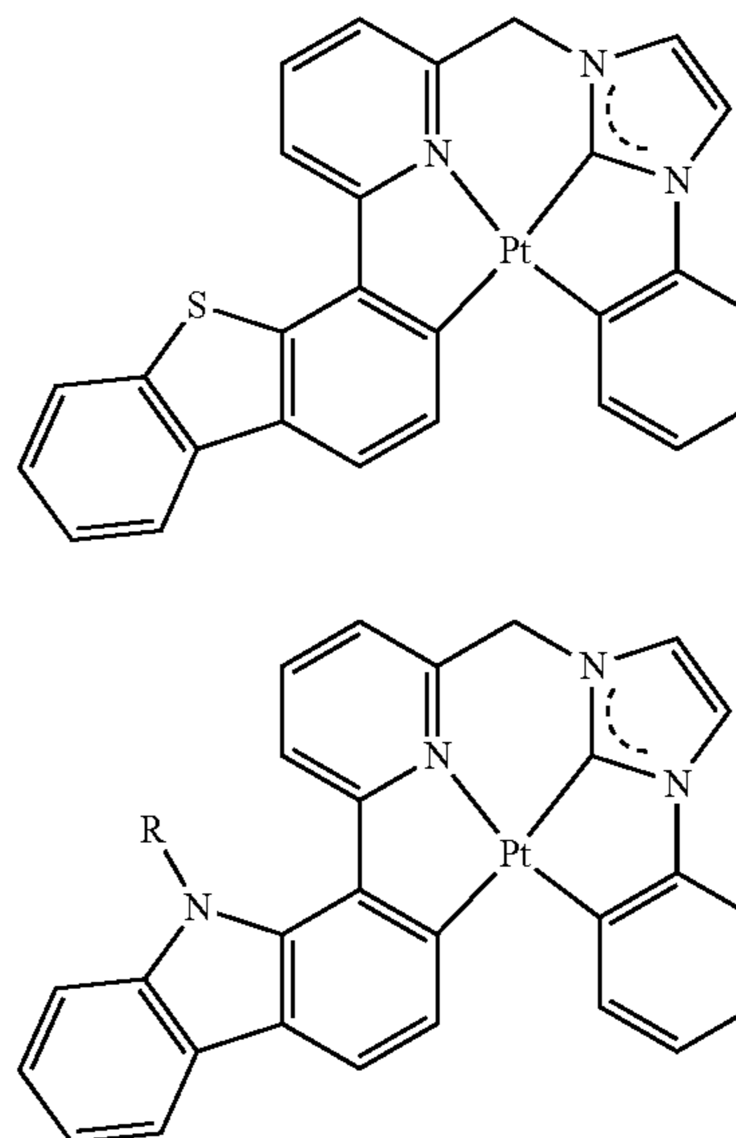
Compound 120
