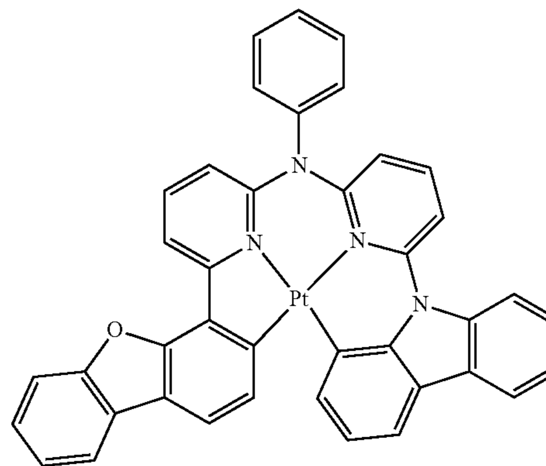
Compound 71
