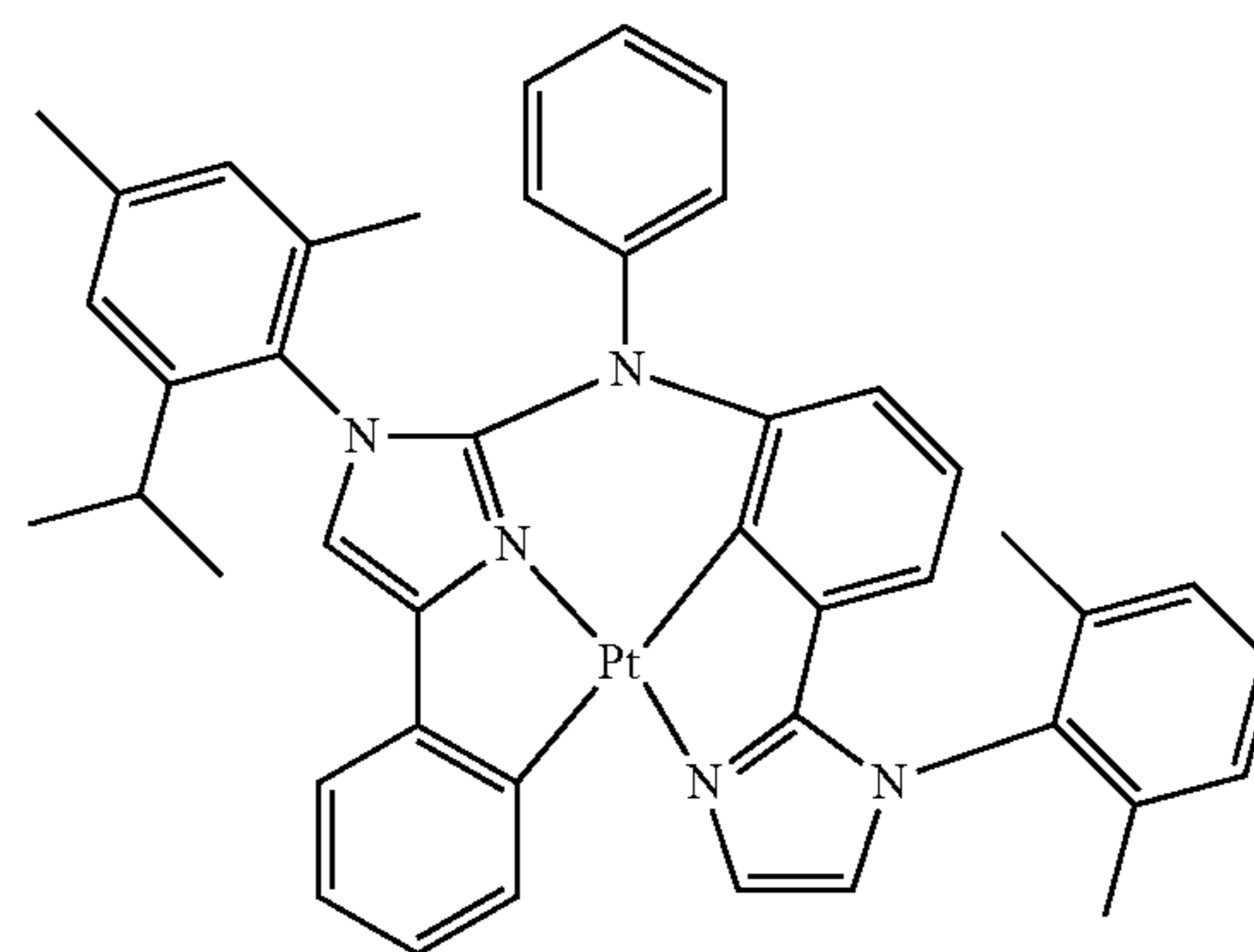
Compound 63'
