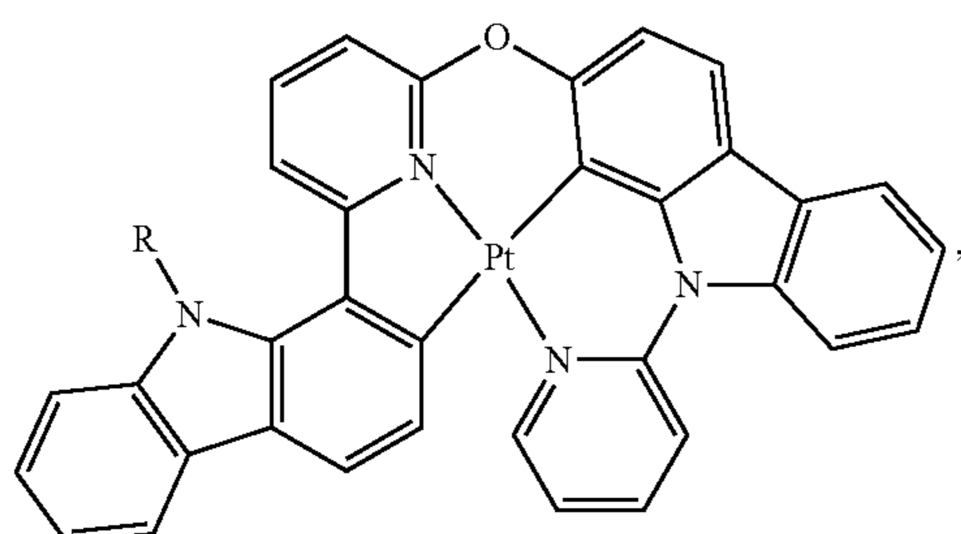
Compound 75
