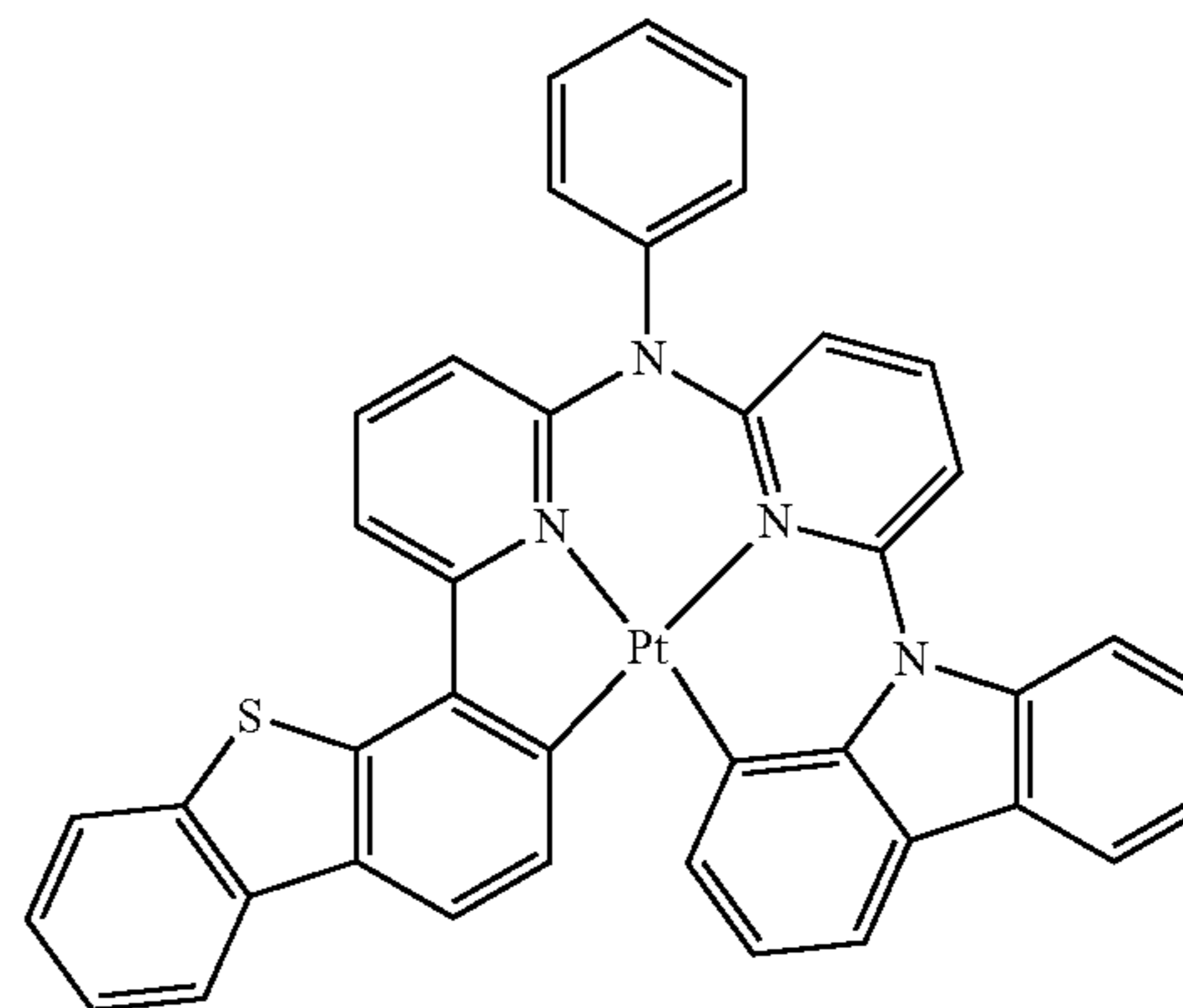
Compound 71
