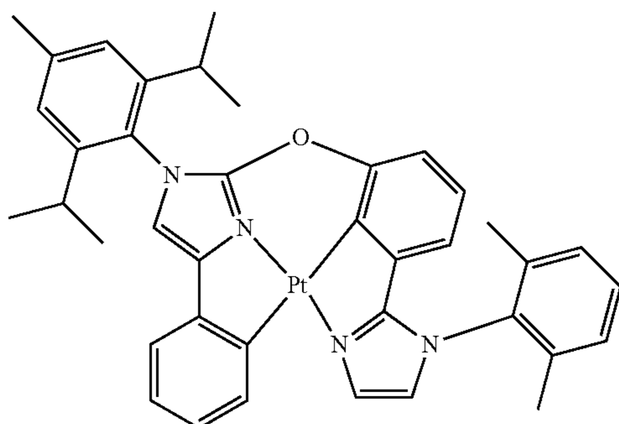
Compound 63'
