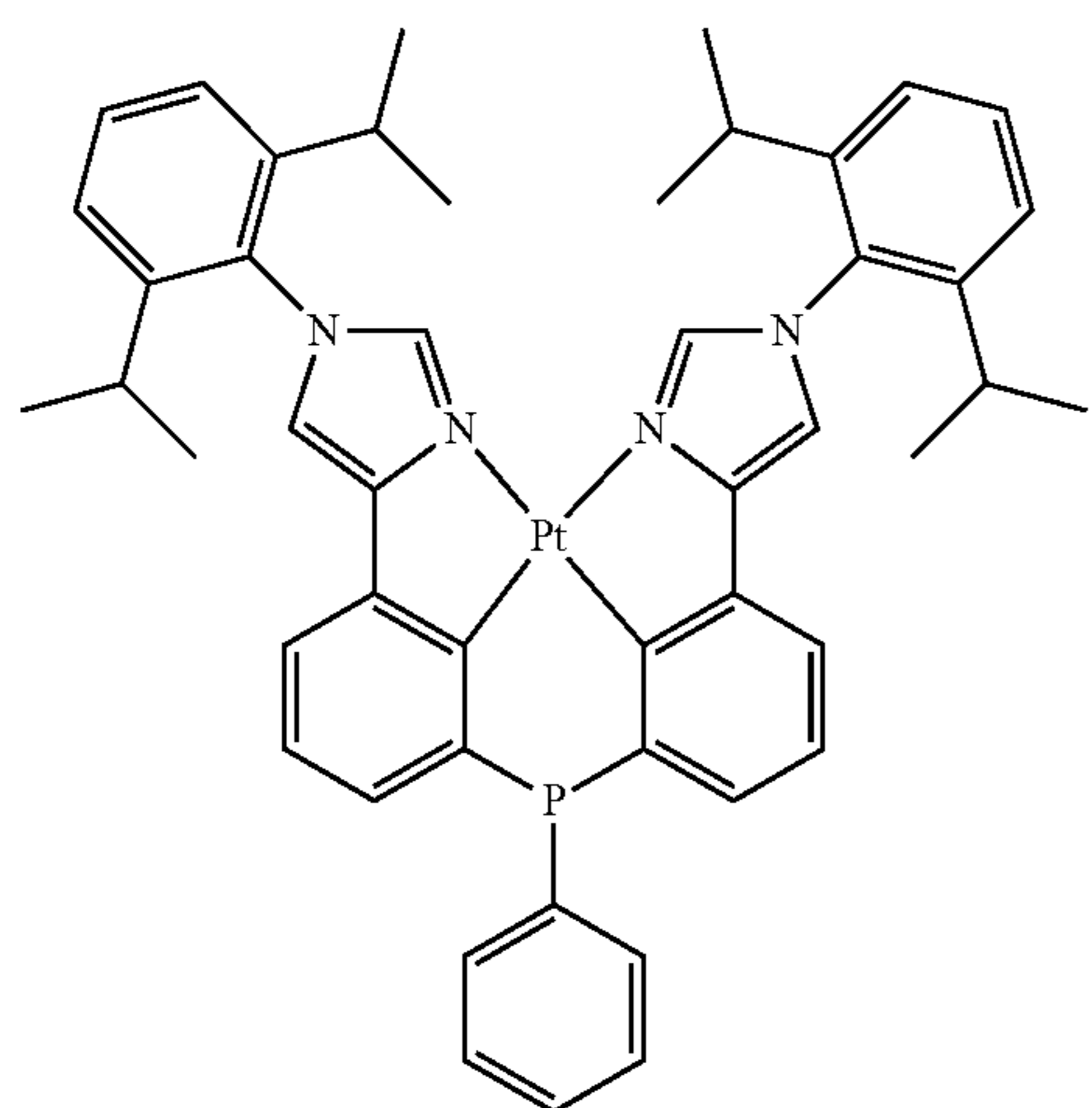
Compound 15'
