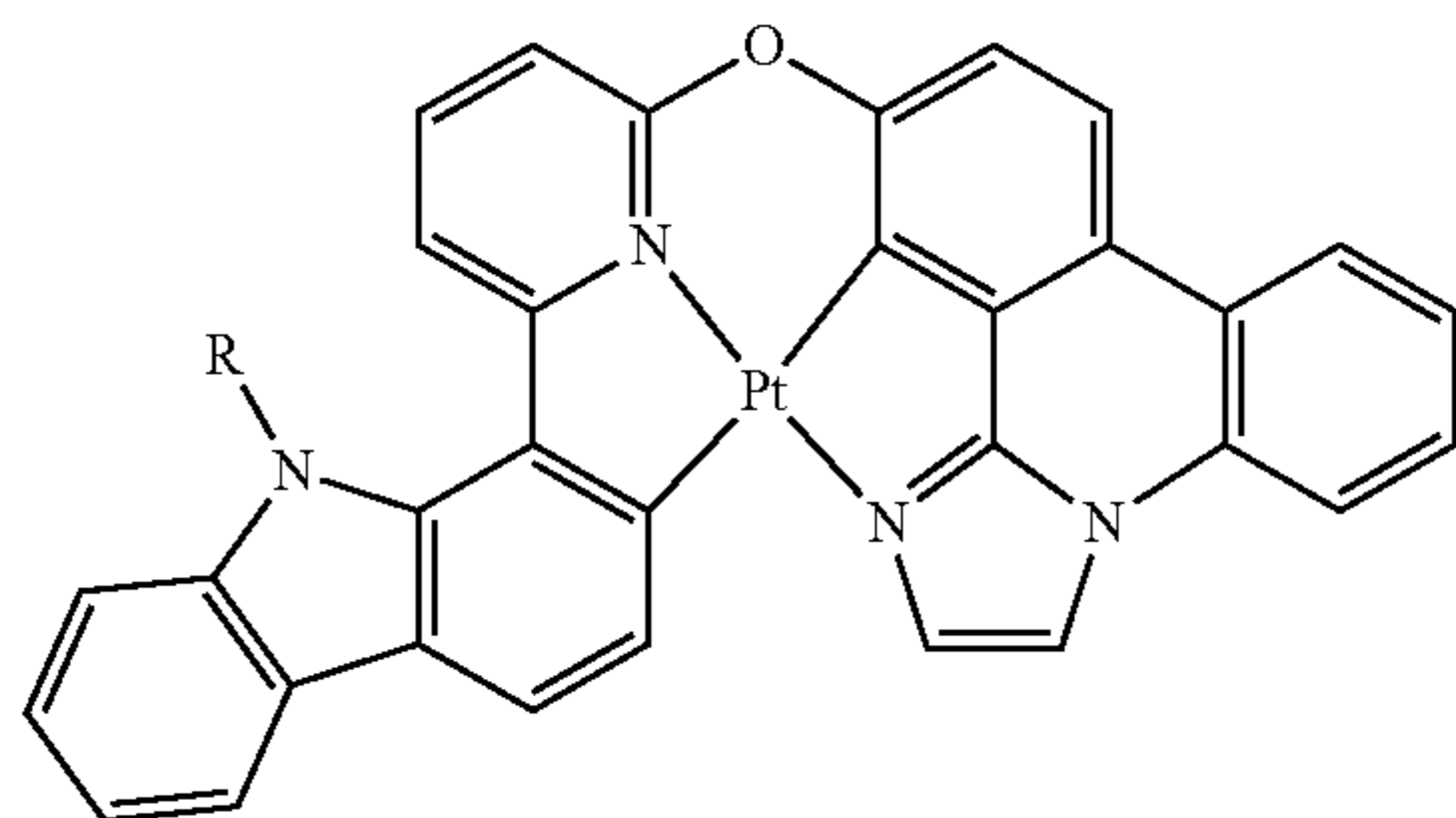
Compound 51
