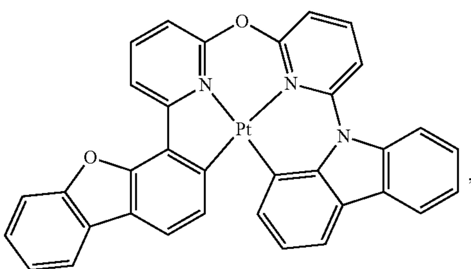
Compound 67
