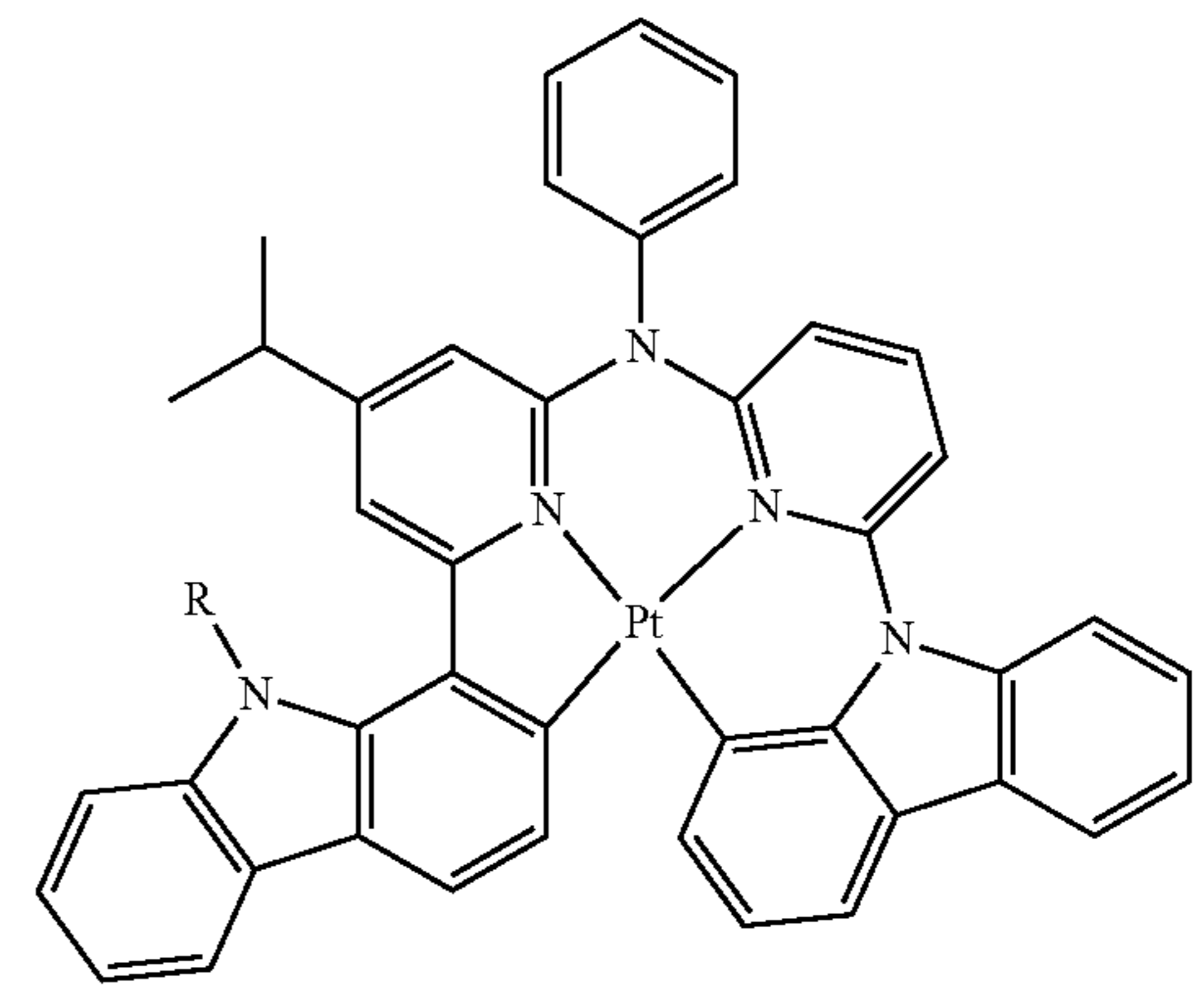
Compound 168
