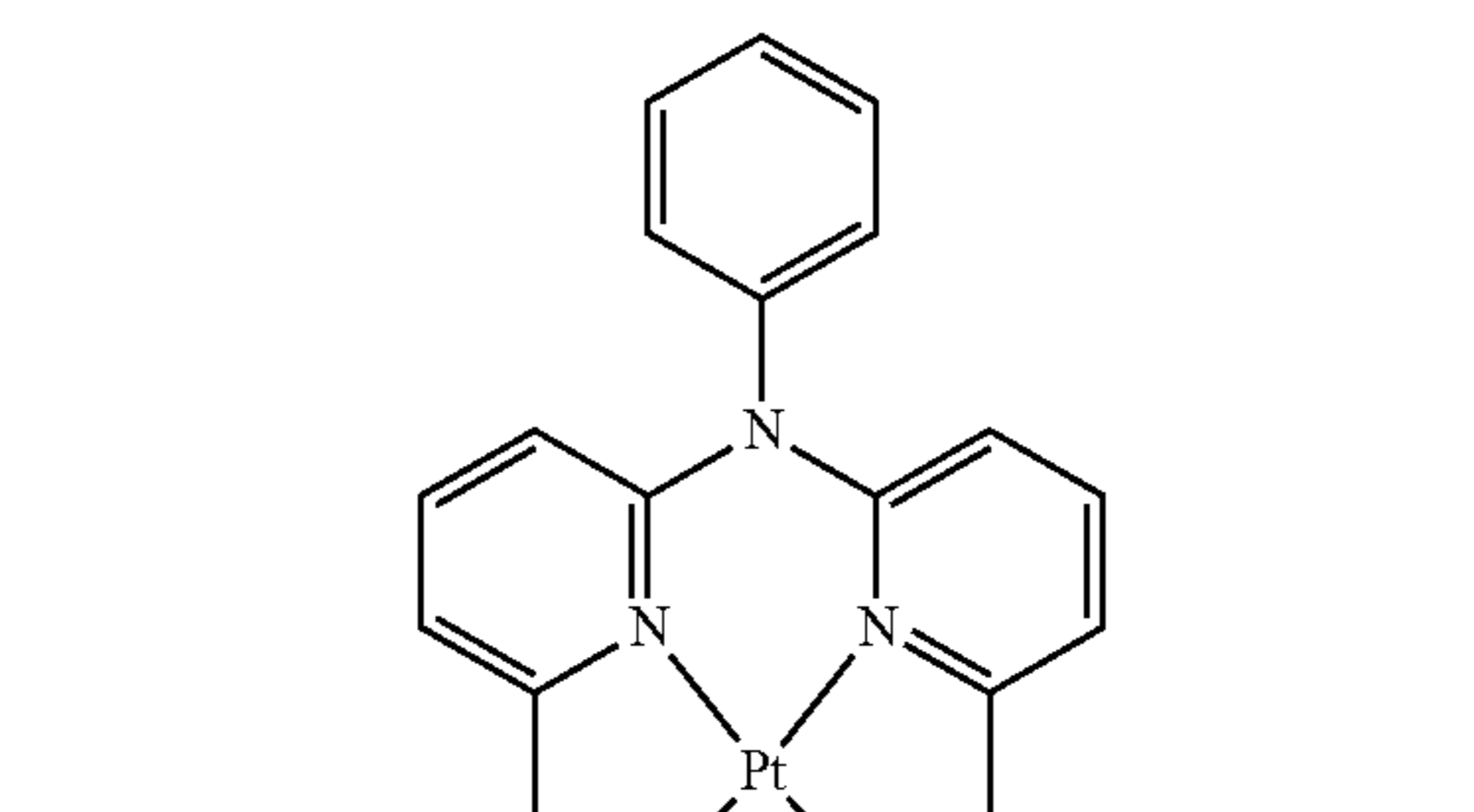
Compound 13
