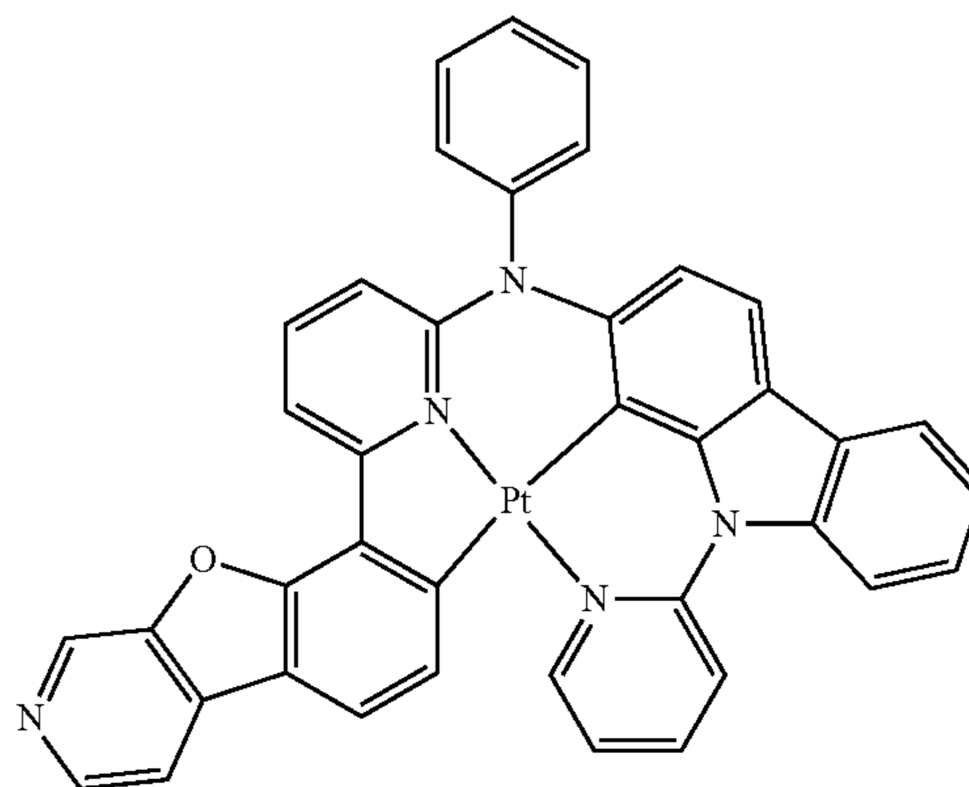
Compound 172
