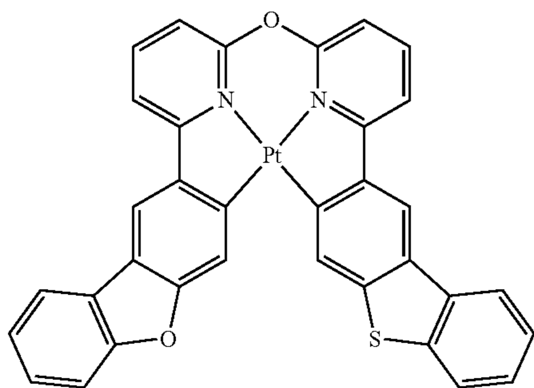
Compound 148
