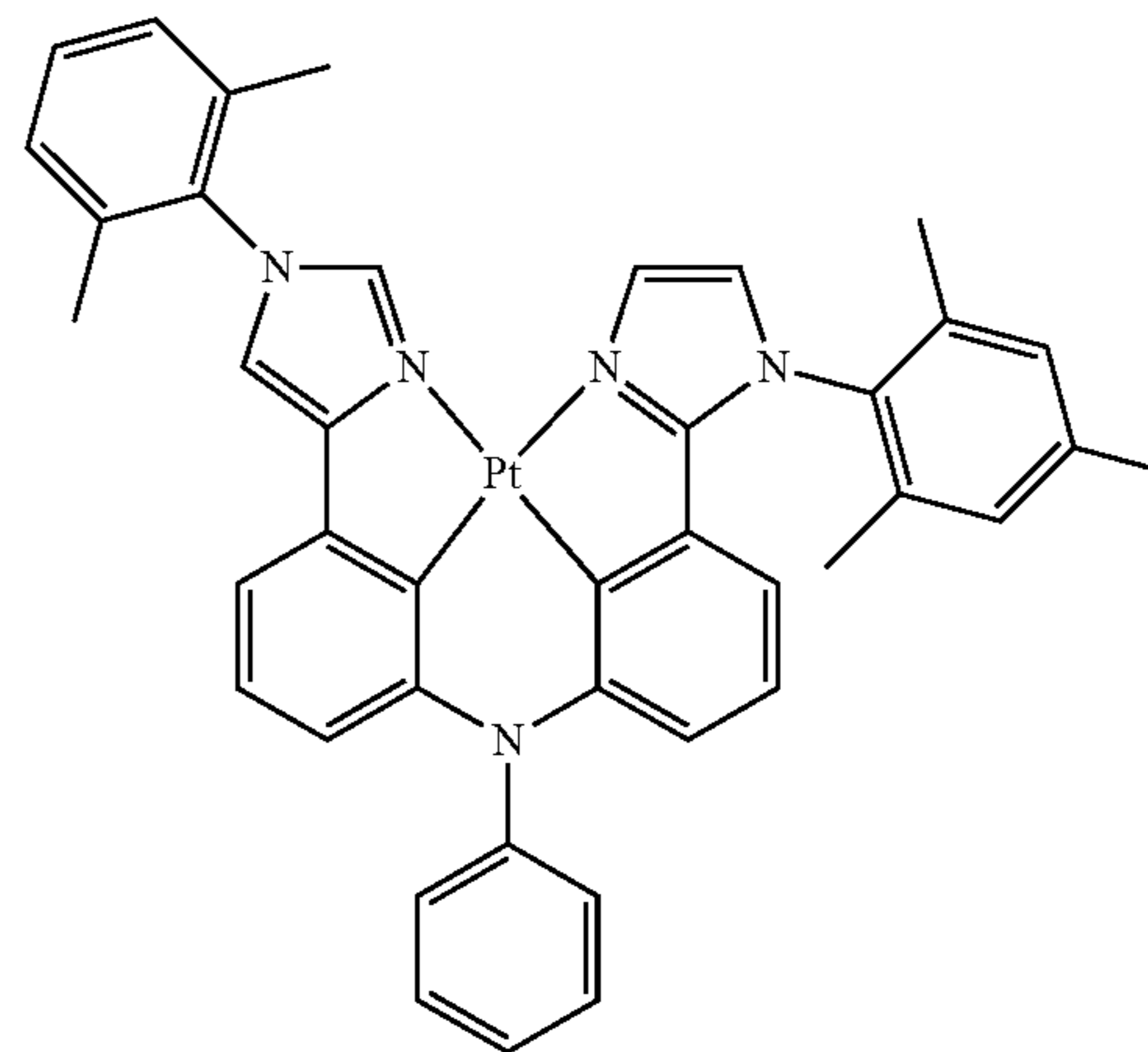
Compound 40'
