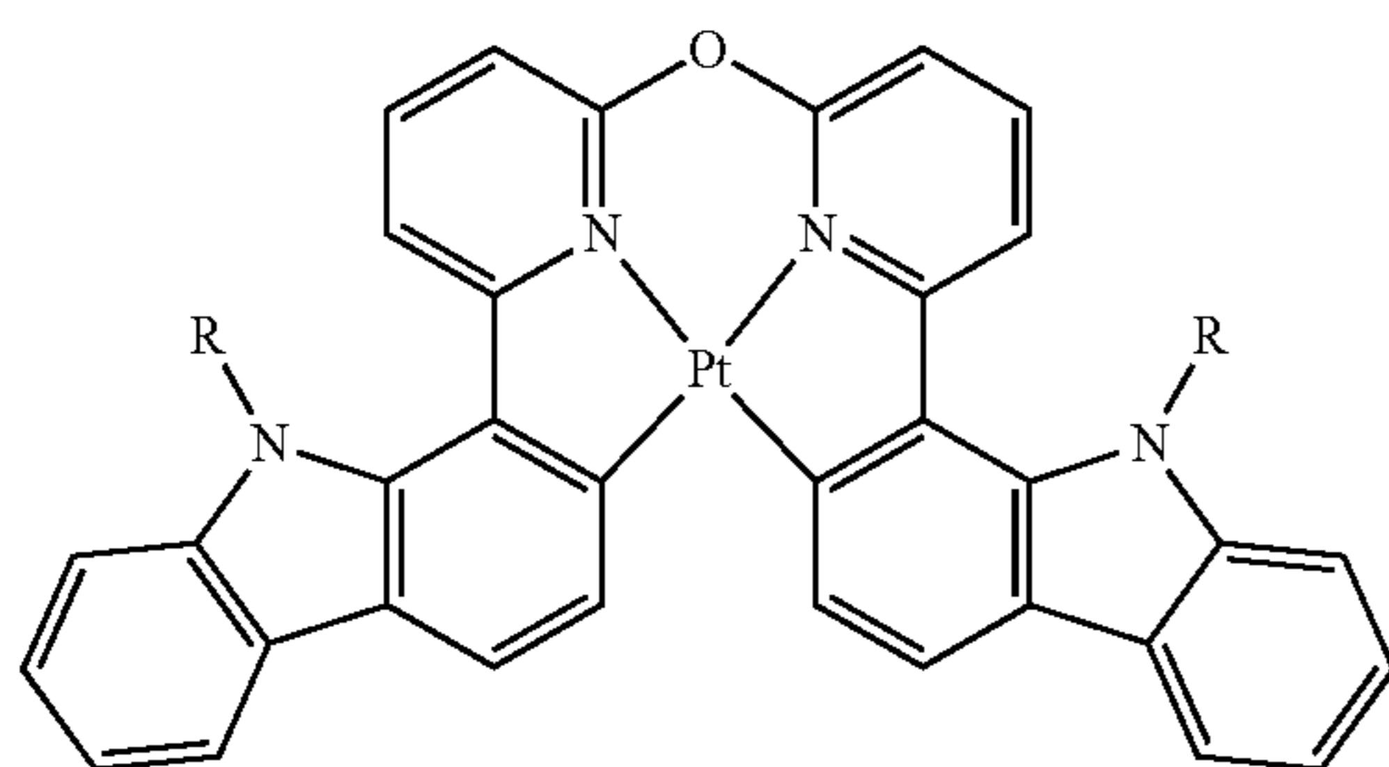
Compound 9
