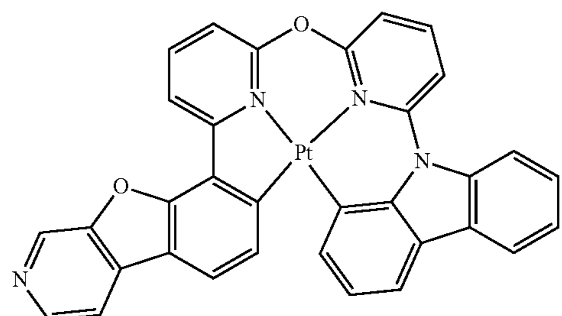
Compound 163
