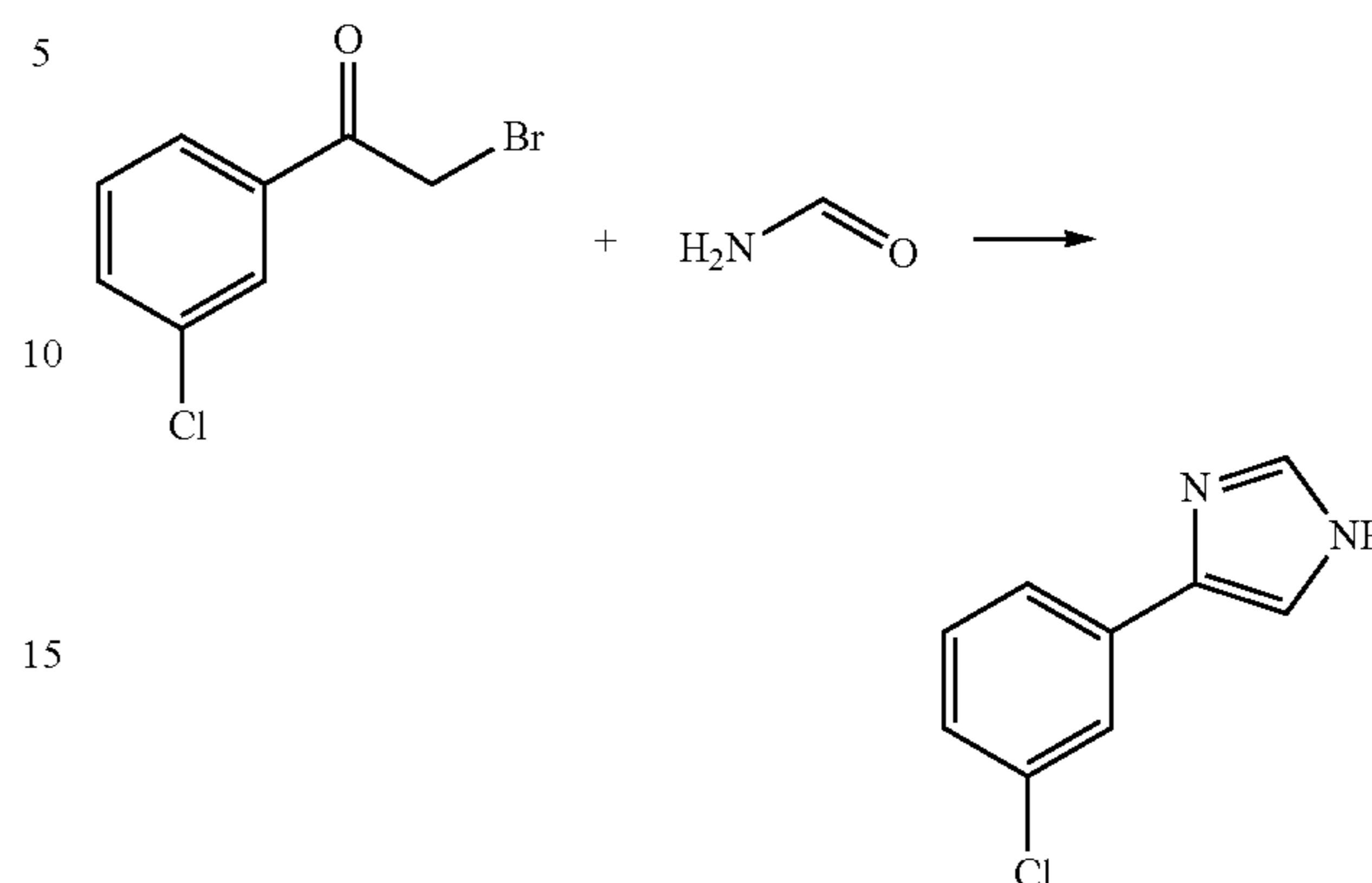
Synthesis of 4-(3-chlorophenyl)-1H-imidazole
