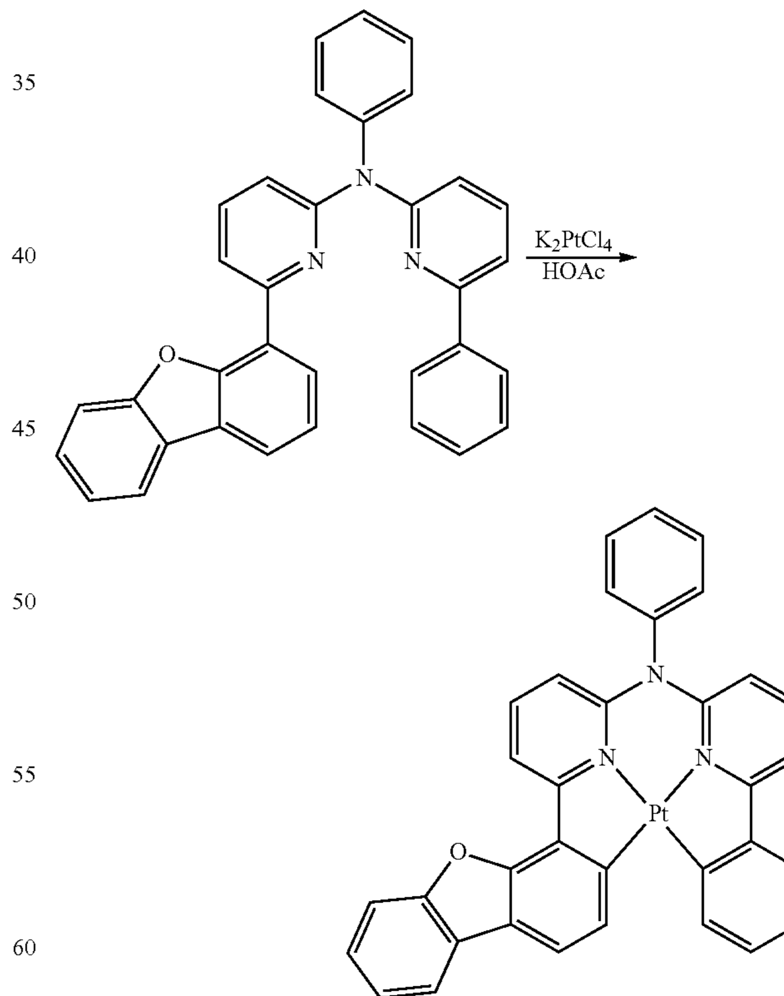
Synthesis of Compound 4
