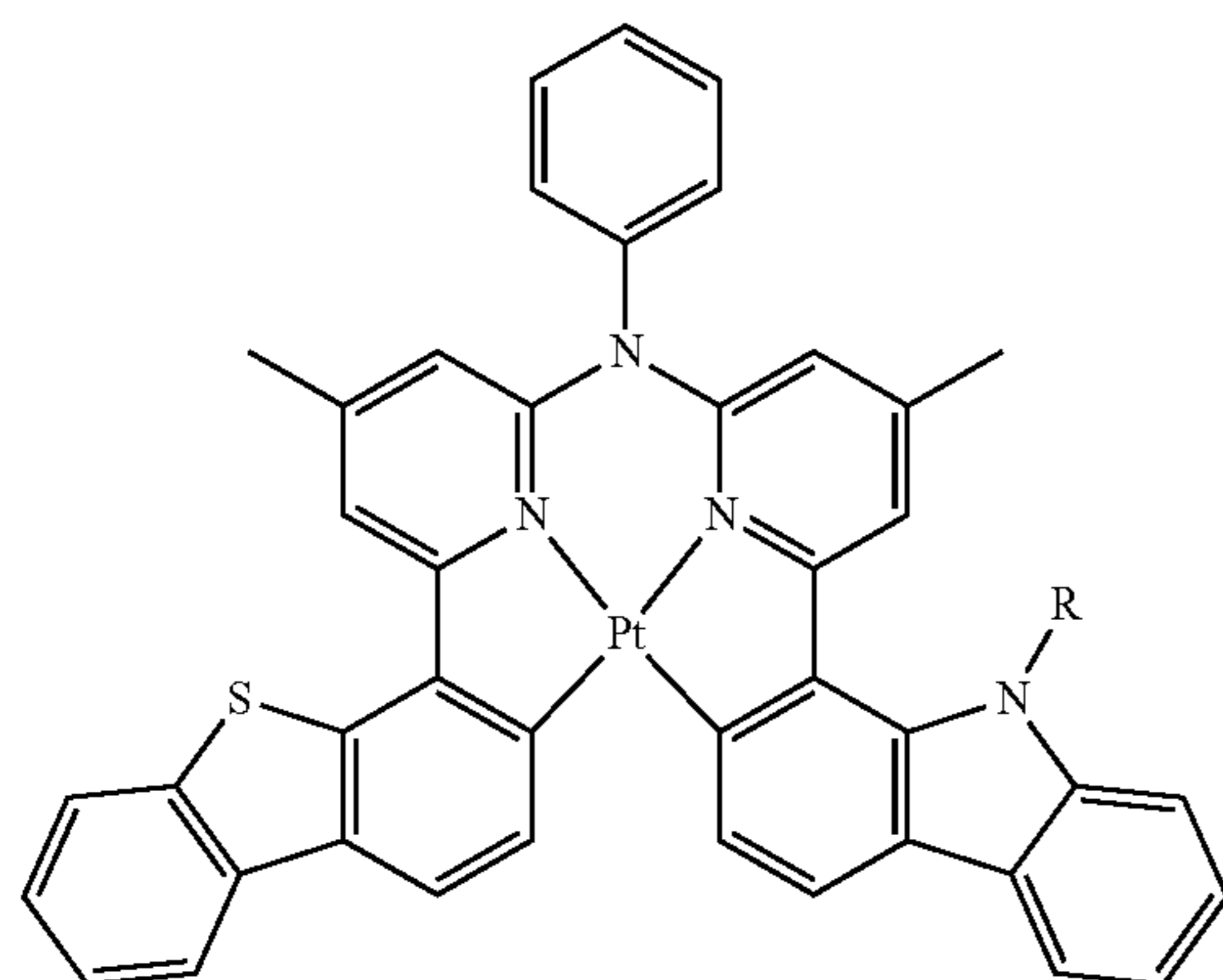
Compound 98
