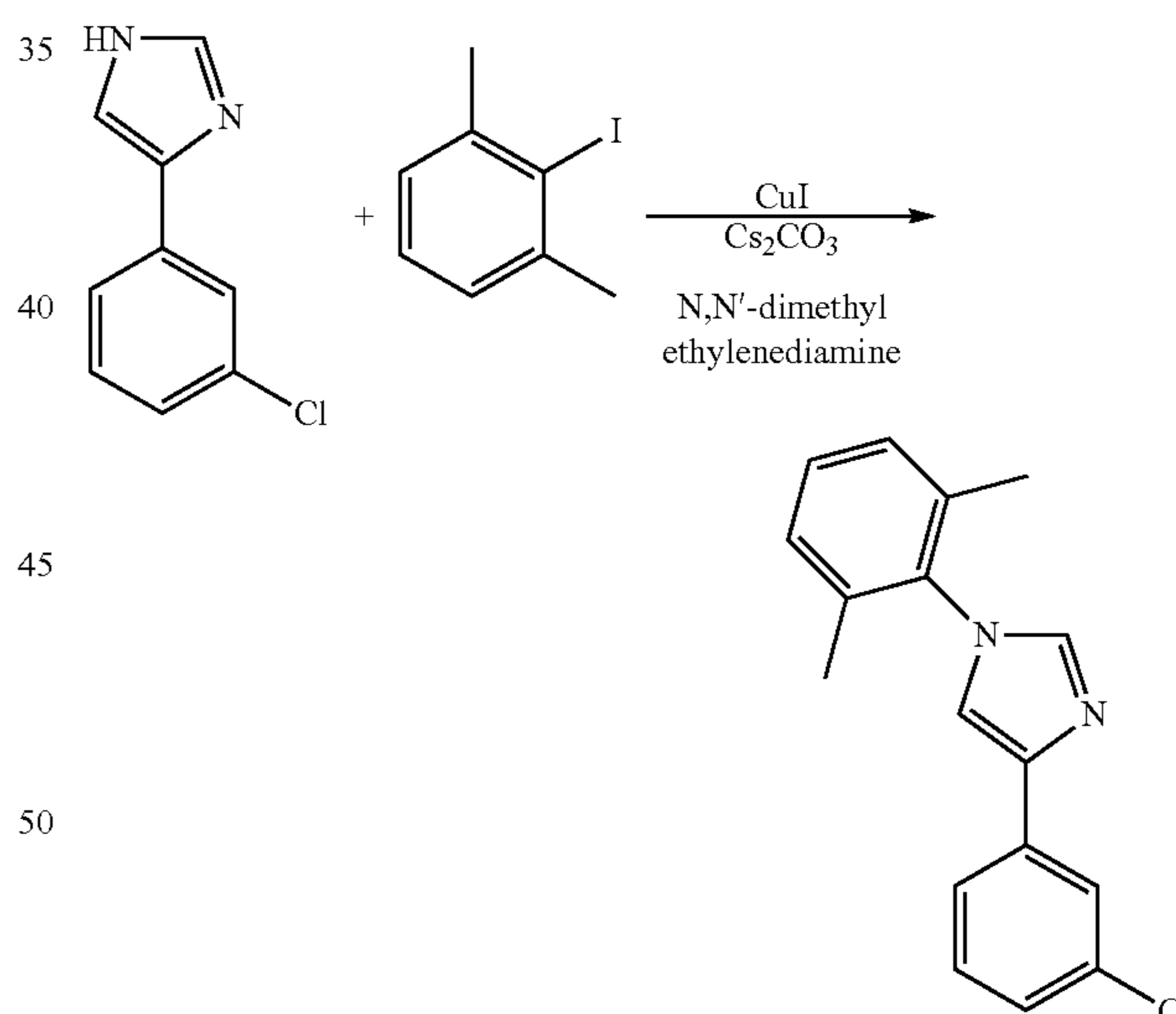
Synthesis of 4-(3-chlorophenyl)-1-(2,6-dimethylphenyl)-1H-imidazole
