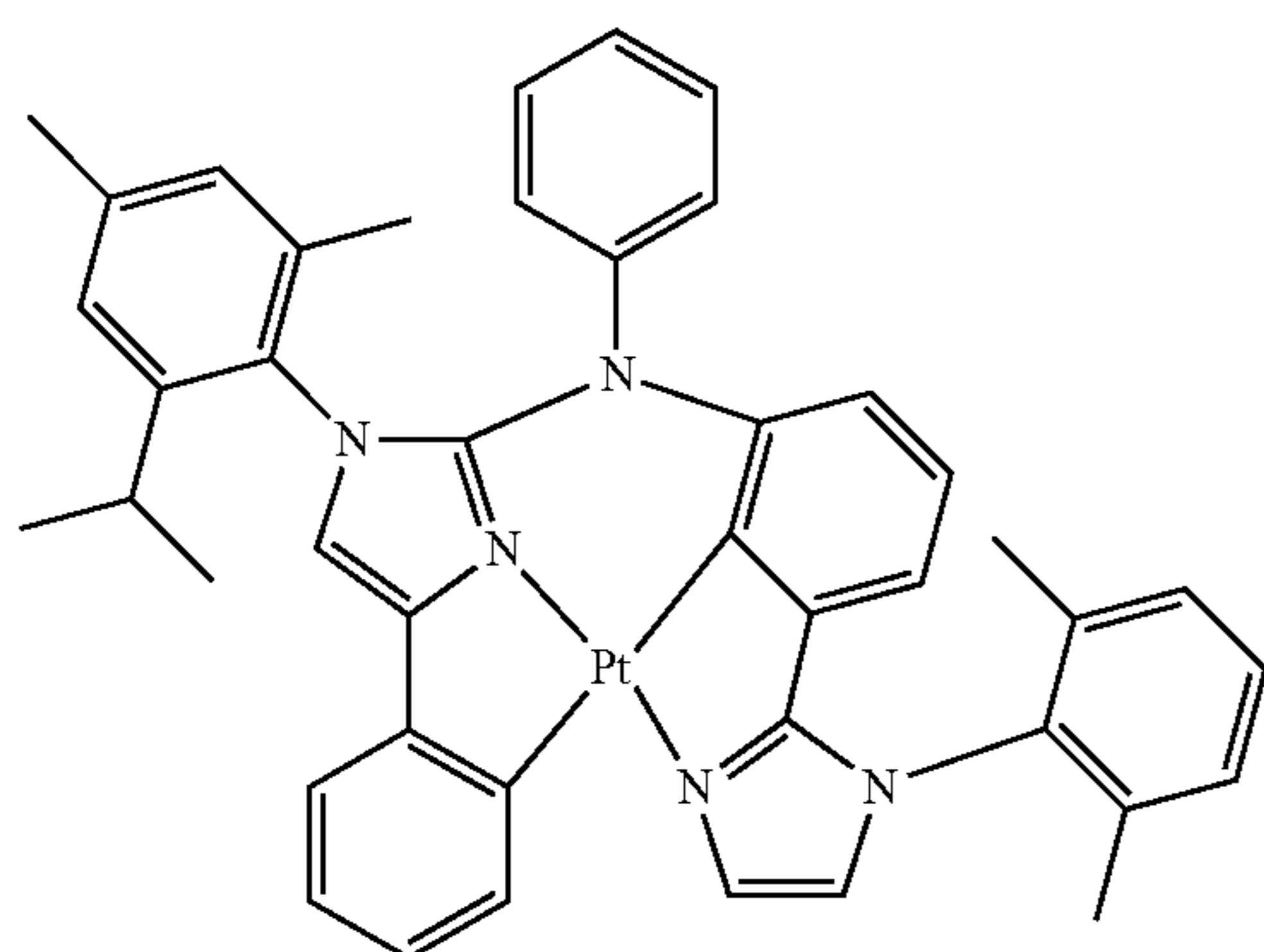
Compound 62'
