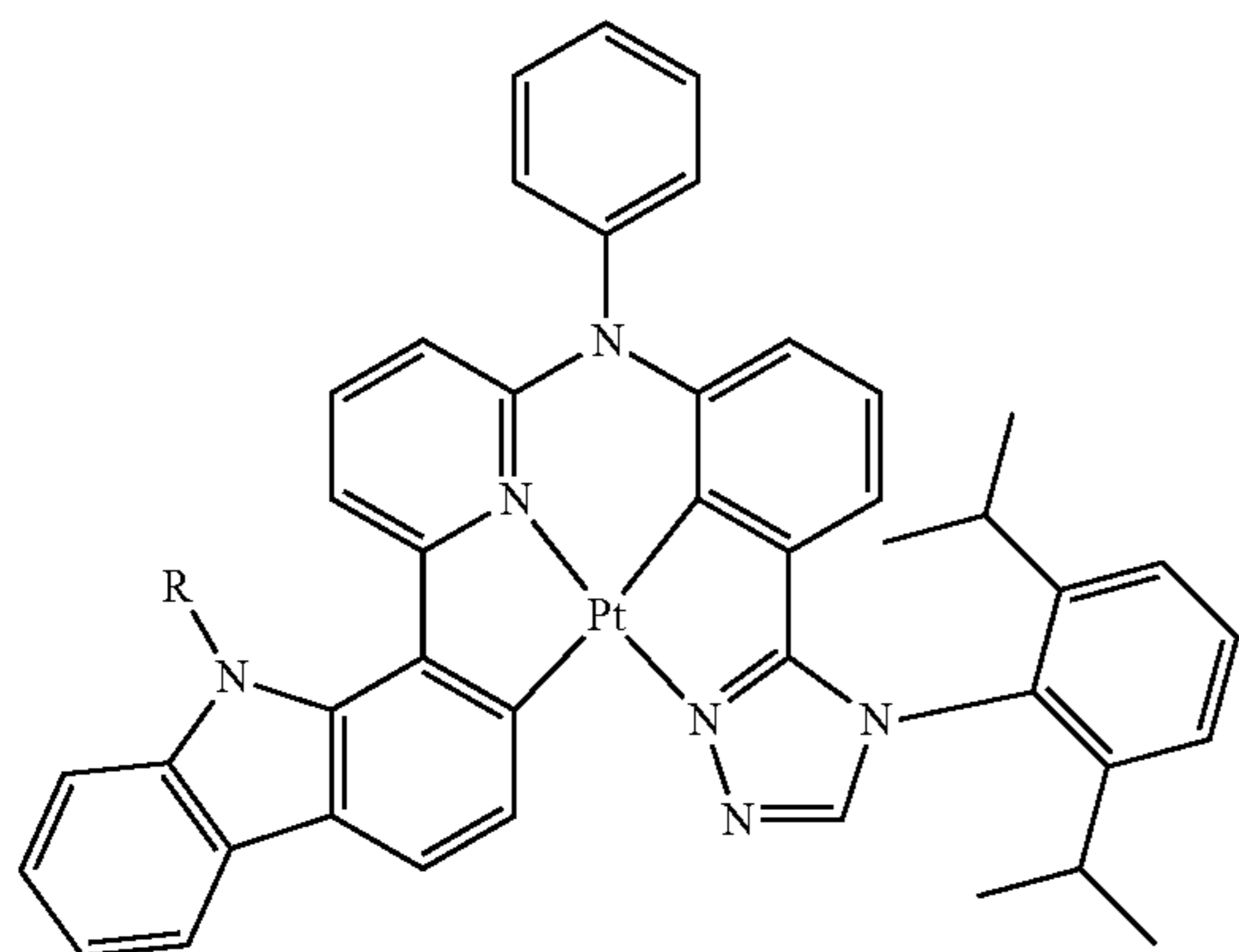
Compound 42
