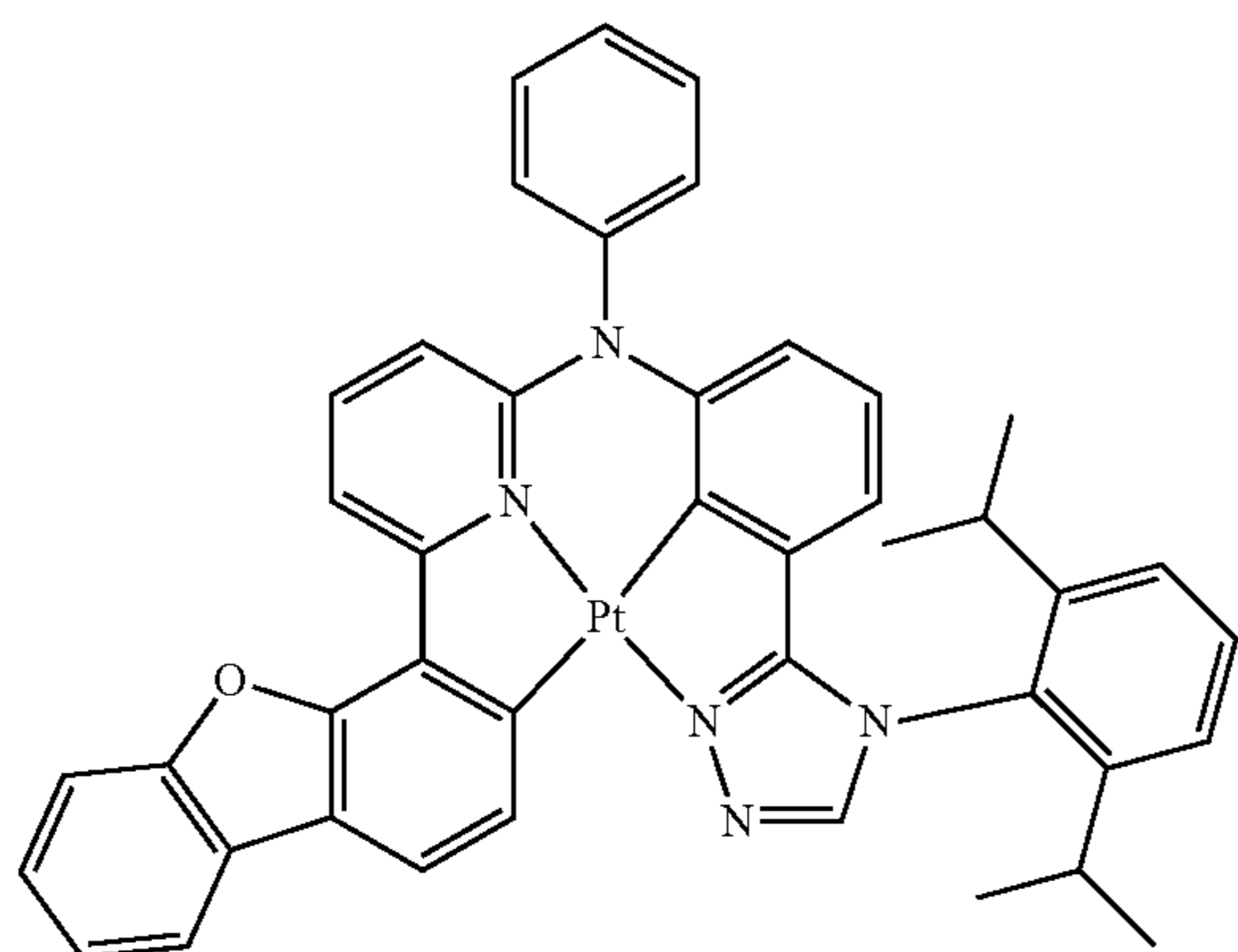
Compound 41
