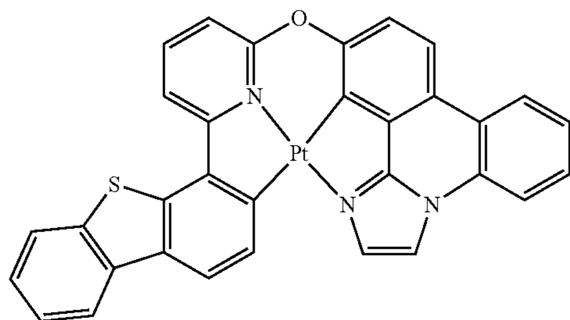
Compound 50
