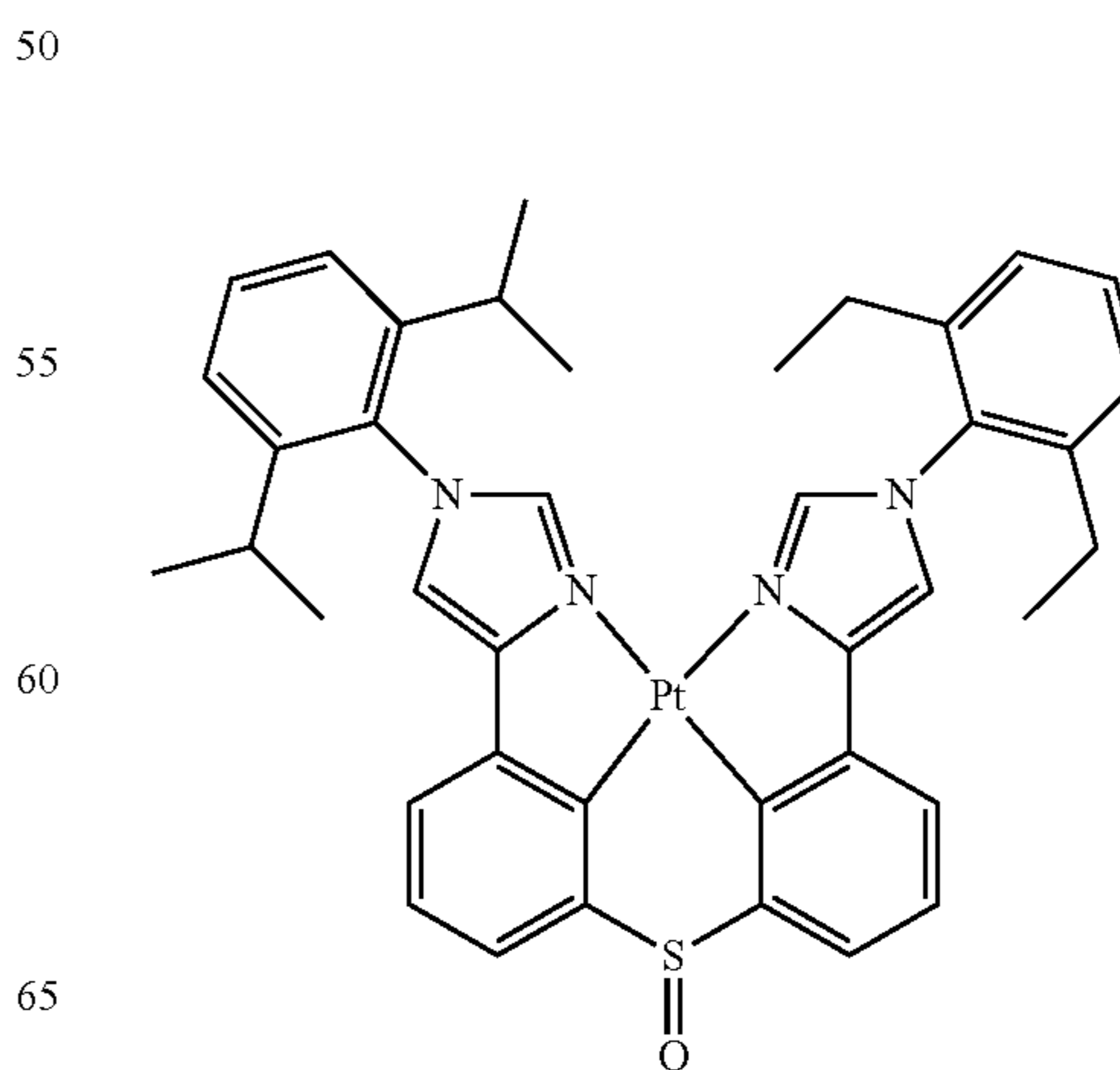
Compound 13'
