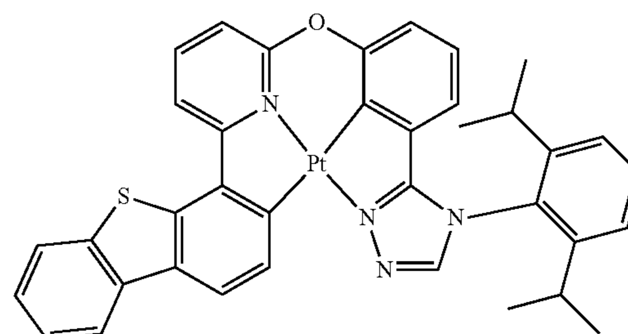
Compound 38
