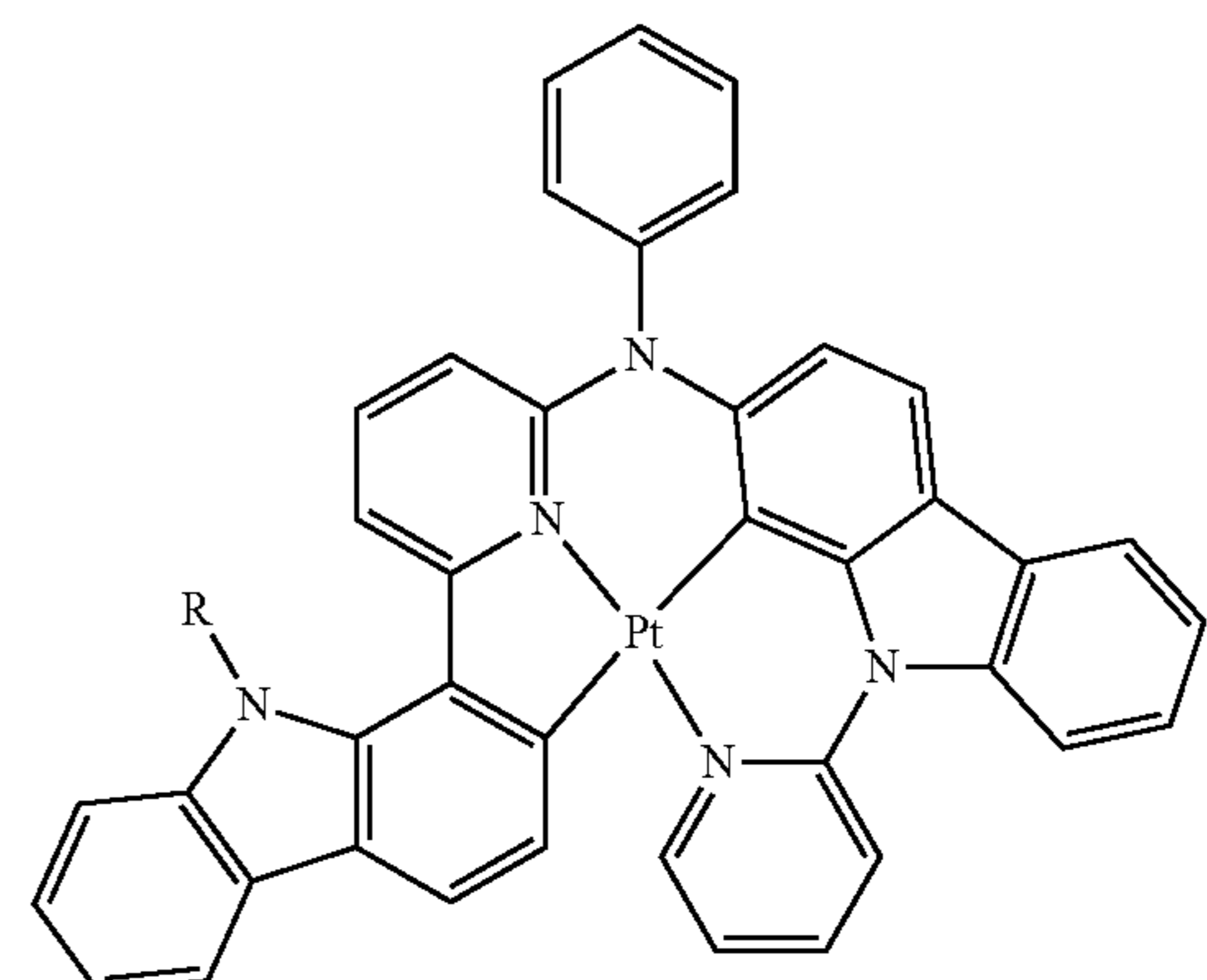
Compound 78
