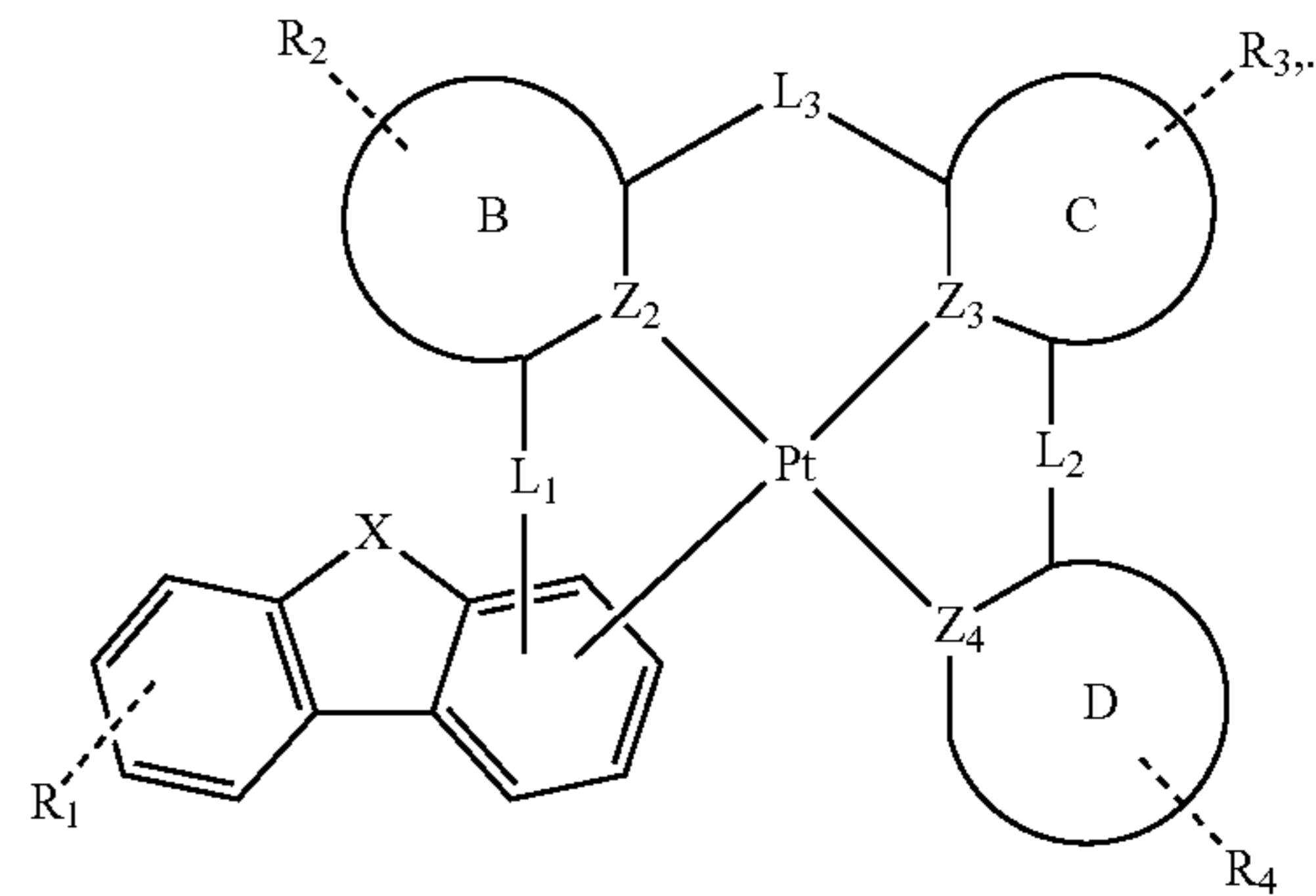
Formula II
