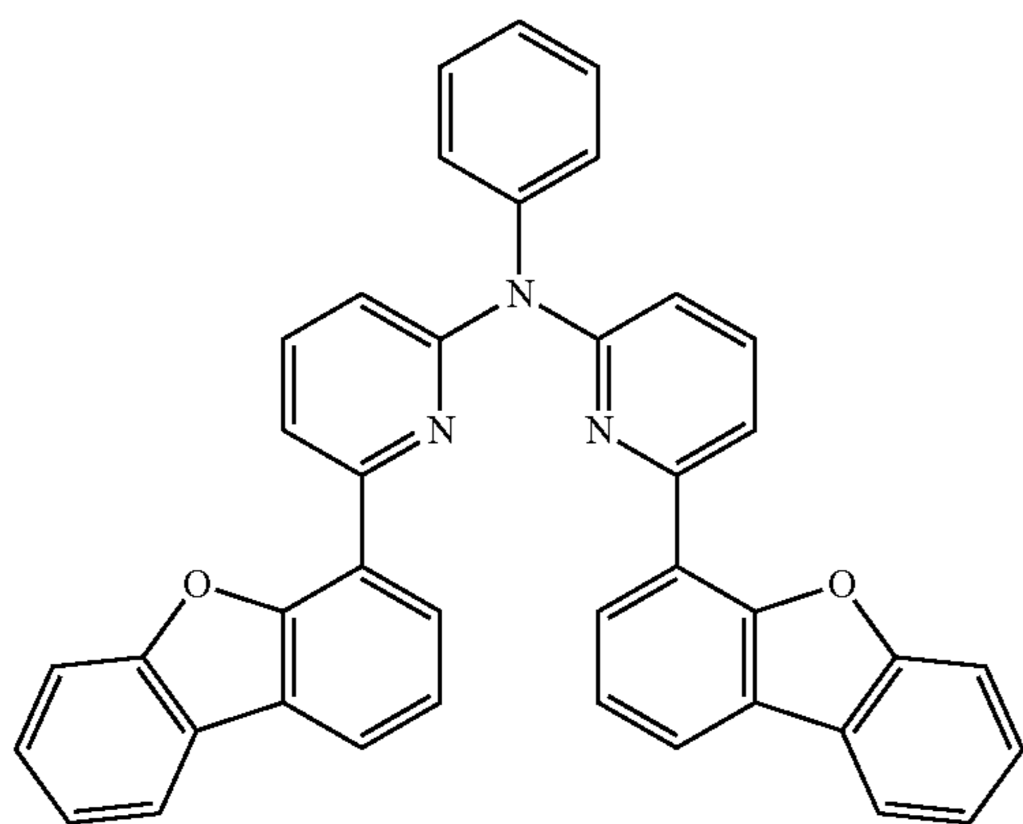
Synthesis of 6-(dibenzo[b,d]furan-4-yl)-N-(6-(dibenzo[b,d]furan-4-yl)pyridin-2-yl)-N-phenylpyridin-2-amine
