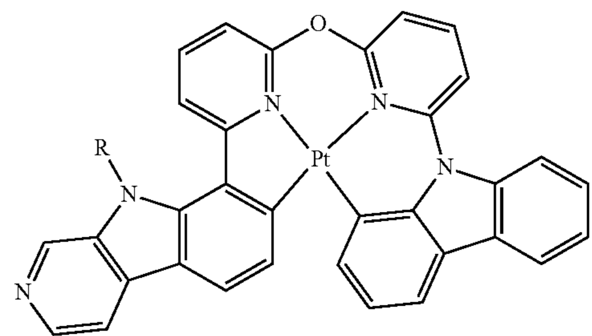
Compound 166
