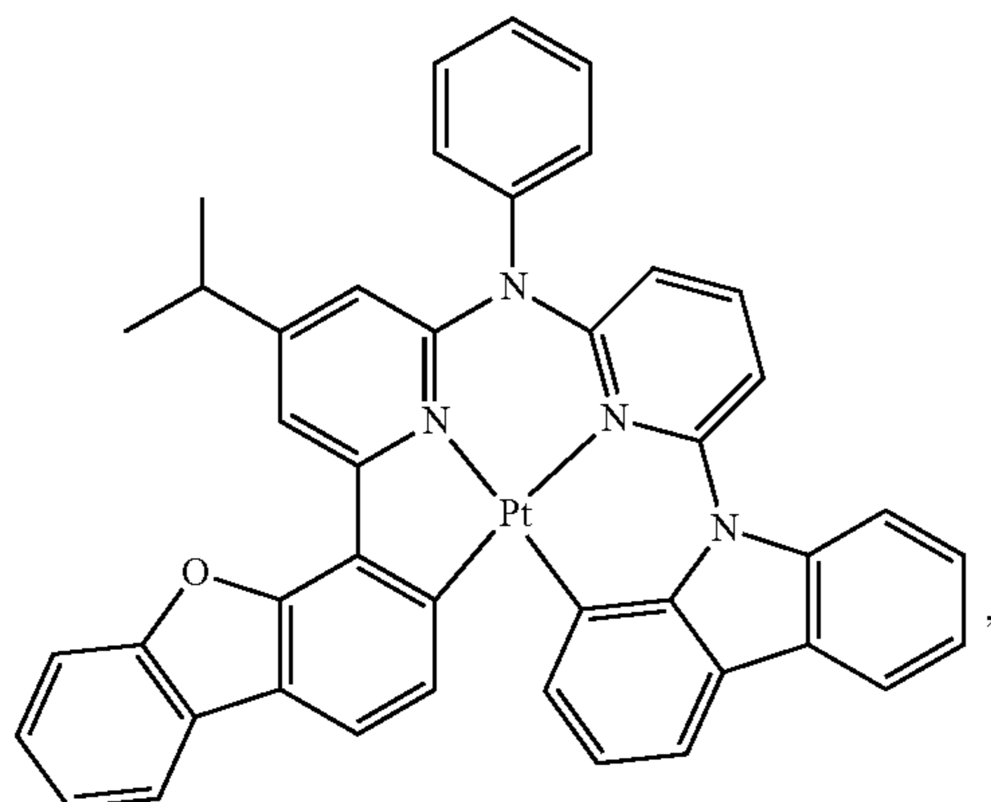
Compound 167
