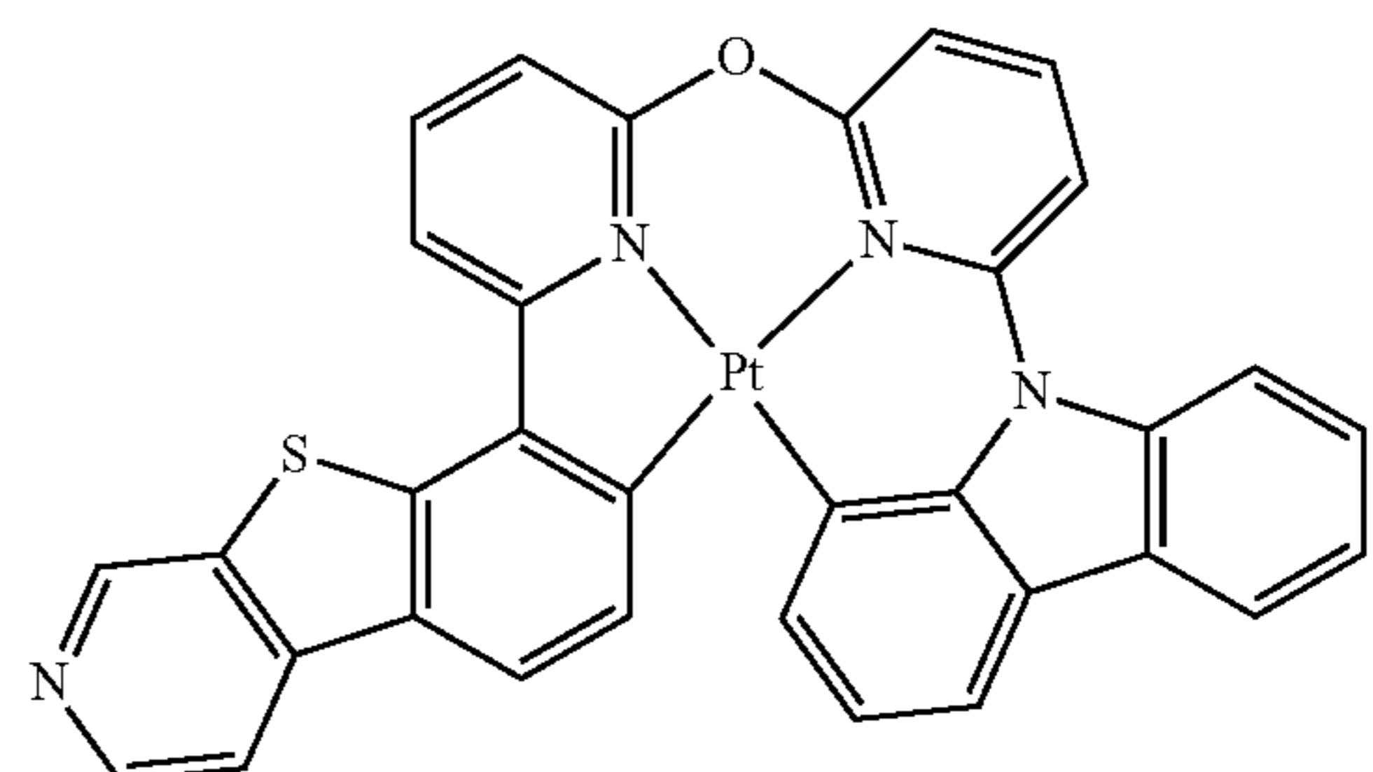
Compound 164
