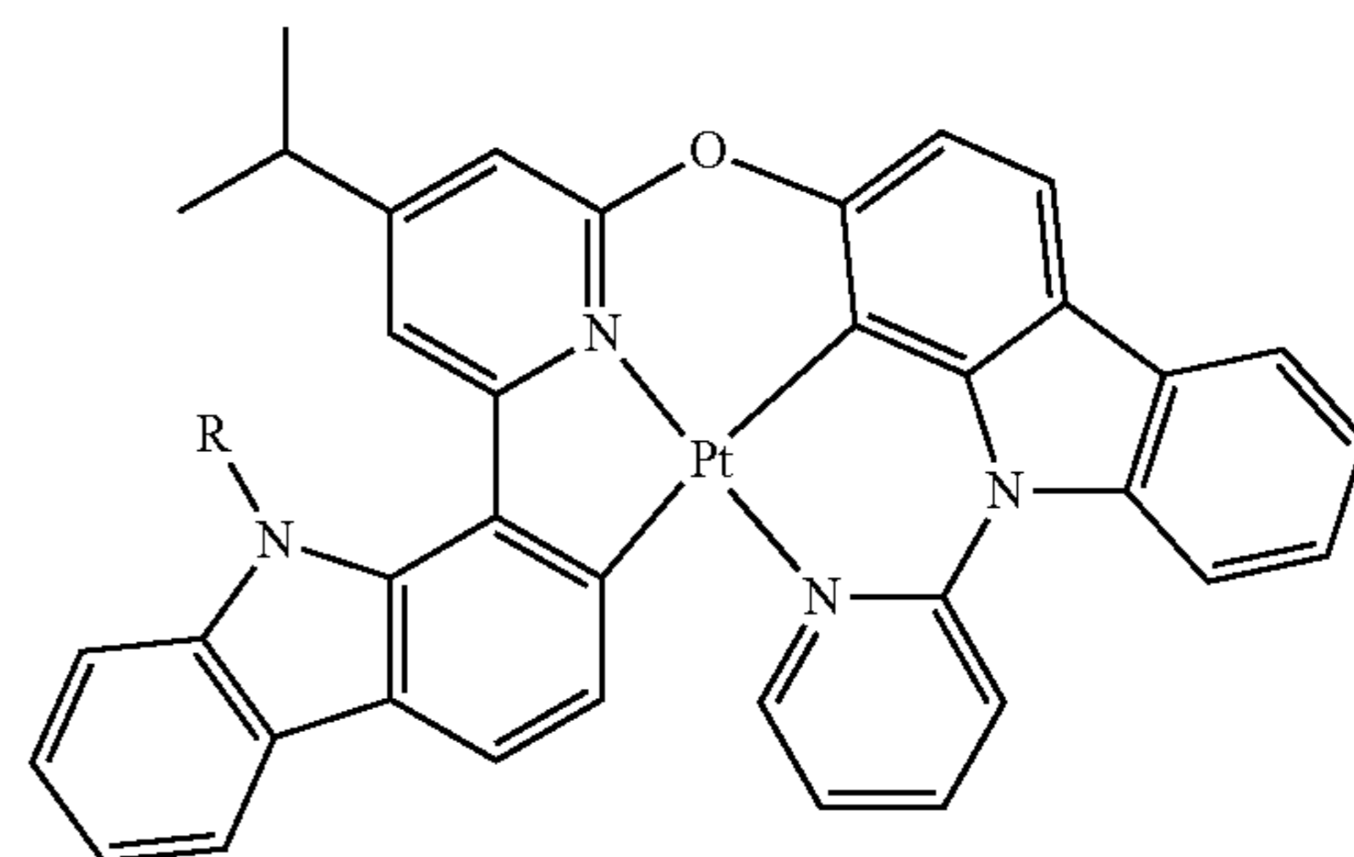
Compound 171
