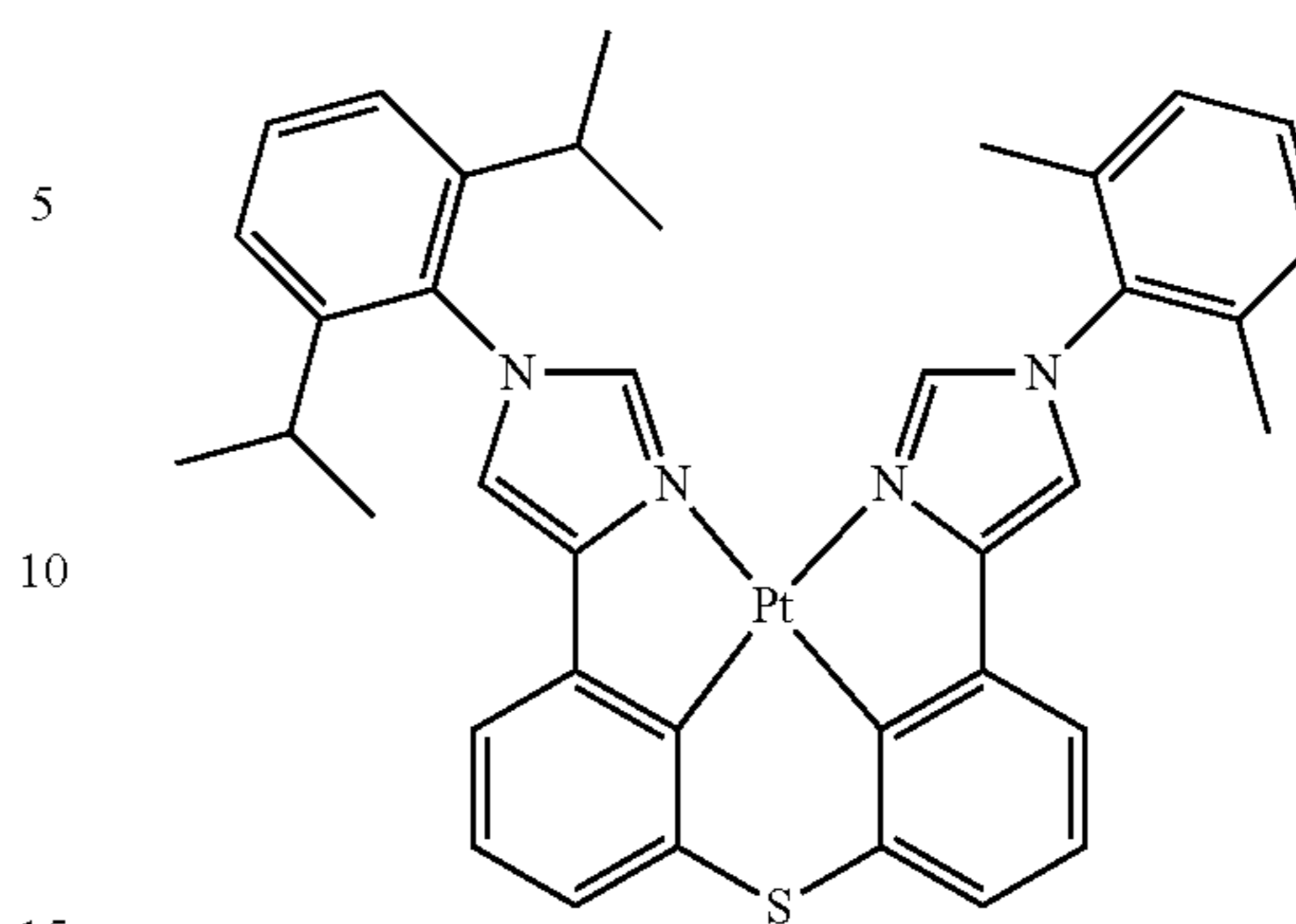
Compound 7'
