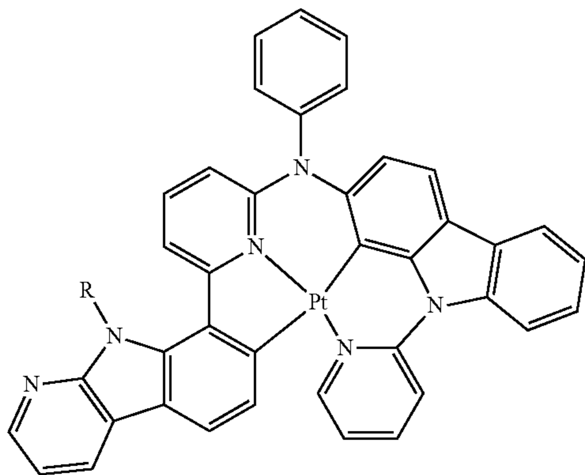
Compound 174
