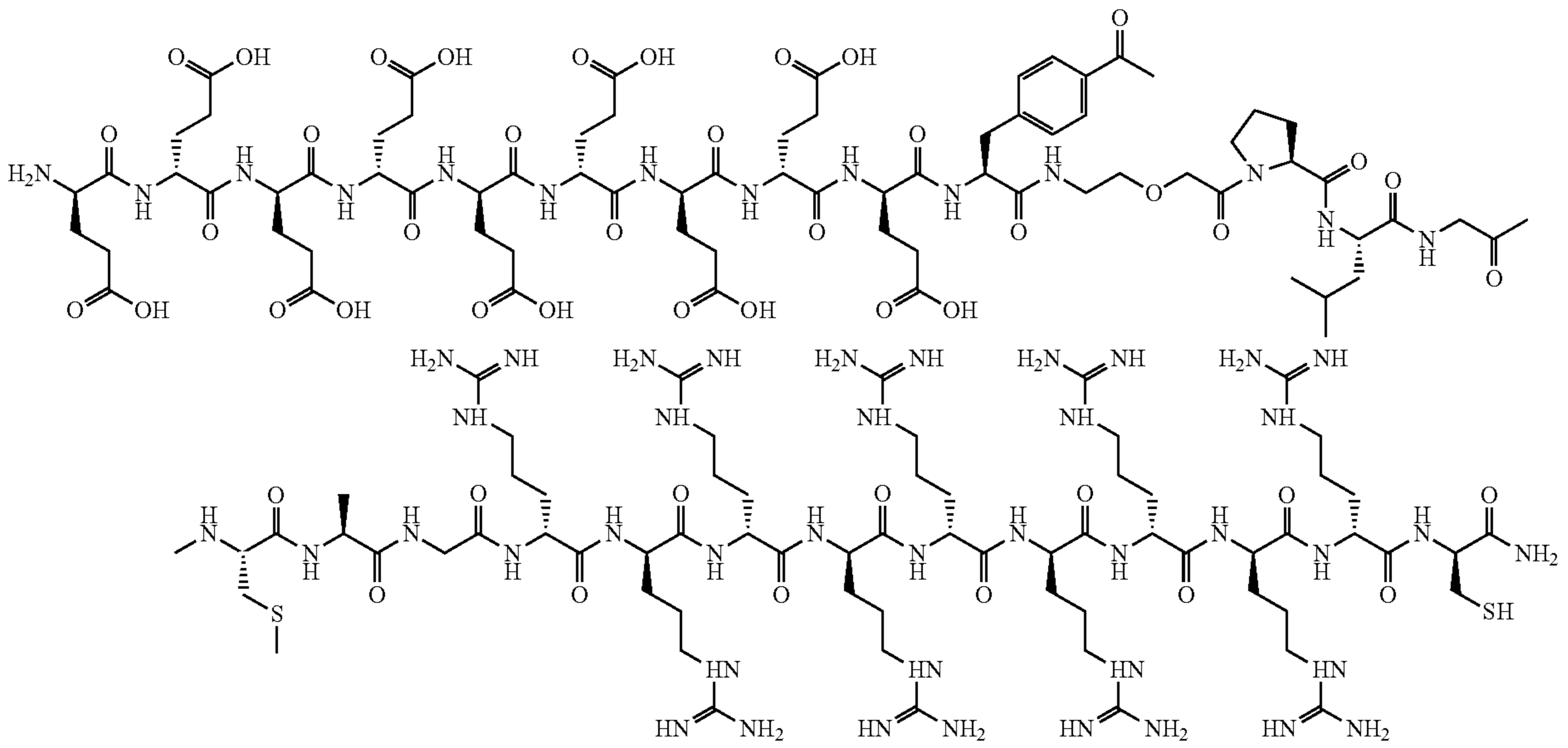
Peptide P-4
