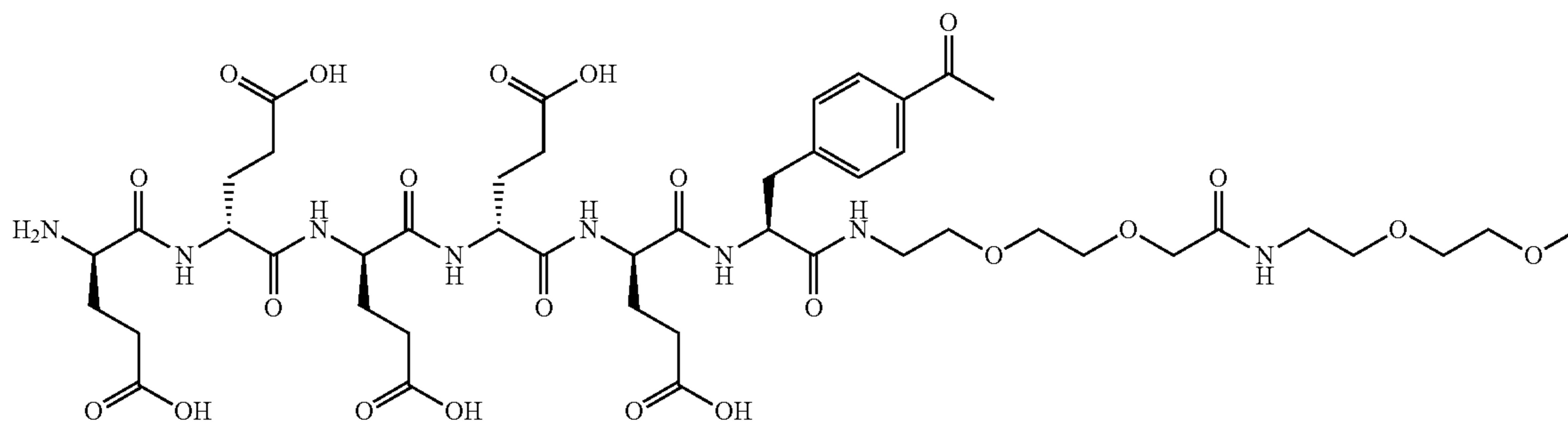
Peptide P-11
