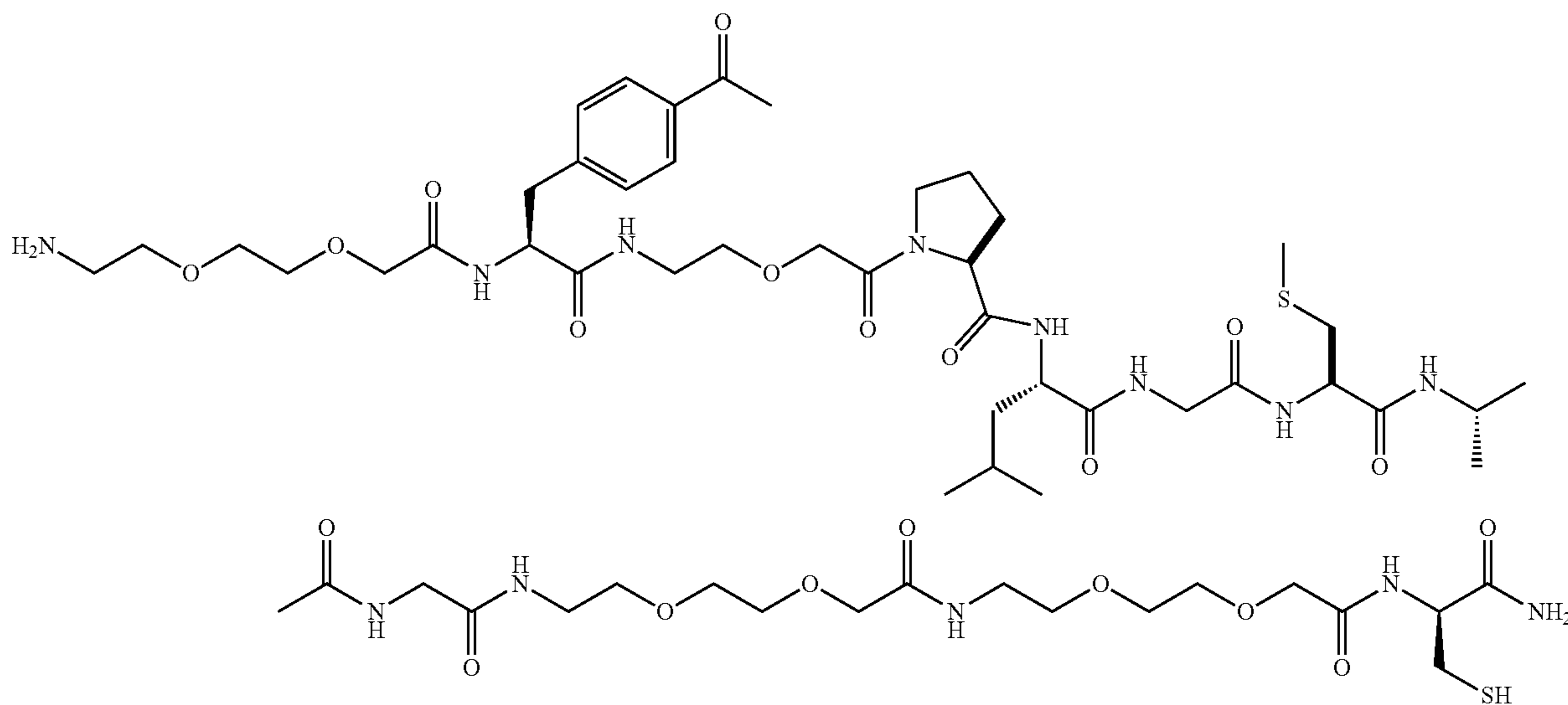
Peptide P-11
