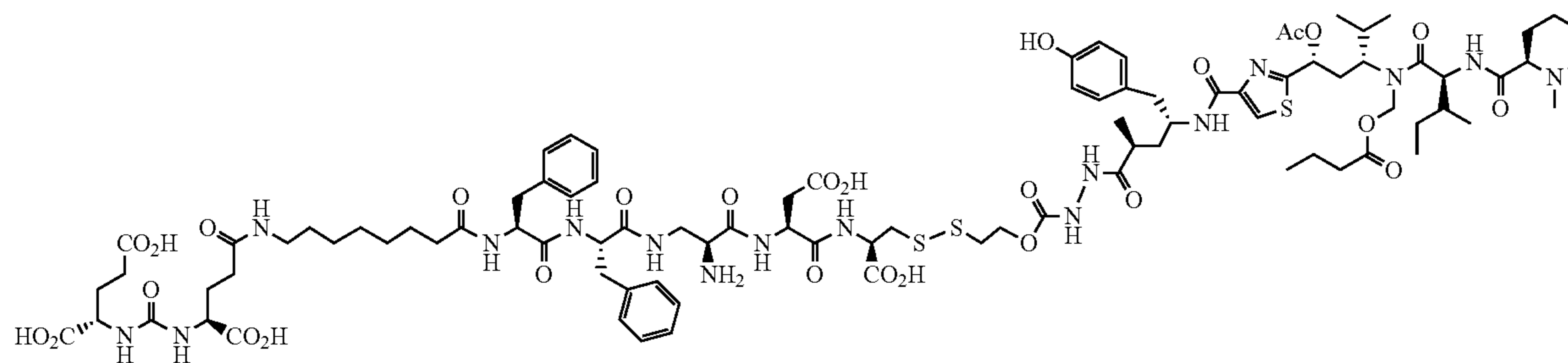
EC1437 C_{92}H_{132}N_{16}O_{28}S_3 Exact Mass: 2004.86 Mol. Wt.: 2006.32
