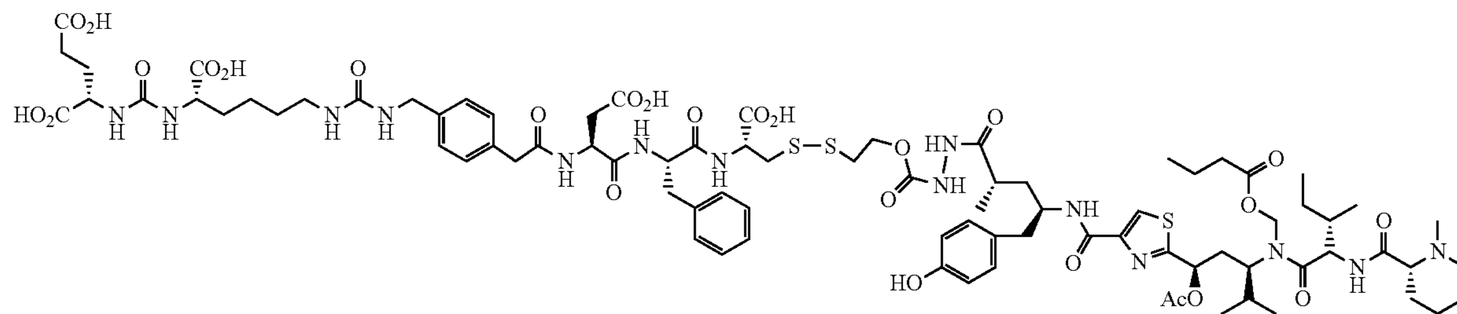
EC1386 C_{83}H_{116}N_{14}O_{26}S_3 Exact Mass: 1820.74
