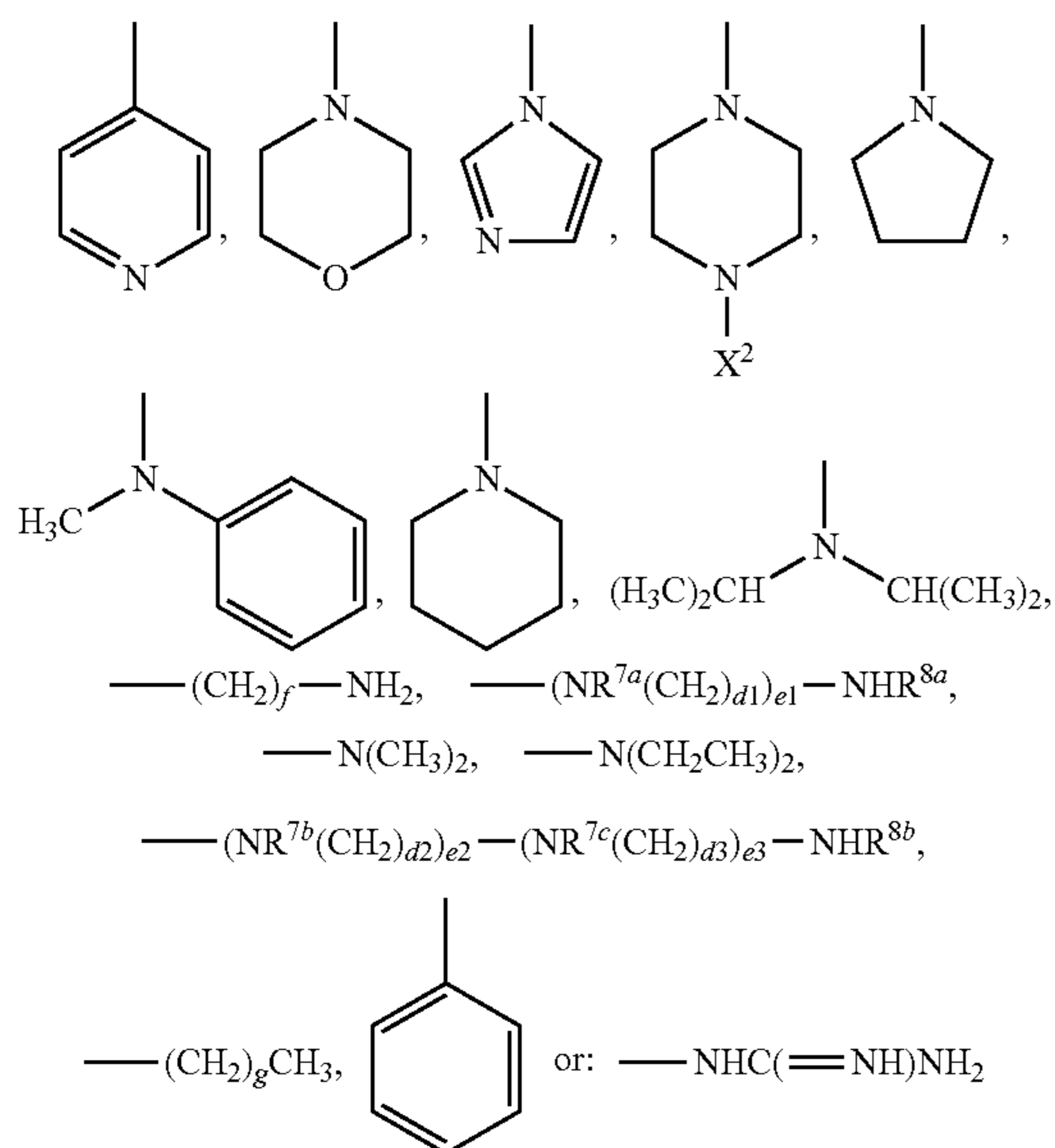
[Chemical Formula 4]
