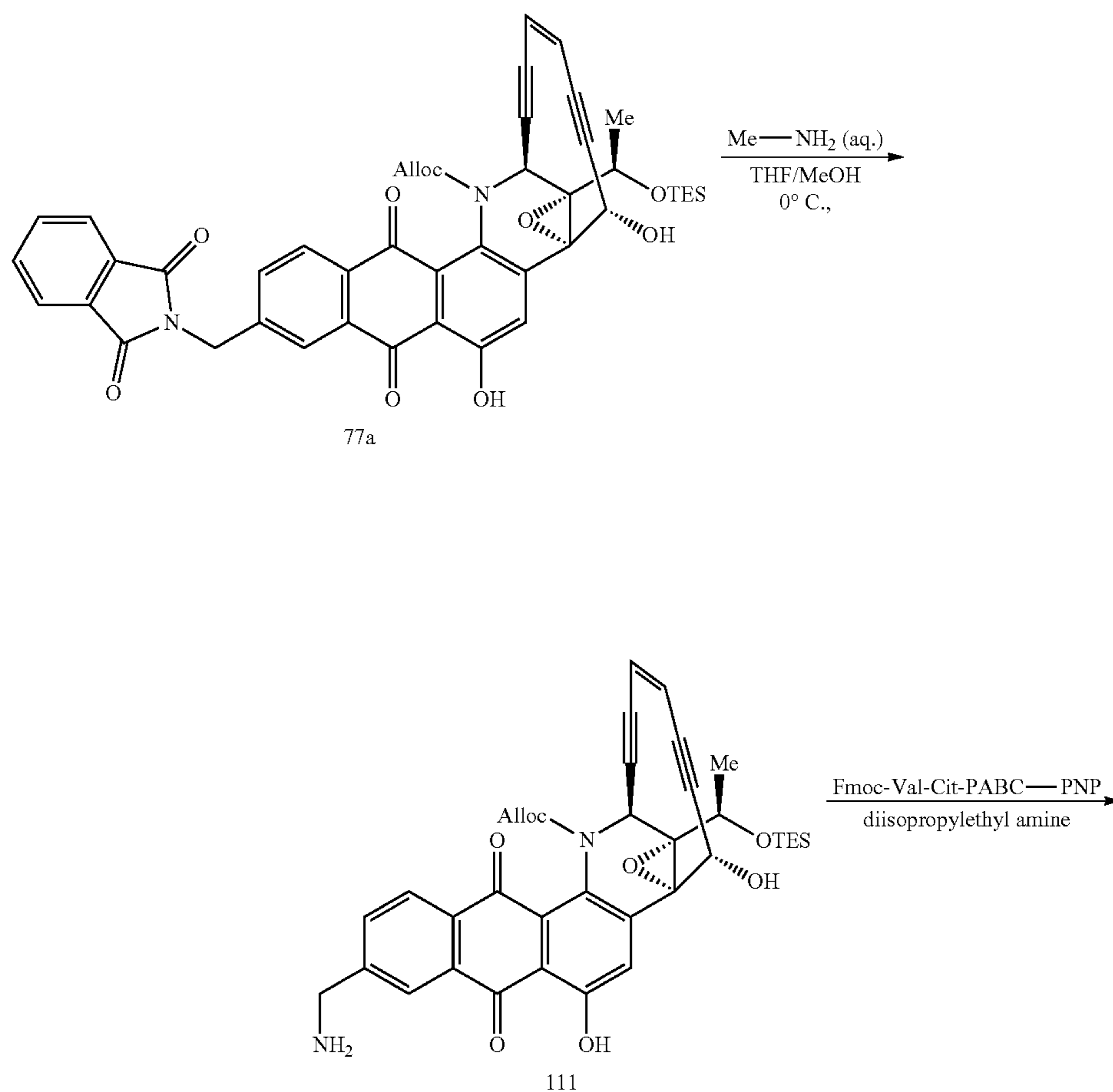
Scheme 22
