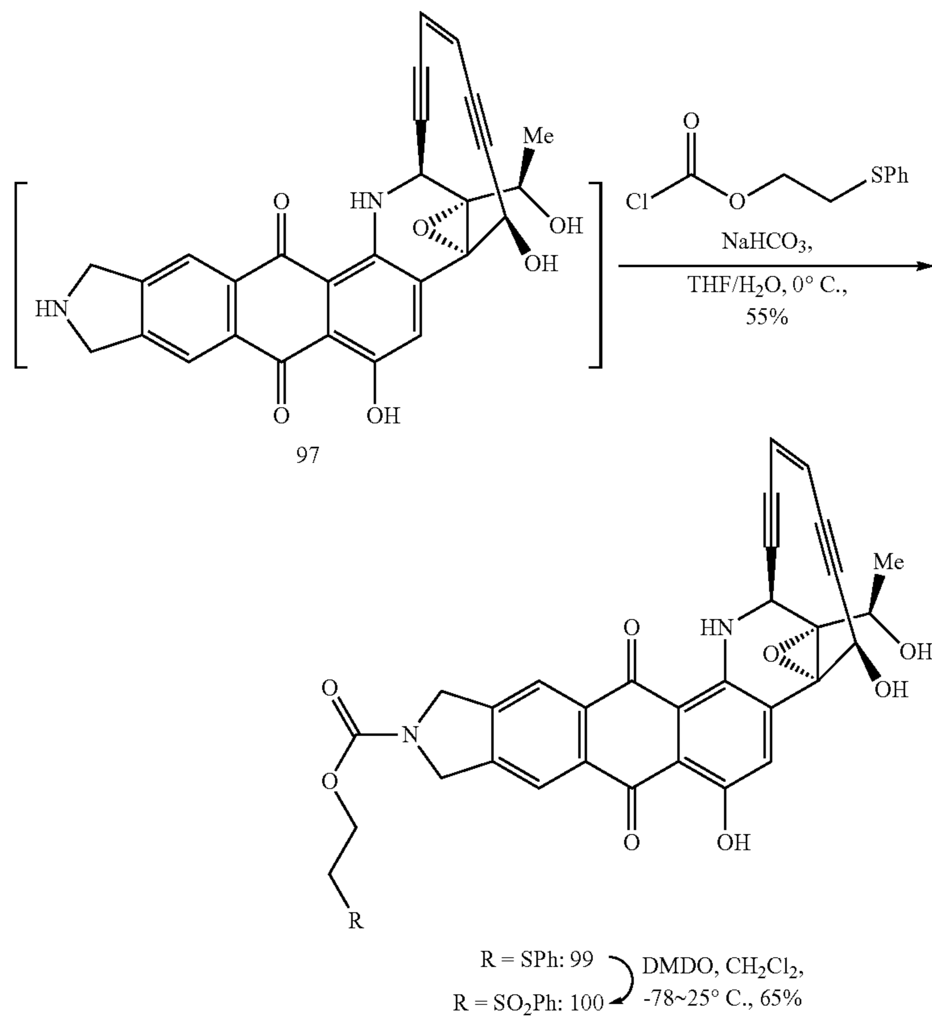
Scheme 19. Synthesis of sulfide 99 and sulfone 100.
