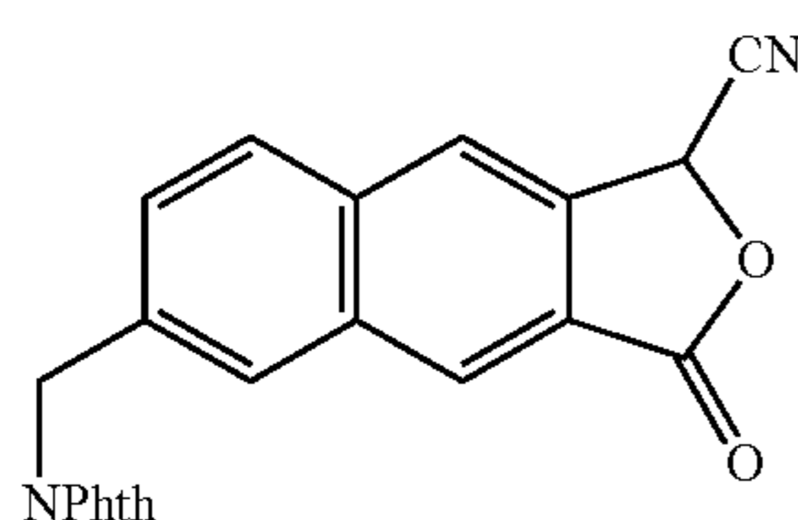
Cyanophthalide 76.
