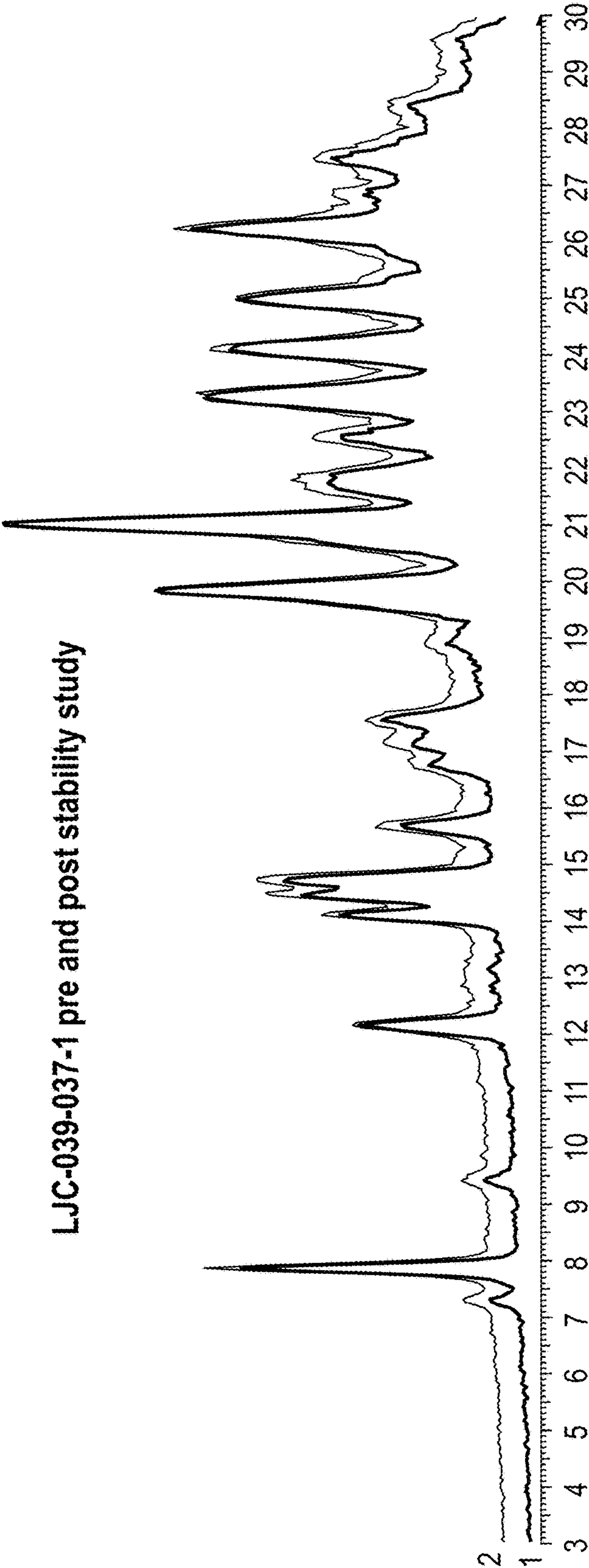
2-Theta - Scale
