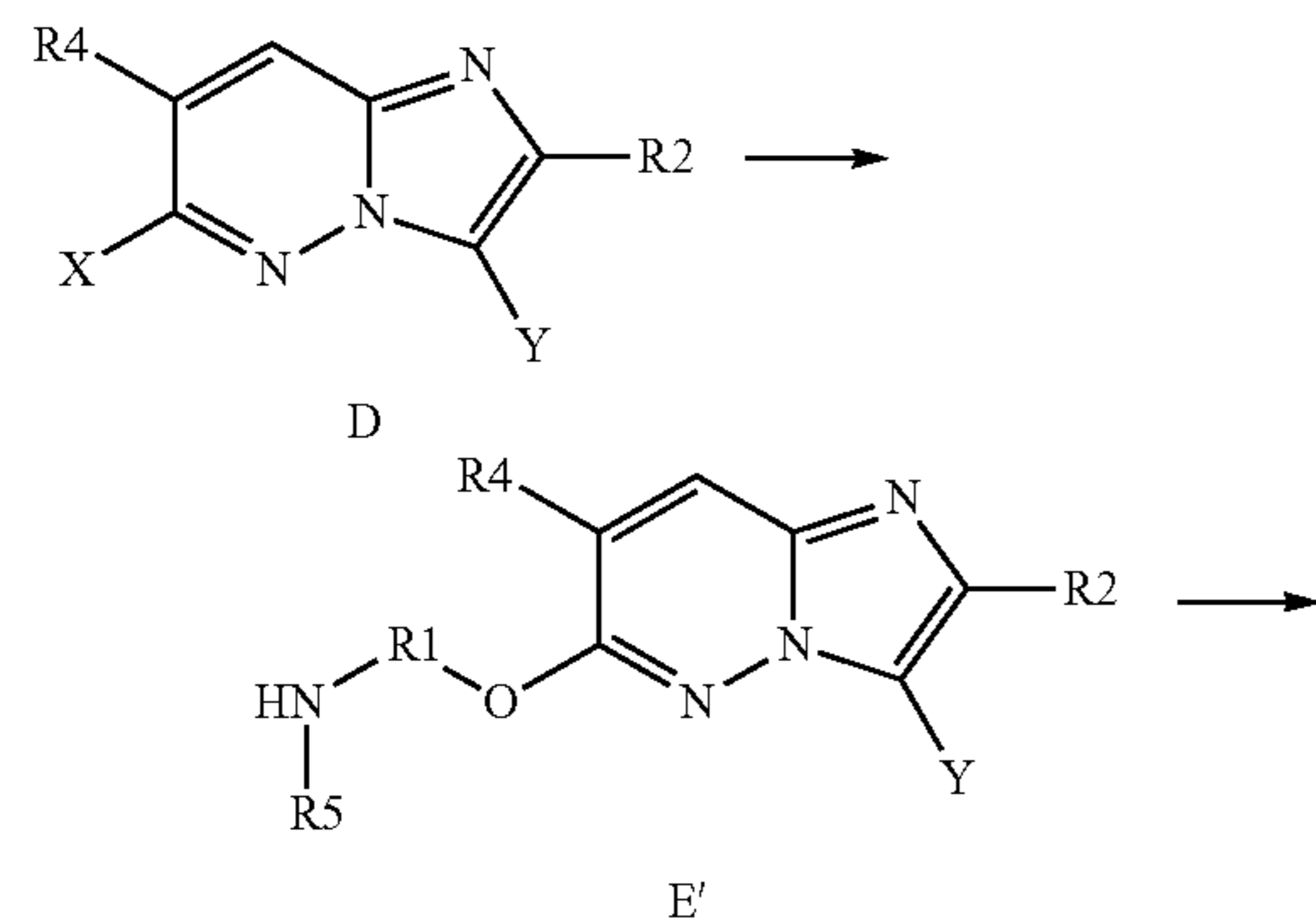
Scheme 2:
