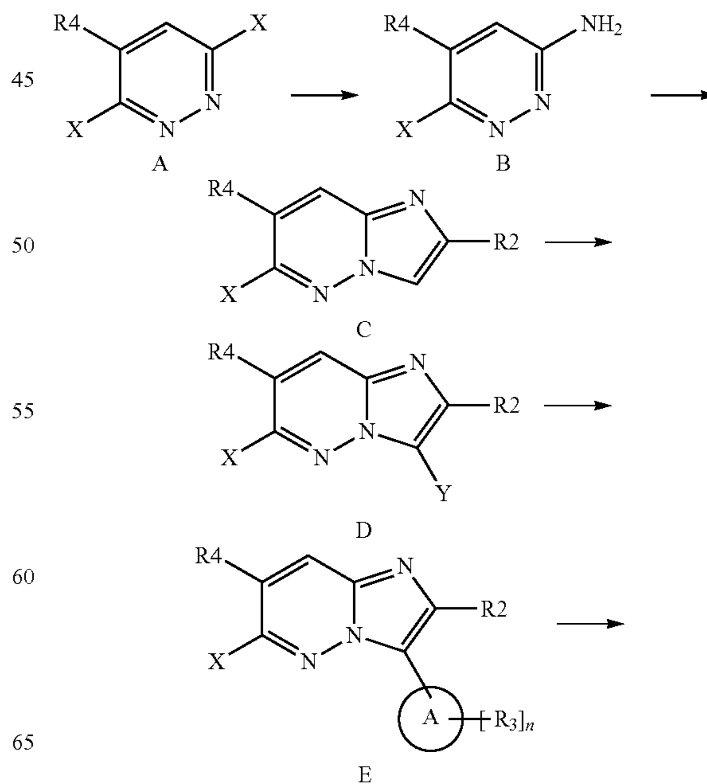
Scheme 1:
