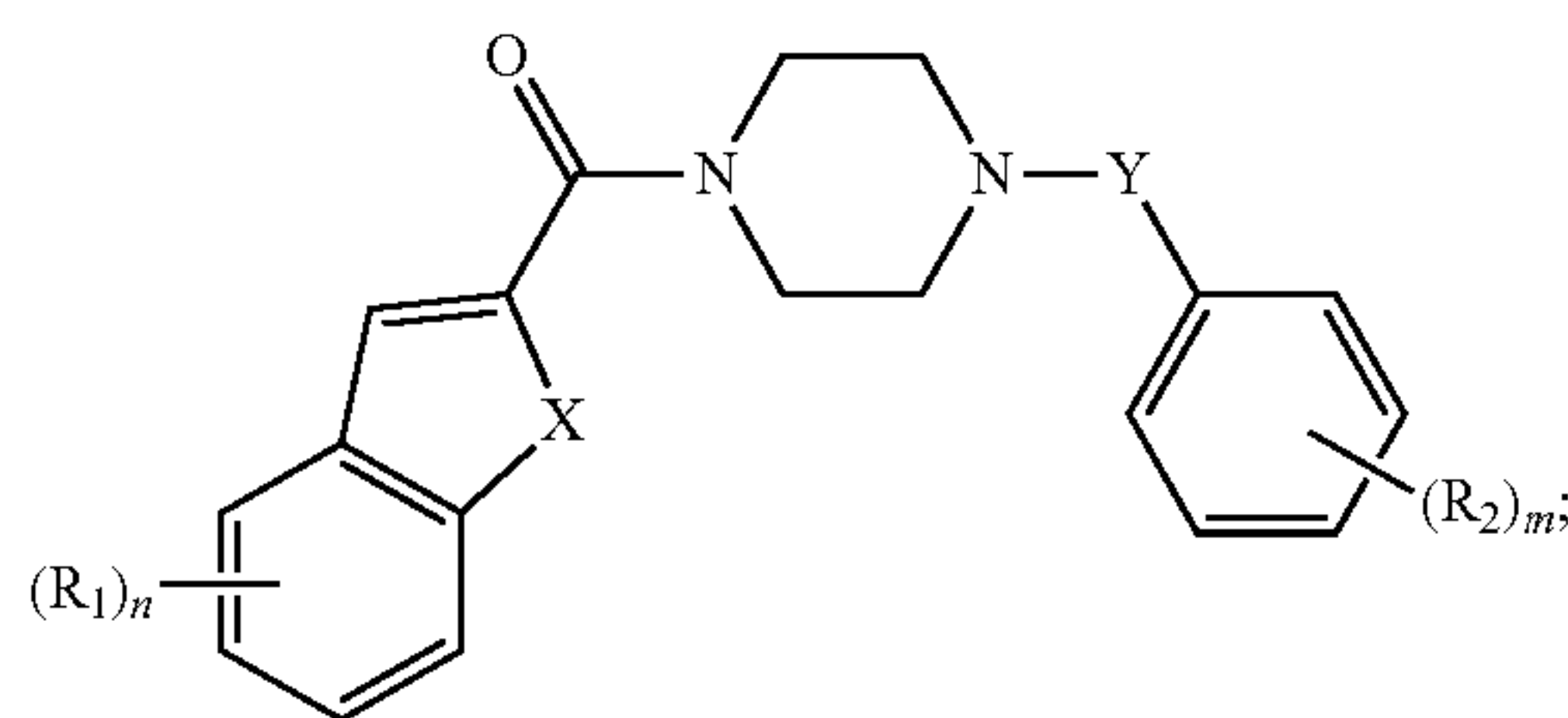
Formula (VIII)
