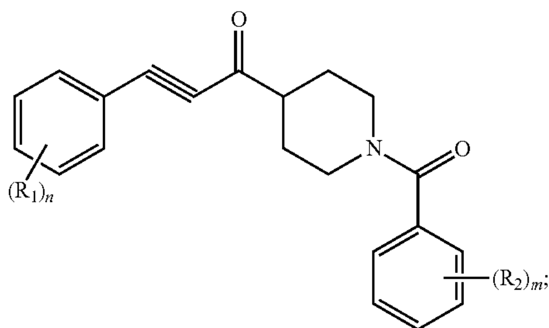
Formula (IV)
