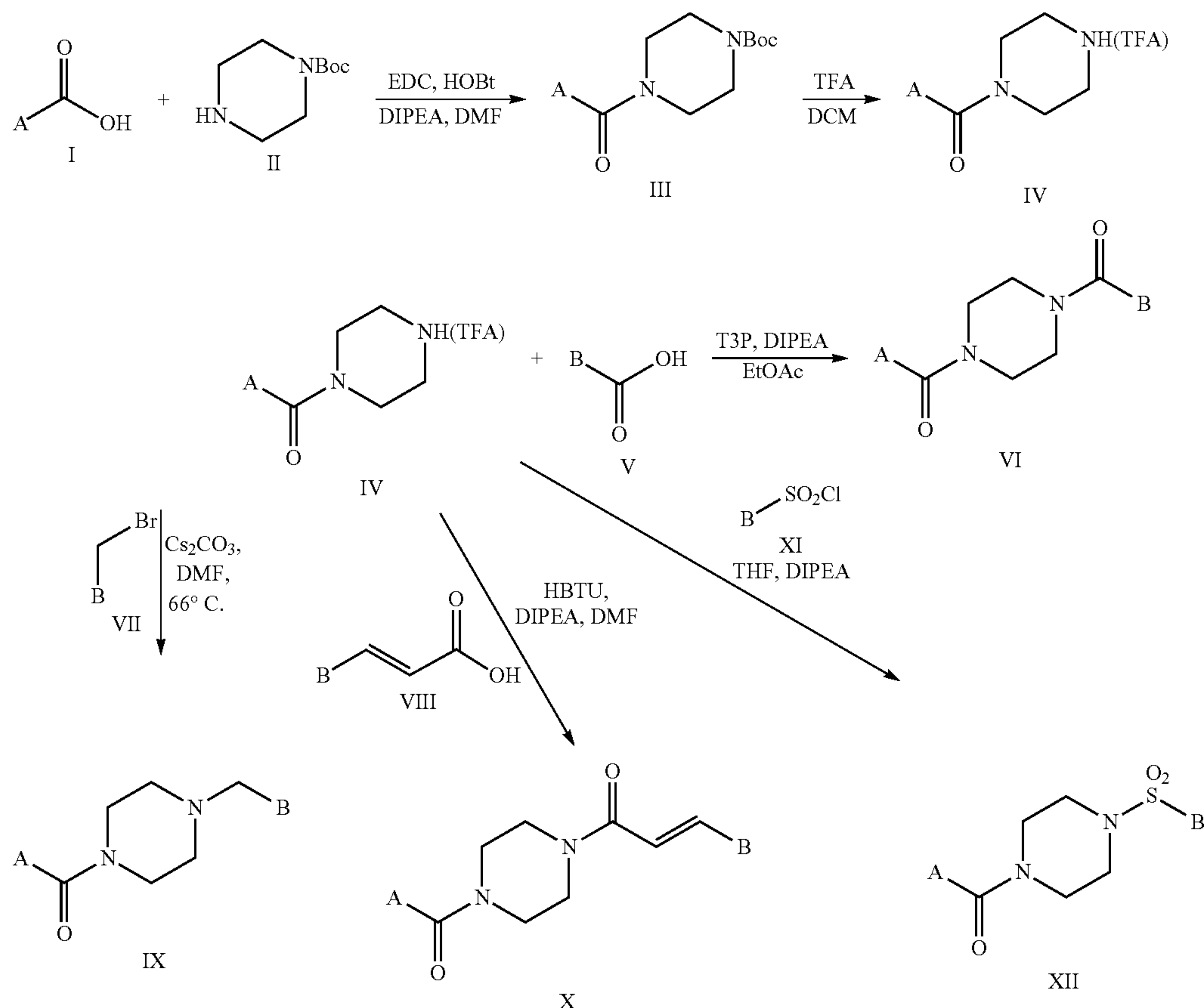
Scheme 1
