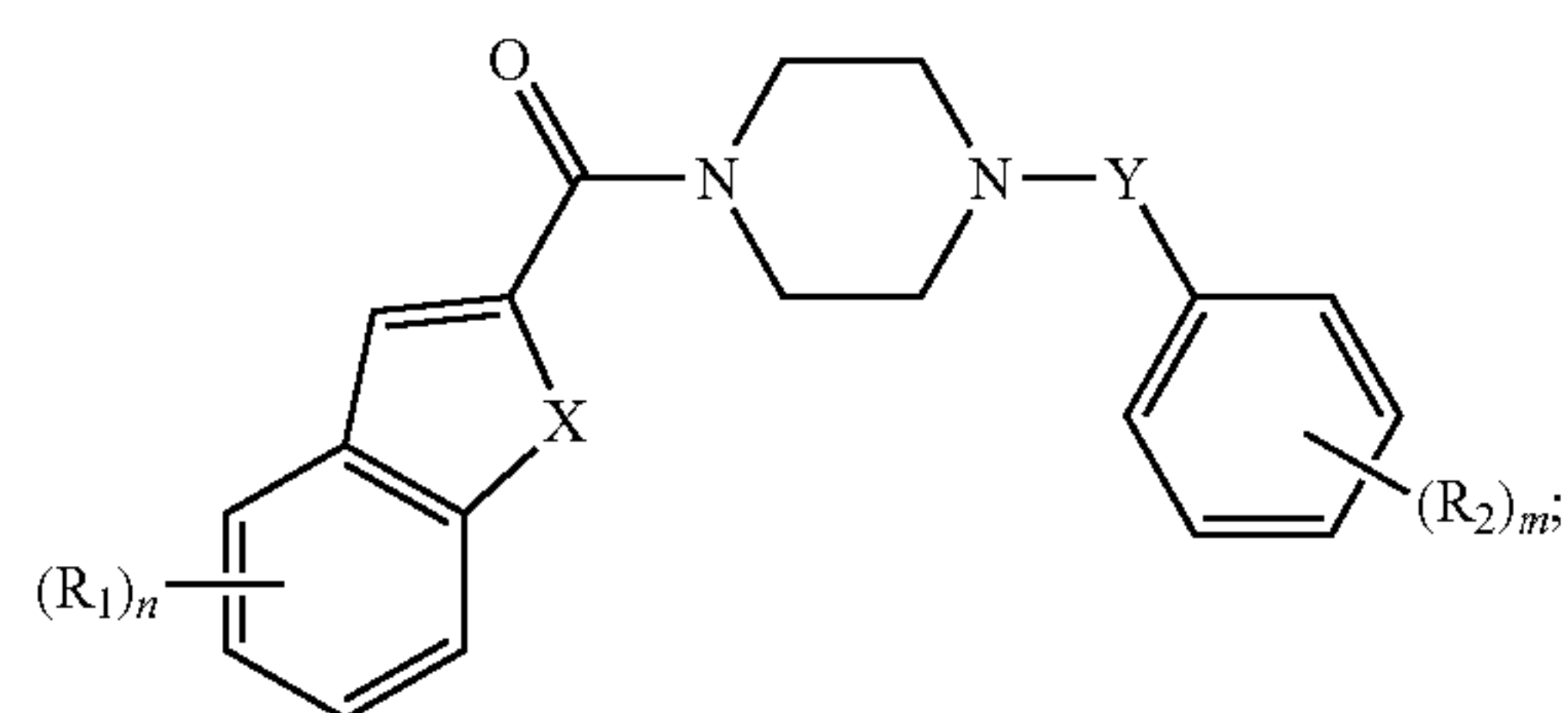
Formula (VIII)
