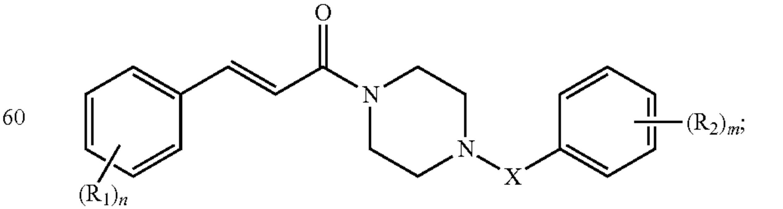
Formula (VII)
