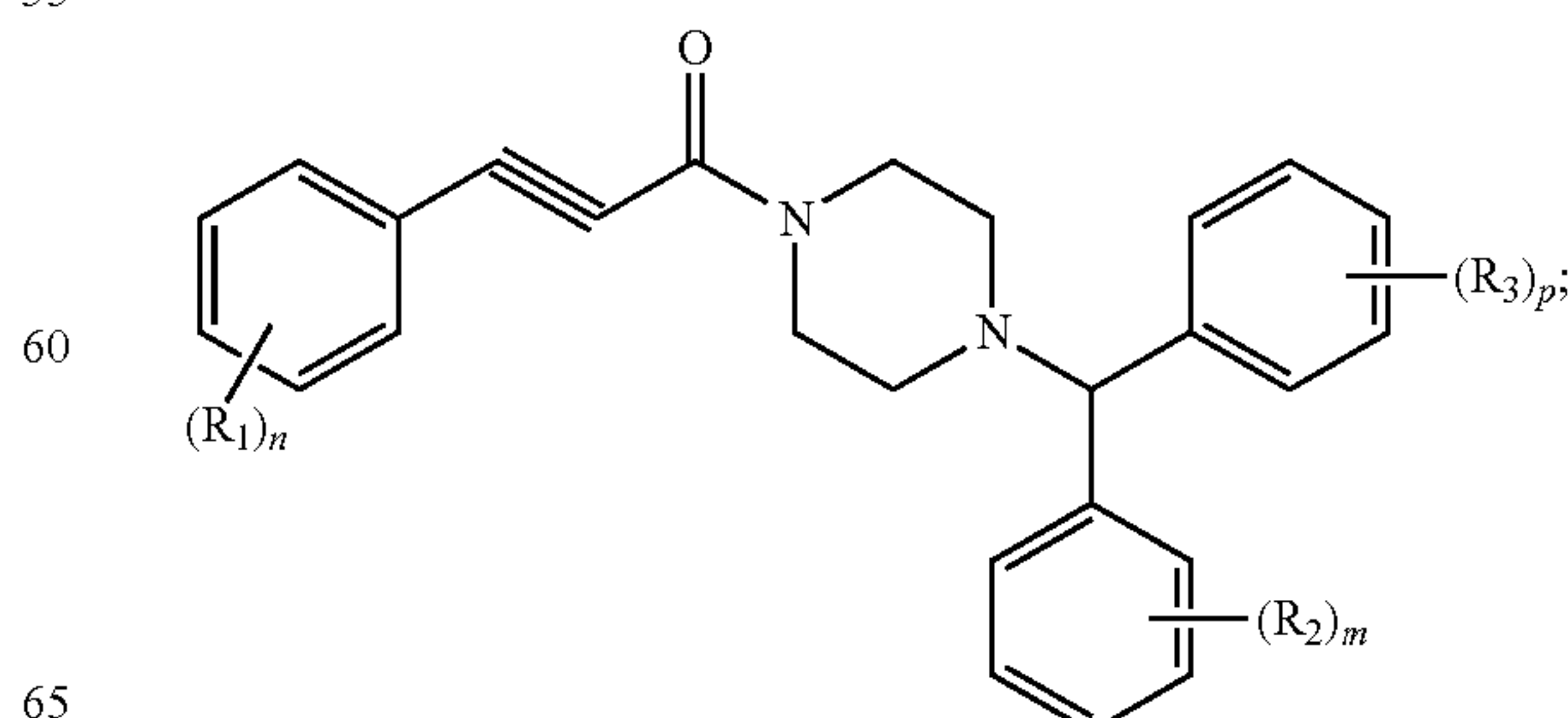
Formula (III)
