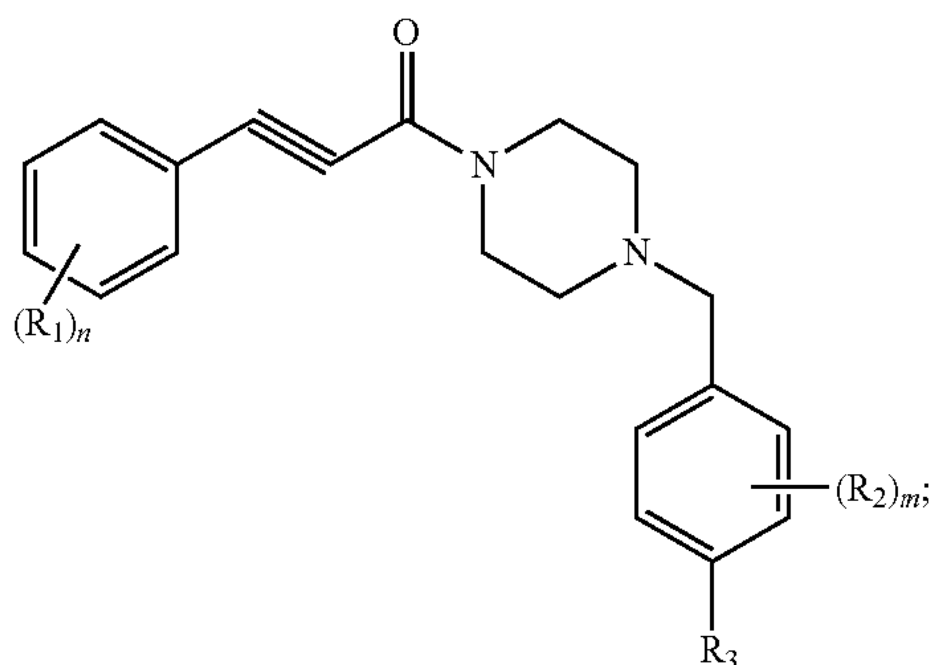
Formula (II)
