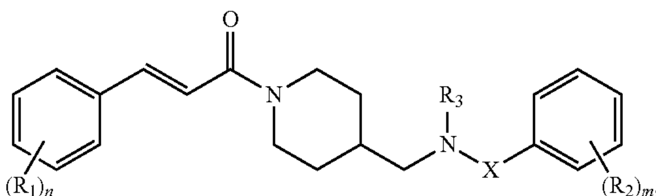
Formula (VI)
