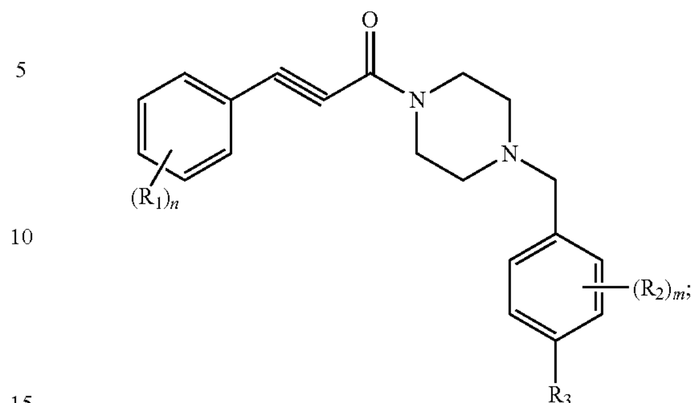
Formula (II)
