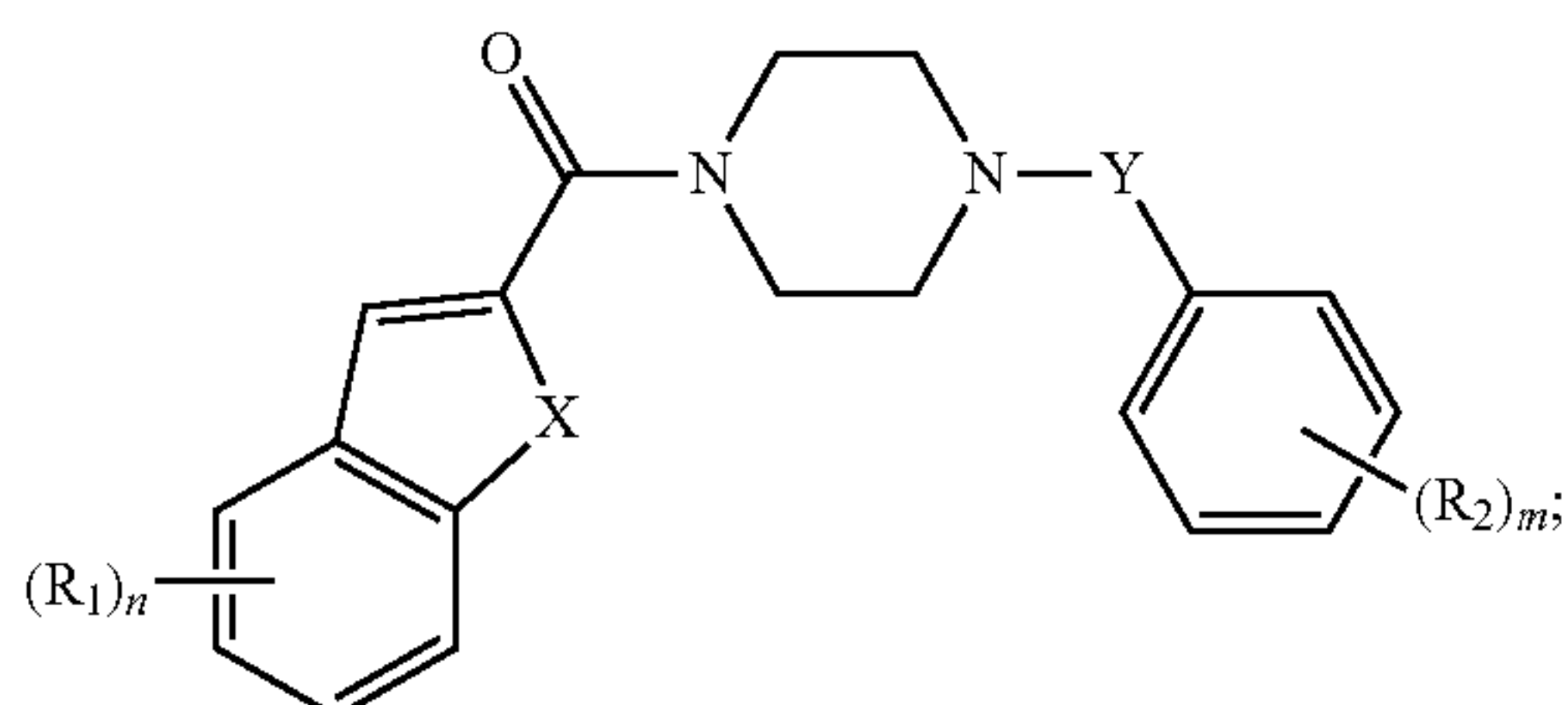
Formula (VIII)
