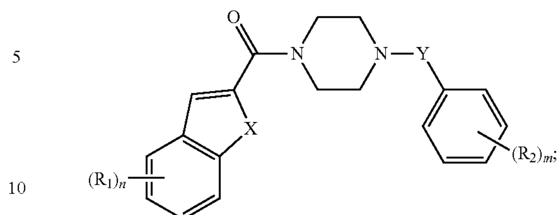
Formula (VIII)
