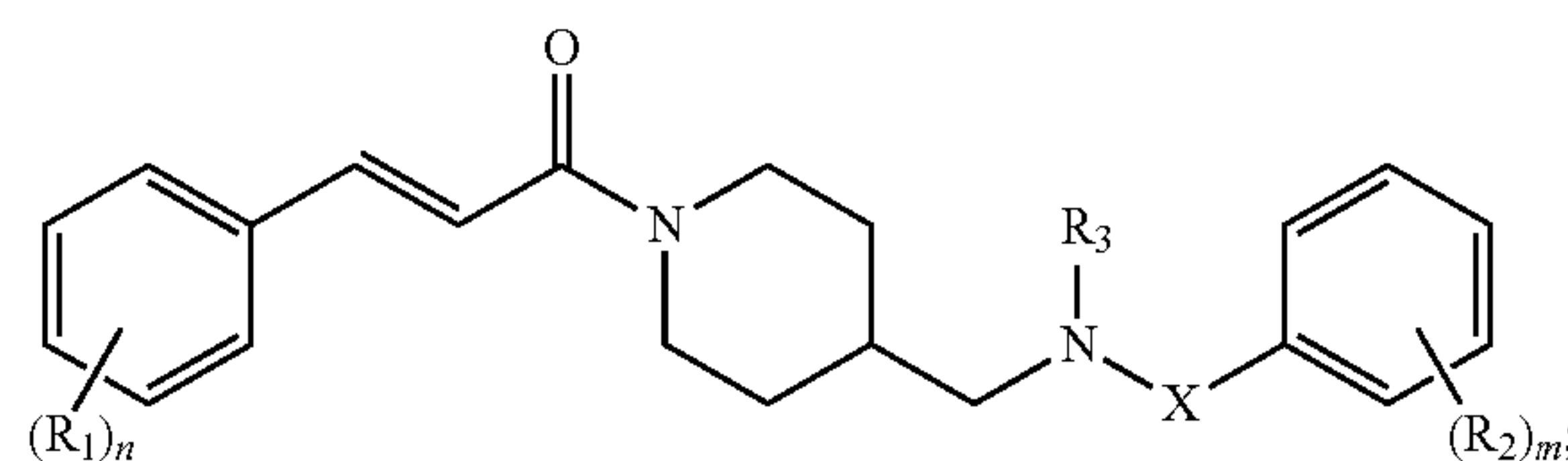
Formula (VI)
