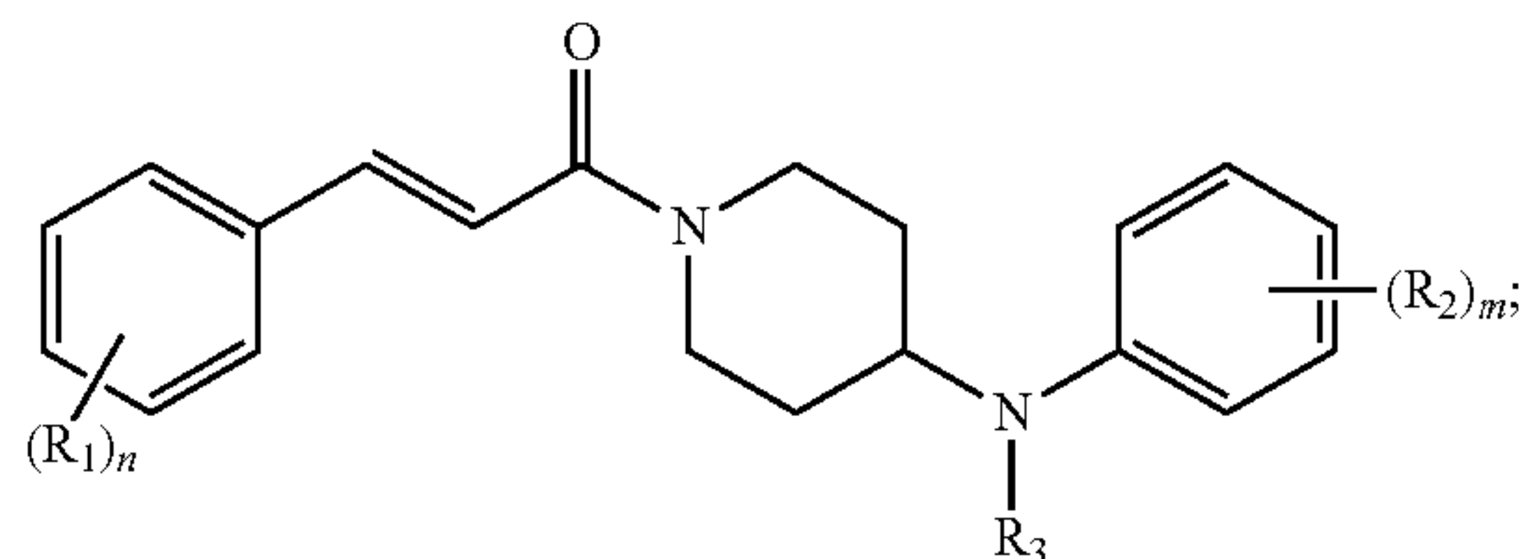
Formula (V)
