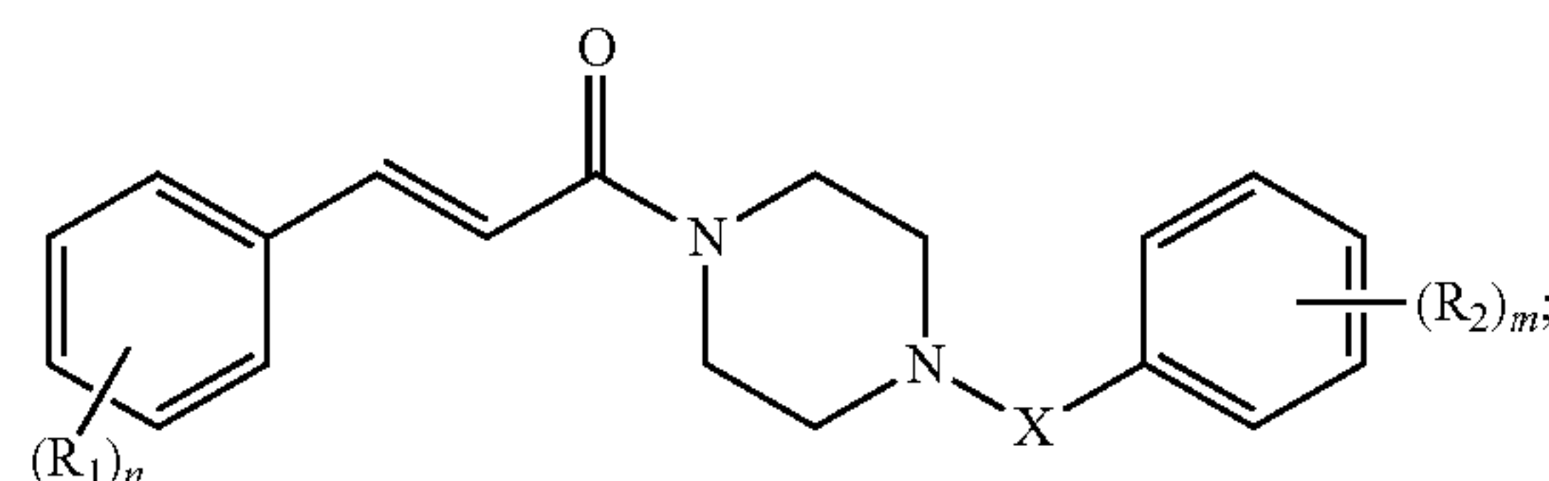
Formula (VII)
