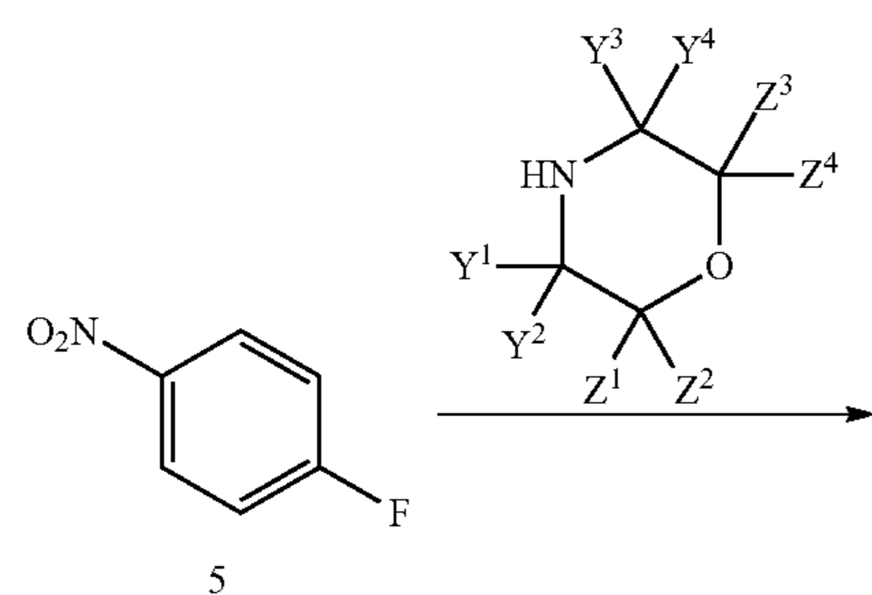
Scheme 2: Preparation of Intermediate 2
