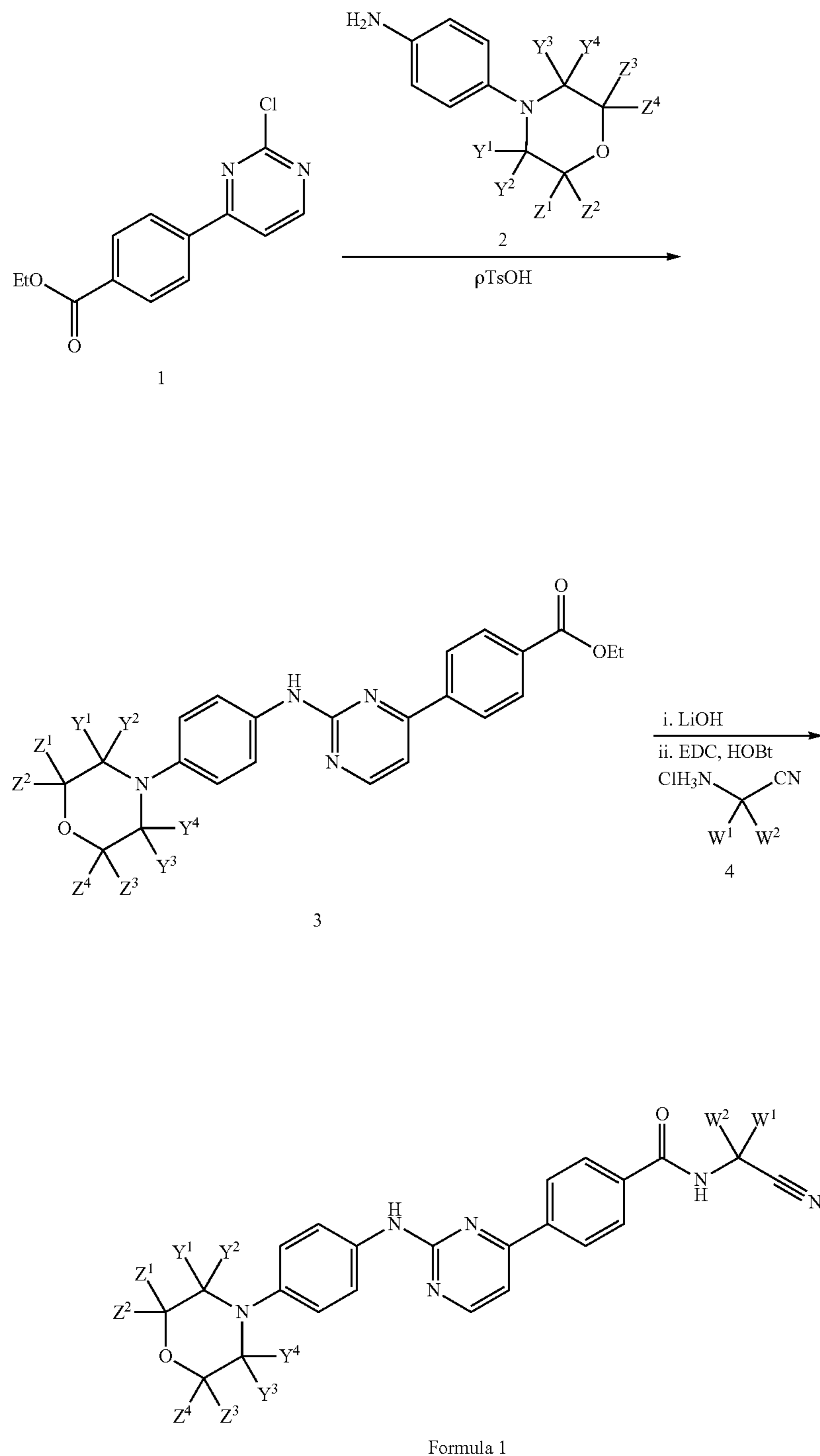
Scheme 1: Preparation of Compounds of Formula I
