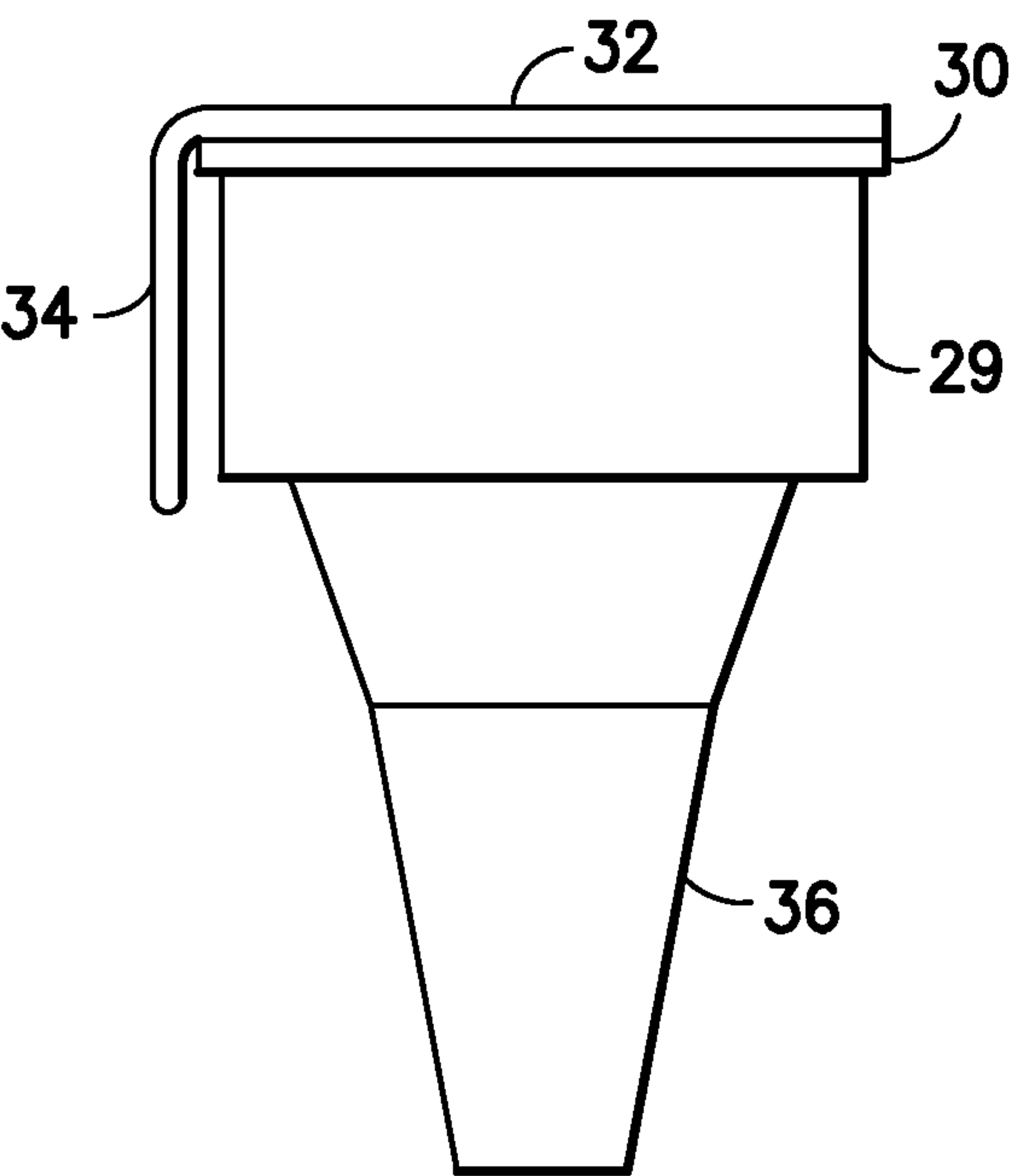
FIG. 8 (PRIOR ART)
