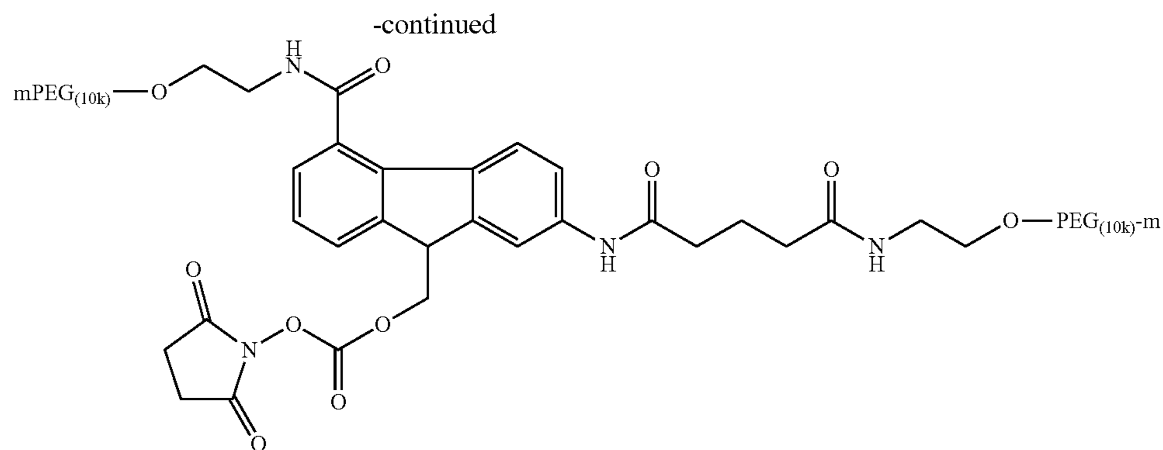
9-hydroxymethyl-4-(mPEG(10,000)-carboxyamide)-7-(mPEG(10,000)-amidoglutaric acid)fluorene-N-hydroxysuccinimide
