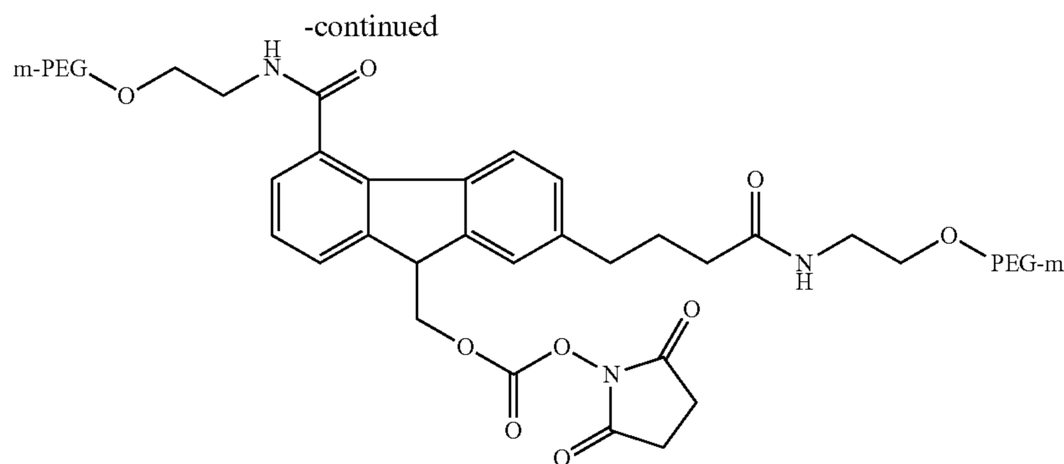
9-hydroxymethyl-4-(mPEG(10,000)-carboxamide)-7-(3-(mPEG(10,000))carbamoyl-propyl)fluorene-N-hydroxysuccinimide
