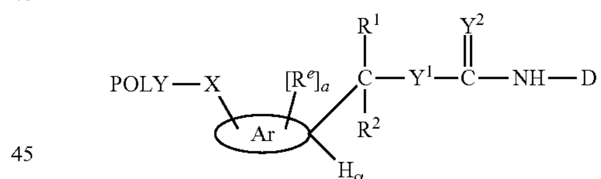
(Formula IV-C)
