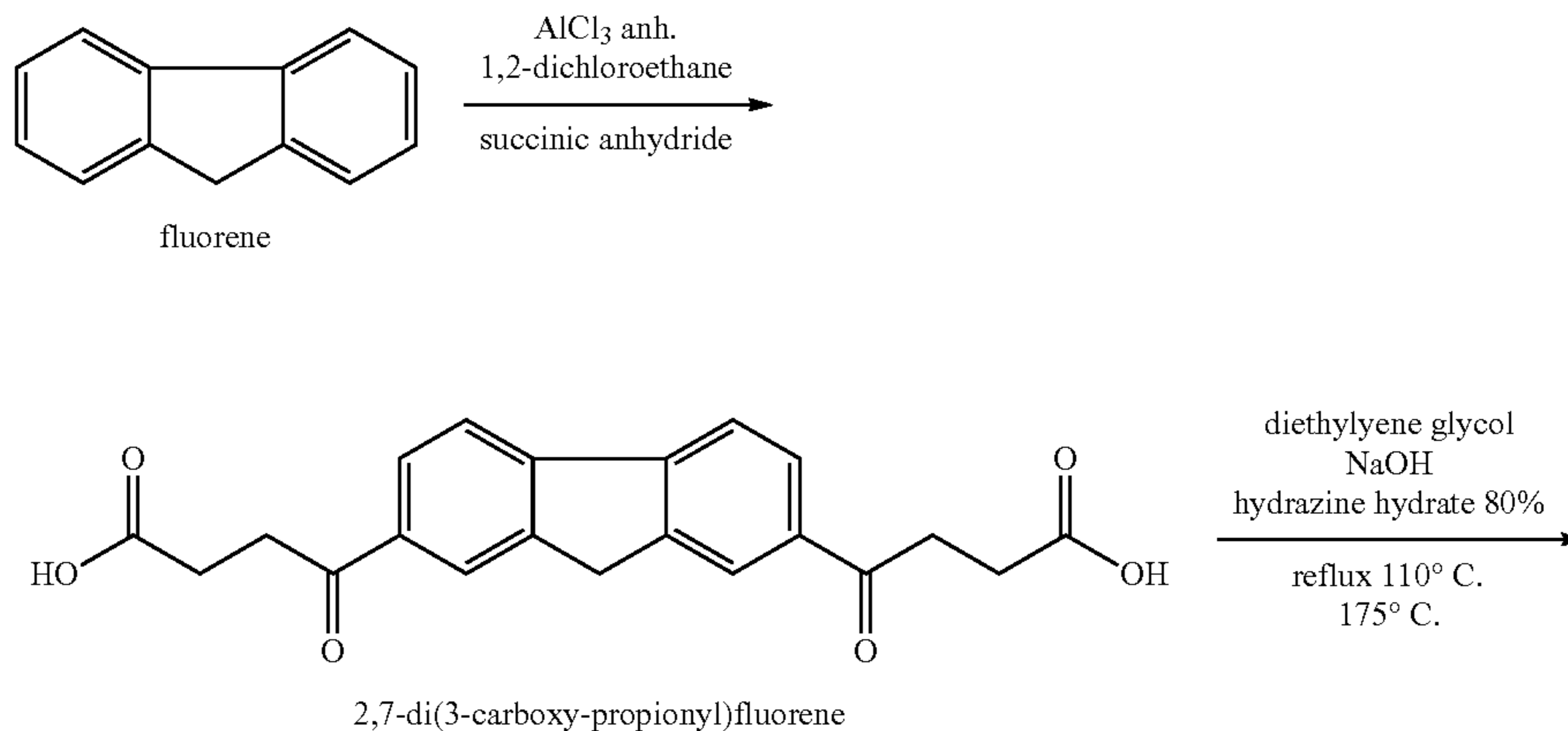
Scheme 6.
