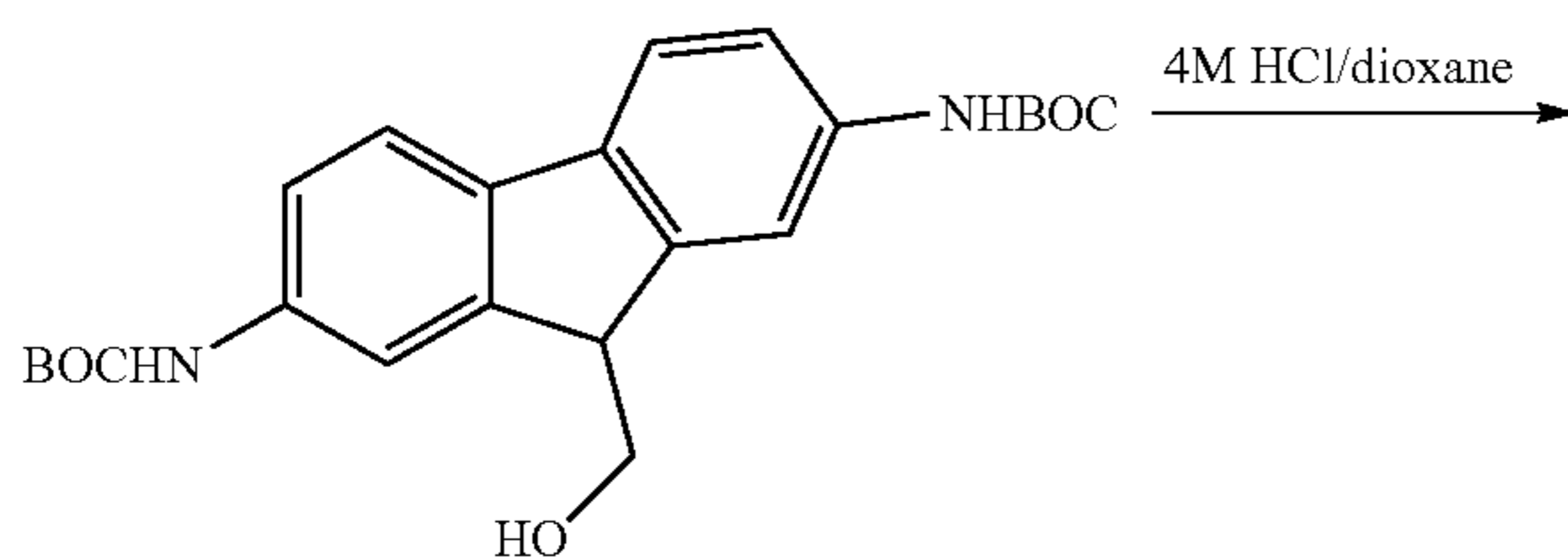
9-hydroxymethyl-2,7-di(Boc-amino)fluorene
