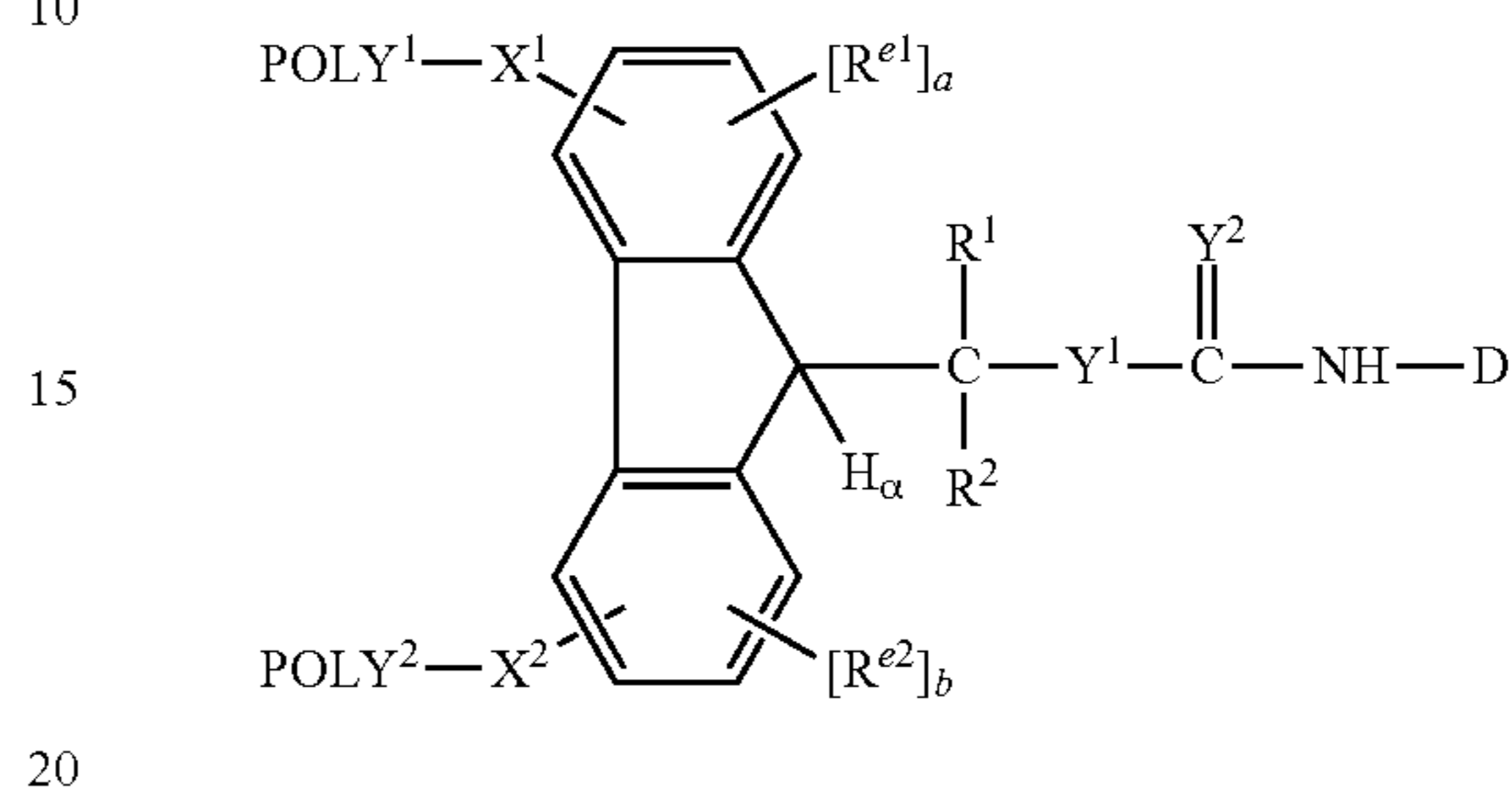
(Formula III-C)
