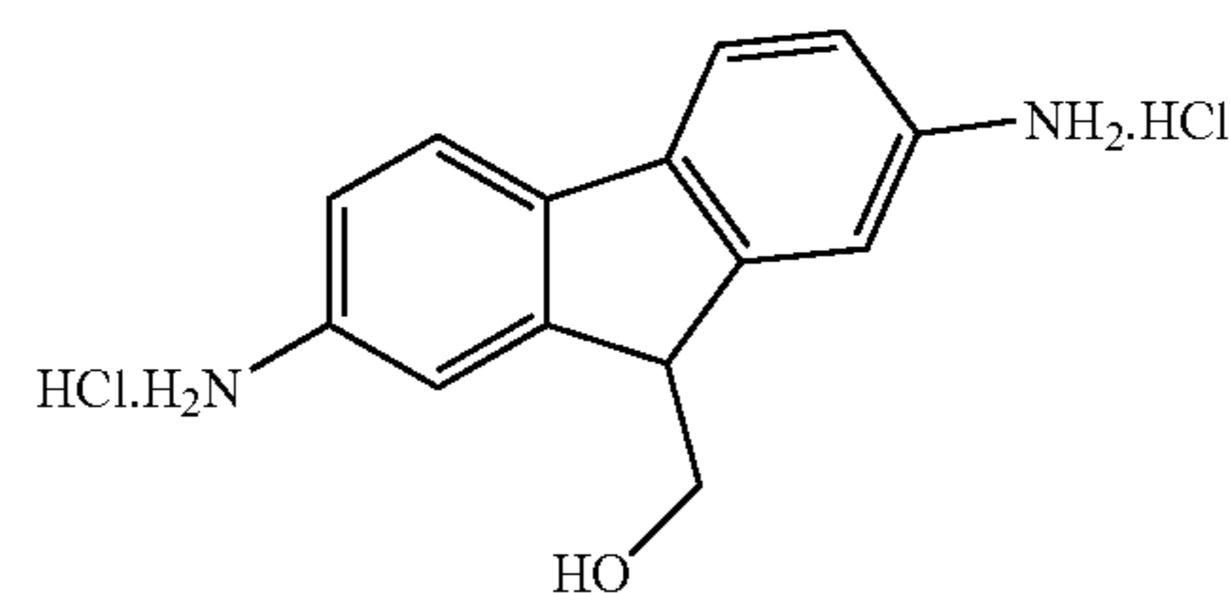
9-hydroxymethyl-2,7-diaminofluorene dihydrochloride
