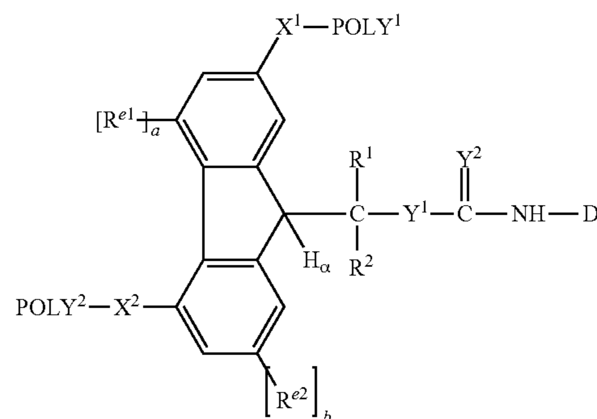
(Formula Vf-C)
