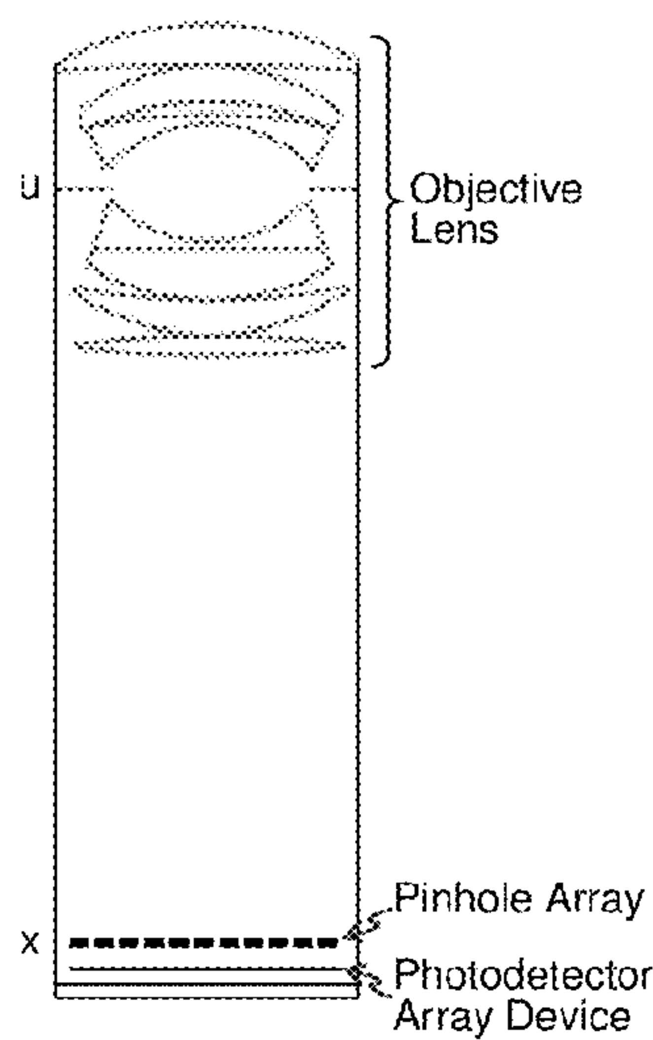
Fig. 1C: Prior Art - Light field Radiance Capture Camera
