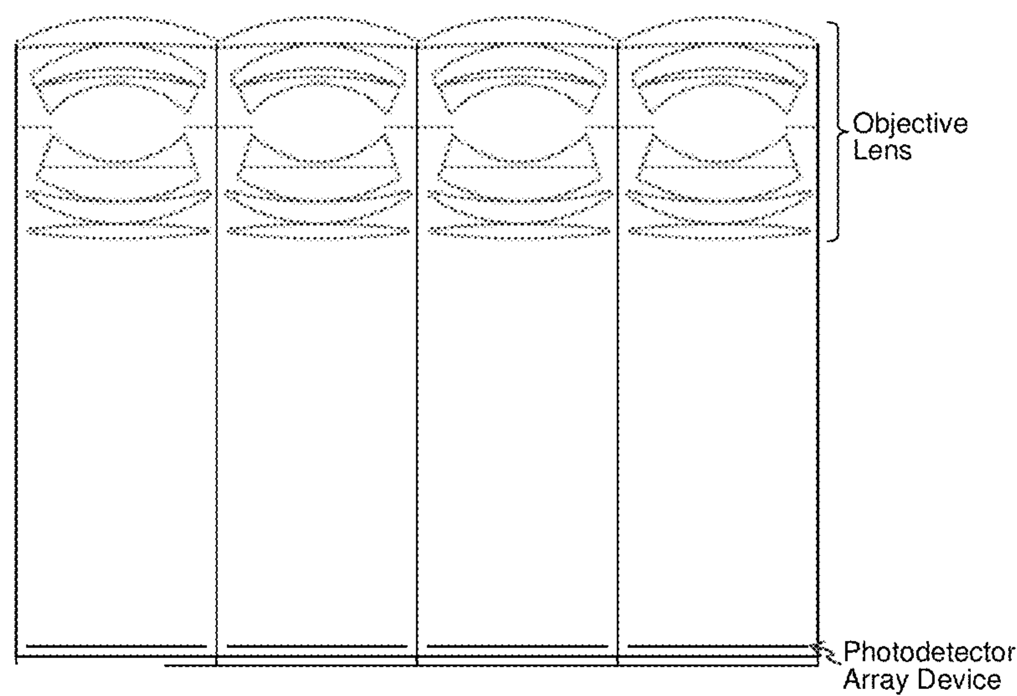
Fig. 1A: Prior Art - Light Field Camera Array
