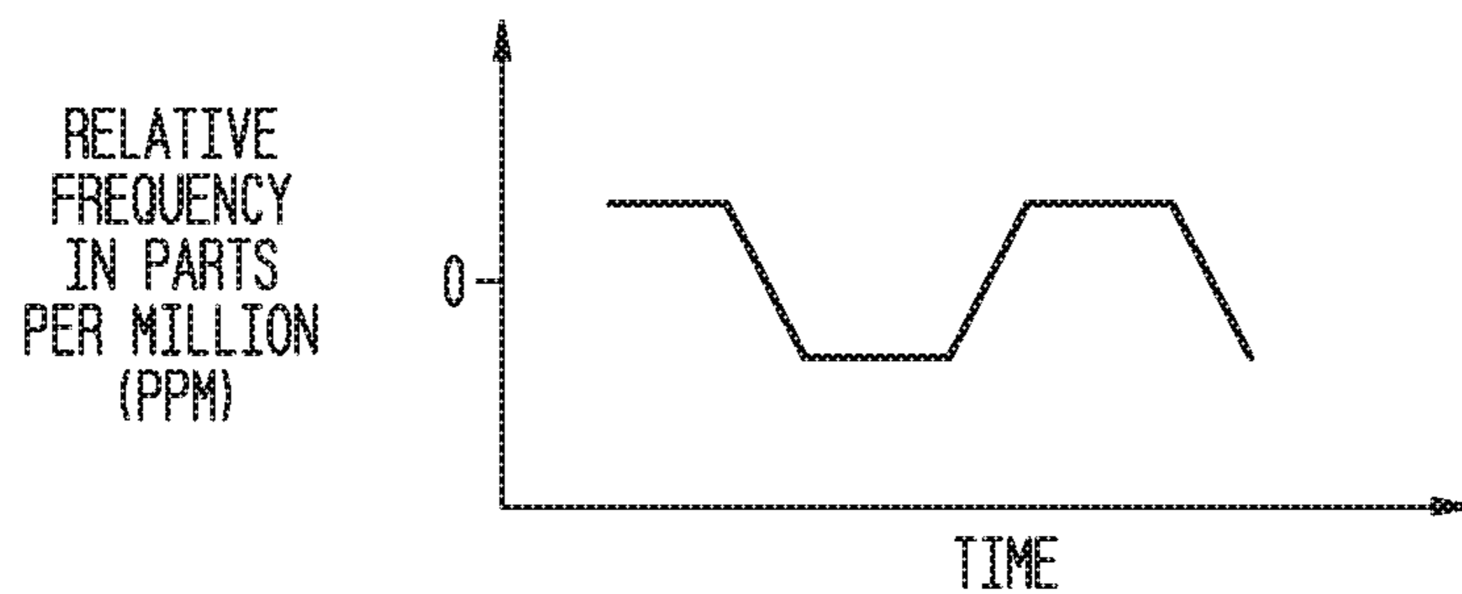
FIG. 2C FREQ OFFSET B/W TX AND RX
