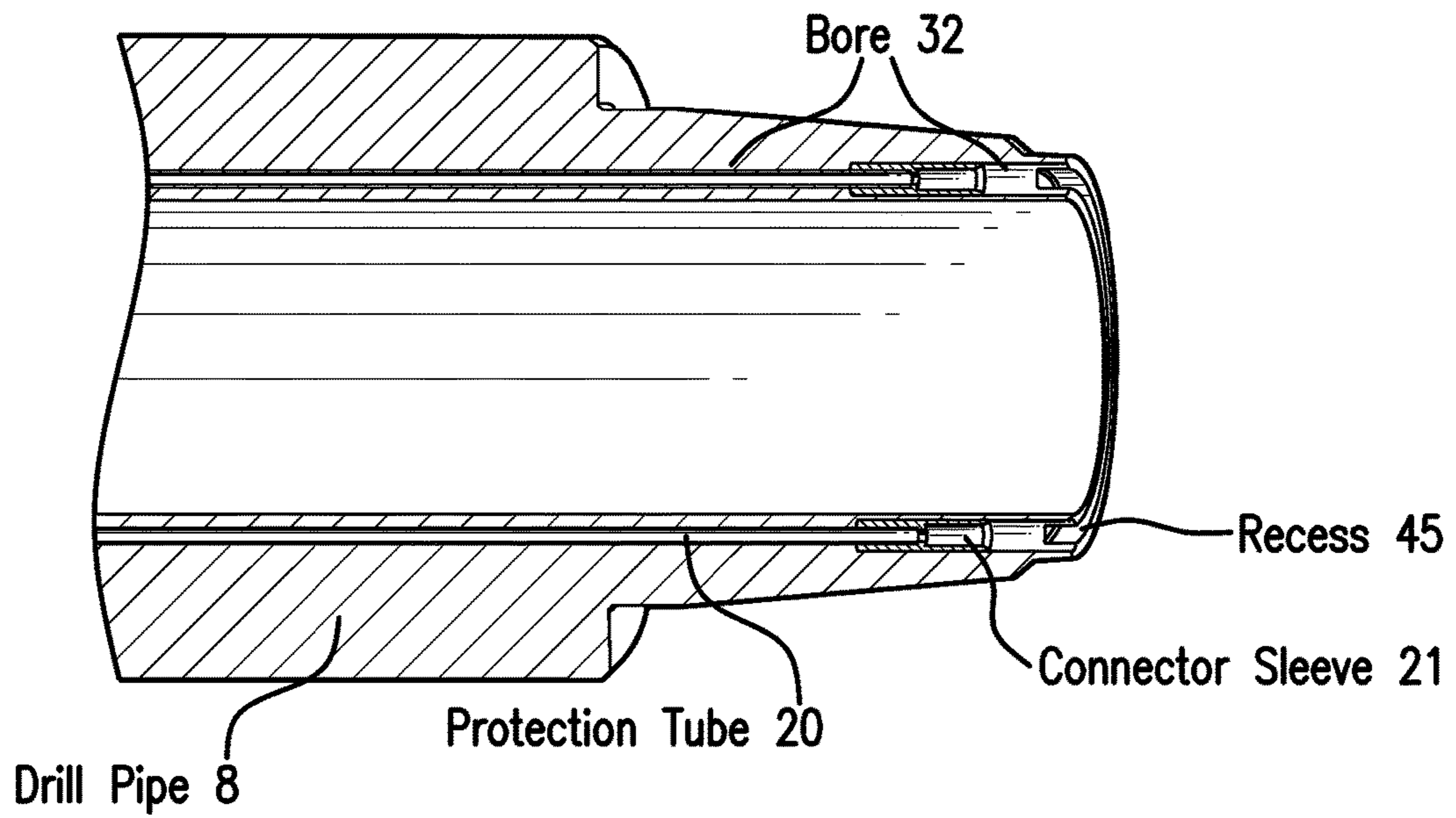
Pin End of Drill Pipe
