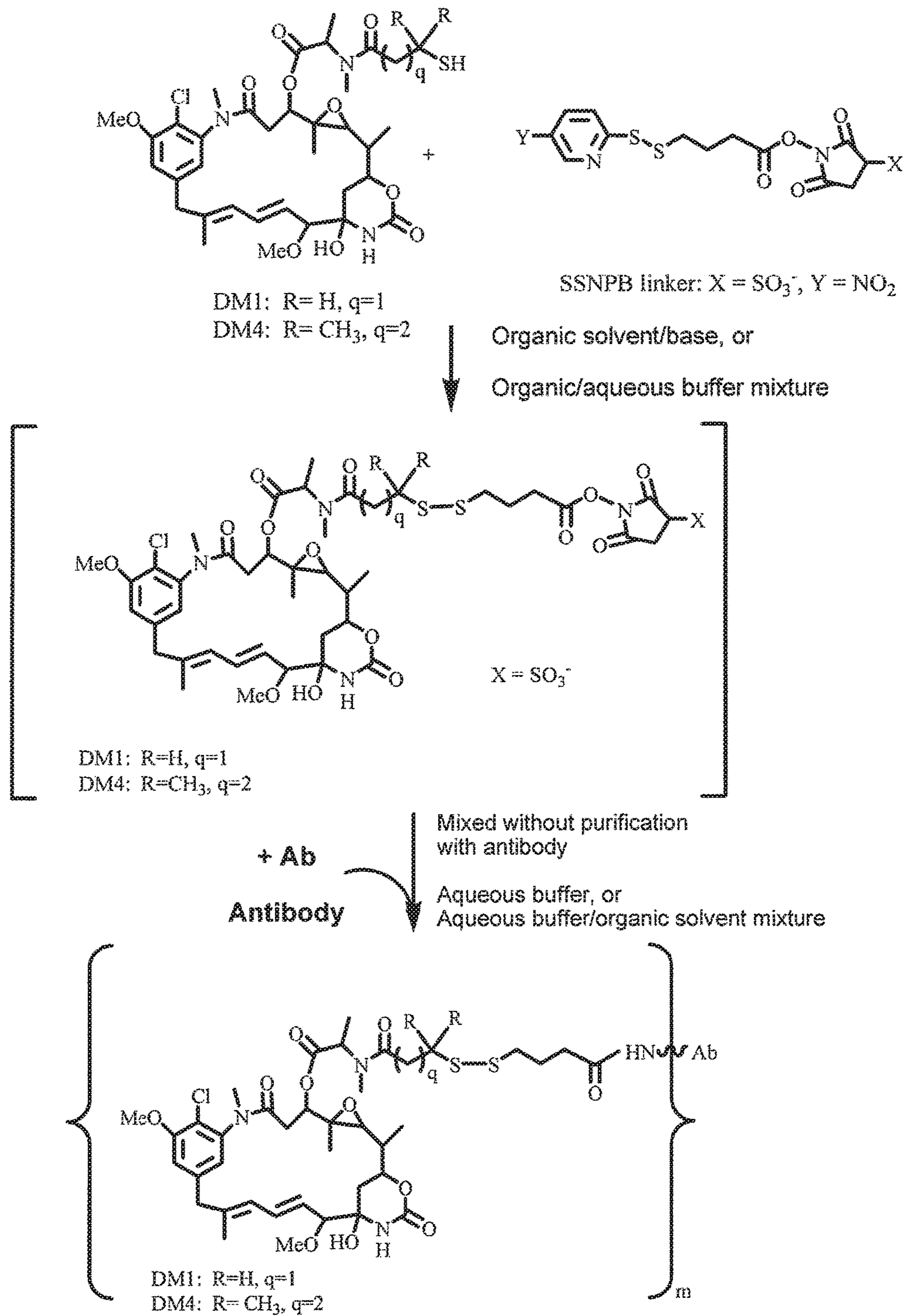
Antibody-maytansinoid conjugate with cleavable, disulfide linker
