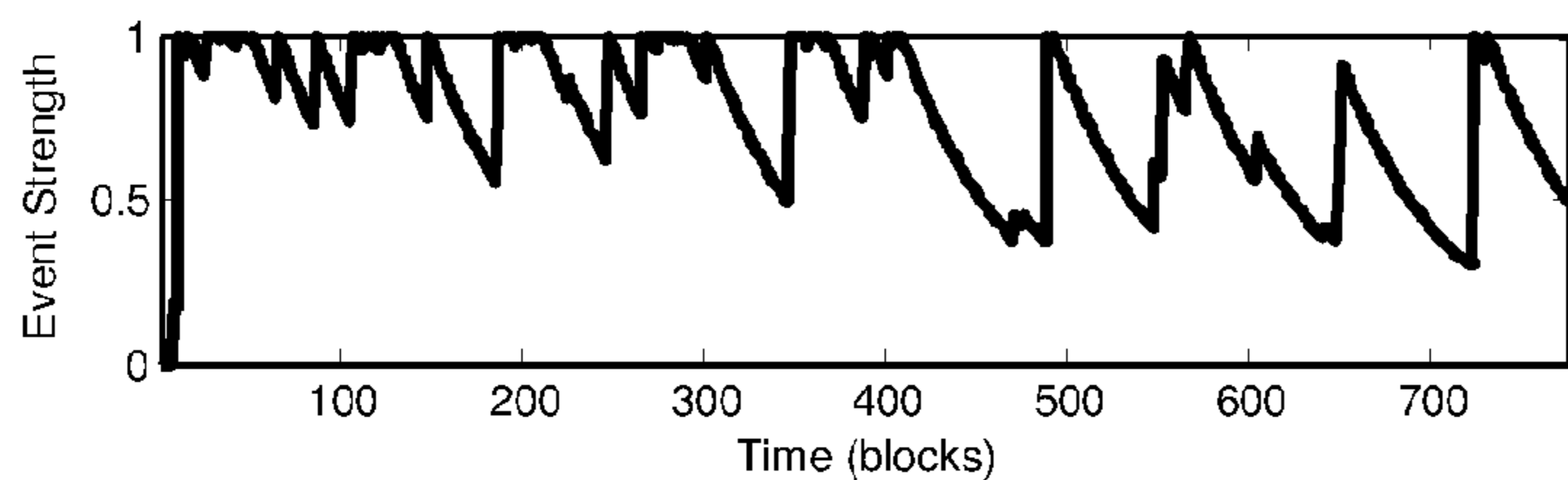
FIG. 10d d) Event control signal
