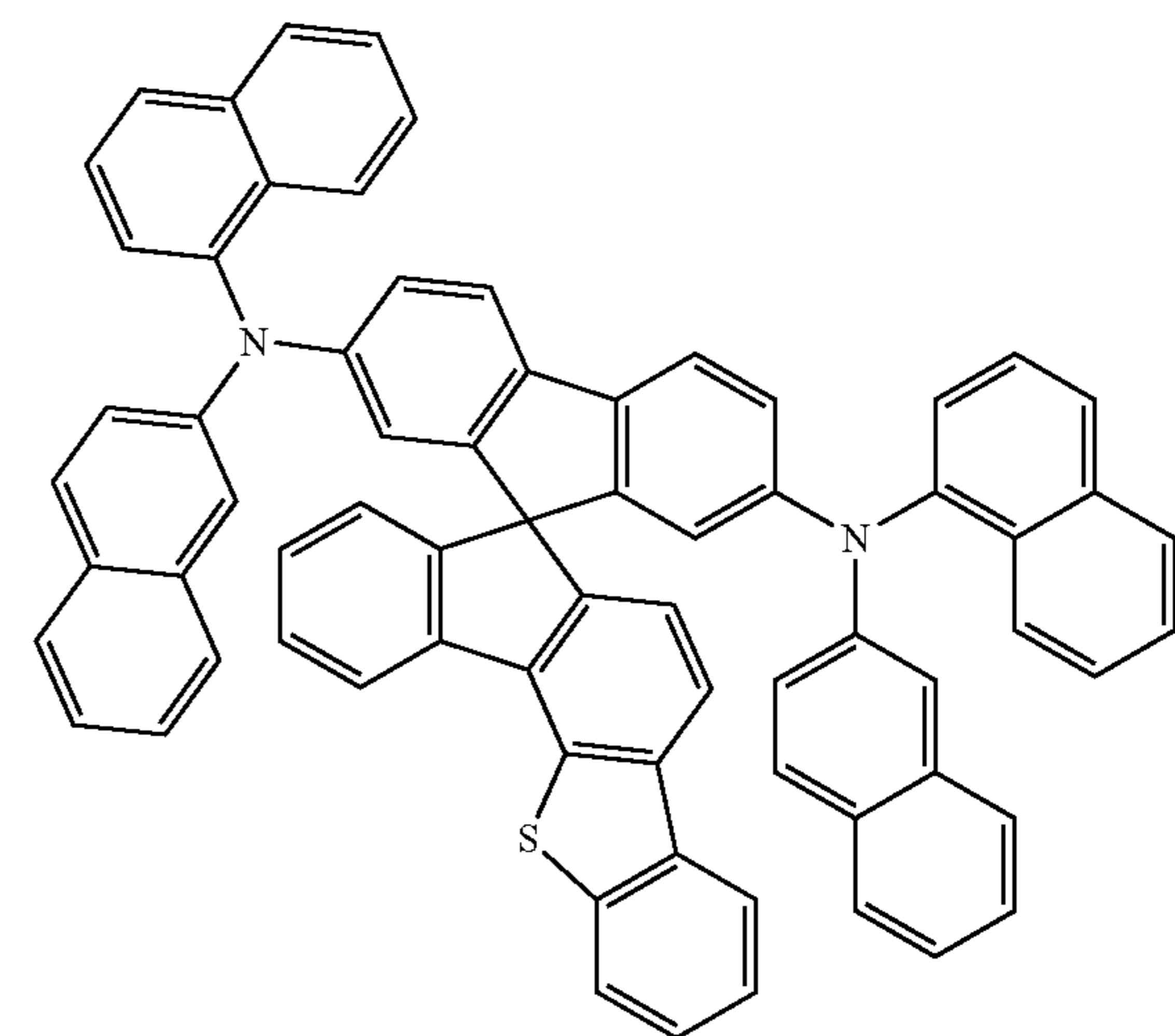
[Chemical Formula B-24]
