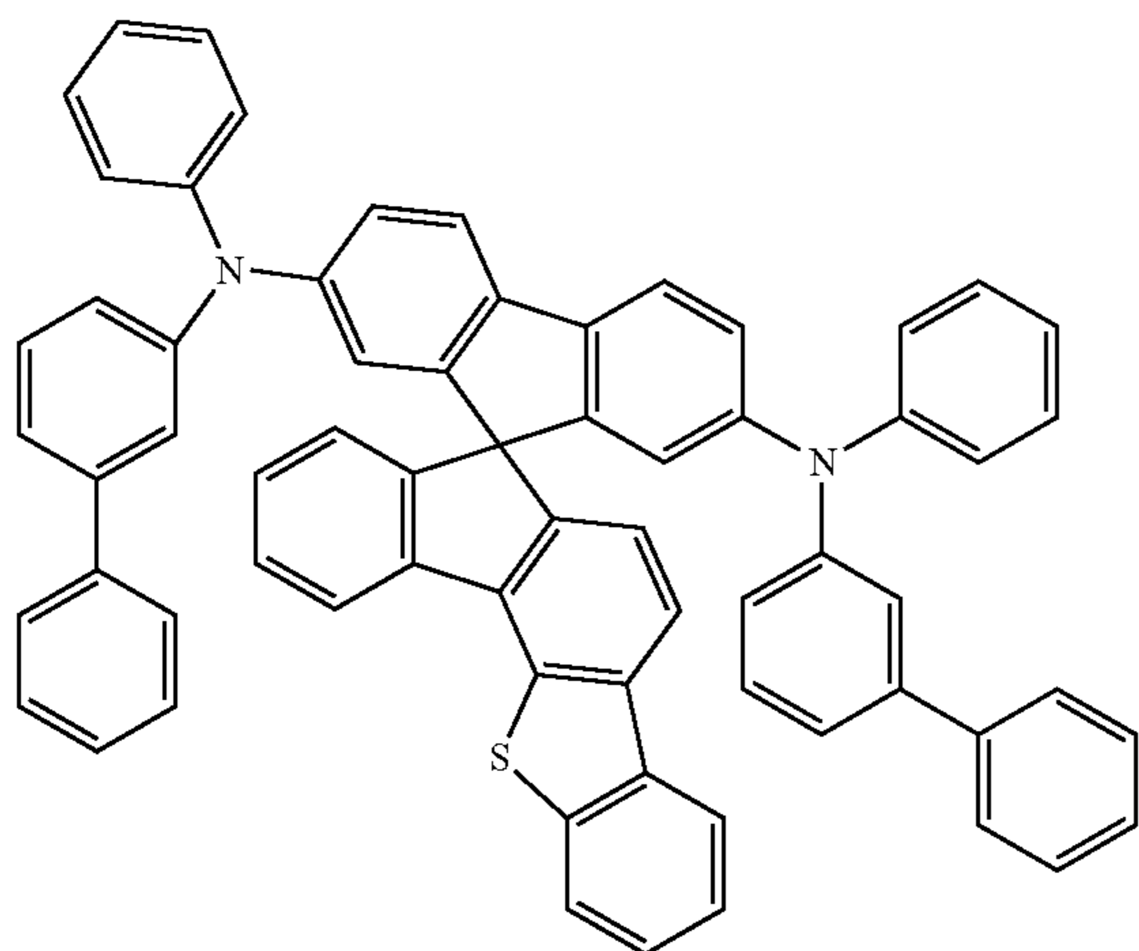
[Chemical Formula B-26]
