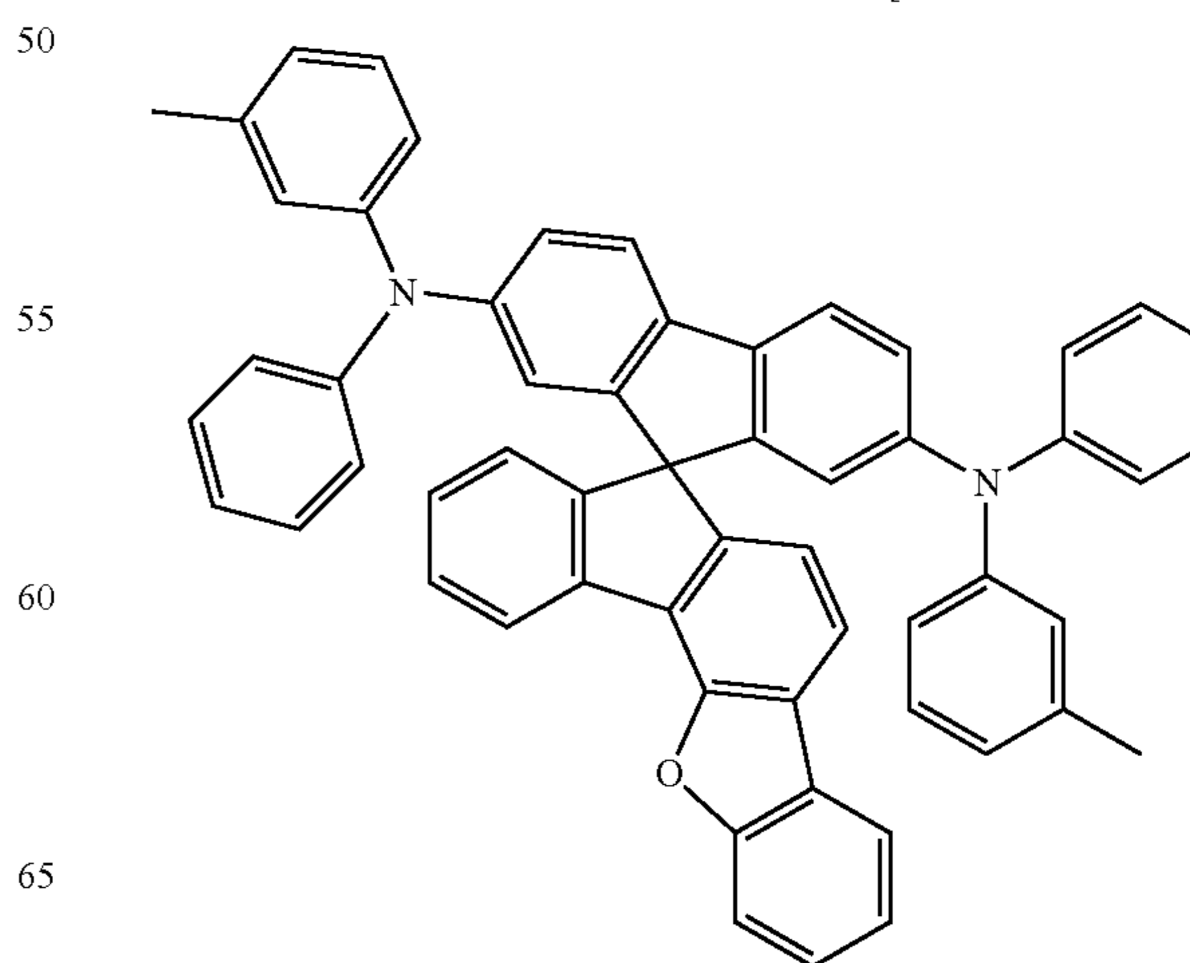
[Chemical Formula B-11]
