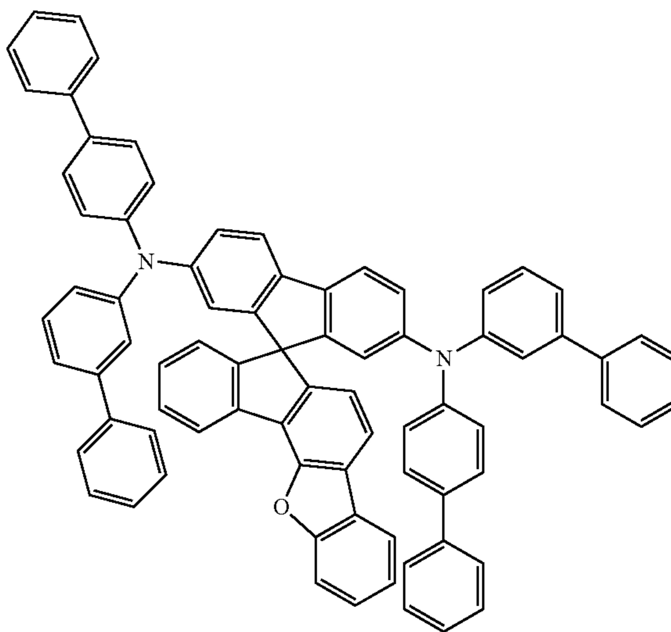
[Chemical Formula B-6]
