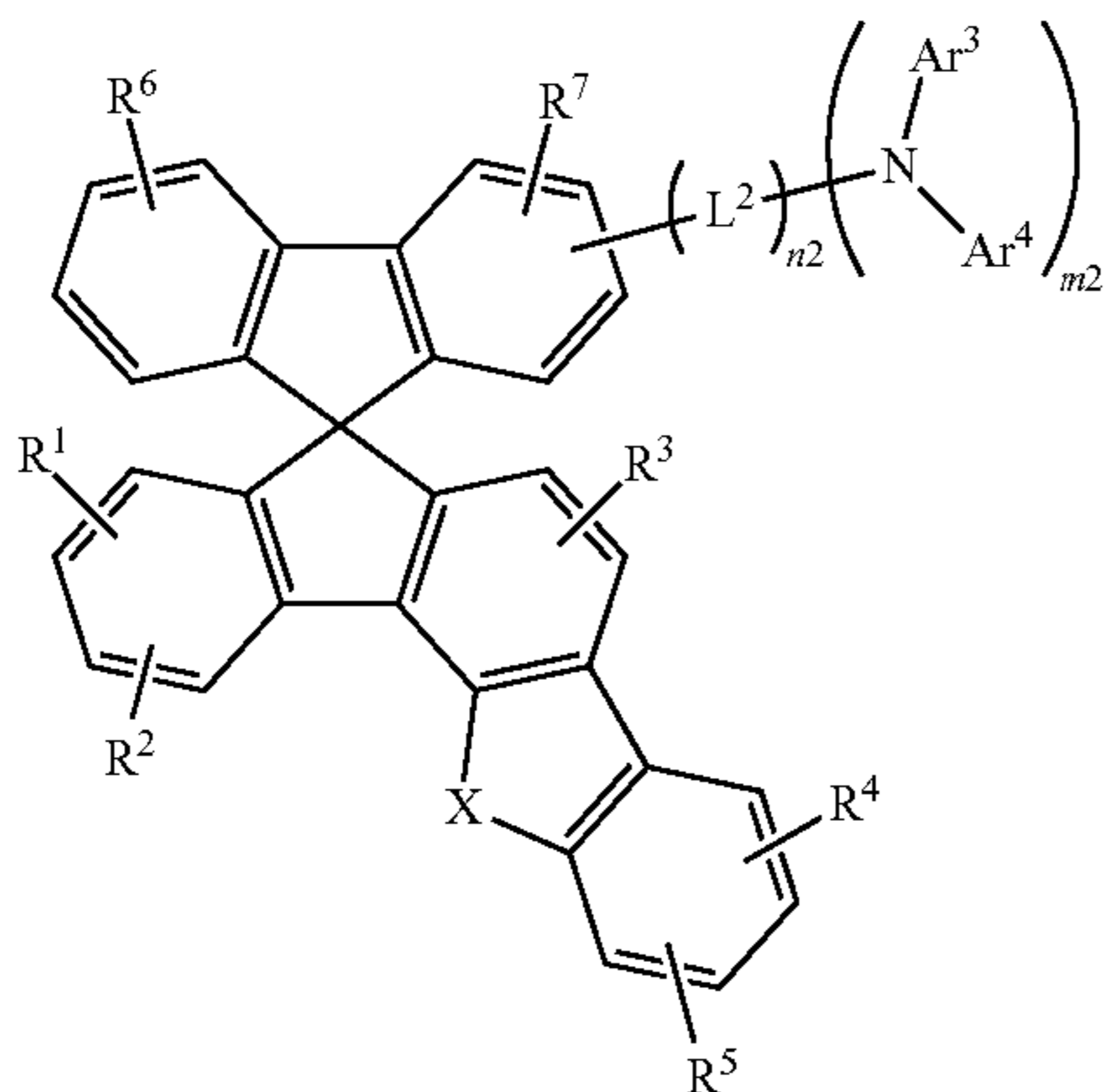
[Chemical Formula 5]
