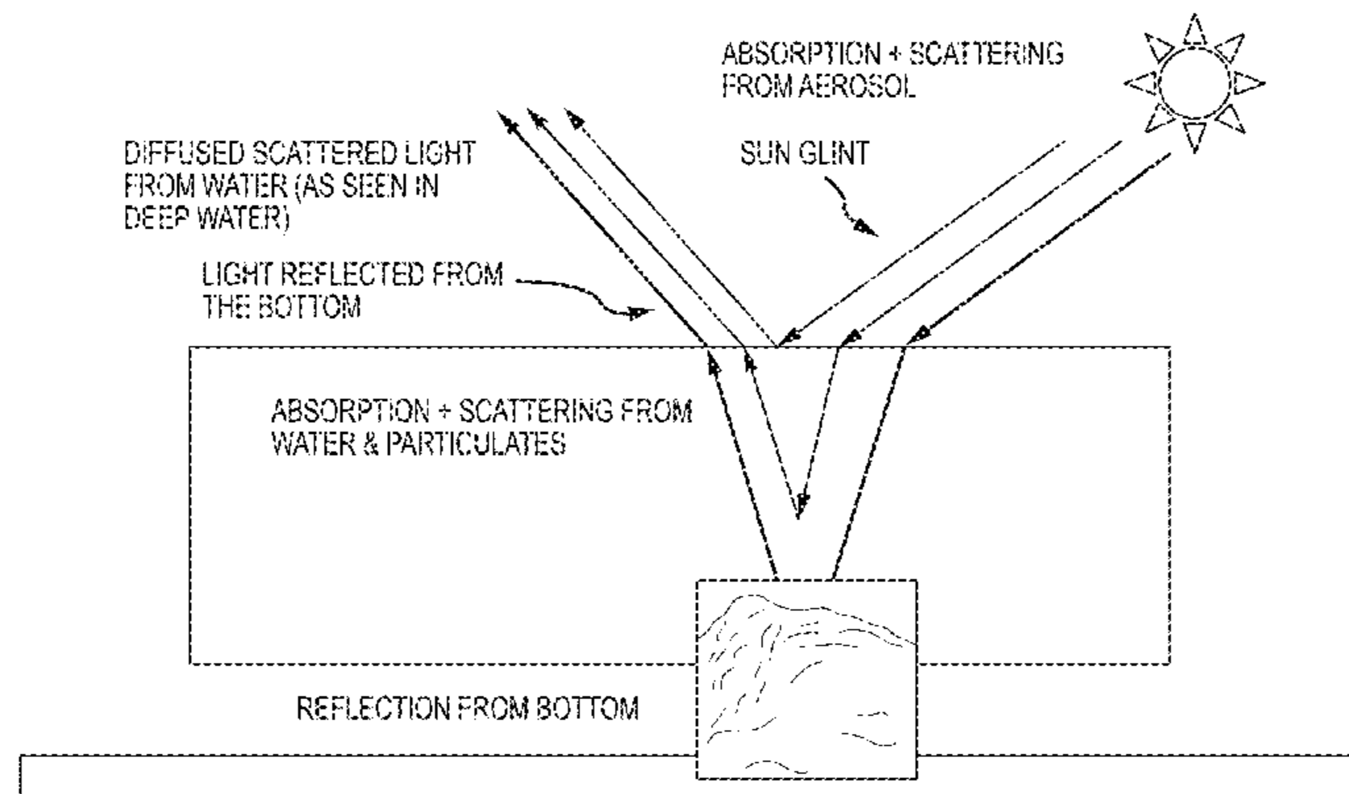
INTERACTION OF LIGHT WITH WATER AND ATMOSPHERE
