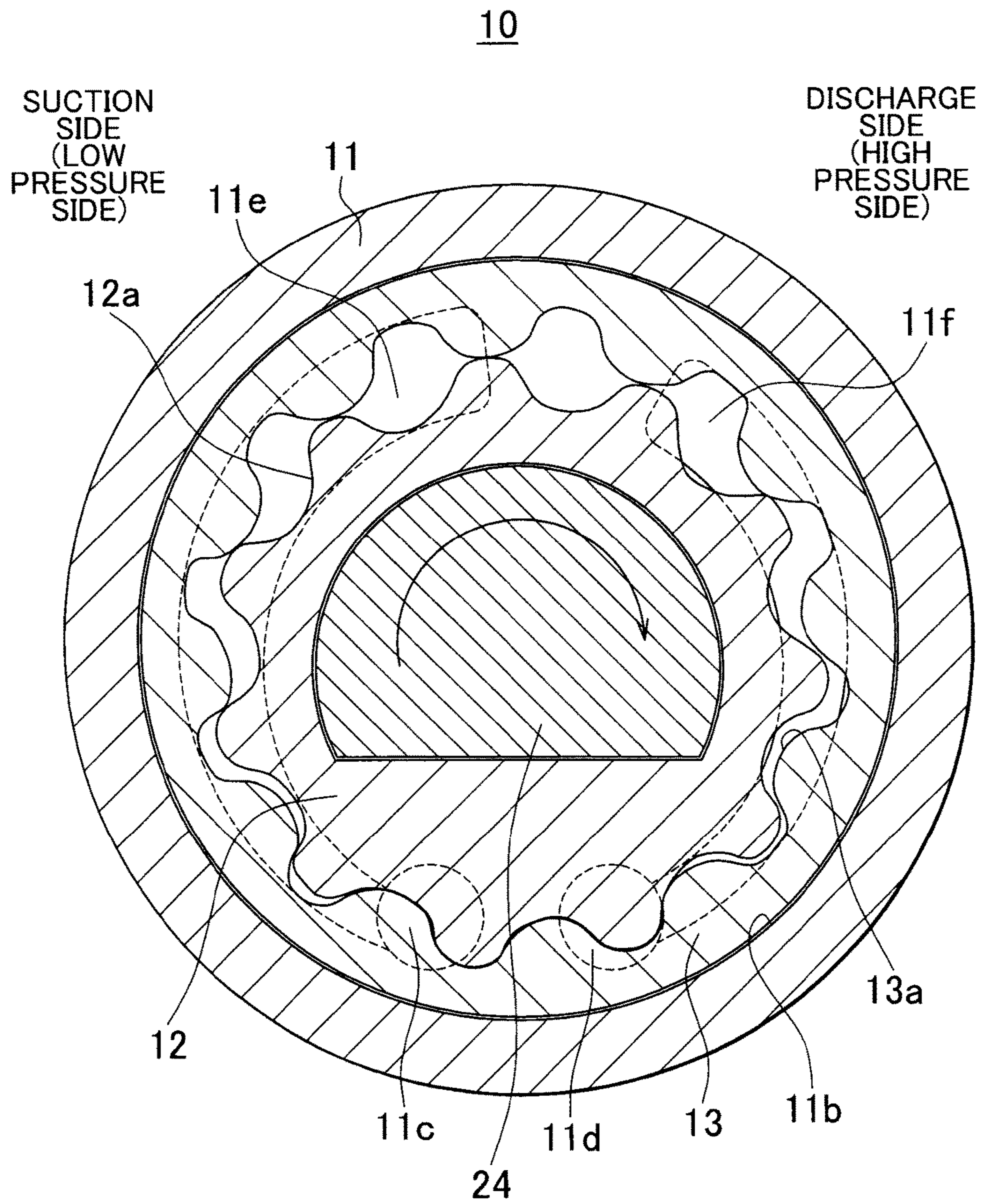
FIG. 2 SECTION TAKEN ALONG LINE A-A
