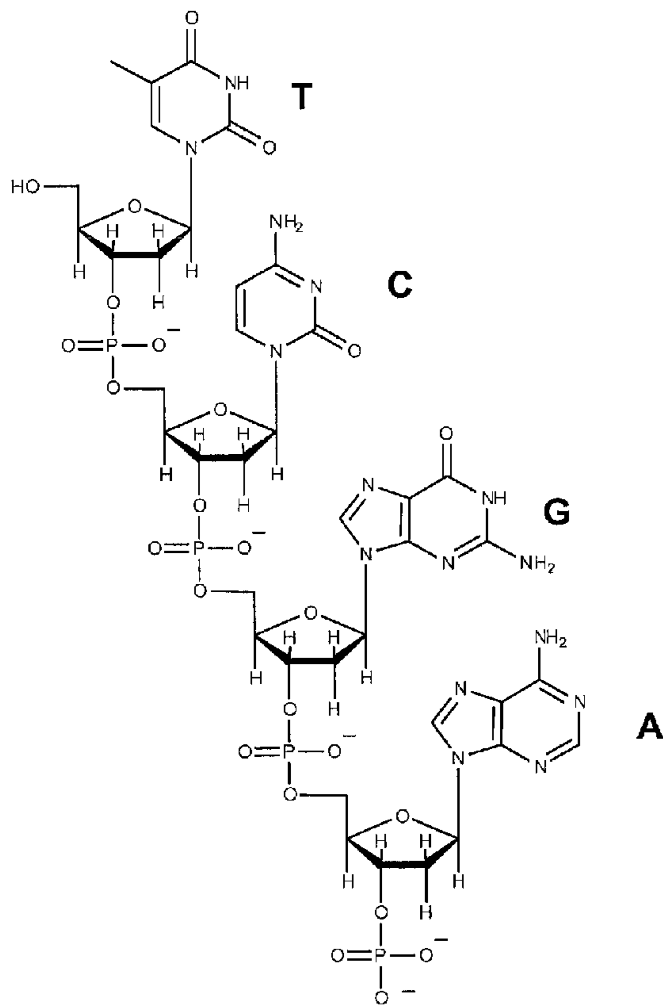
Natural DNA
