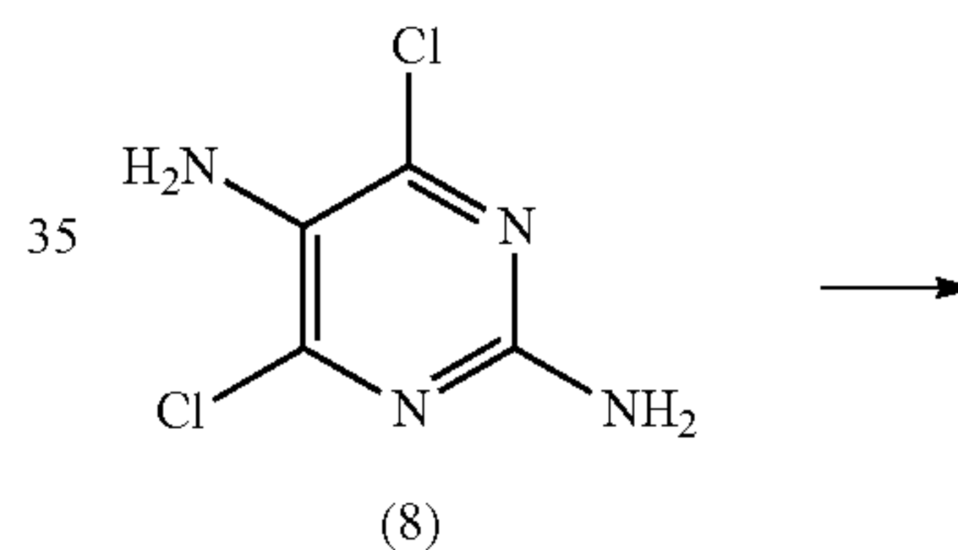
Reaction Scheme 2
