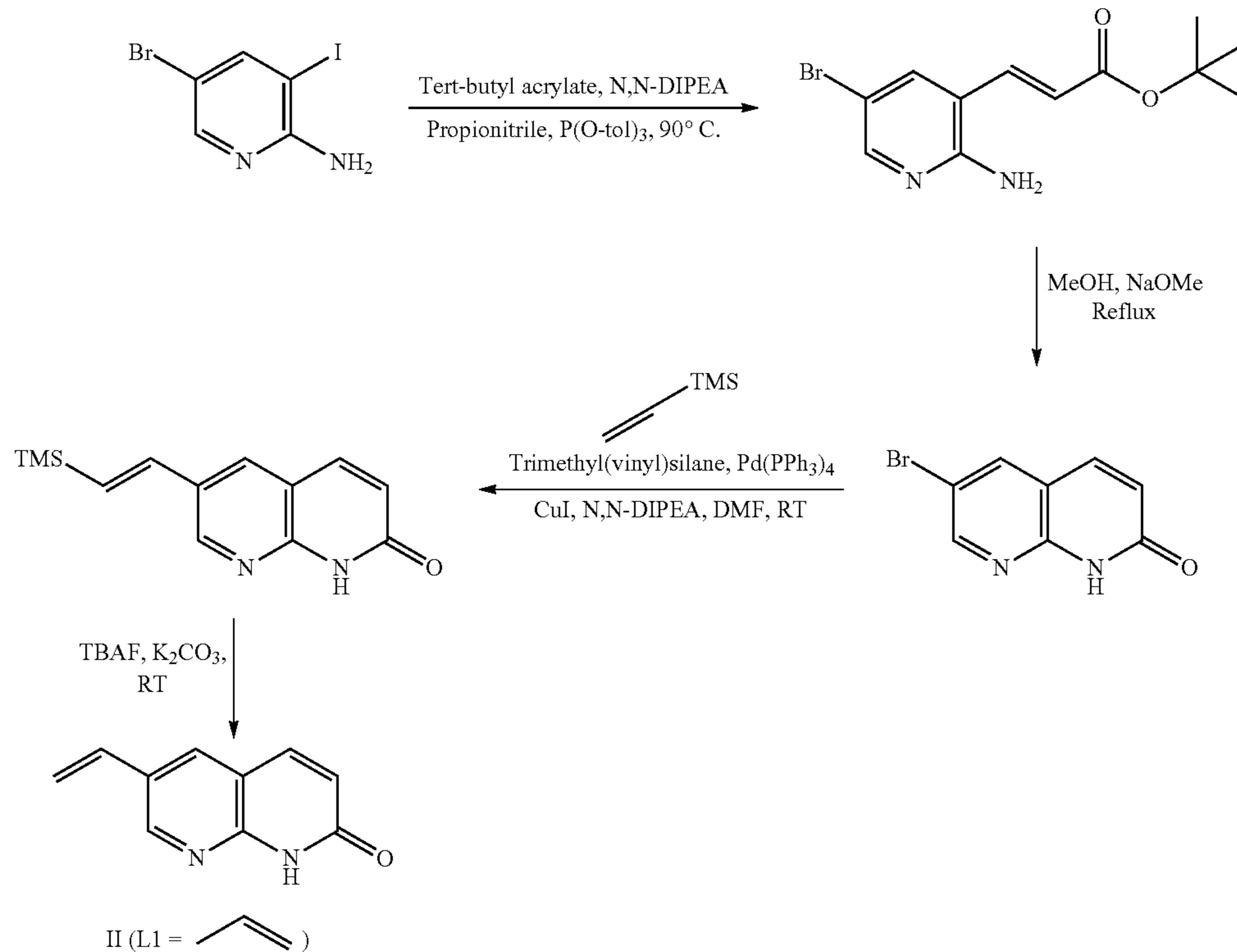
Scheme-3: Represents preparation of intermediates-II: (Second set)
