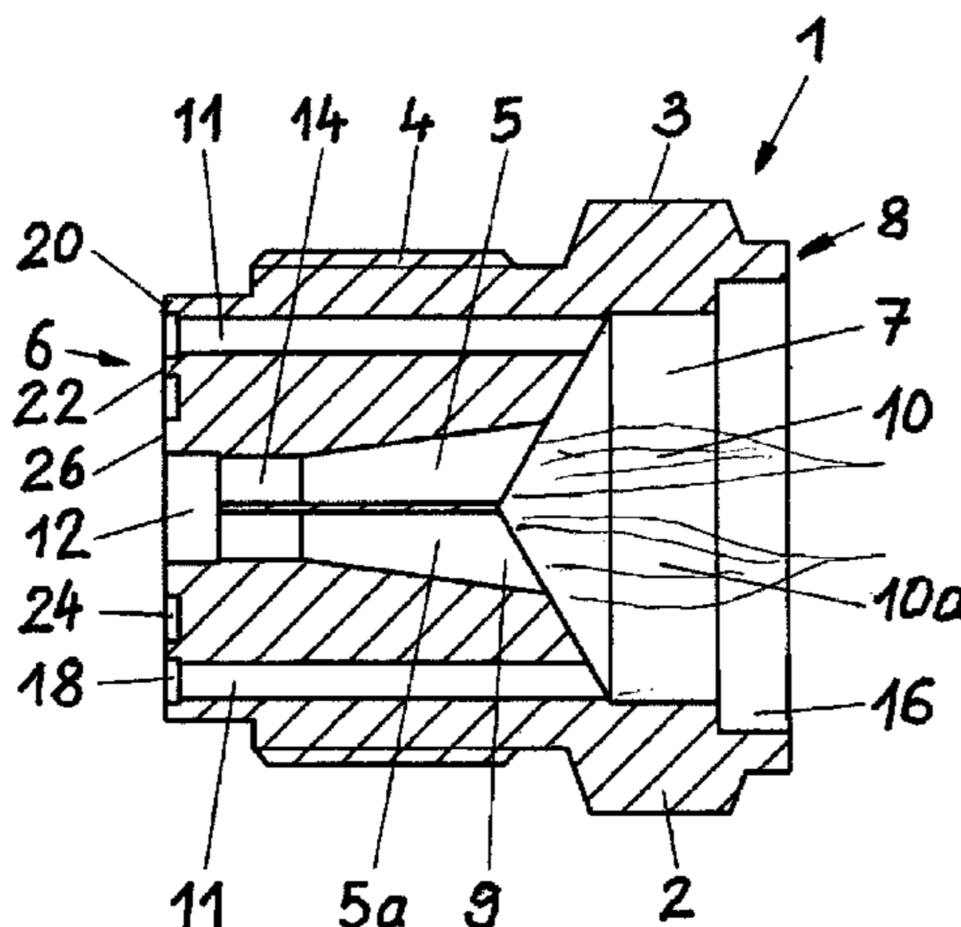
Cross-section A-A
