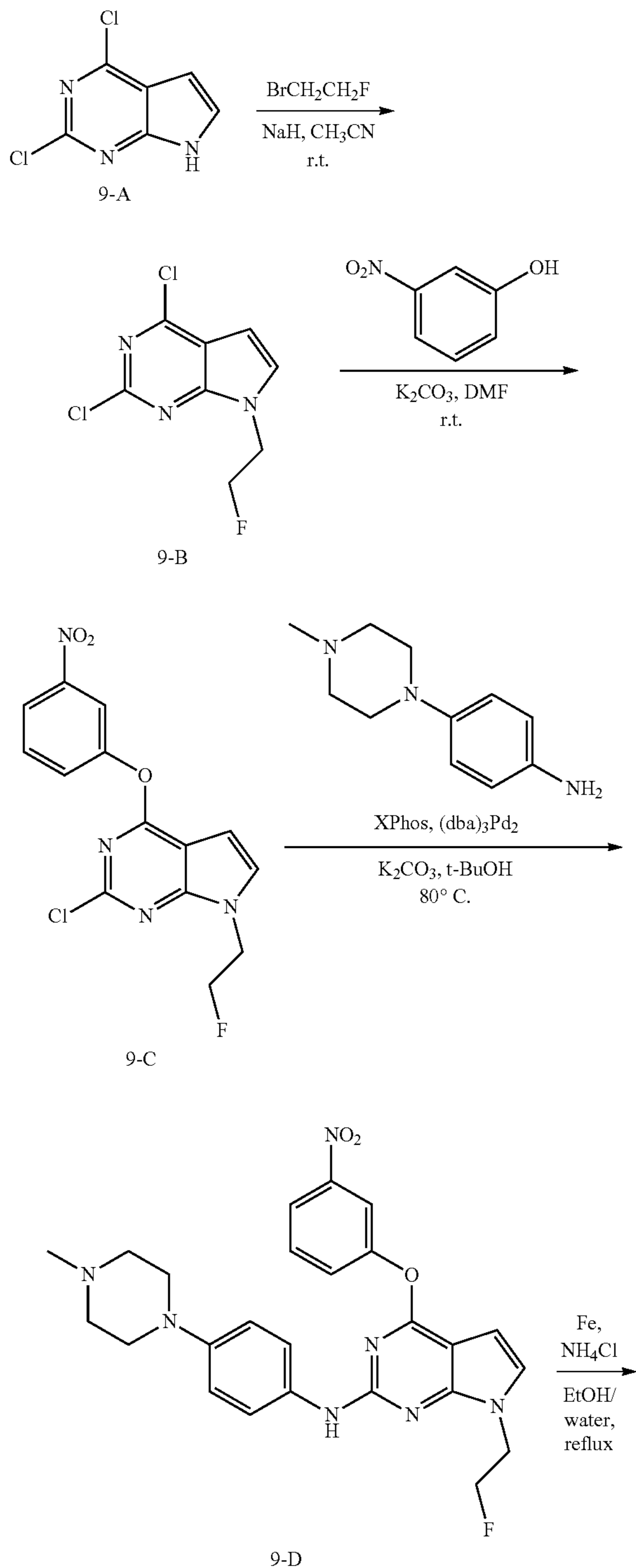
Scheme 9
