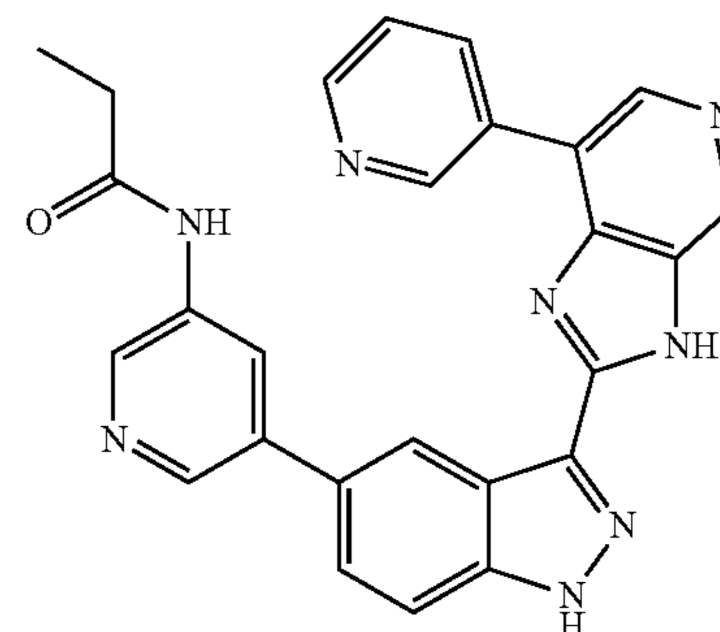
N-(5-(3-(7-(pyridin-3-yl)-3H-imidazo[4,5-c]pyridin-2-yl)-1H-indazol-5-yl)pyridin-3-yl)propionamide 4
