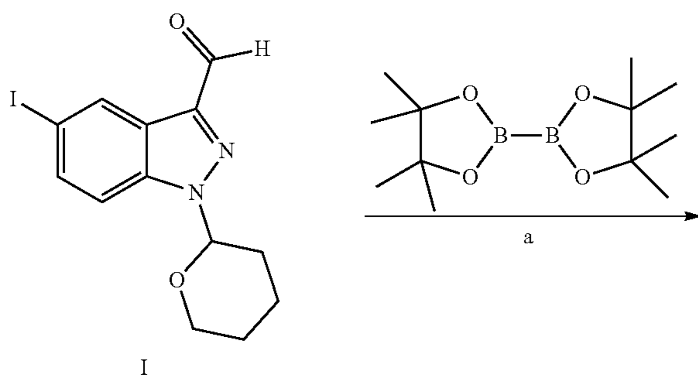
Scheme 6
