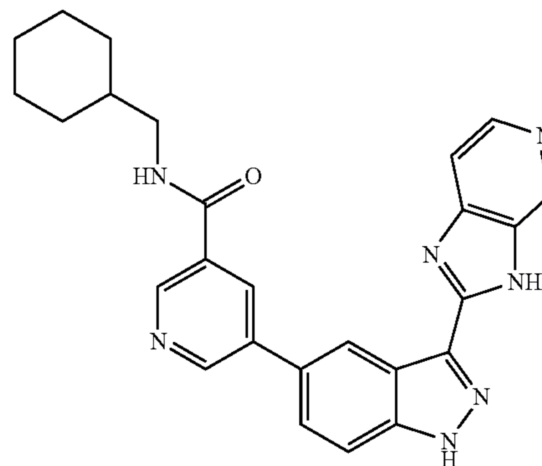
5-(3-(3H-imidazo[4,5-c]pyridin-2-yl)-1H-indazol-5-yl)-N-(cyclohexyl methyl)nicotinamide 2
