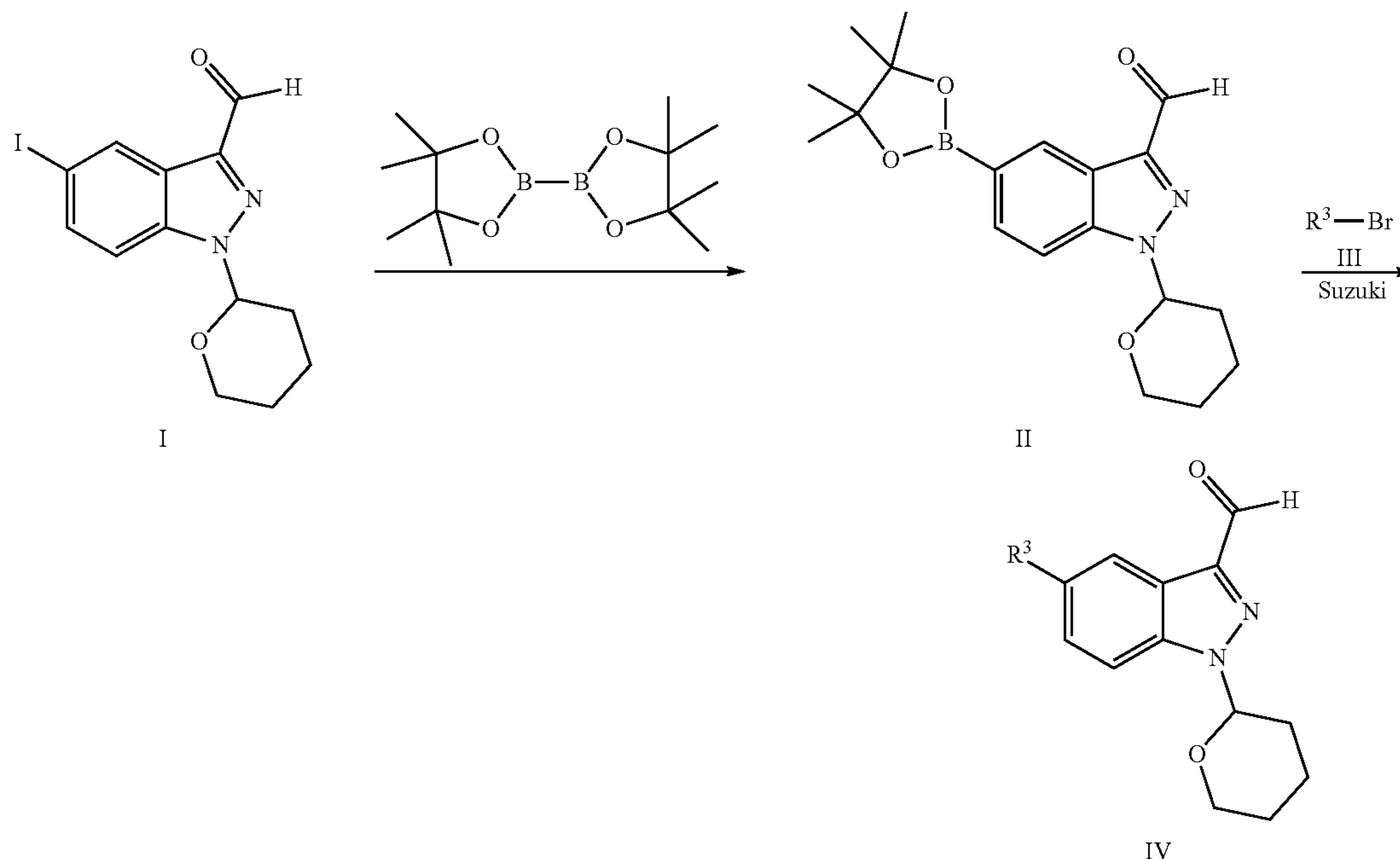
Scheme 1
