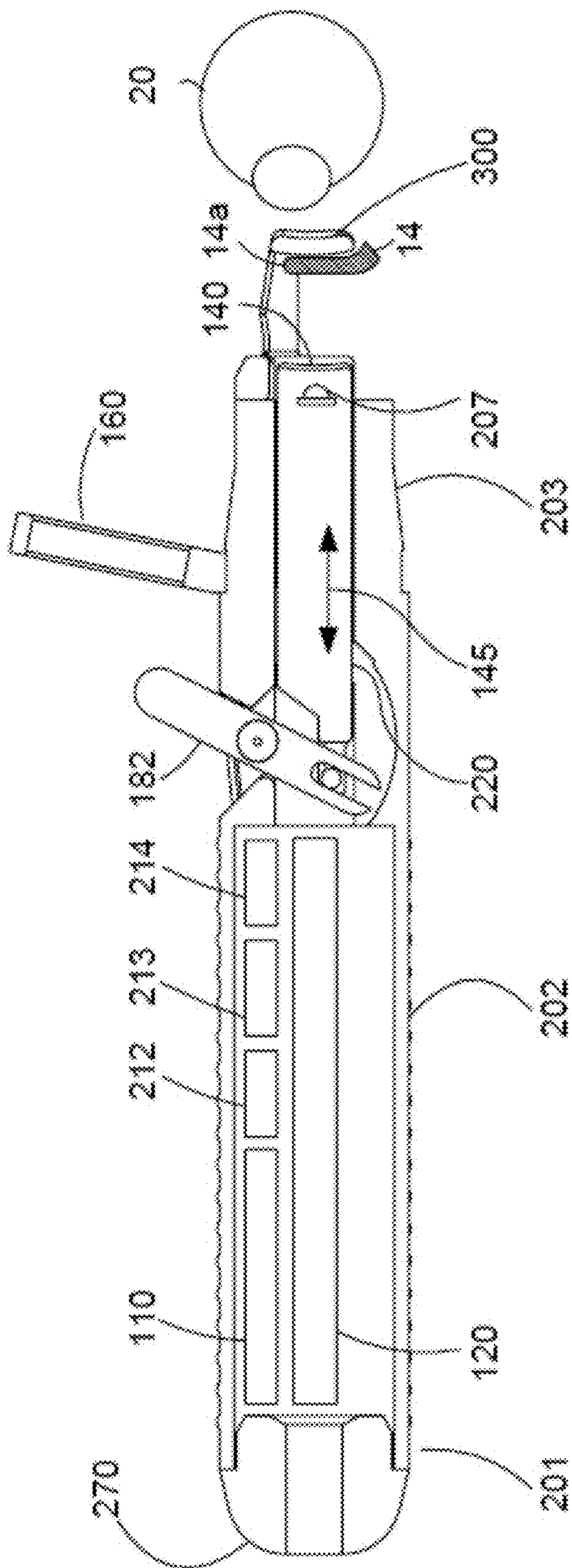
SECTION B-B
