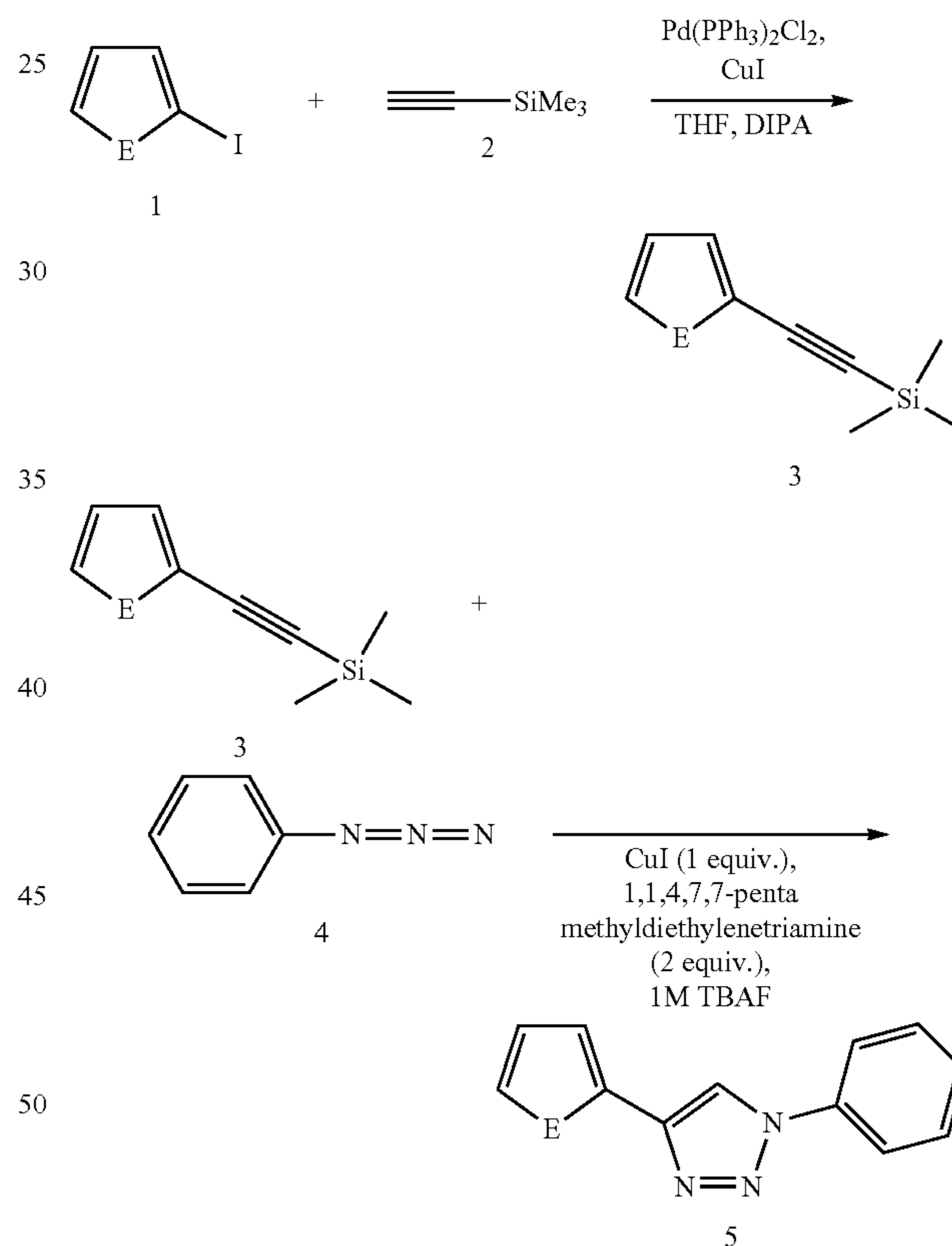
Scheme 1: Synthetic scheme for the preparation of compounds of Formula Ia
