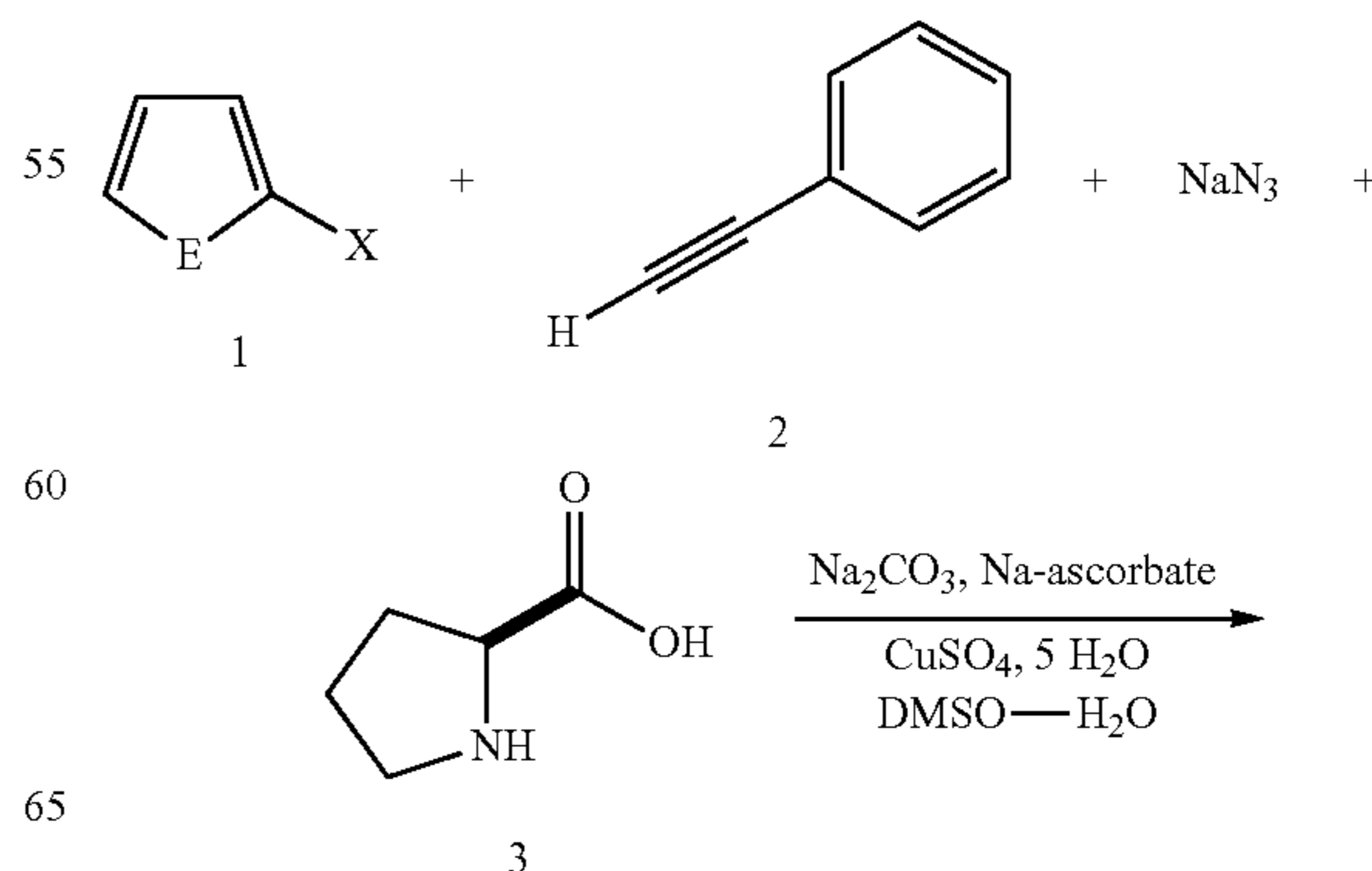
Scheme 6: Synthetic scheme for the preparation of compounds of Formula IIa
