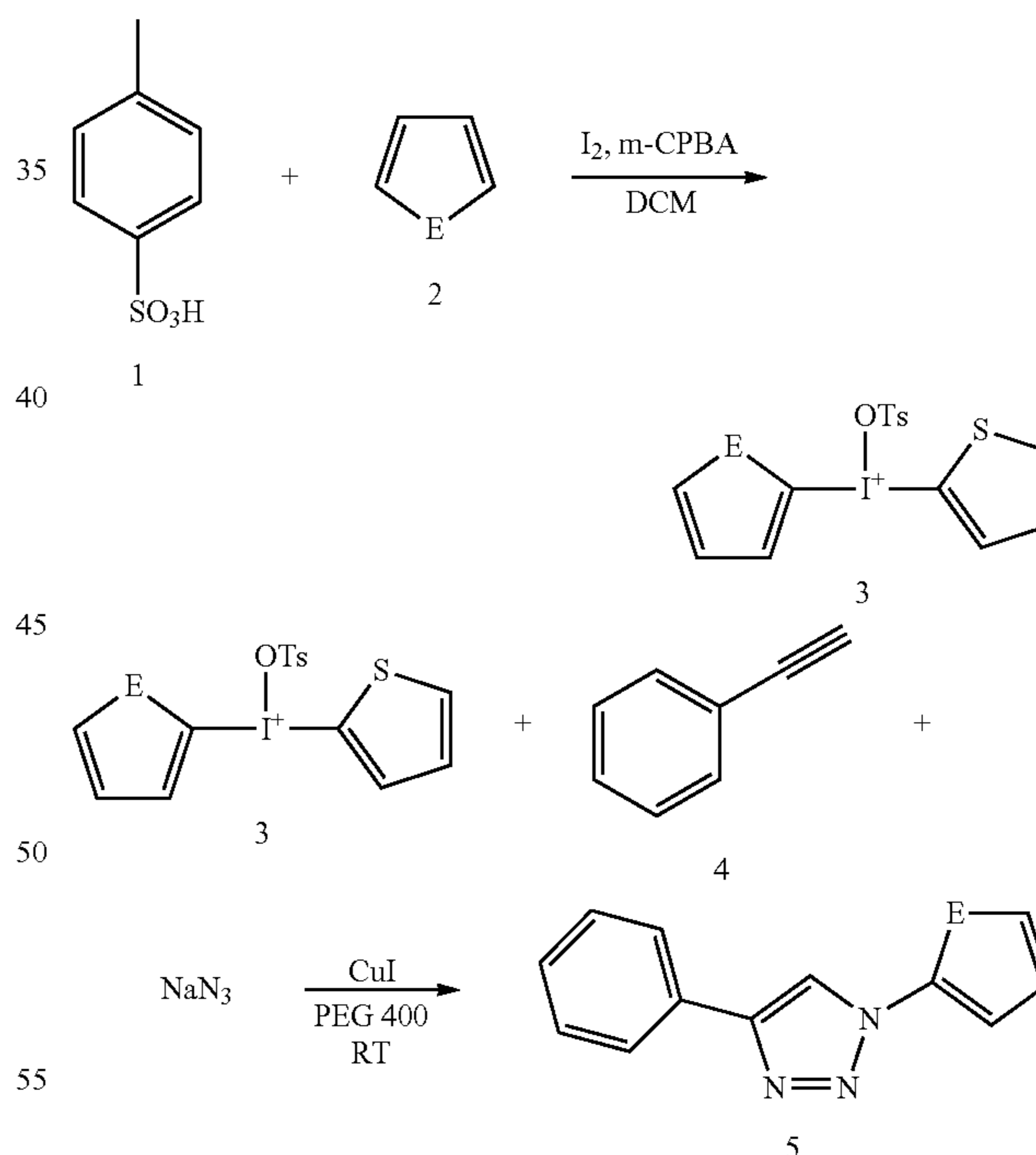
Scheme 7: Synthetic scheme for the preparation of compounds of Formula IIa
