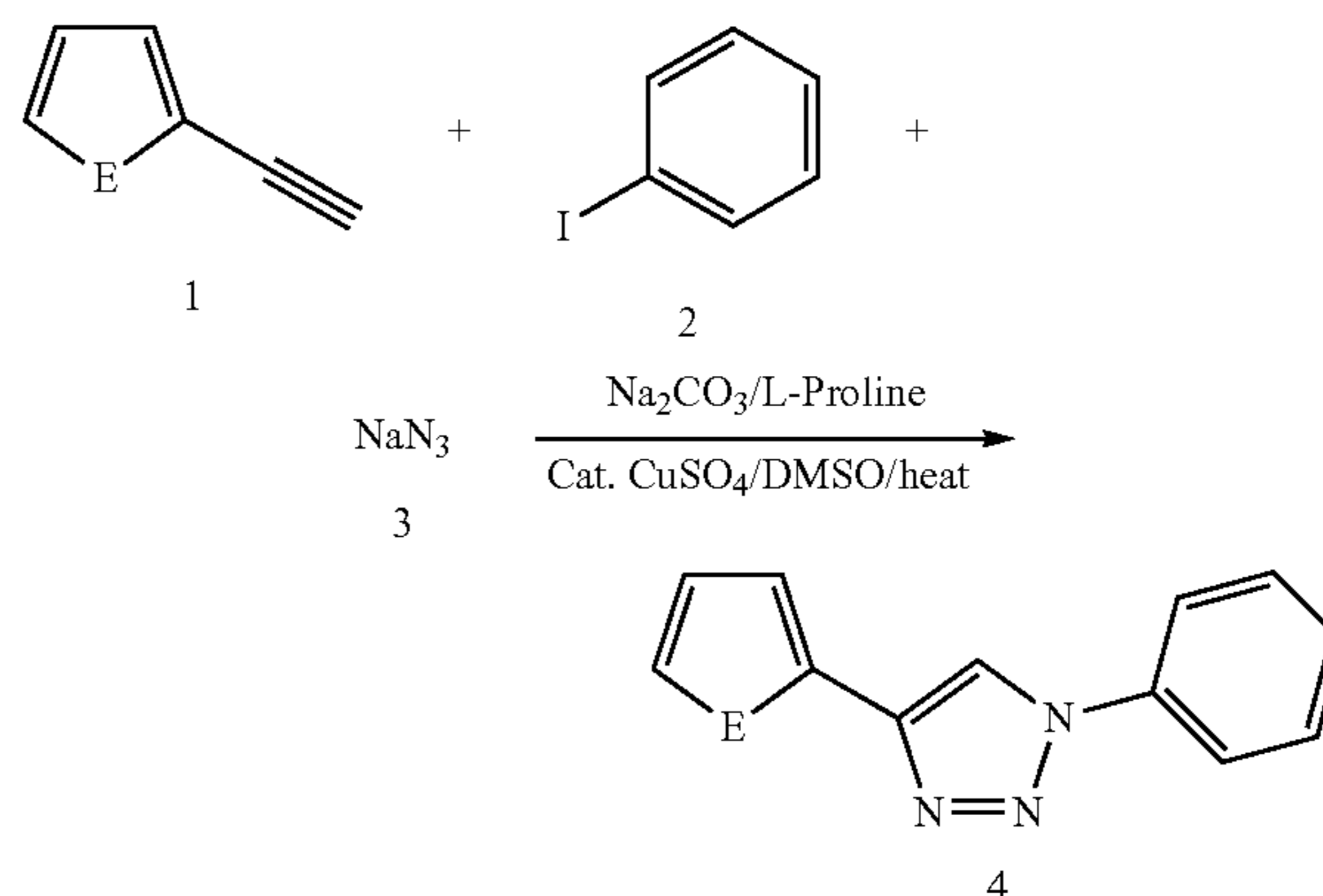
Scheme 2: Synthetic scheme for the preparation of compounds of Formula Ia
