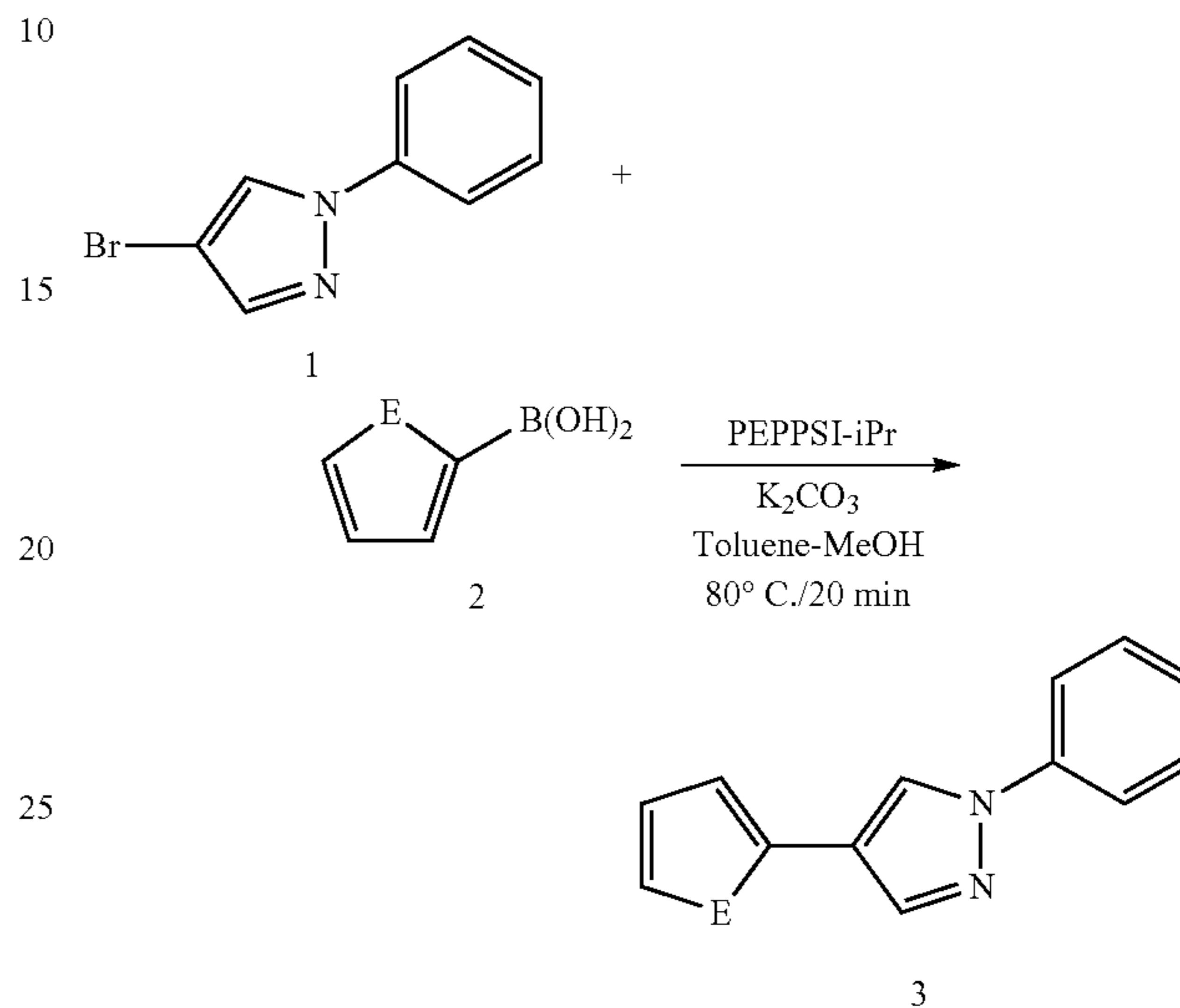
Scheme 3: Synthetic scheme for the preparation of compounds of Formula Ib
