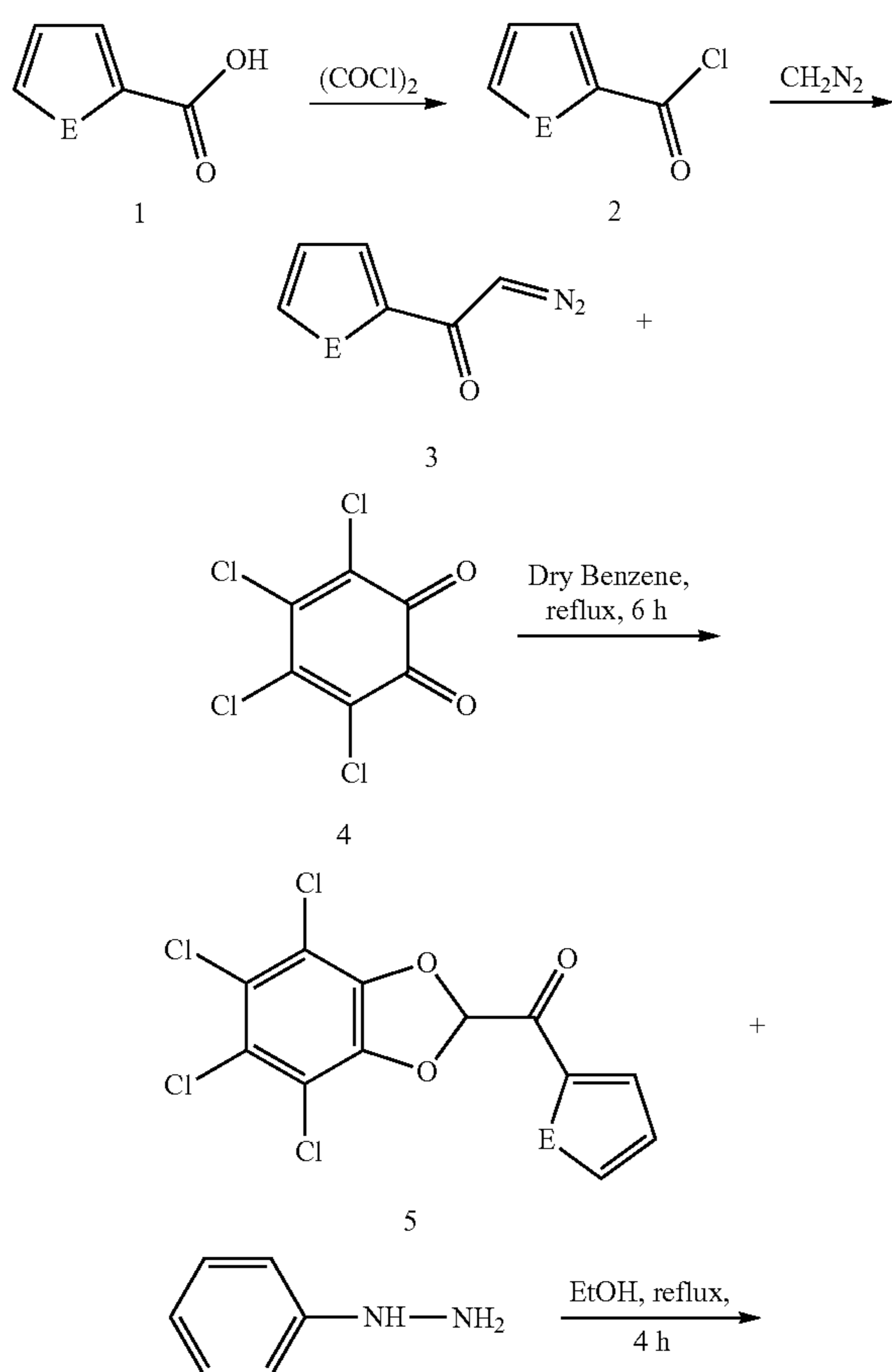
Scheme 5: Synthetic scheme for the preparation of compounds of Formula Id
